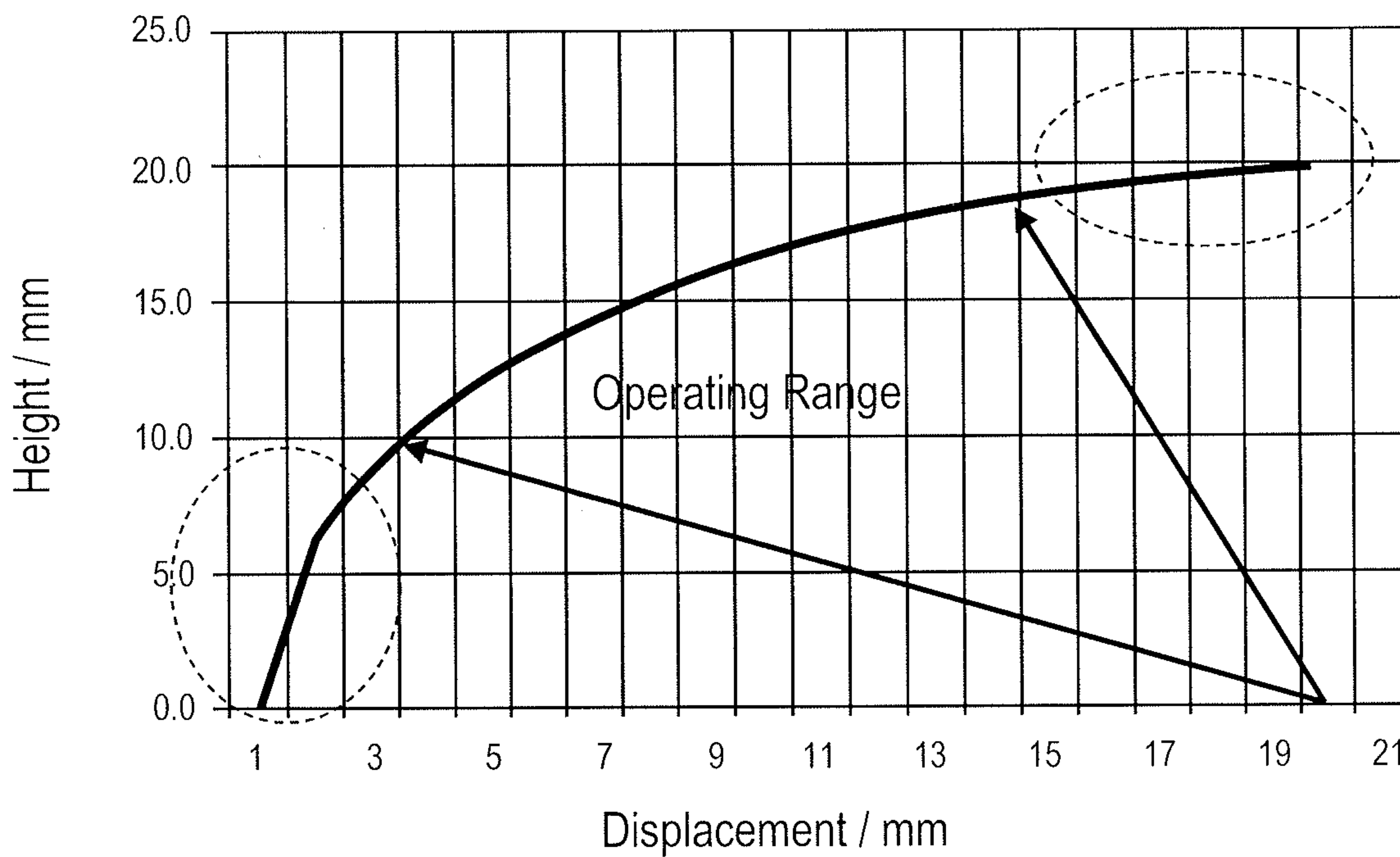
Platform Trajectory Link = 20 mm
