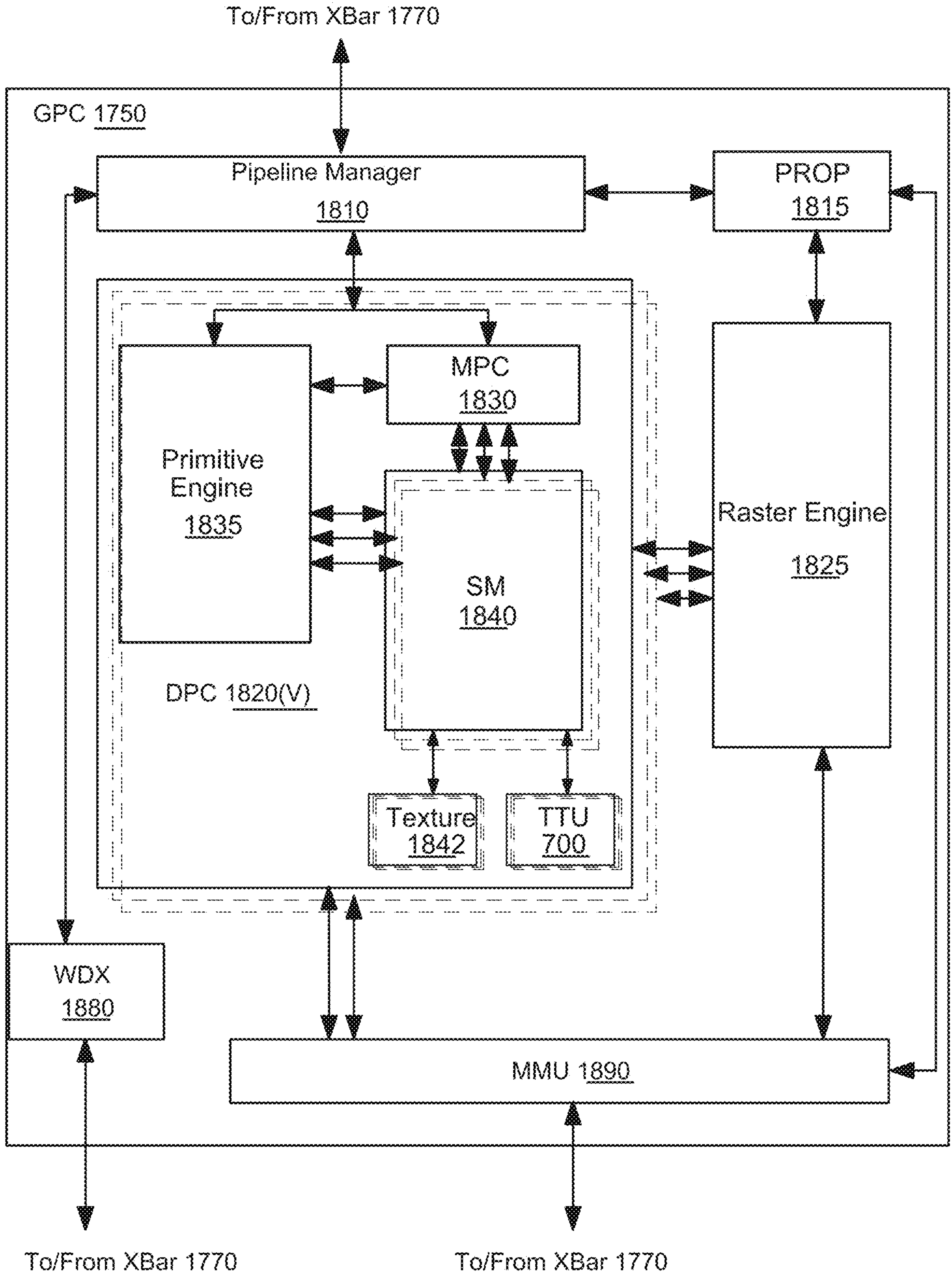
FIG. 17 Example General Processing Cluster
