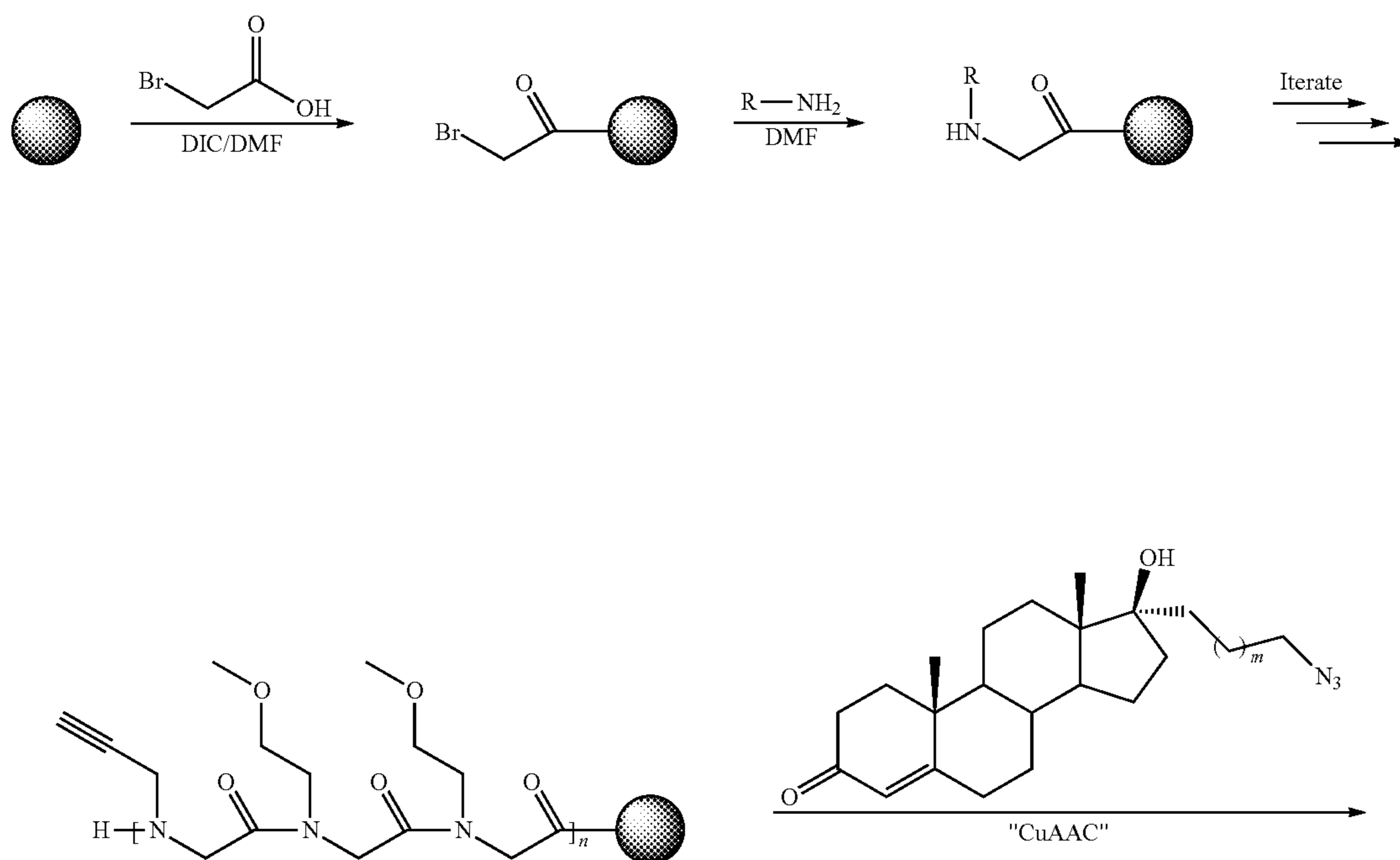
Scheme 2: Synthesis of Peptoid oligomers of the Invention
