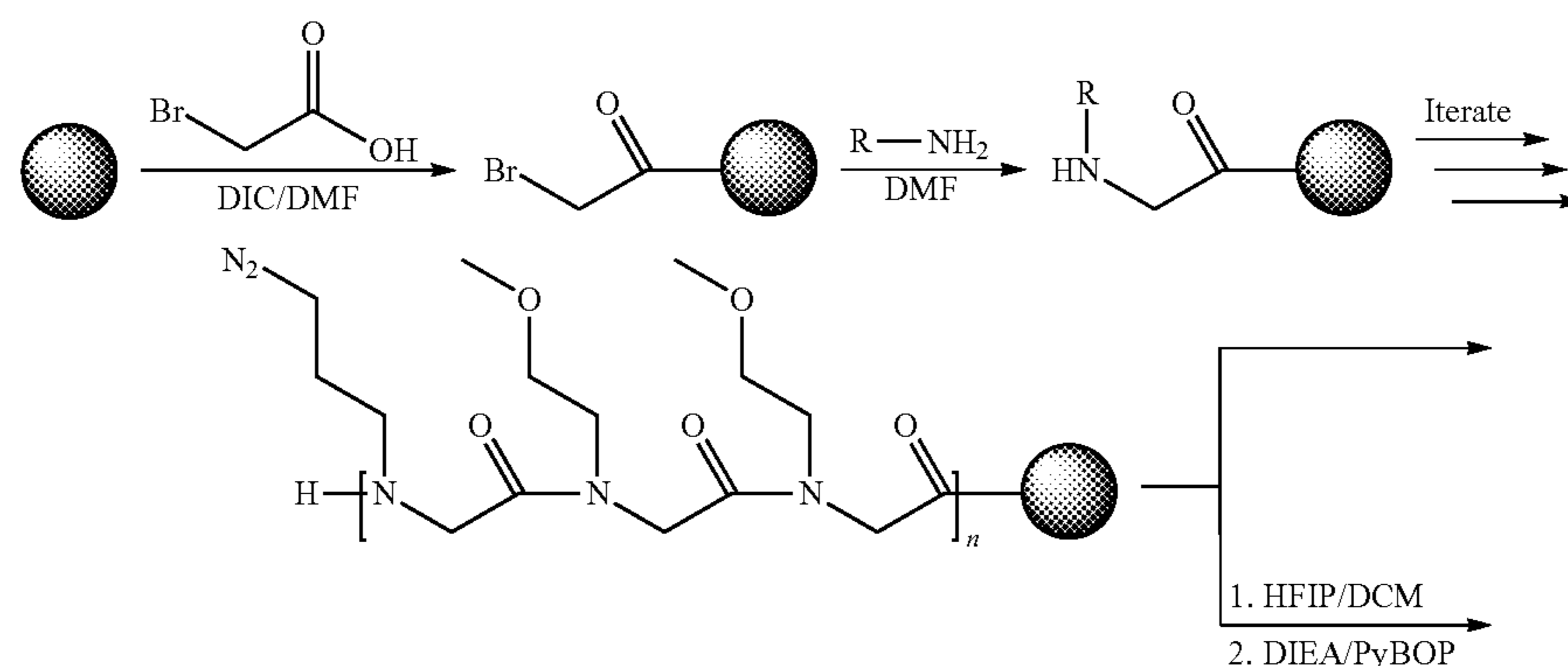
Scheme 1: Synthesis of Peptoid oligomers of the Invention a
