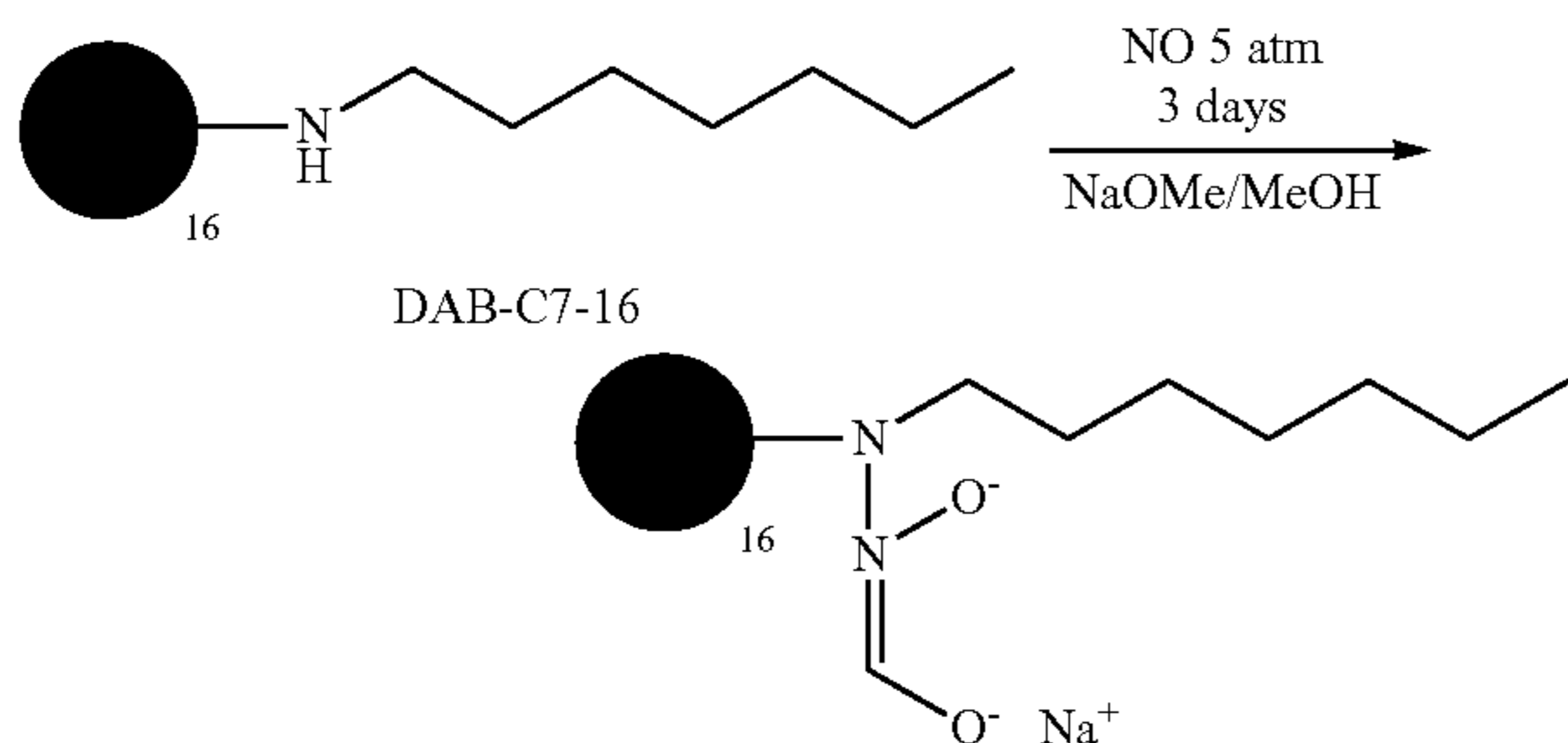
Scheme 5. Preparation of DAB-C7-16 diazeniumdiolate.
