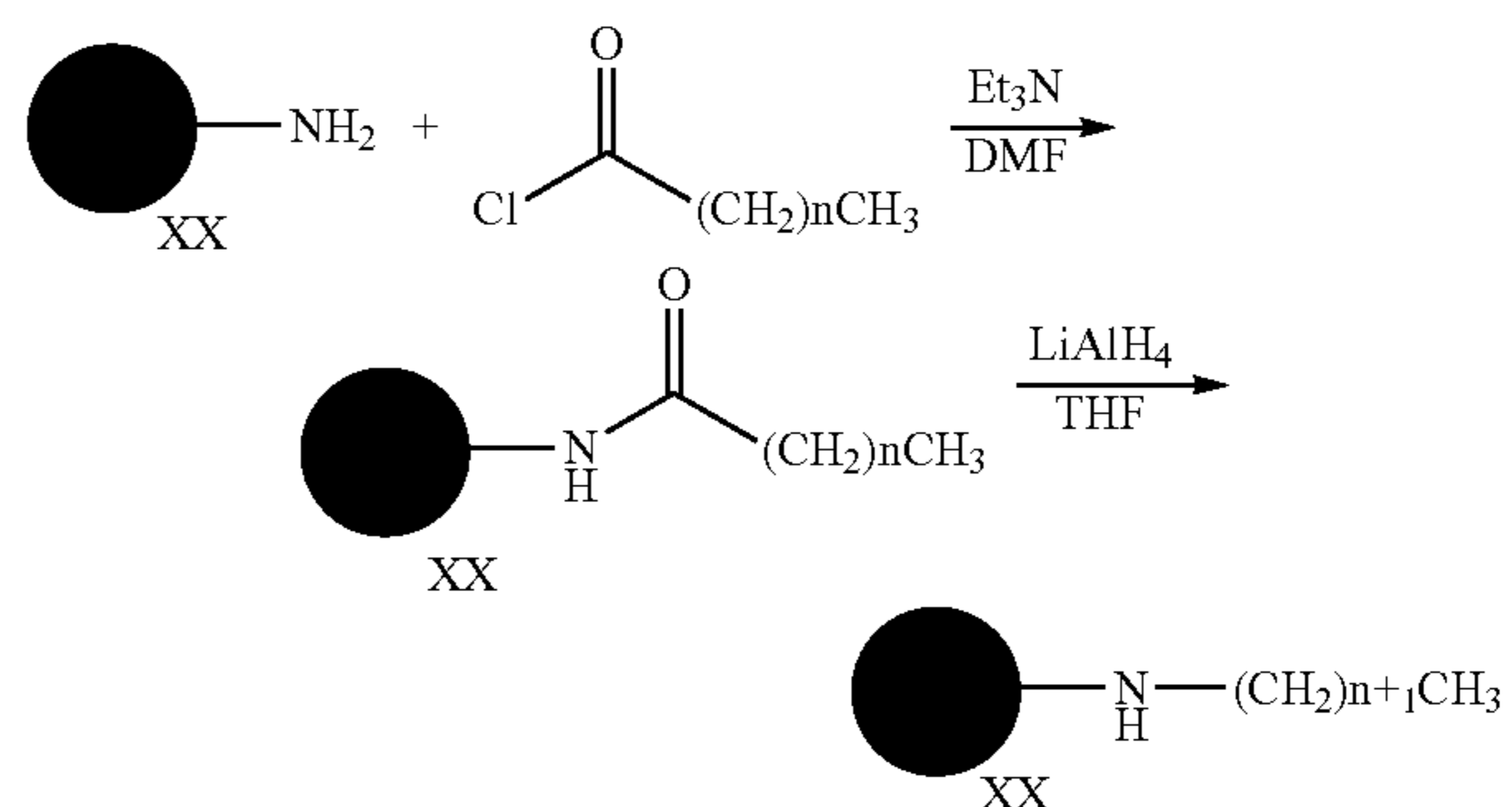
Scheme 3. General procedure for dendrimers with lipophilic tails.
