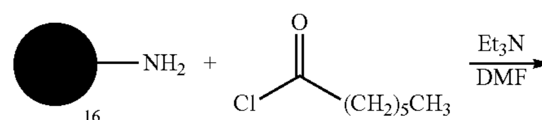
Scheme 4. Preparation of DAB-C7-16.
