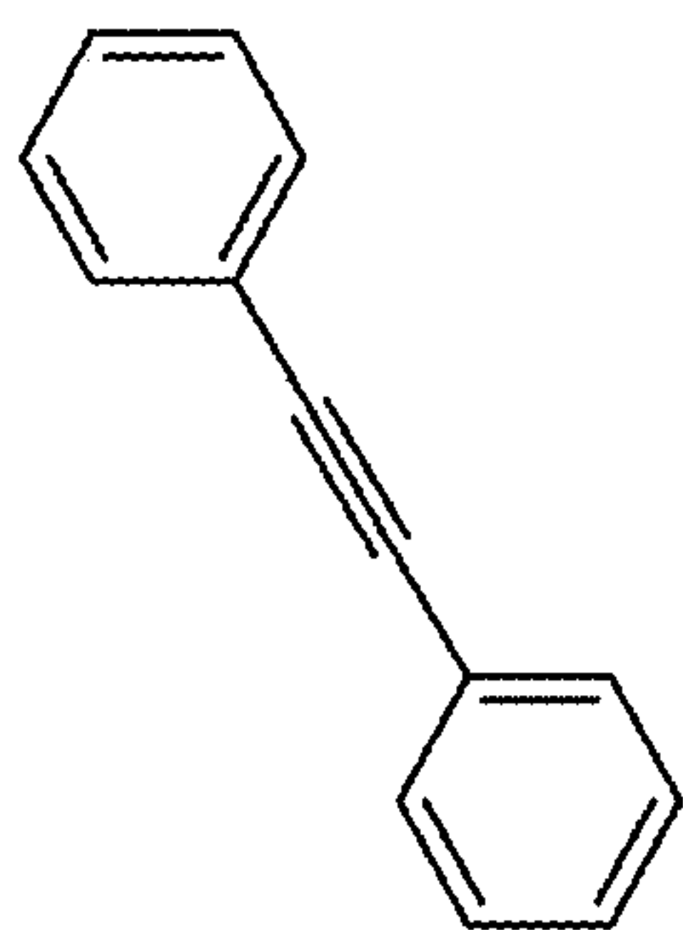
Diphenylacetylene
