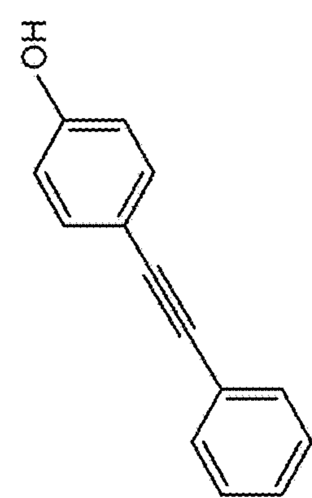
4-(2-Phenylethynyl)phenol
