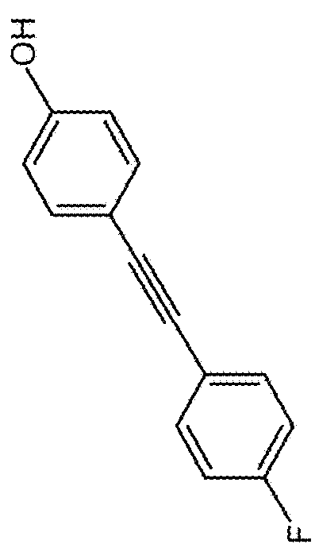
4-[(4-Flouropheny)]Ethyny]]phenol
