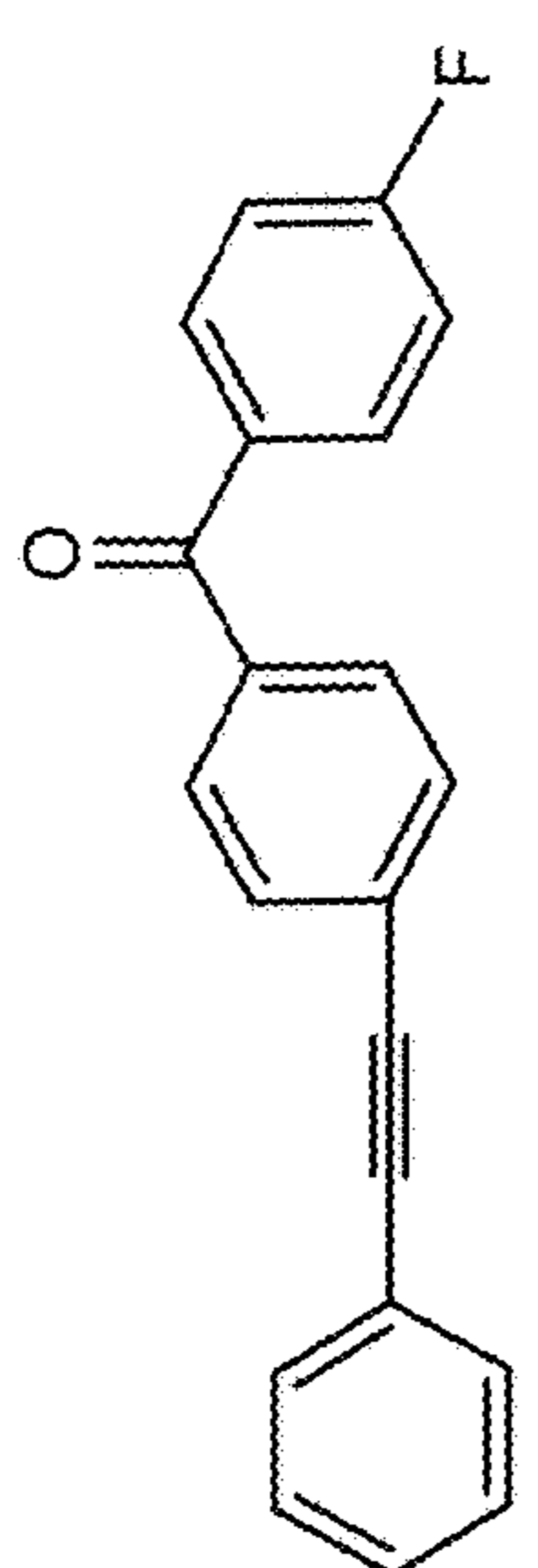
4-Flouro-4'-(Phenylethynyl)Benzophenone
