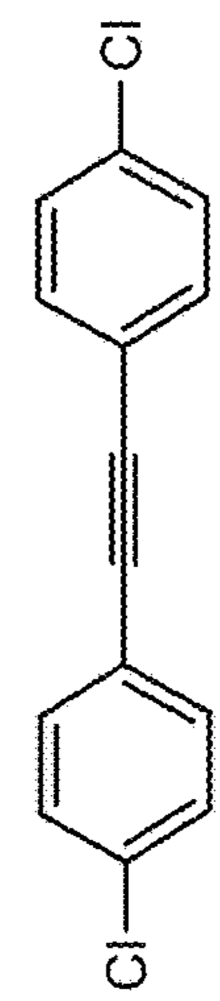
1-(4-Chlorophenylethynyl)-4-chlorobenzene
