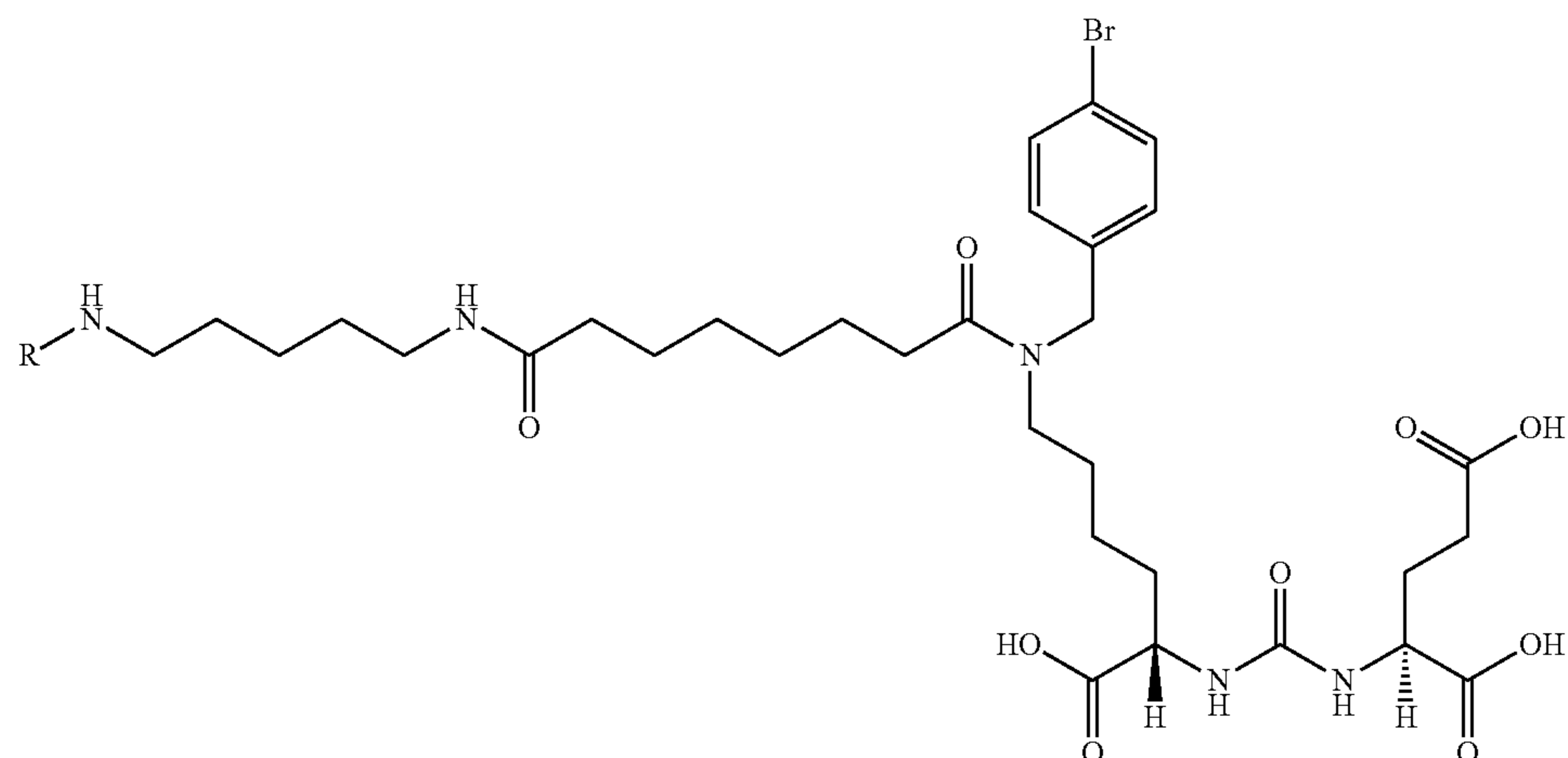
6: R = H DyLight800-6: R = DyLight800
