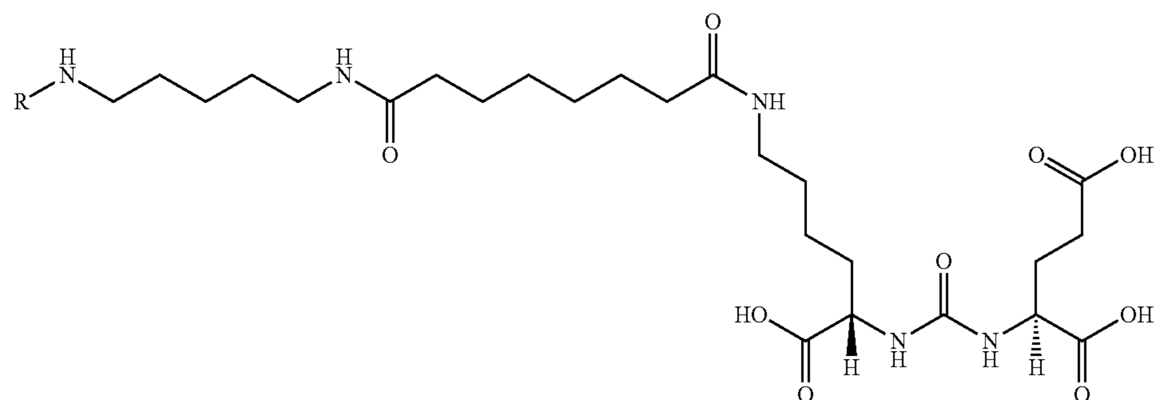
5: R = H DyLight800-5: R = DyLight800
