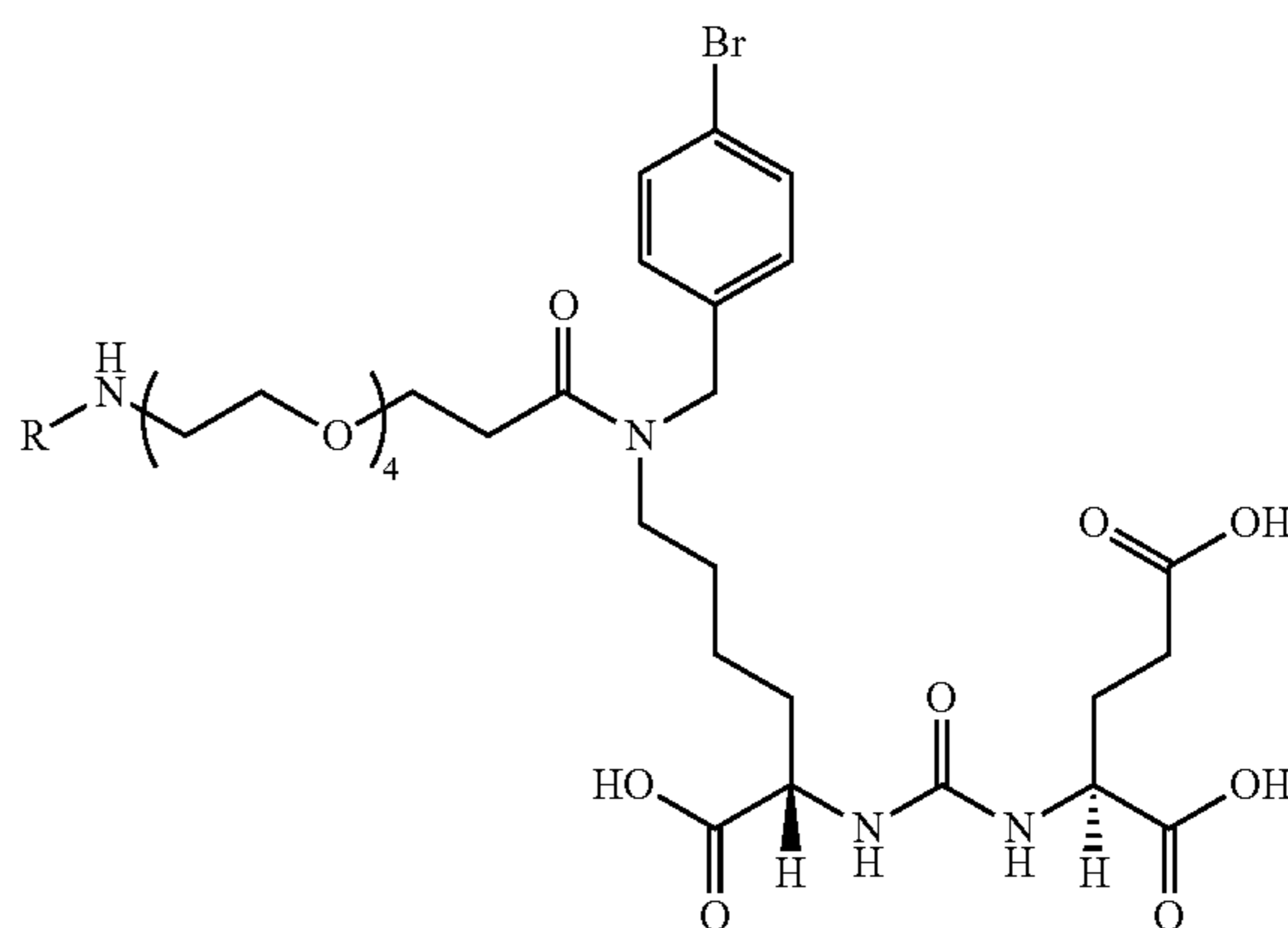
8: R = H DyLight800-8: R = DyLight800
