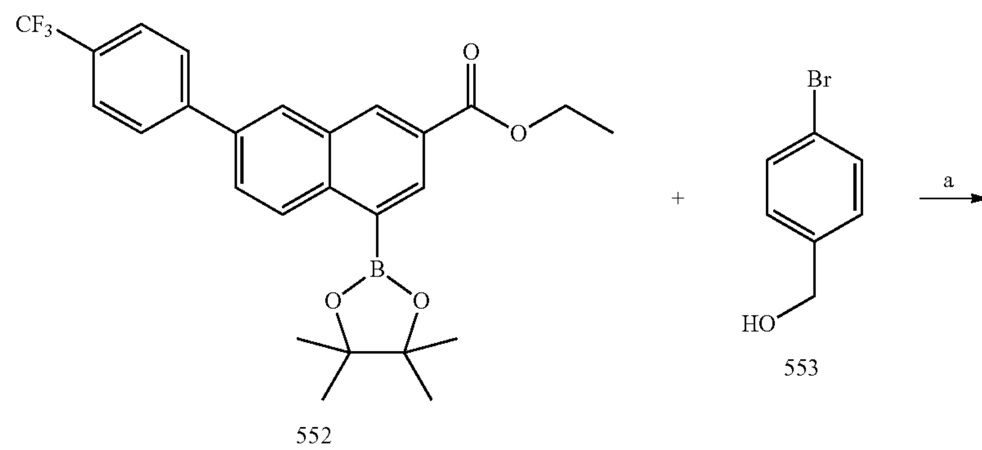
Scheme 25. Preparation of truncated PPTN-glucose analogue
