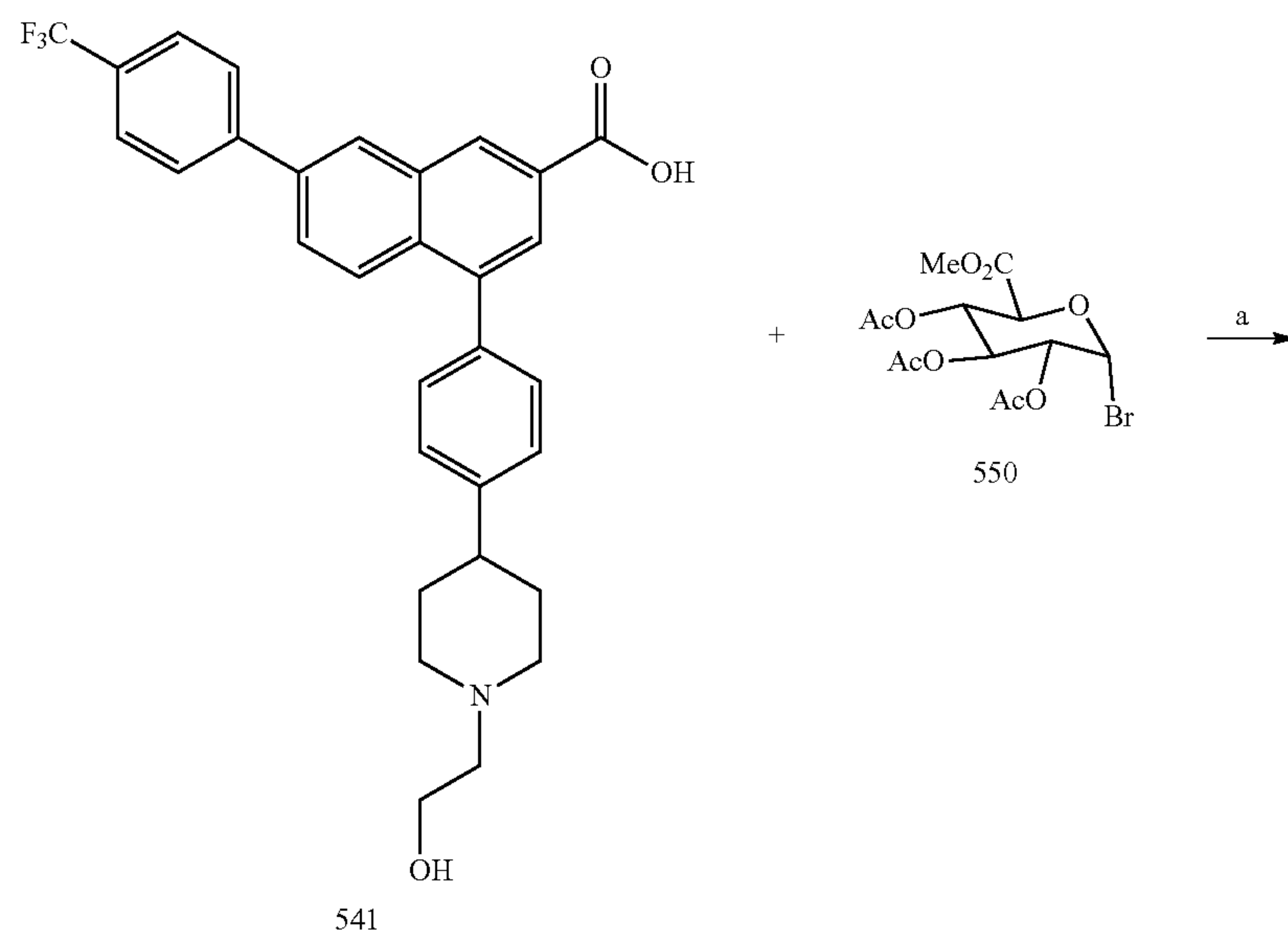
Scheme 24. Preparation of PPTN analogues with O-β-glucuronide
