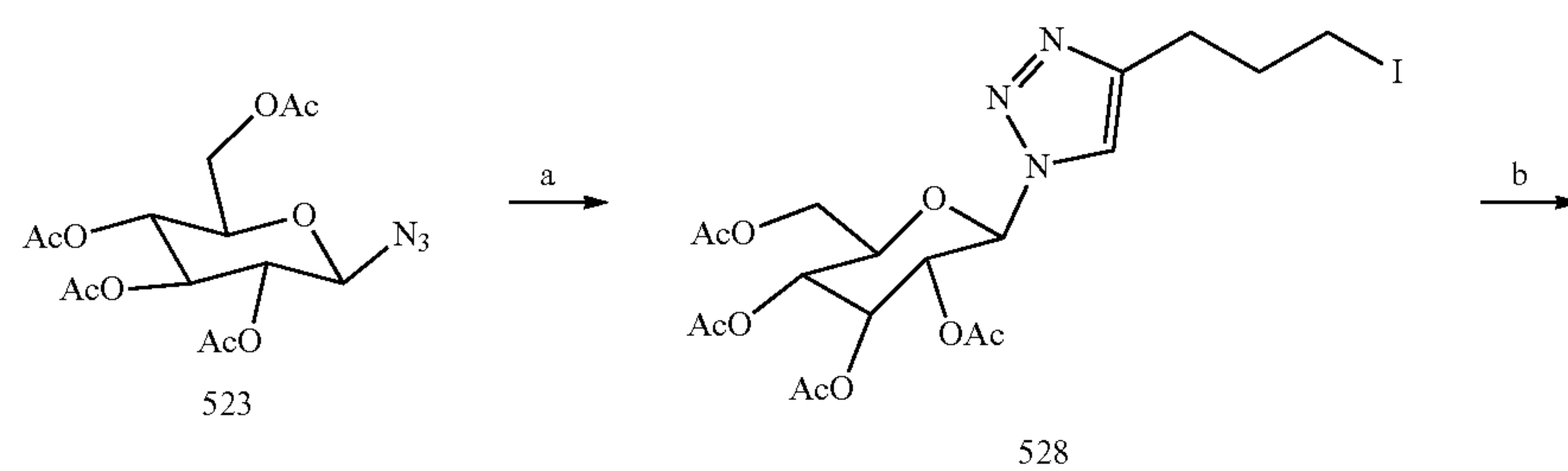
Scheme 19. PPTN-glucose analogues bridged with propyltriazolyl linker
