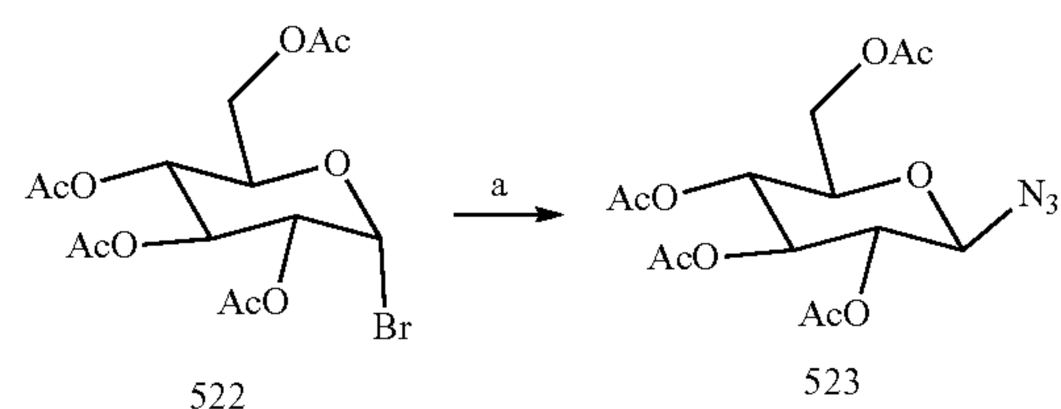
Scheme 18. PPTN analogues with \beta -D-glucose bridged by triazole
