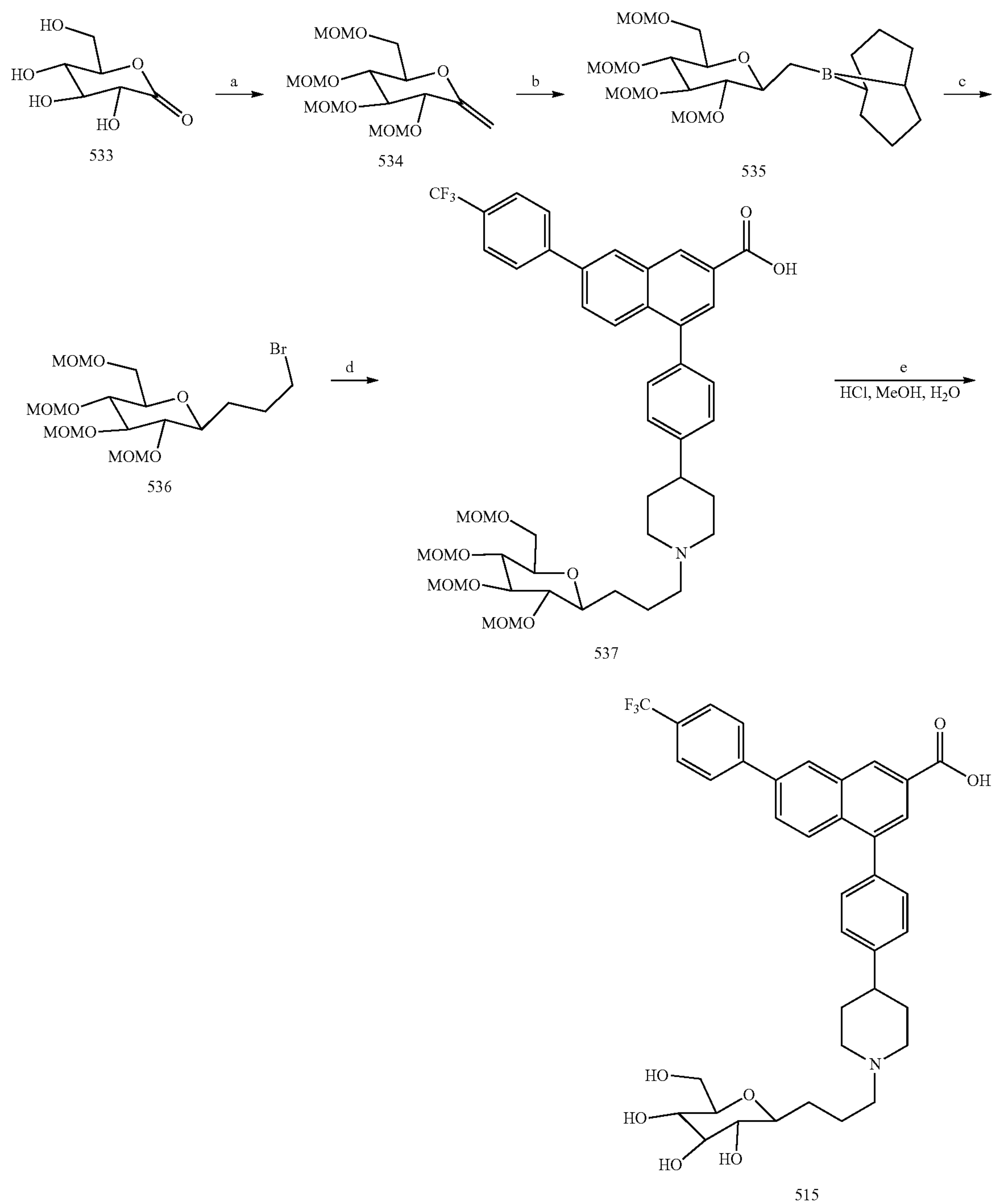
Scheme 21. Alternative synthetic strategy for the preparation of C-b-D-glycosyl
