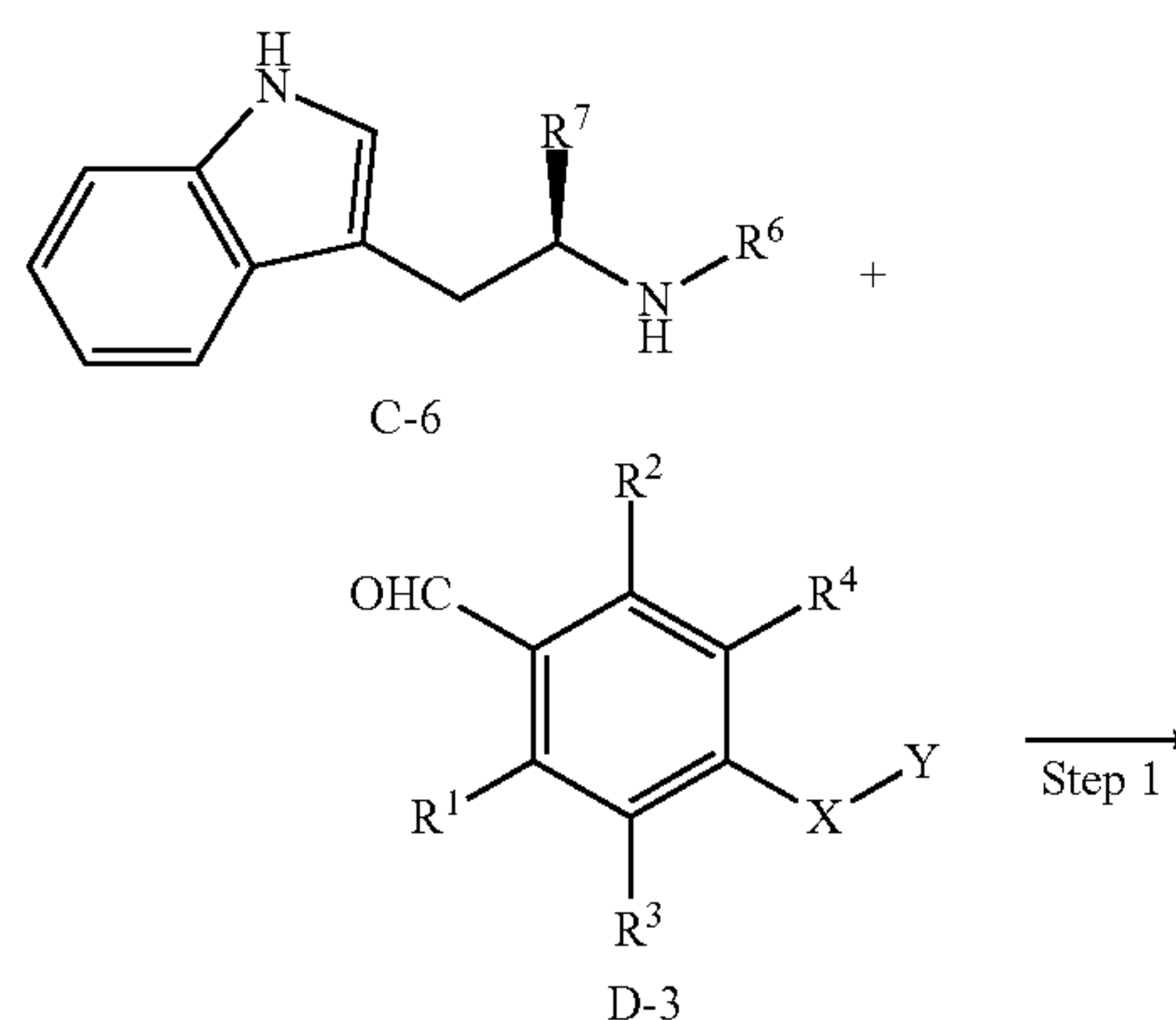
SCHEME D
