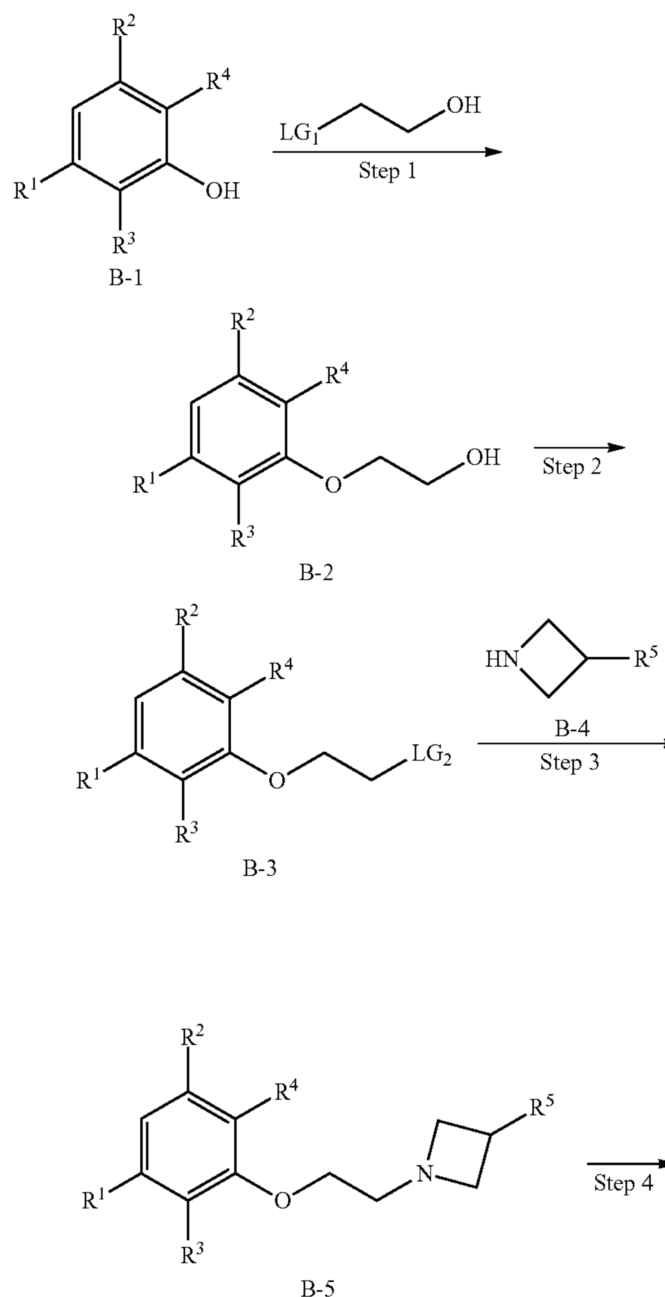
SCHEME B
