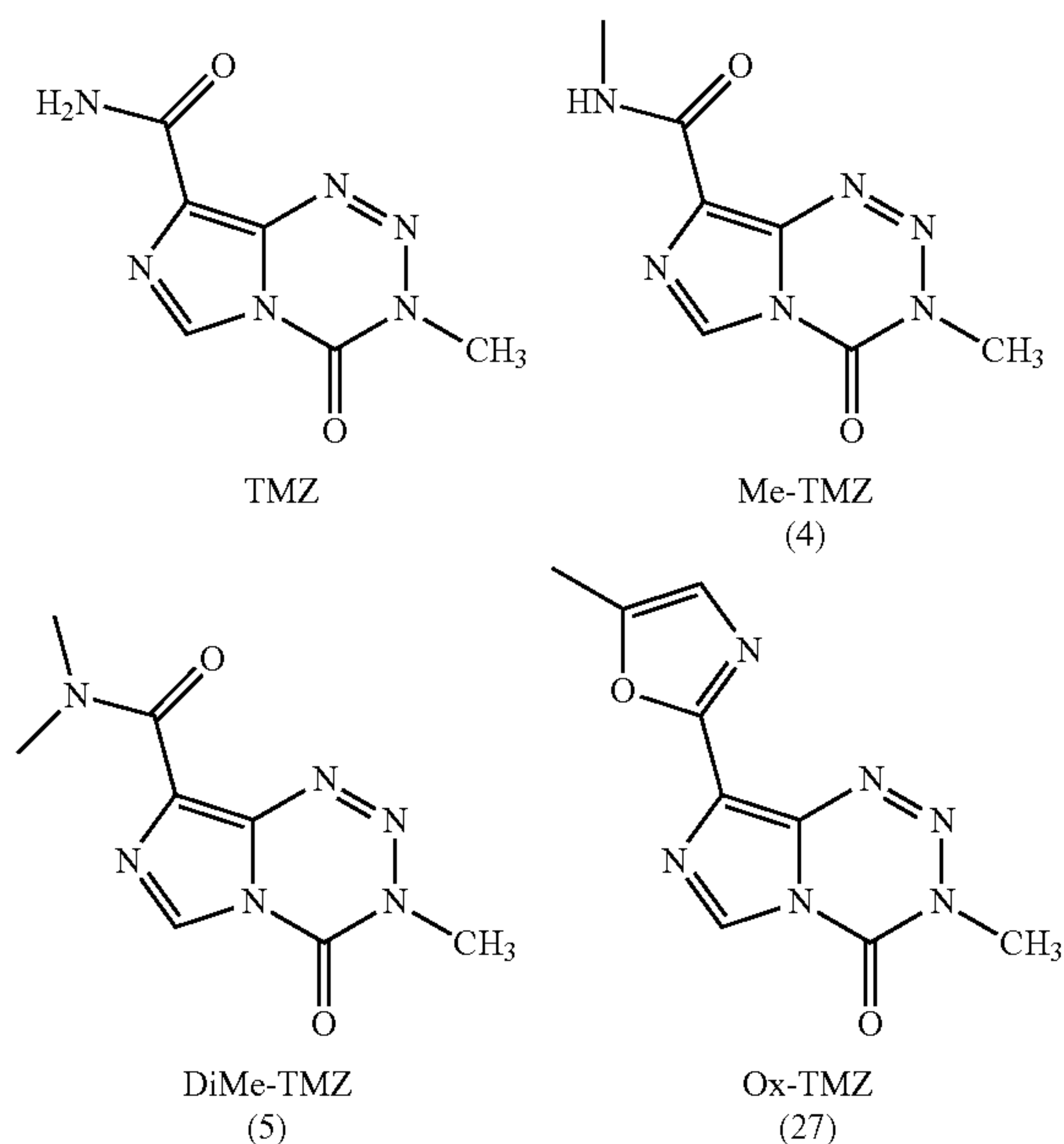
Scheme 2b. Structures of lead C8-substituted compounds. Blood-brain barrier permeability of imidazotetrazines (see Figure 2).
