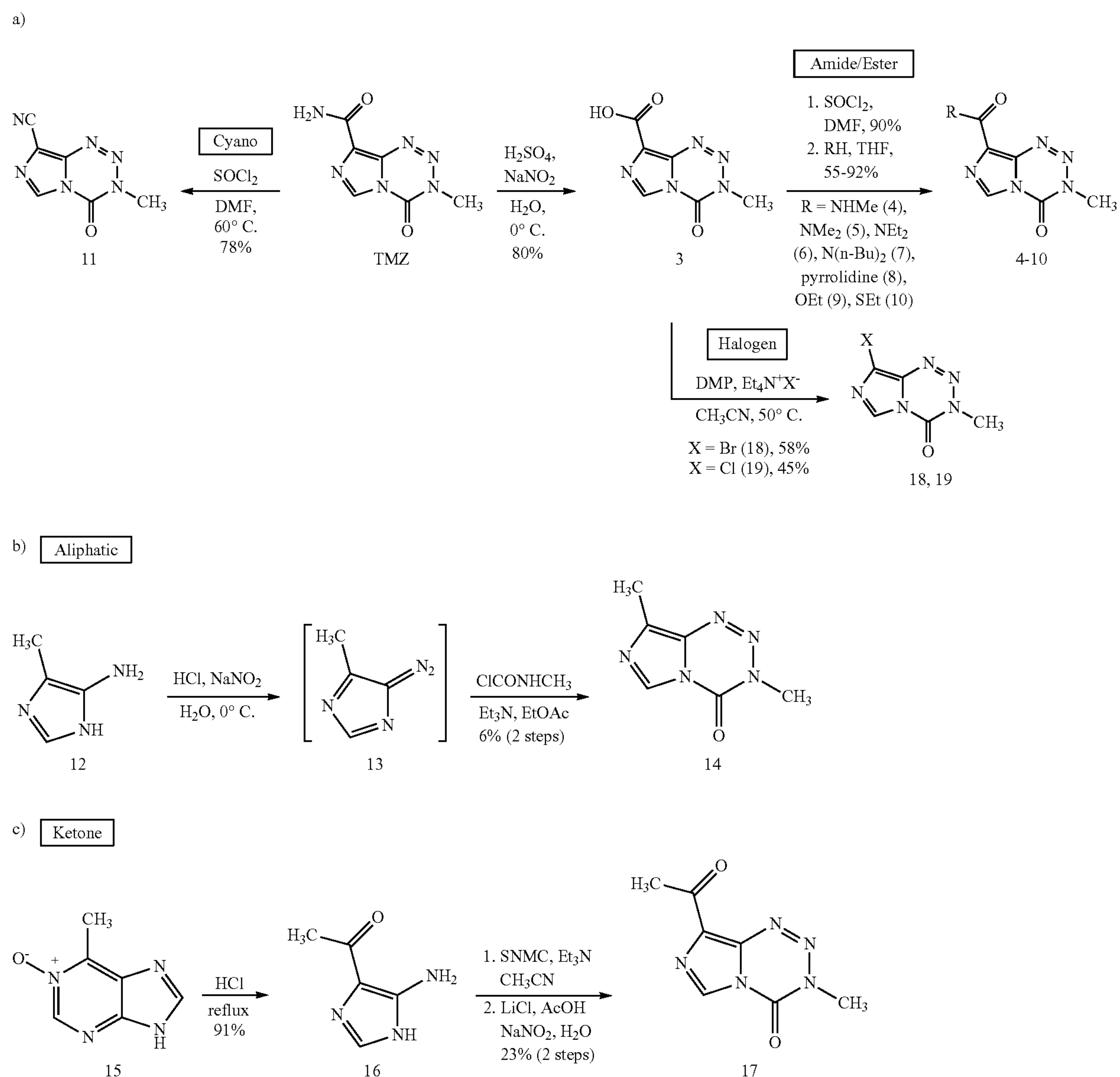
Scheme 2. Synthesis of novel C8-substituted imidazotetrazines.
