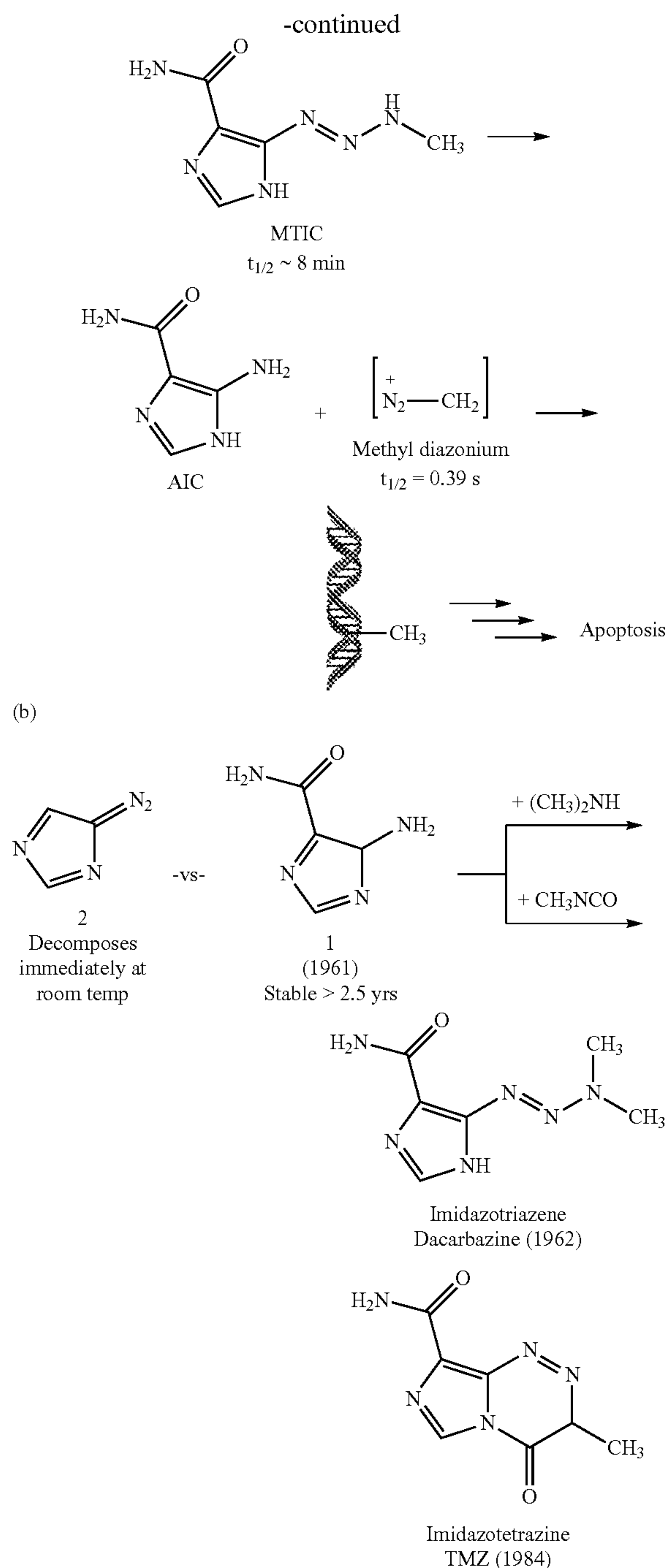
(a) Mechanism of temozolomide (TMZ) activation in aqueous solution. (b) The favorable stability of compound 1 relative to related versions (such as 2) accounts for the incorporation of the amide at C8 of TMZ.
