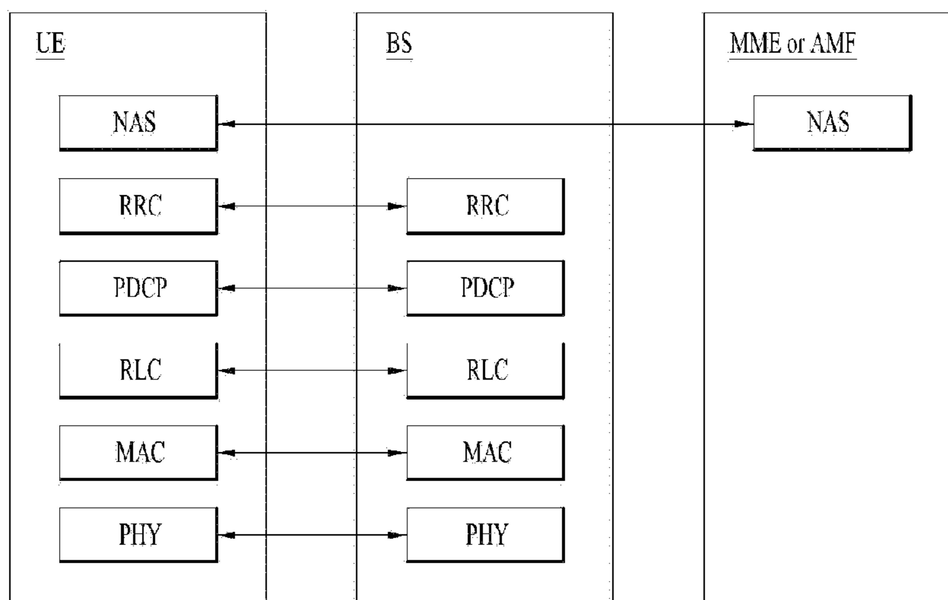
(b) Control Plane Protocol Stack
