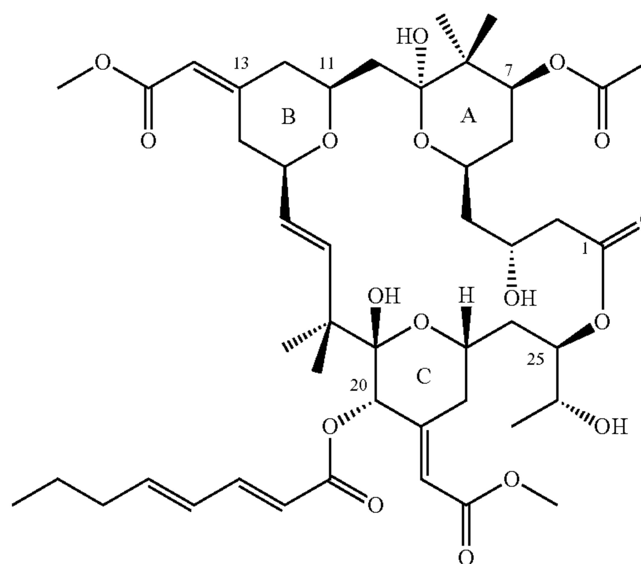
Bryostatin 1
