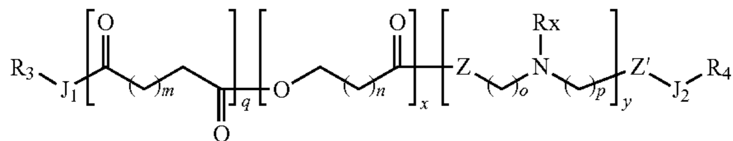
Formula II
