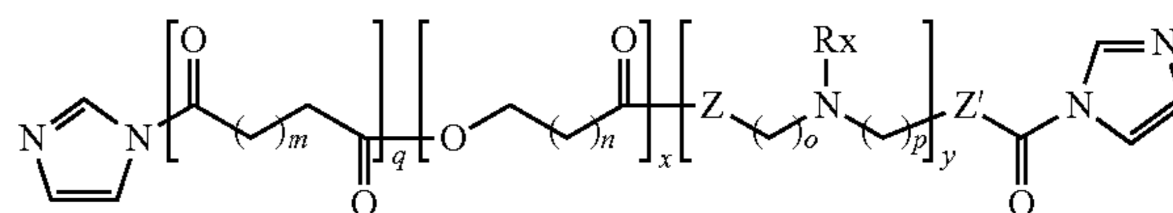
Formula IV
