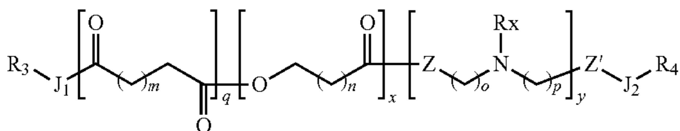
Formula II
