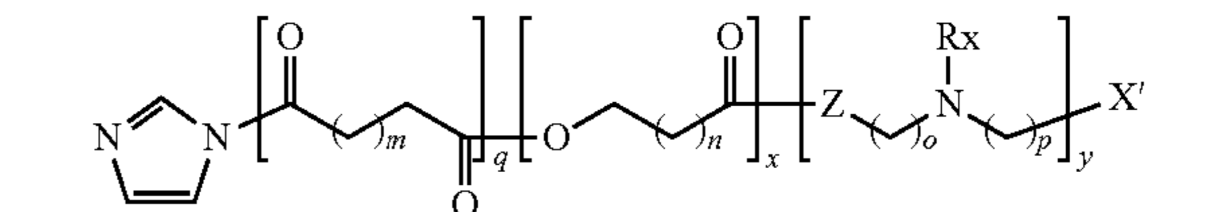
Formula VI
