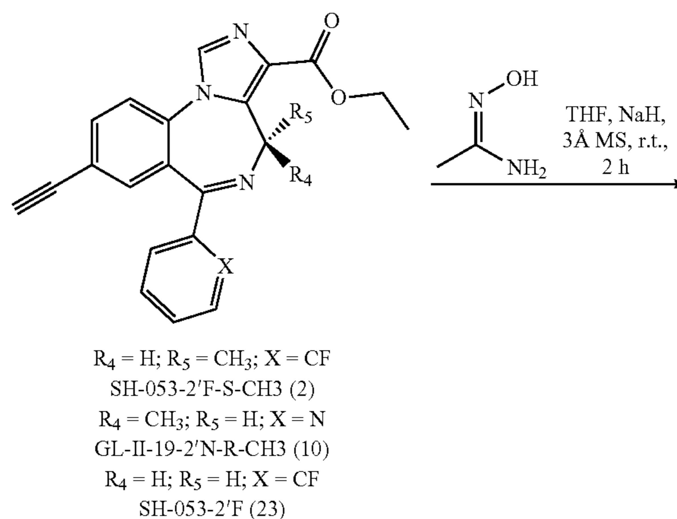
Scheme 10. General synthetic route to oxadiazoles.
