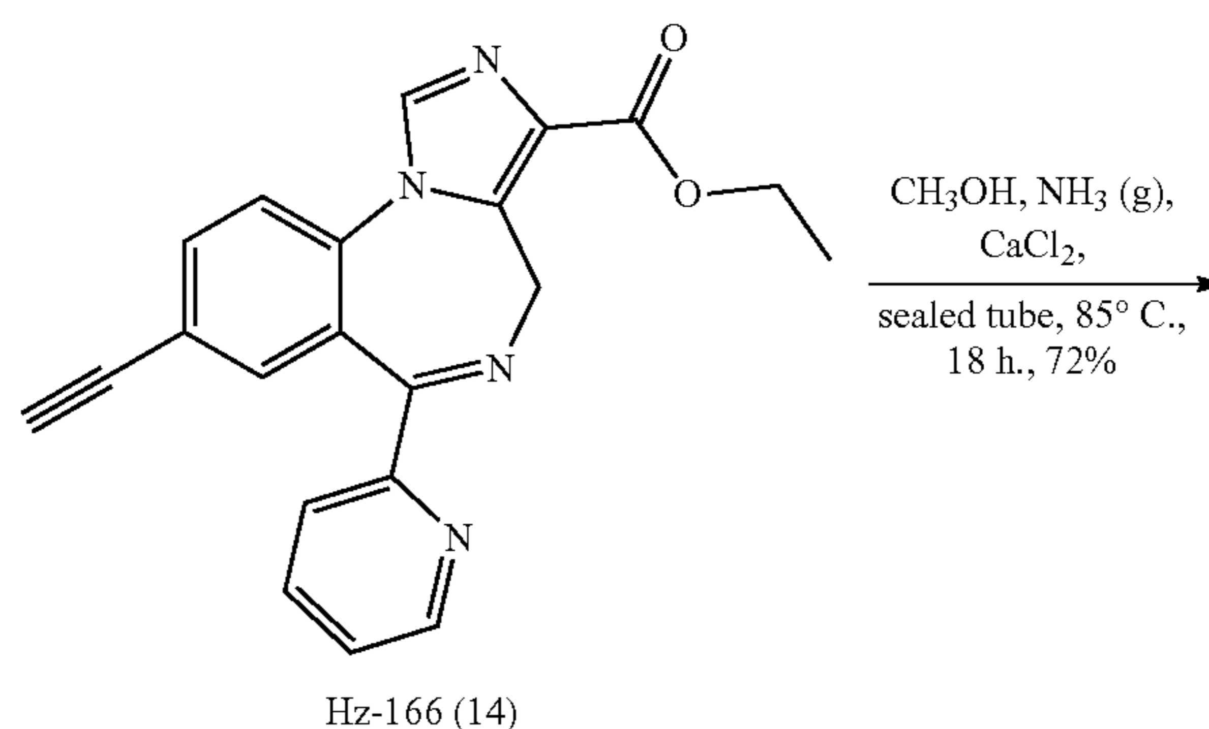
Scheme 6. Synthesis of MP-II-065.
