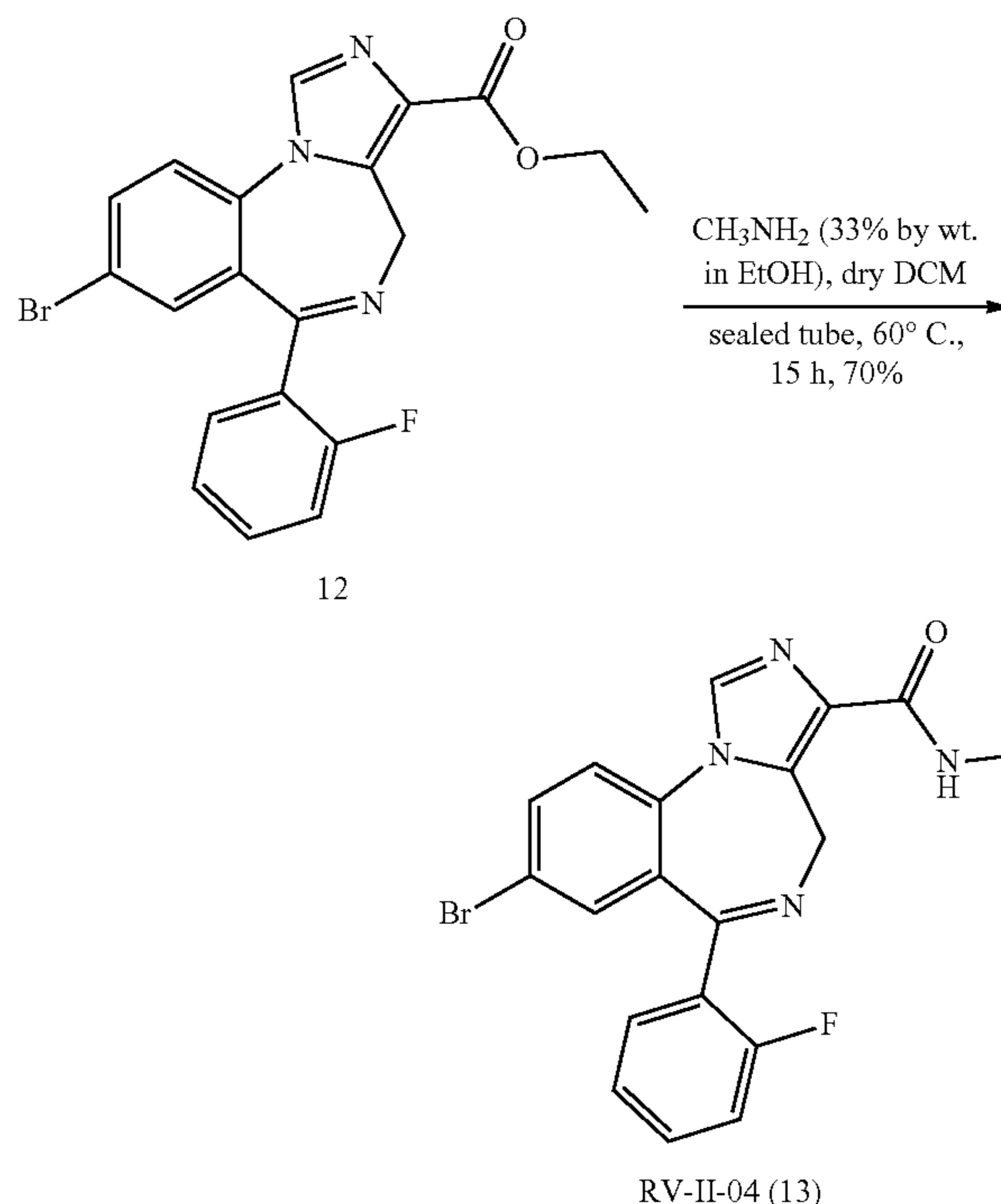
Scheme 5. Synthesis of RV-II-04.
