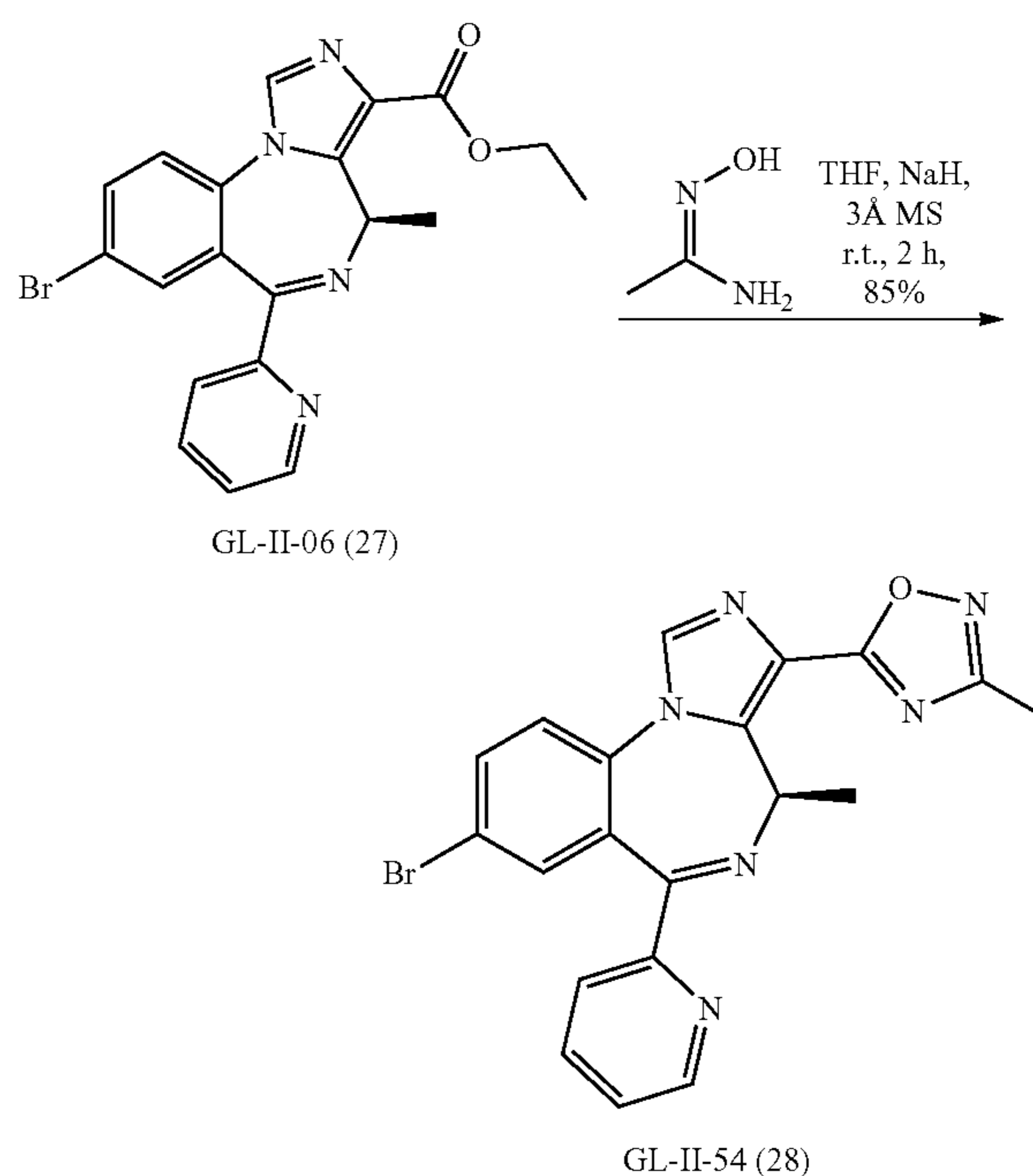
Scheme 11. Synthesis of GL-II-54.
