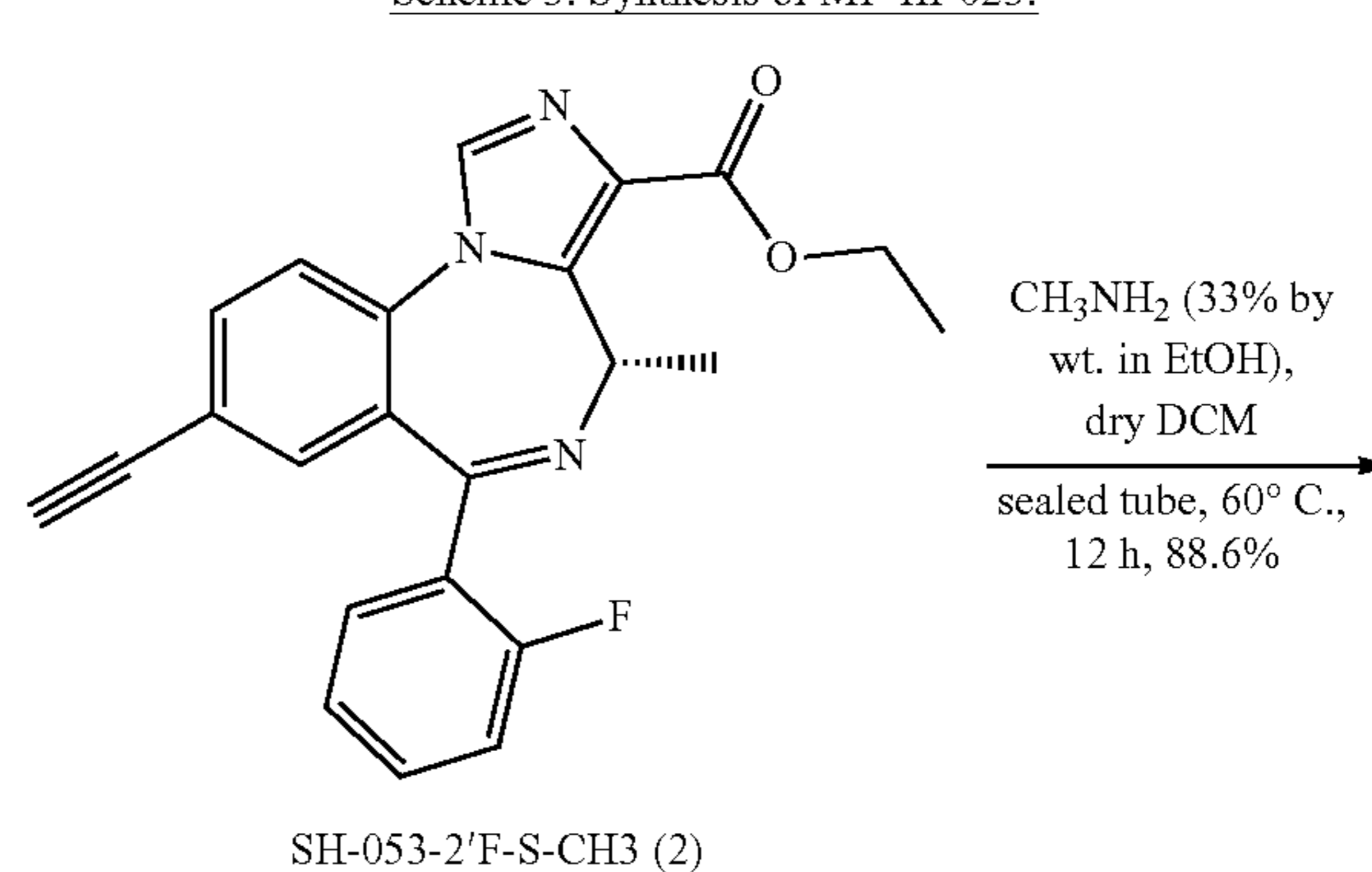
Scheme 3. Synthesis of MP-III-023.
