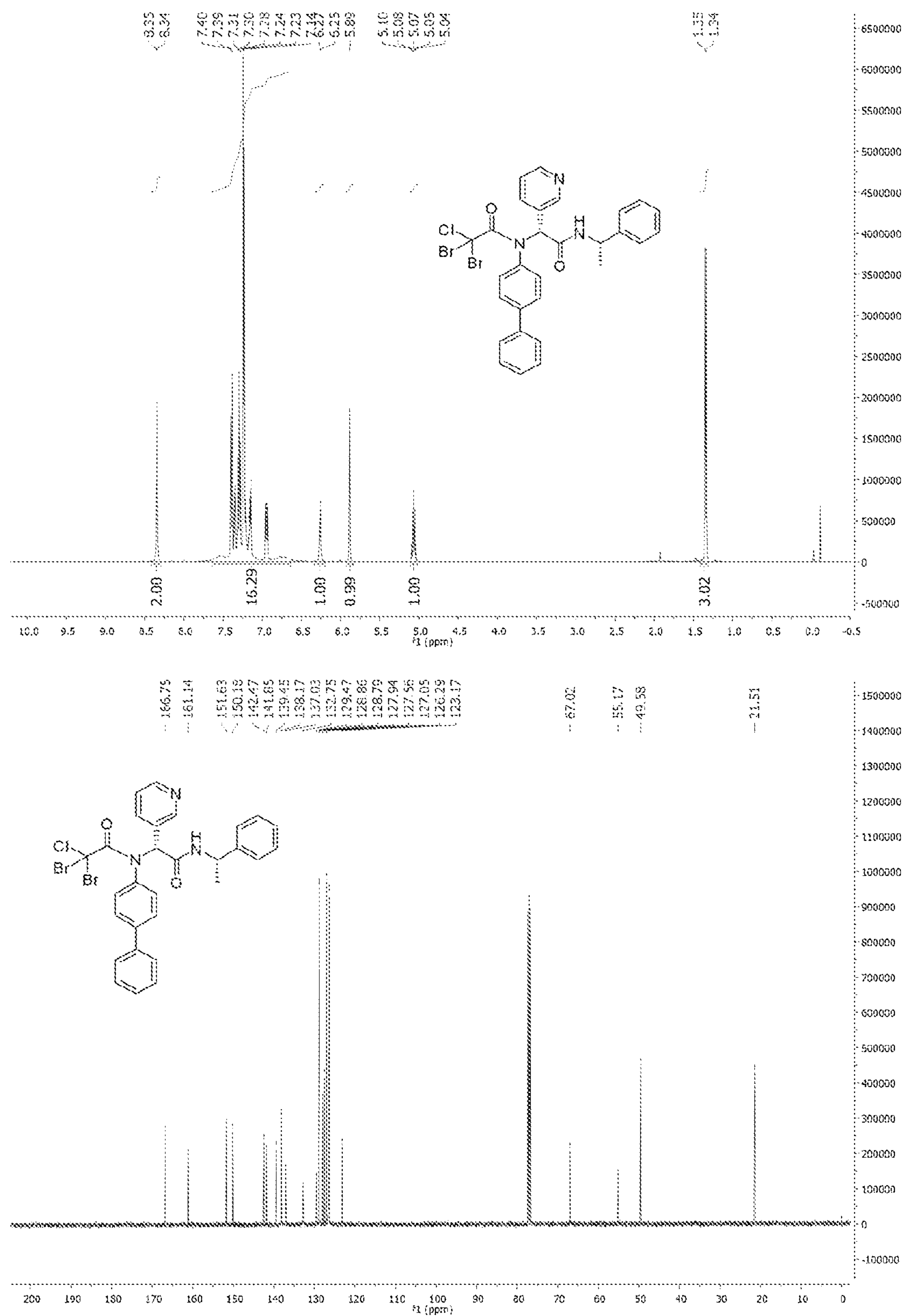
HNMR and CNMR spectra of Jun9-89-4S
