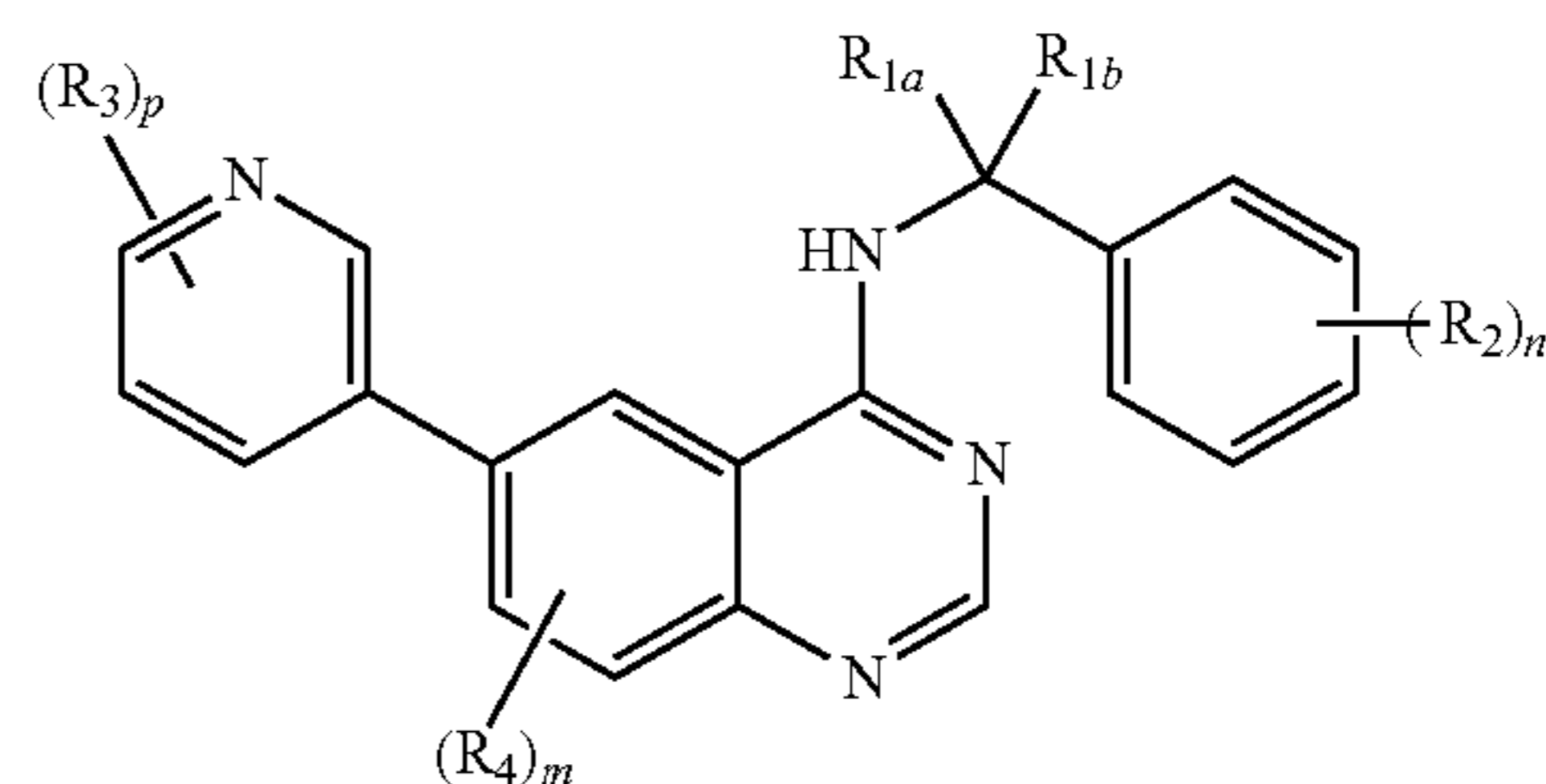
Formula Ia-2
