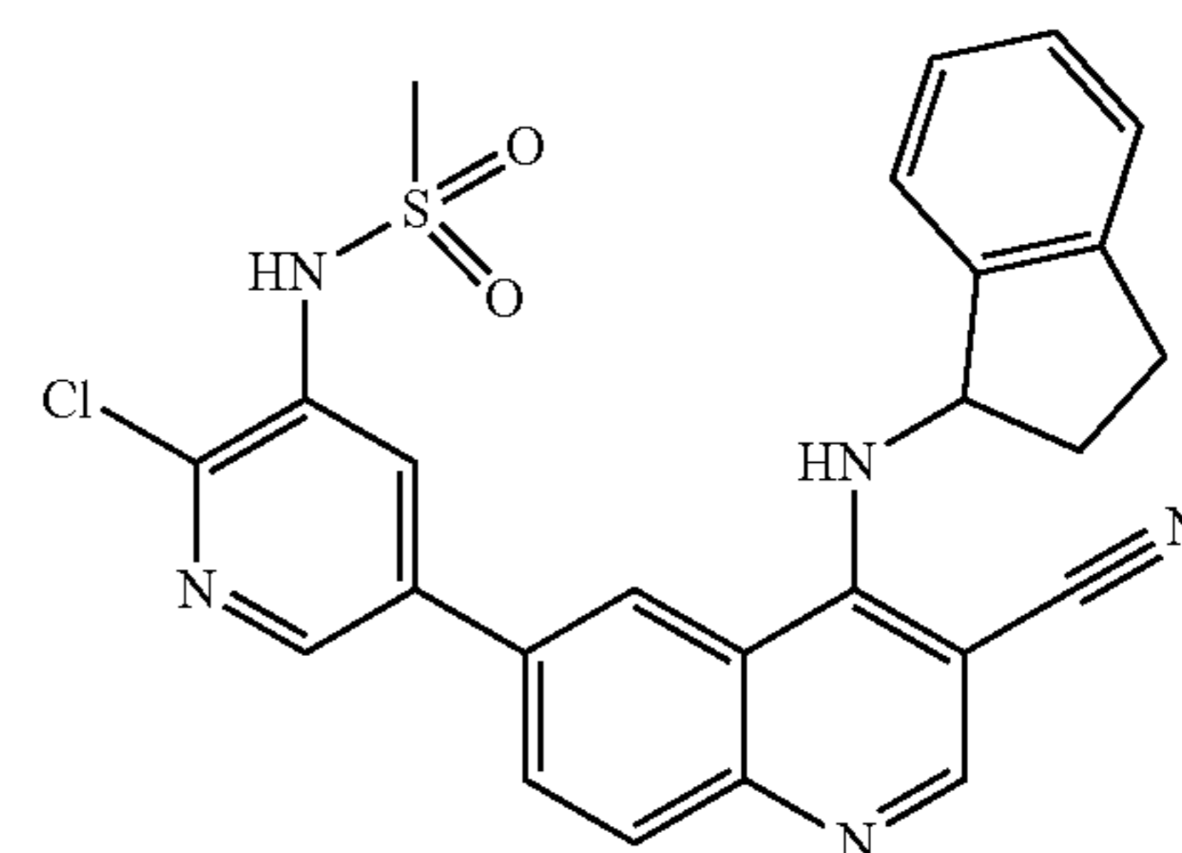
Compound 101
