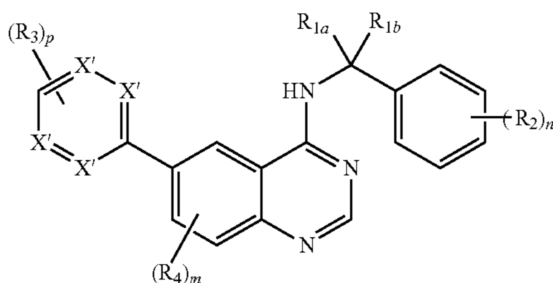
Formula Ia-1
