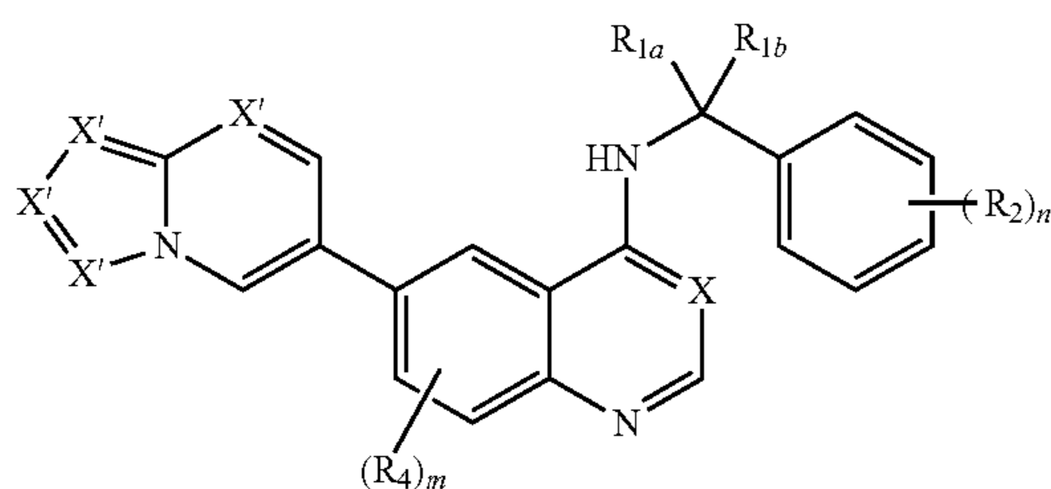
Formula Ic-2
