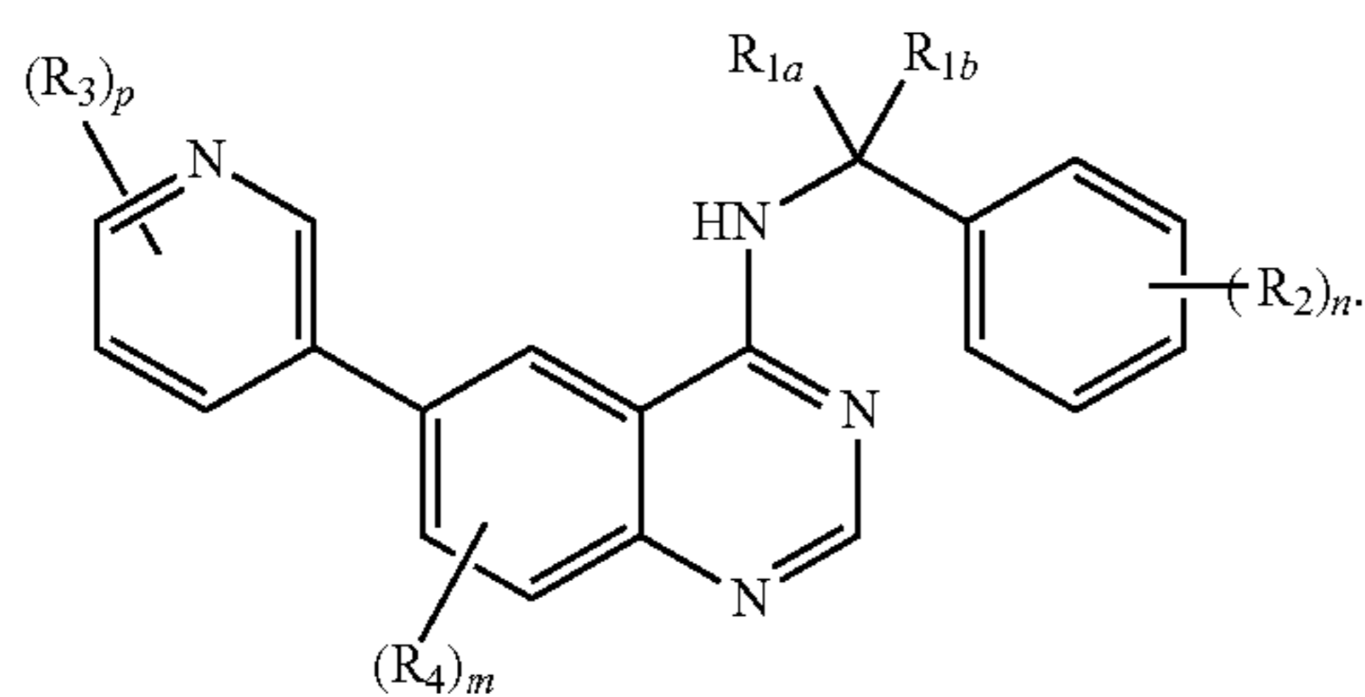
Formula Ia-2
