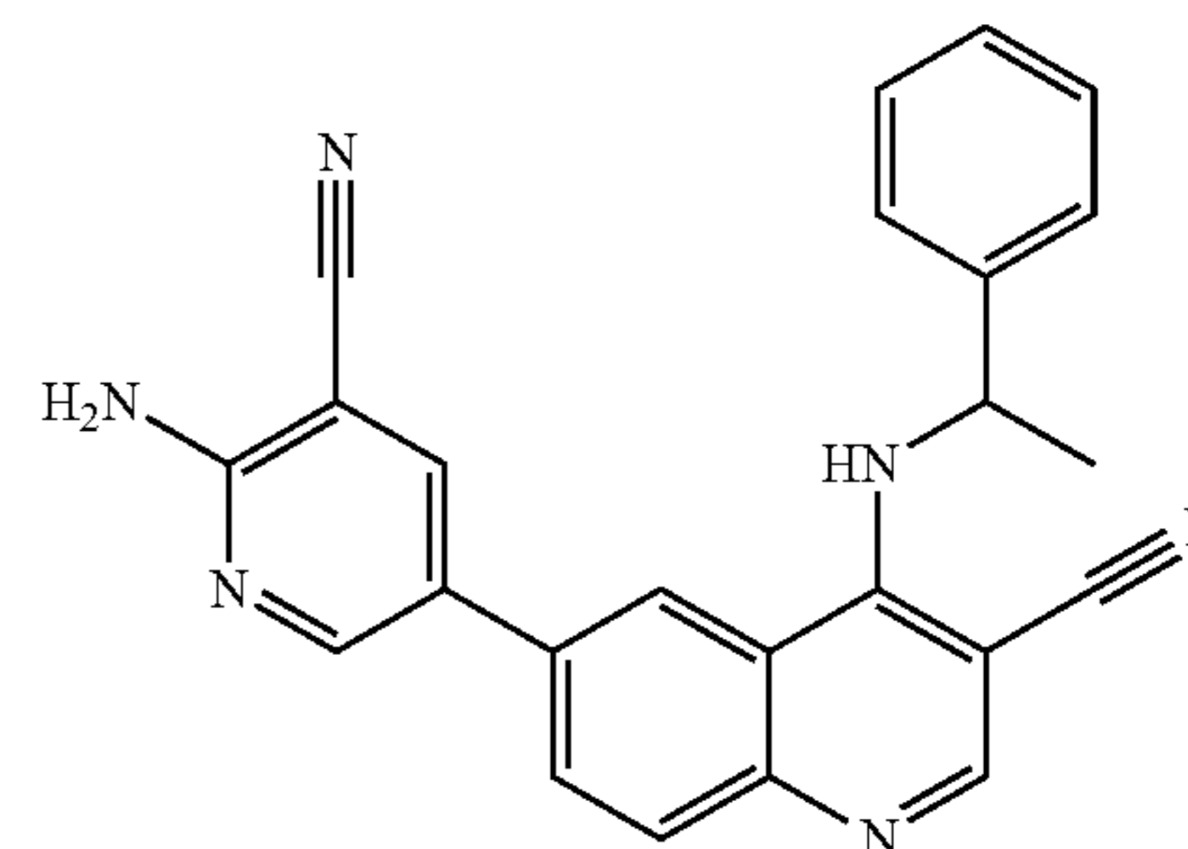
Compound 65
