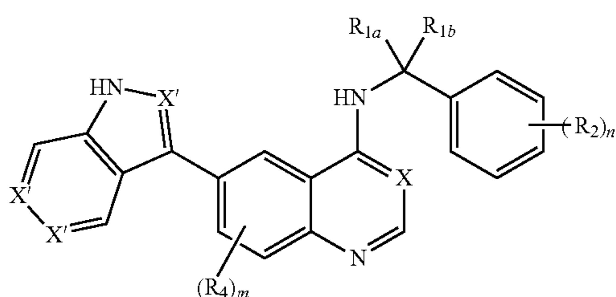
Formula Ic-2
