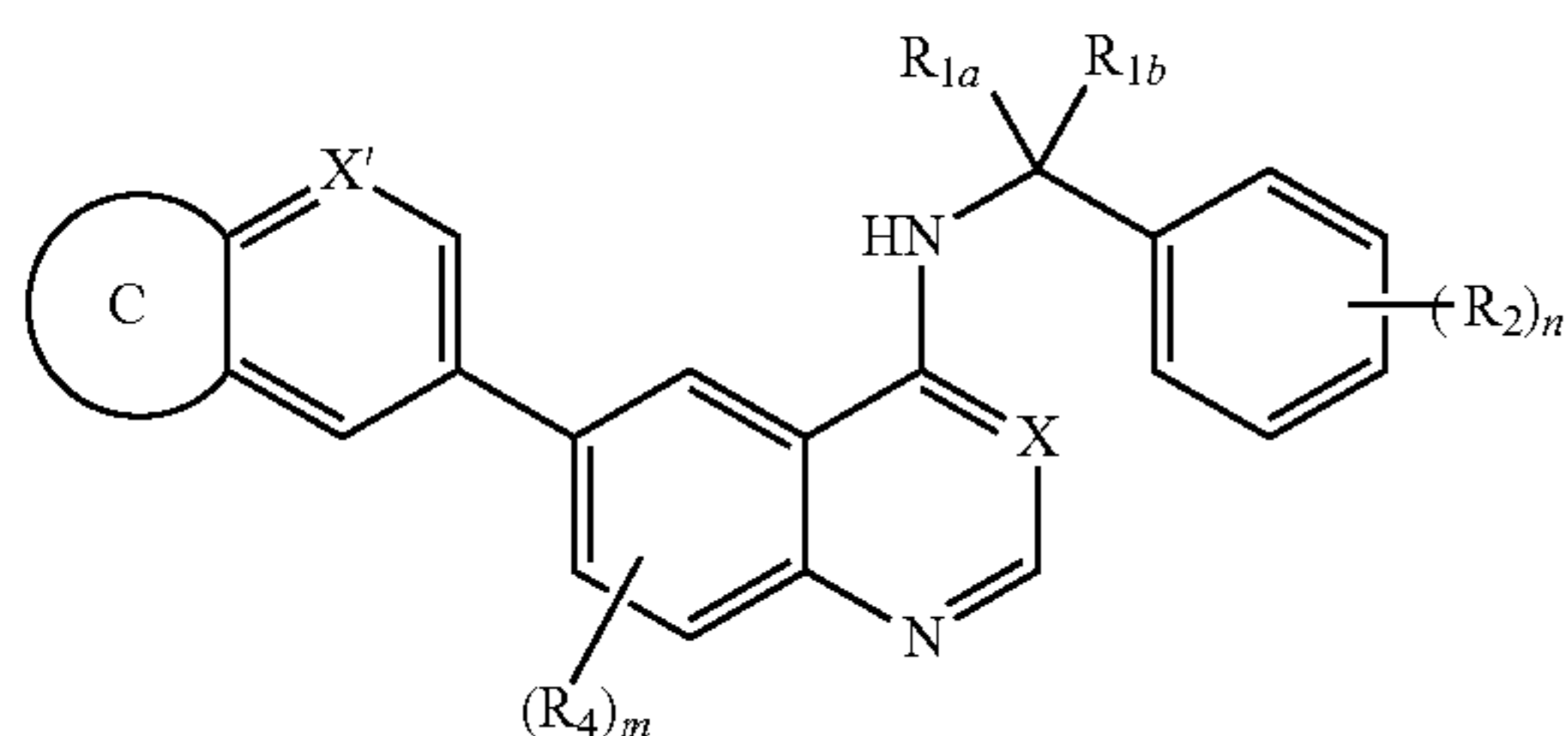
Formula Ib
