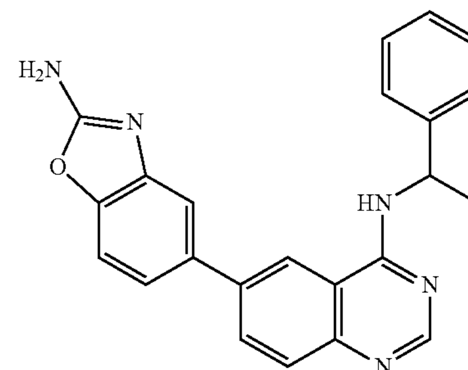
Compound 41
