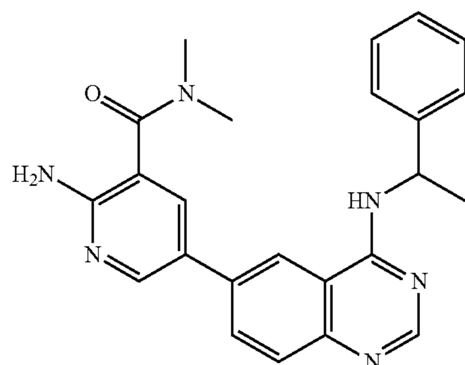
Compound 36
