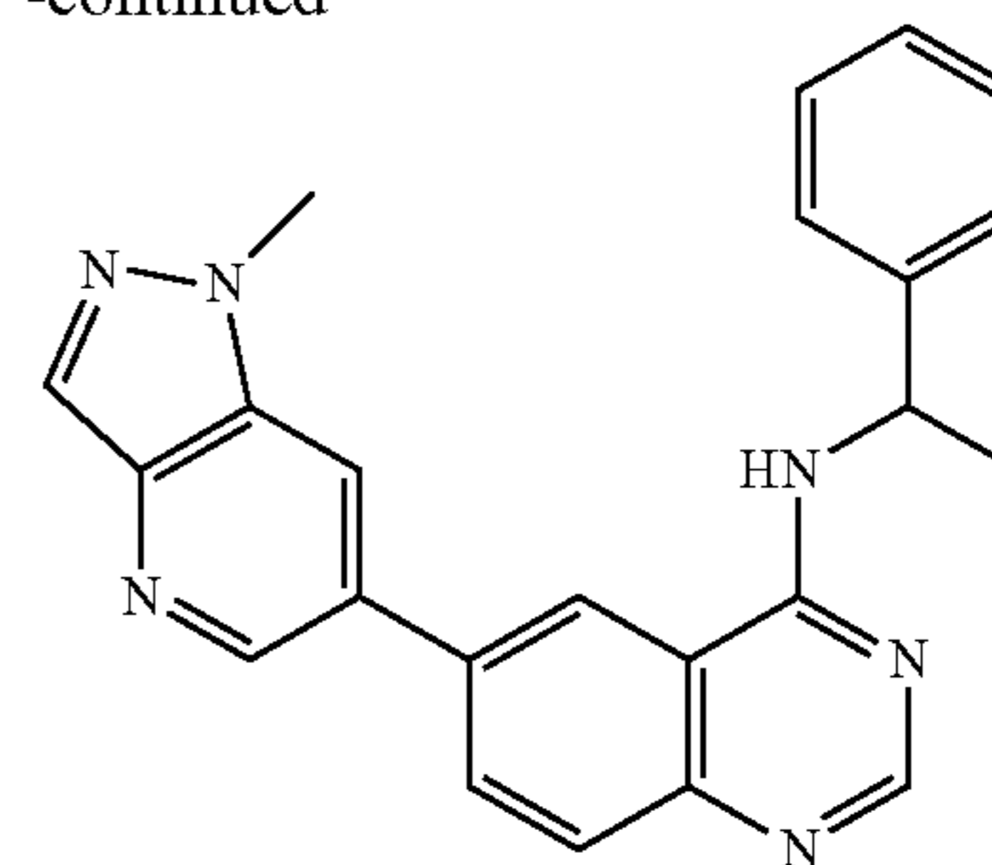
Compound 27
