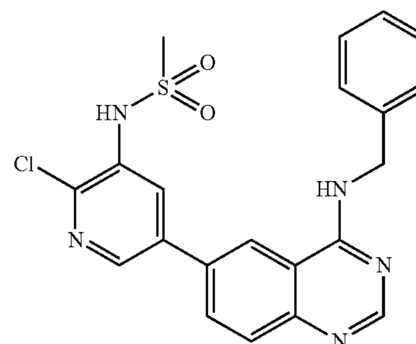
Comparative Compound 3
