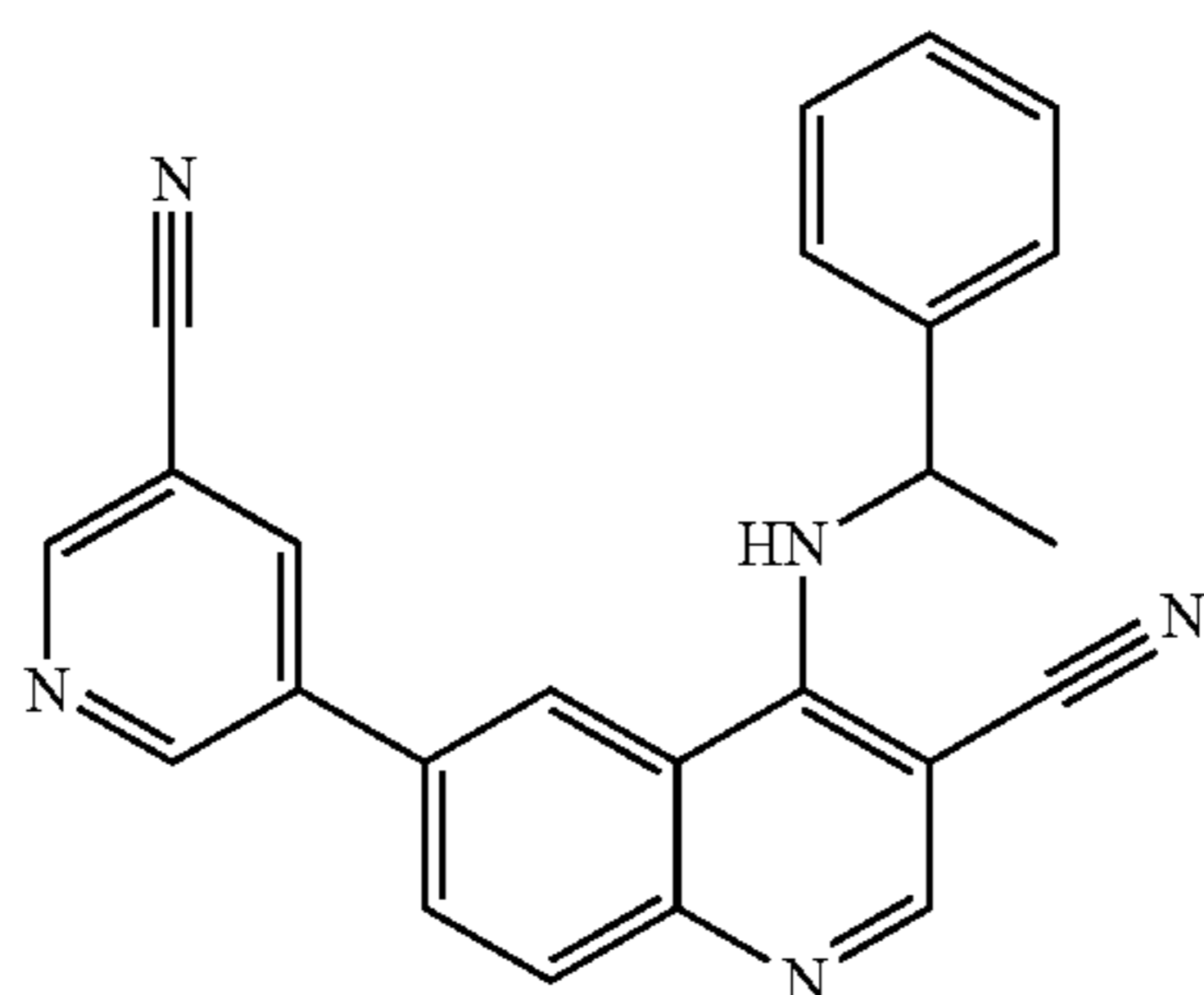
Compound 64
