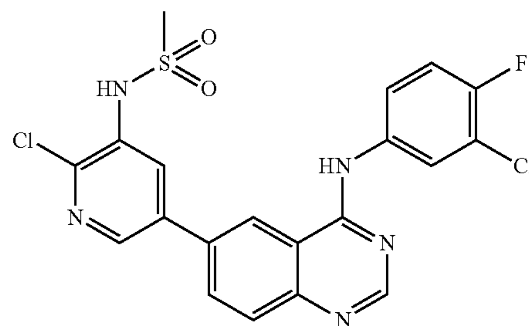
Comparative Compound 2
