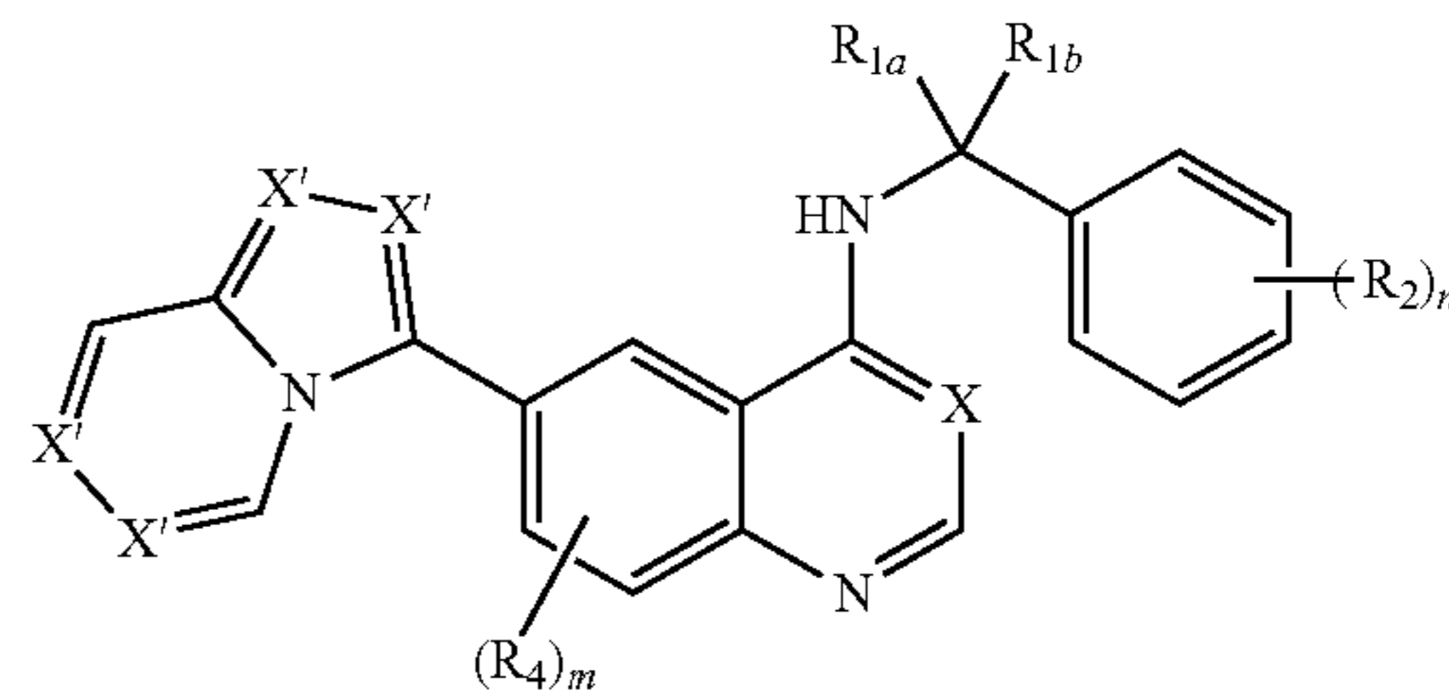
Formula Ic-3
