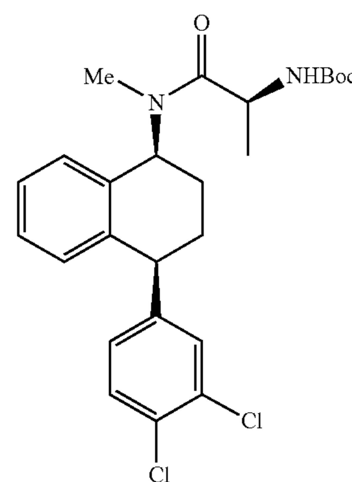
MP_080 diastereoselectivity: 3:1
