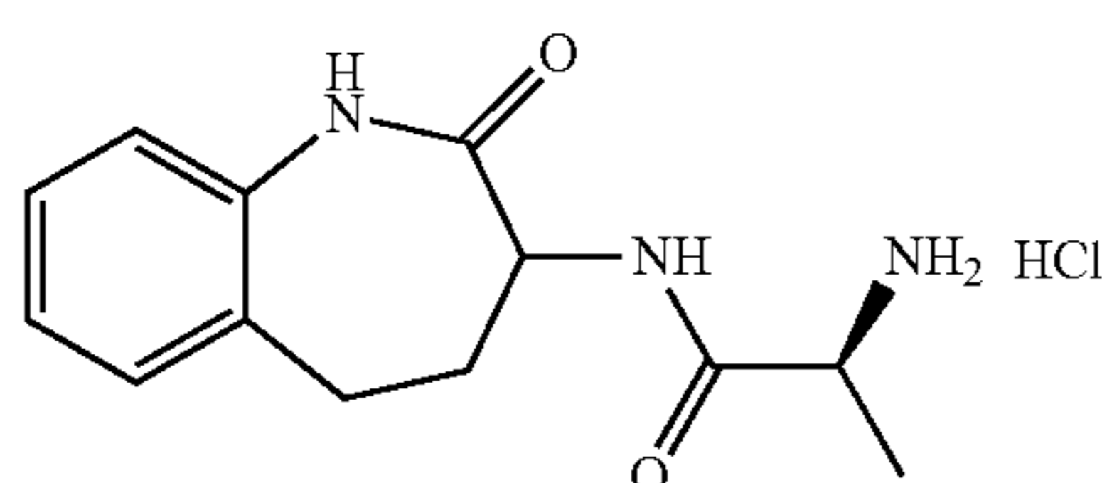
MP_084 diastereoselectivity = 1:1
