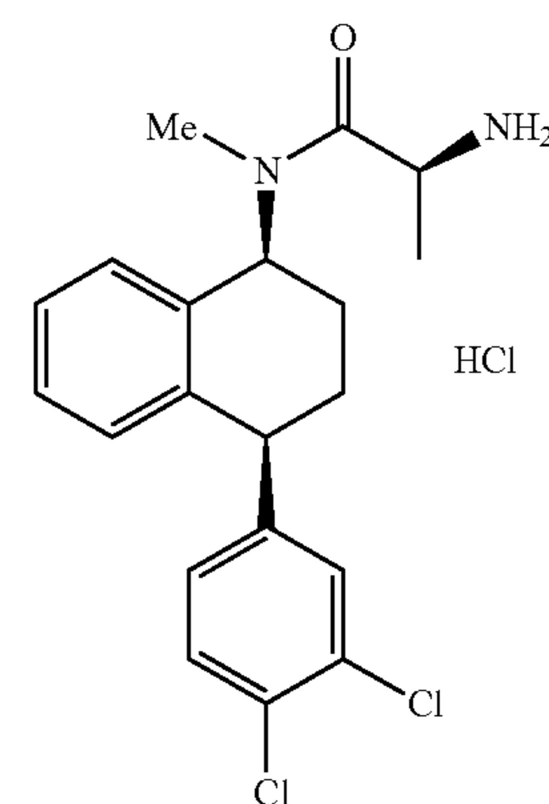
MP-81 diastereoselectivity: 3:2
