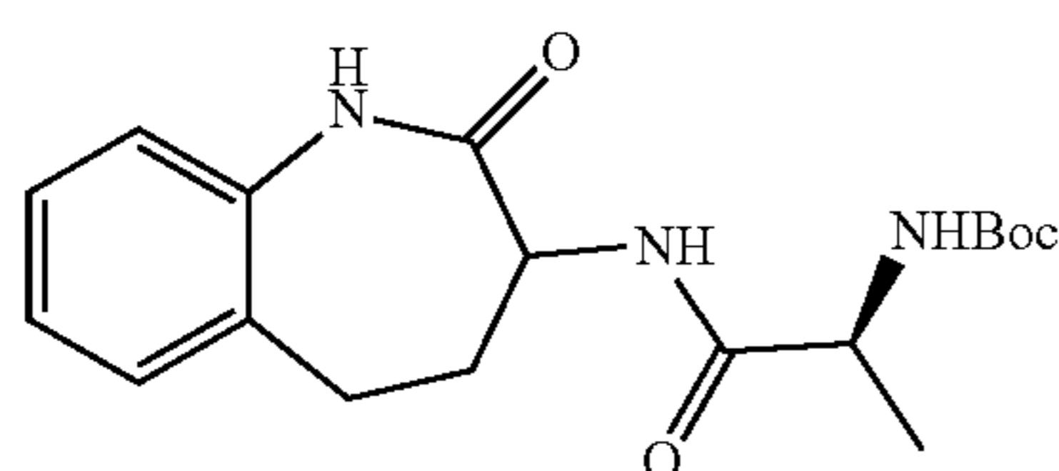
diastereoselectivity = 2:1
