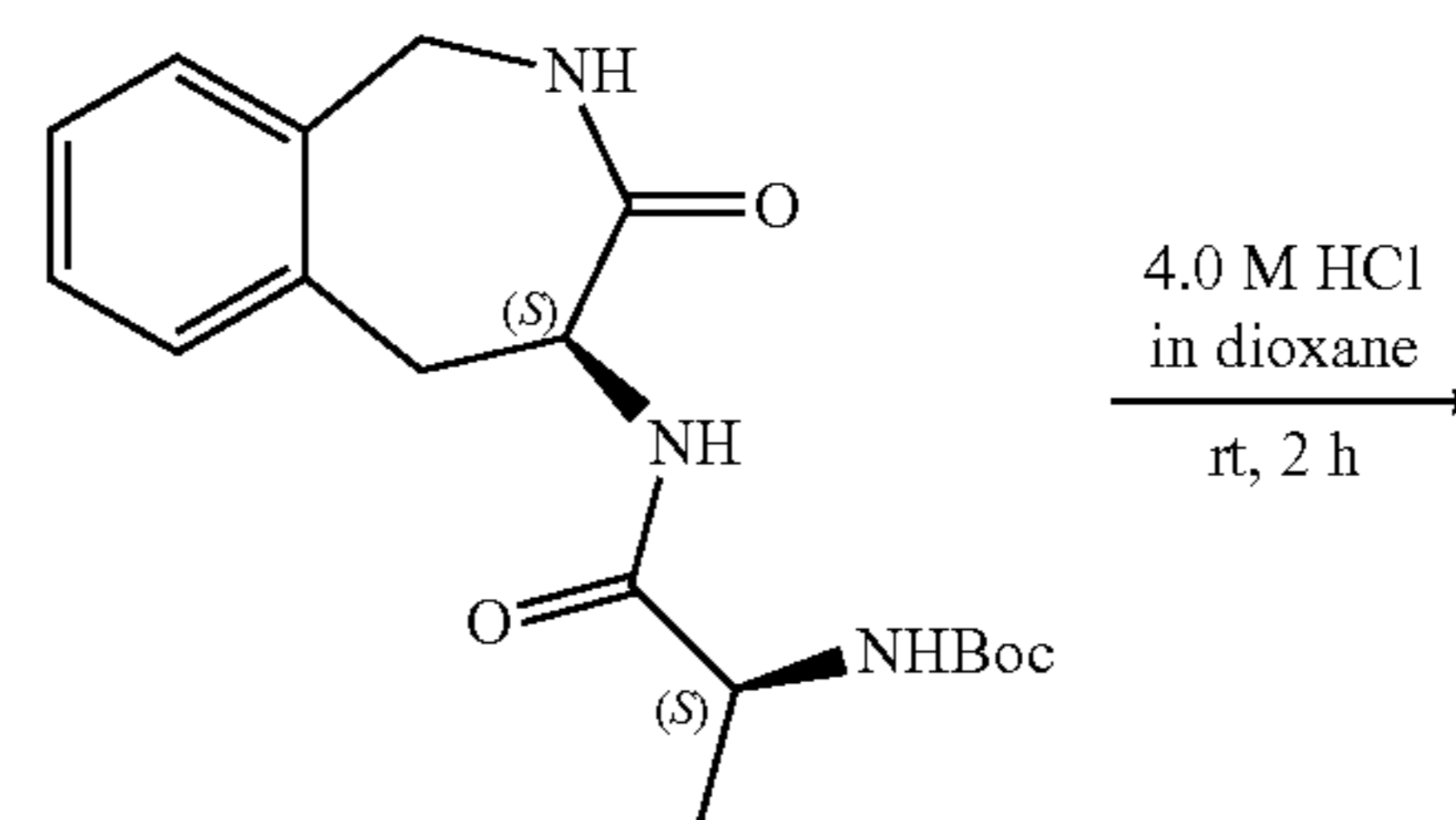
MP-105a
