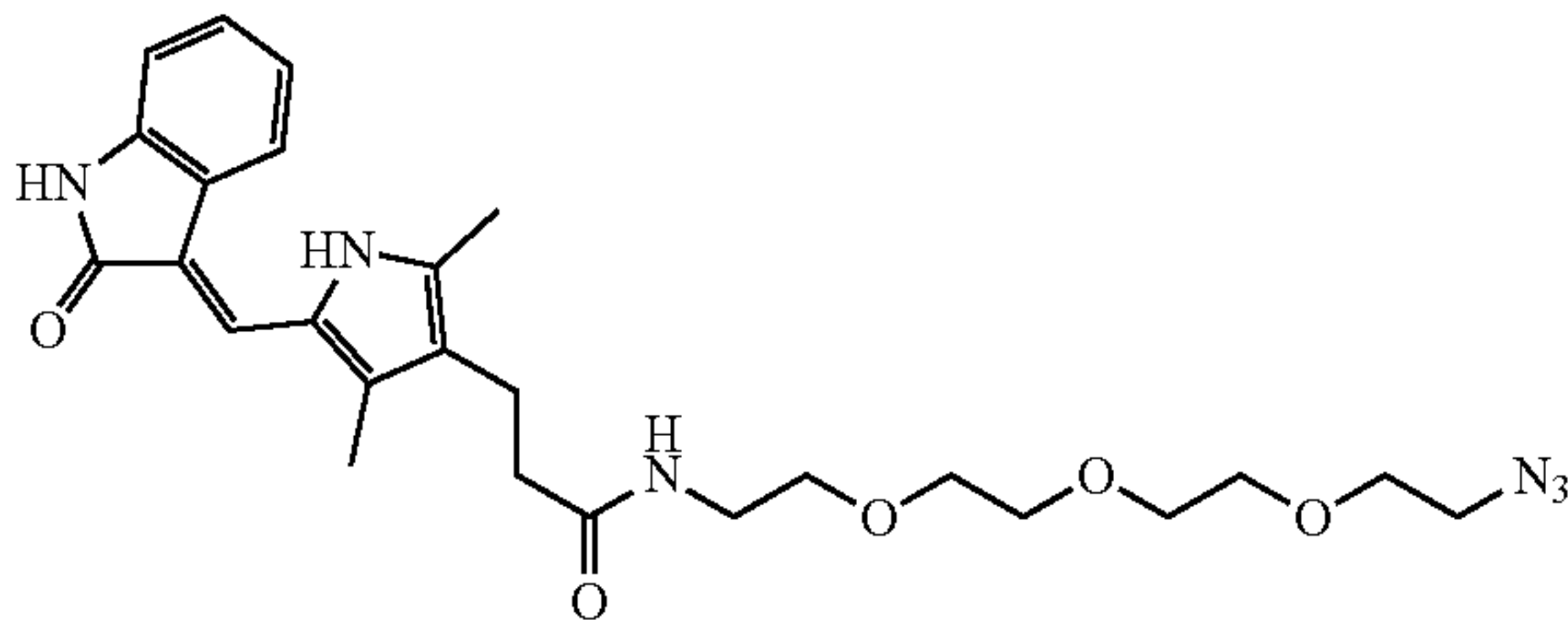
Structure IV: Chemical Structure of Orantinib Analogue [0102]
