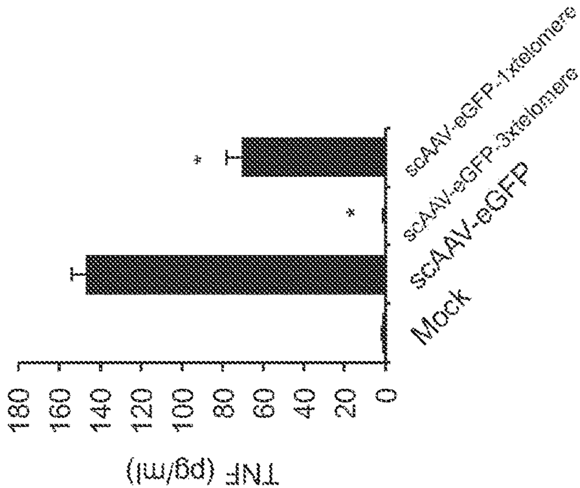
Fig. 10C Primary macrophages
