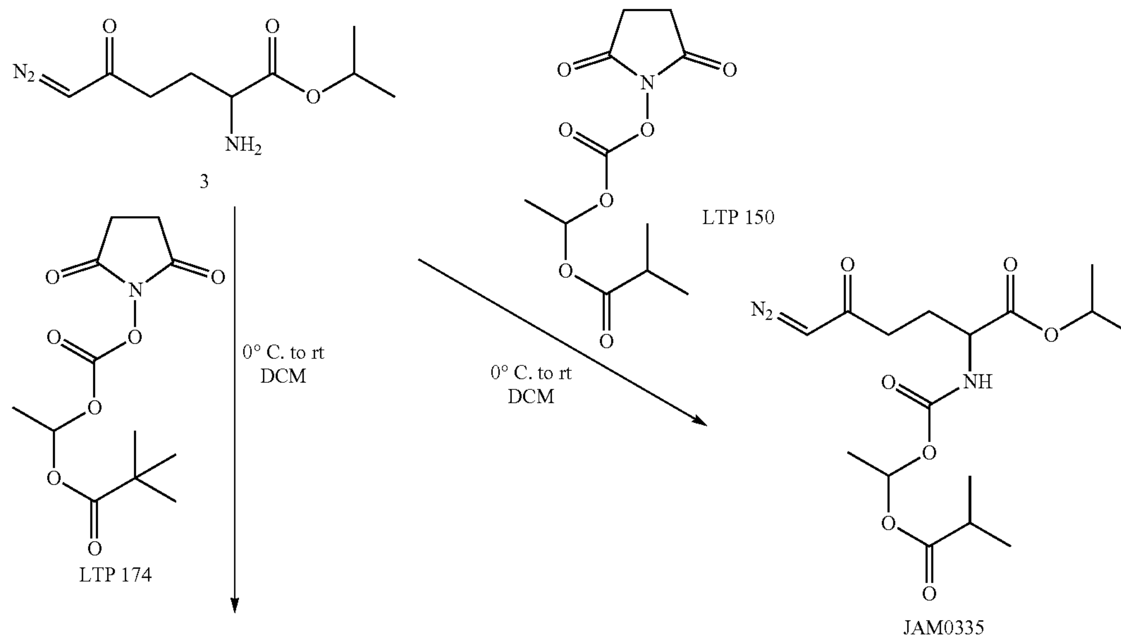
Scheme 2
