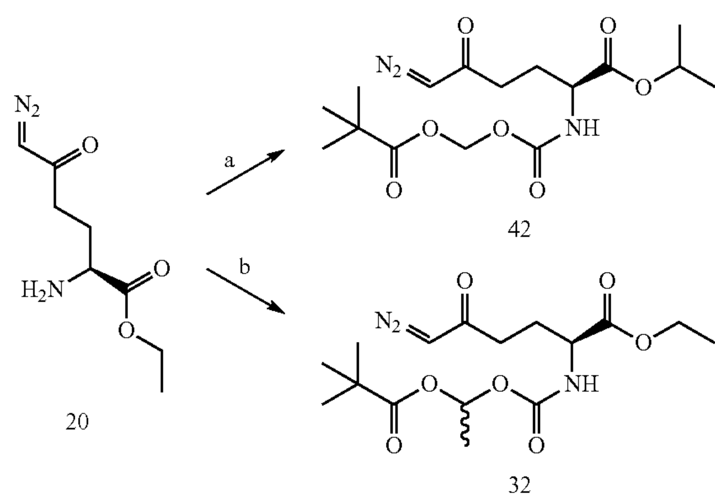
Scheme 4
