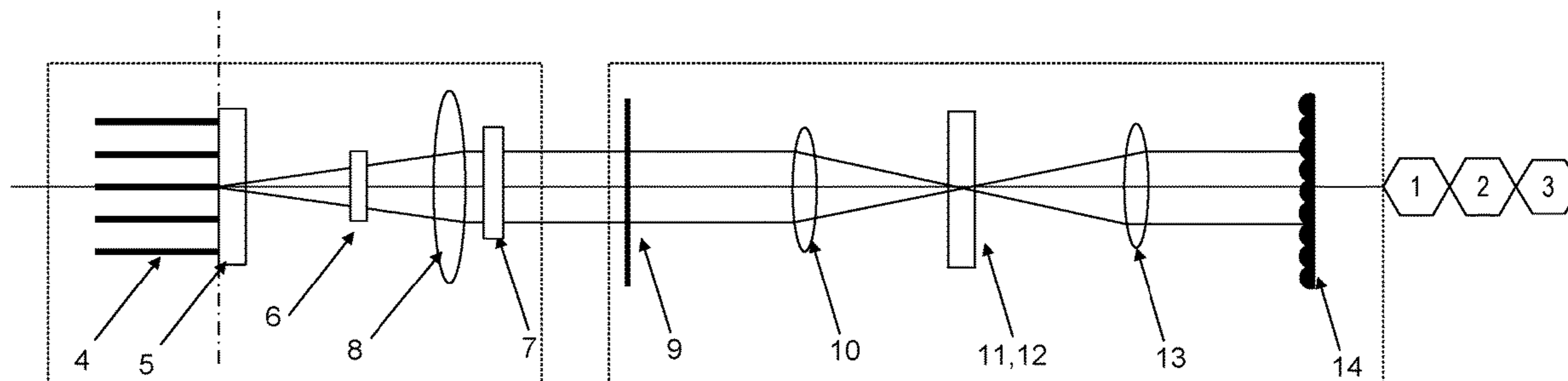
Wavelength-Selective Switch
