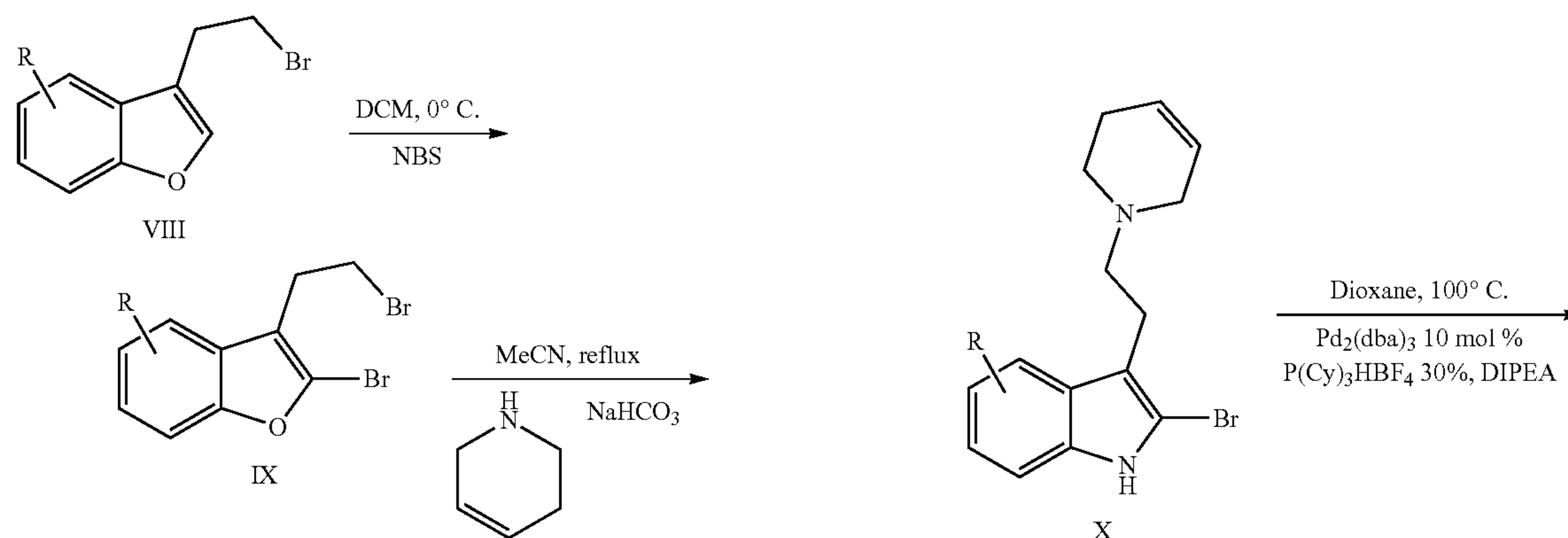
Scheme 15. Synthesis of benzofuran-bicyclic derivatives.
