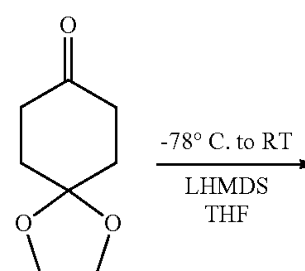
Scheme 6. Synthesis of 2-propyl-1-(2,2,2-trifluoroacetyl)azepan-4-one
