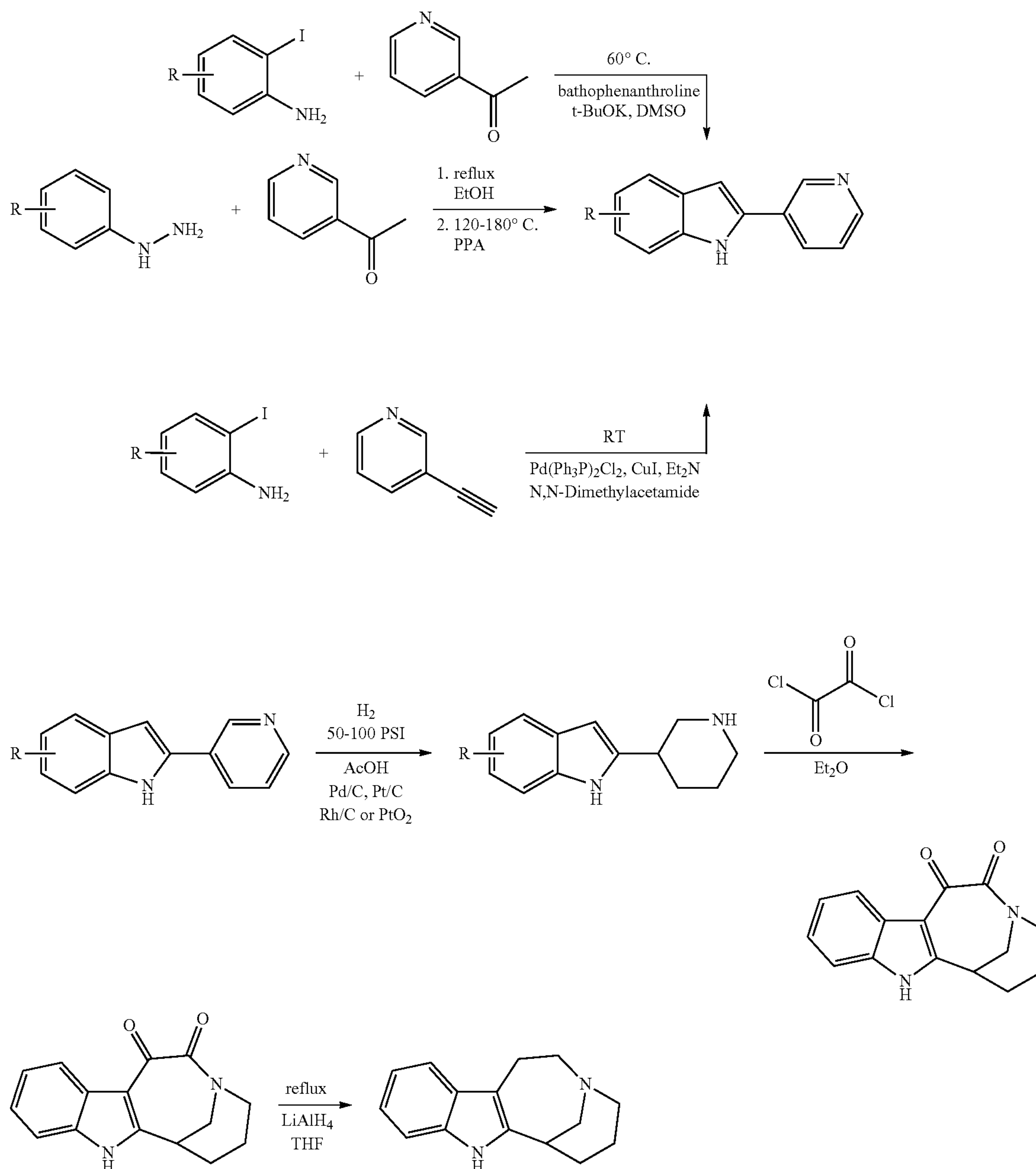
Scheme 12. Alternative route for preparation of indole-bicyclic azepines.
