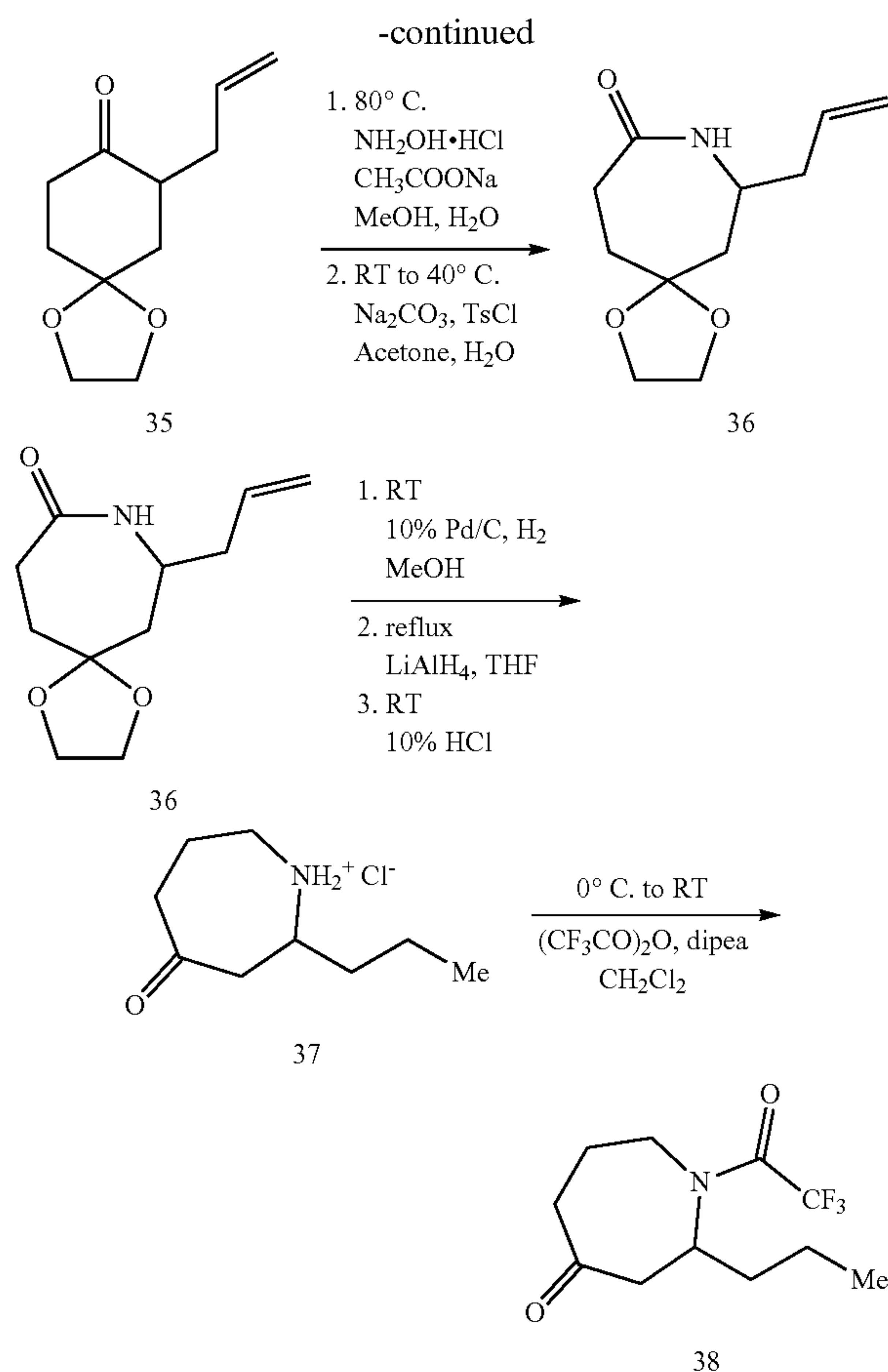
Example 27. 7-allyl-1,4-dioxaspiro[4.5]decan-8-one 35
