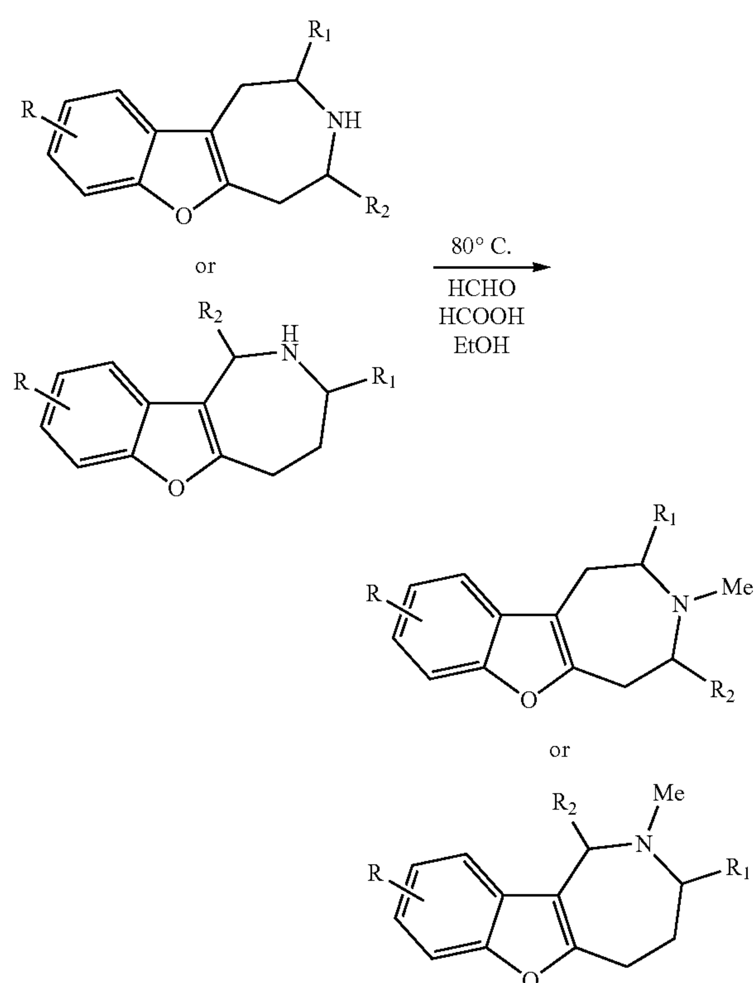
Scheme 4. General procedure D for the N-methylation of the azepino-benzofuran derivatives.
