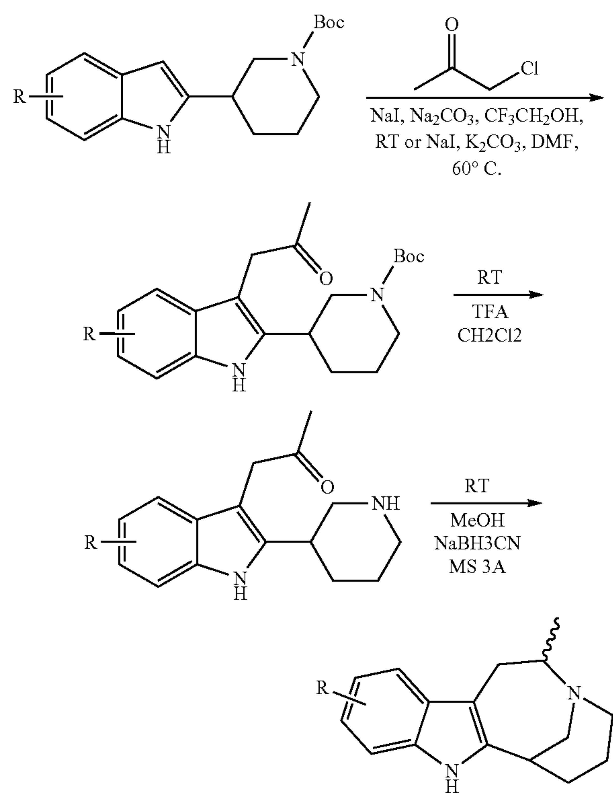
Scheme 13. Alternative route for preparation of \alpha -methyl indole-bicyclic azepines.
