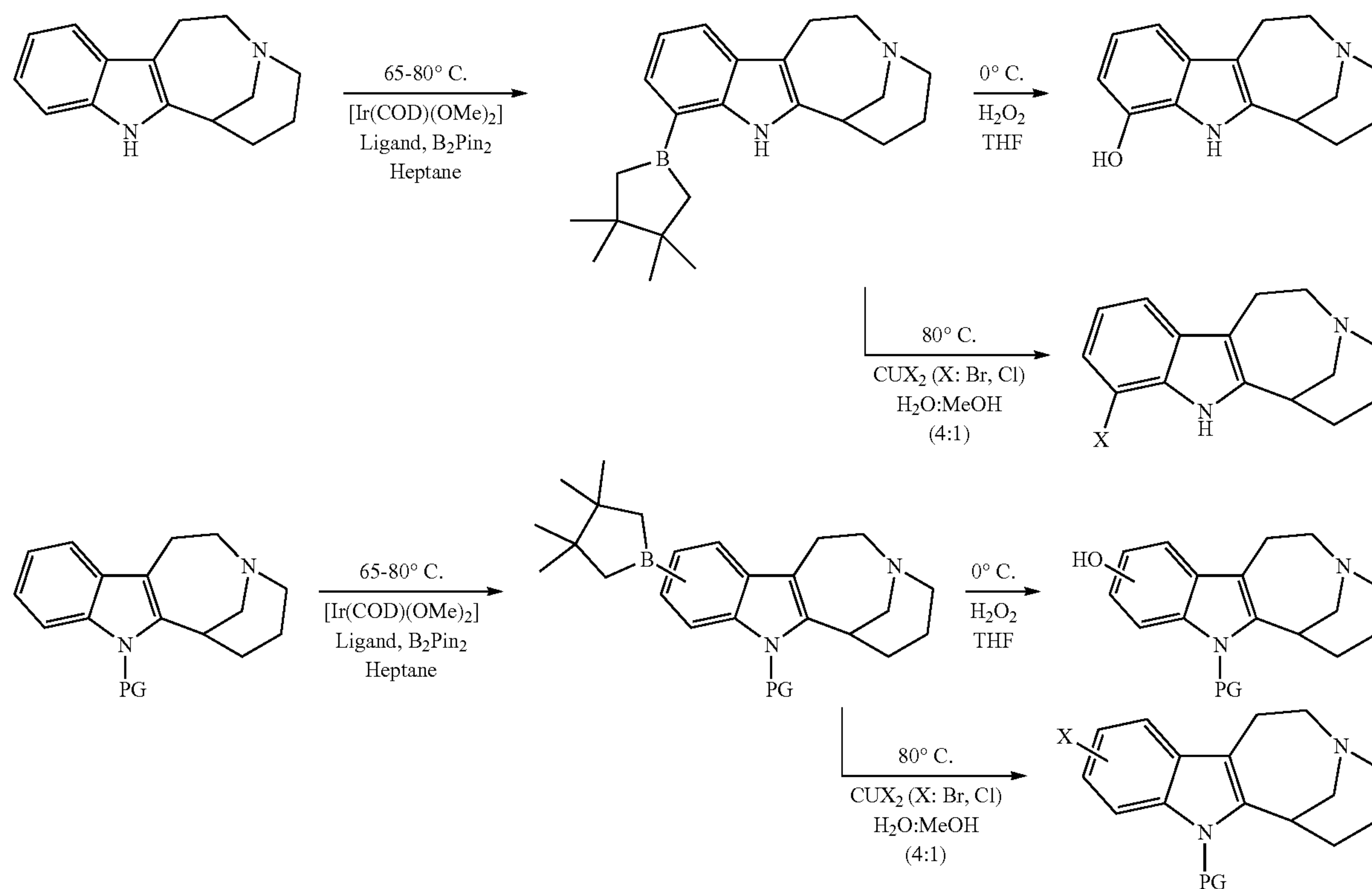
Scheme 14. Late-stage functionalization of indole-bicyclic azepines.
