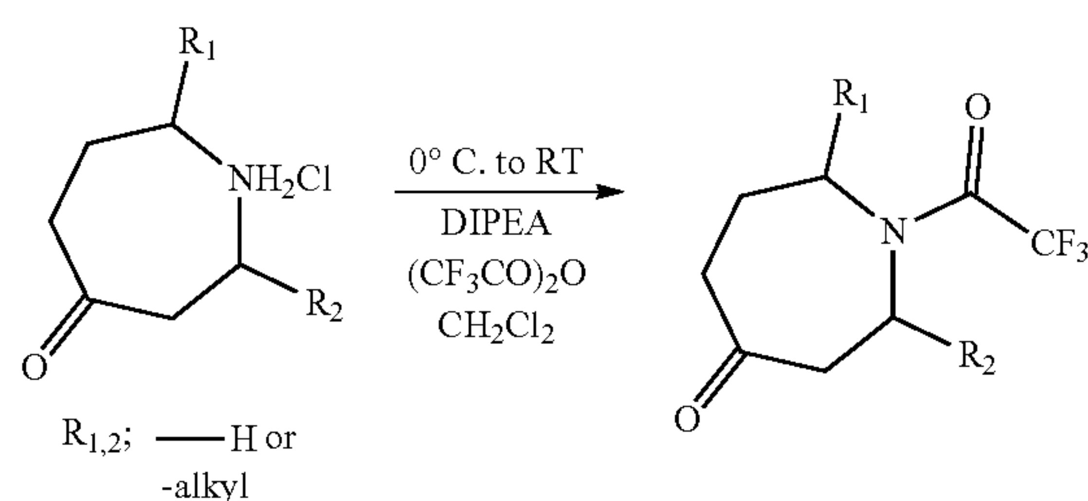
Scheme 1. General procedure A for the synthesis of N-(Trifluoroacetyl) azepan-4-one derivatives
