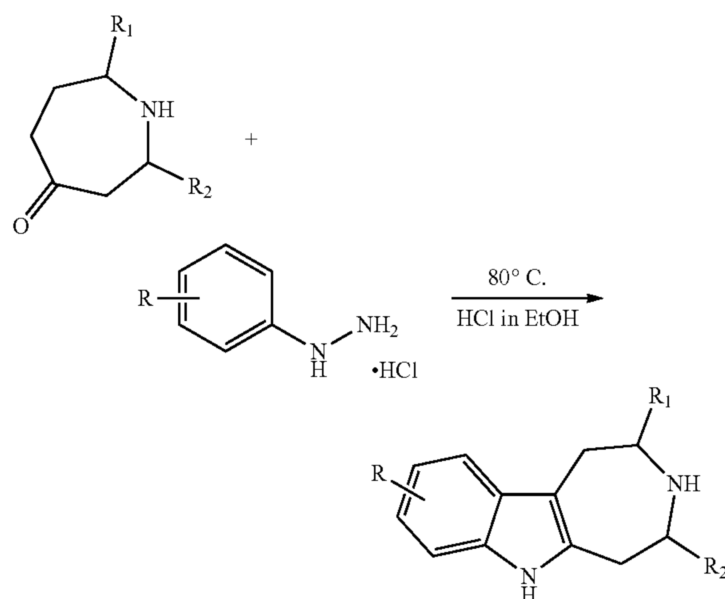
Scheme 5. General procedure E for the preparation of 1,2,3,4,5,6-hexahydroazepino[4,5-b]indole derivatives.
