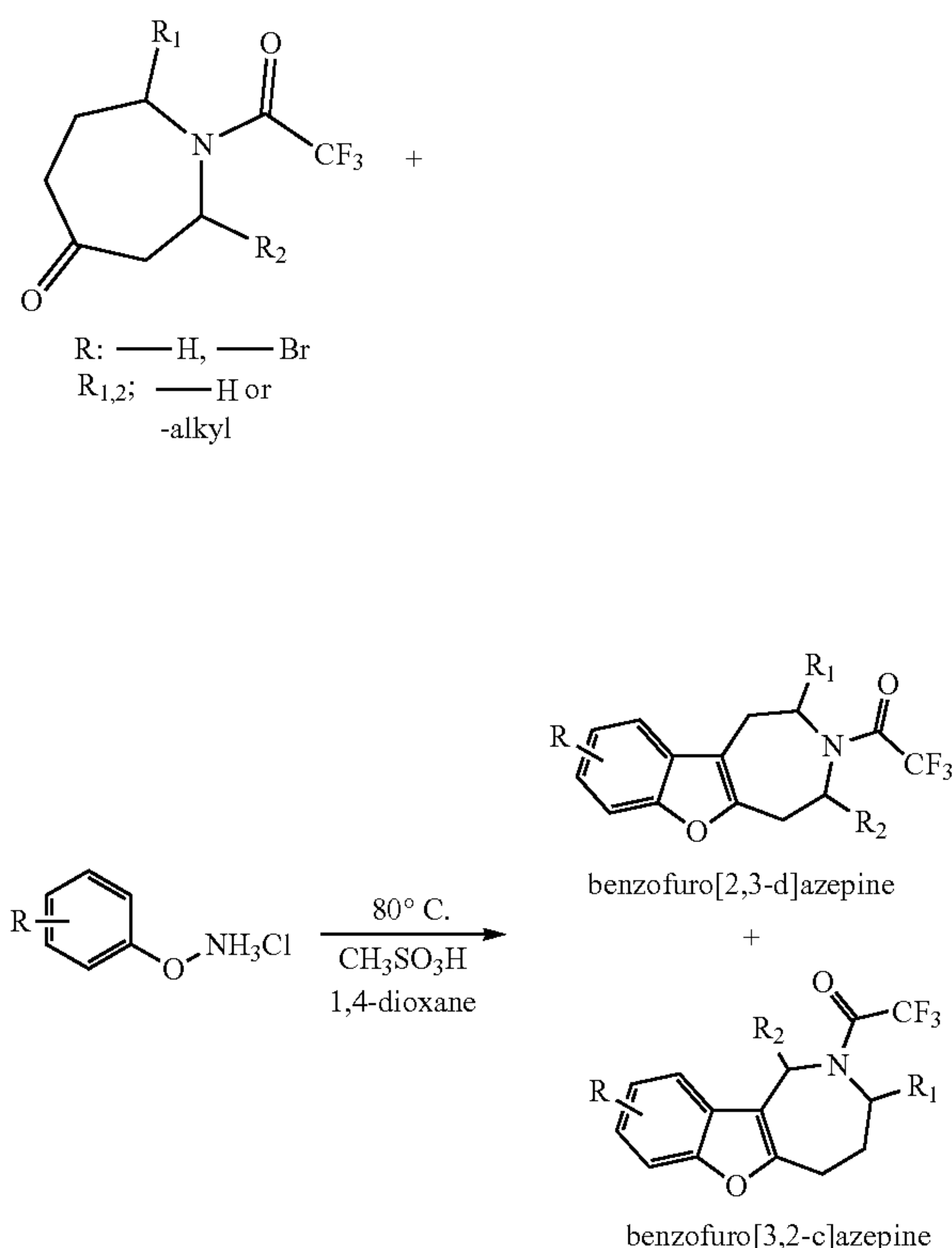
Scheme 2. General procedure B for the preparation of N-(trifluoroacetyl)-2,3,4,5-tetrahydro-1H-benzofuro[2,3-d]azepine and N-(trifluoroacetyl)-2,3,4,5-tetrahydro-1H-benzofuro[3,2-c]azepine derivatives.
