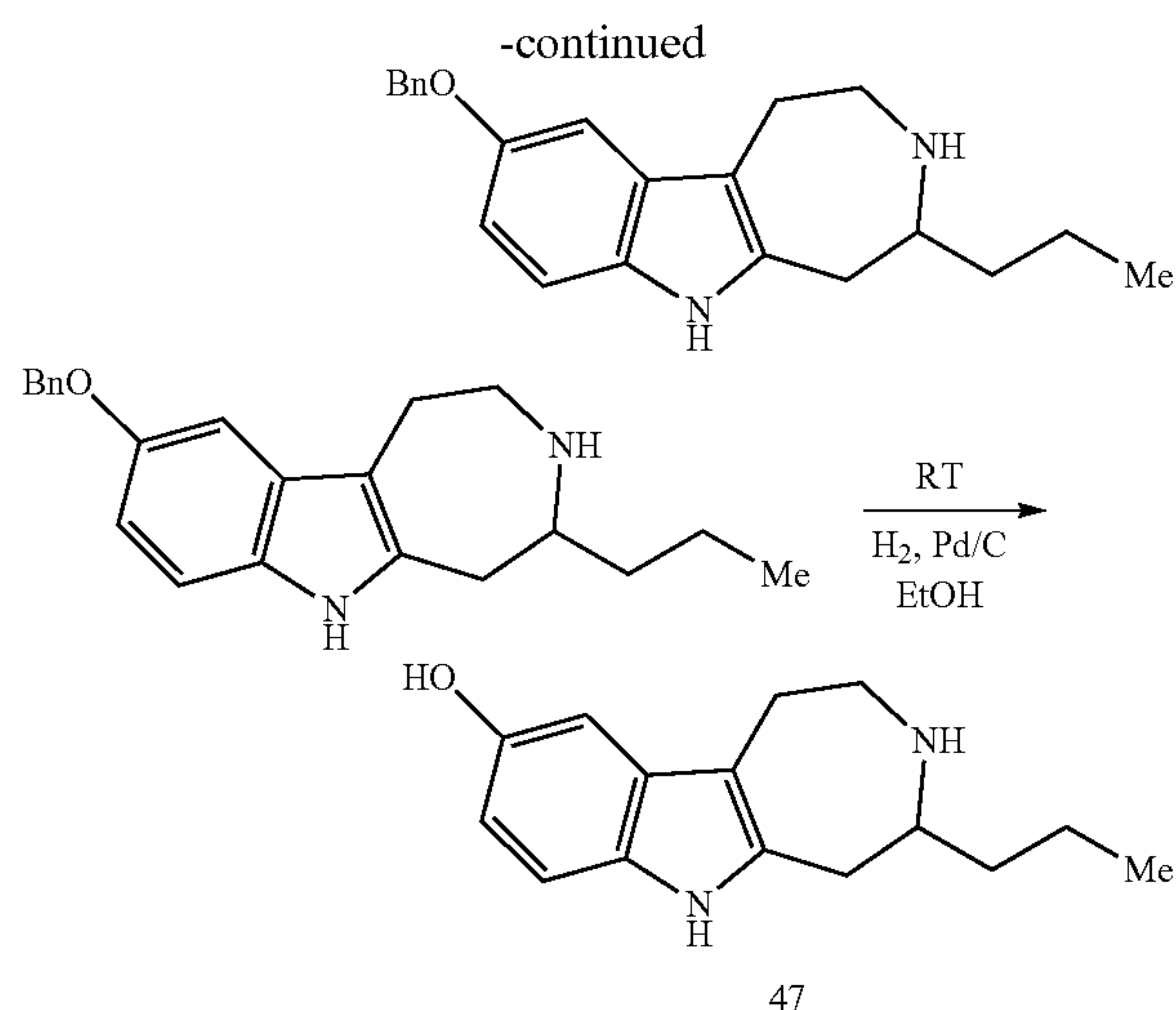
Example 37. 9-hydroxy-4-propyl-1,2,3,4,5,6-hexahydroazepino[4,5-b]indole 47
