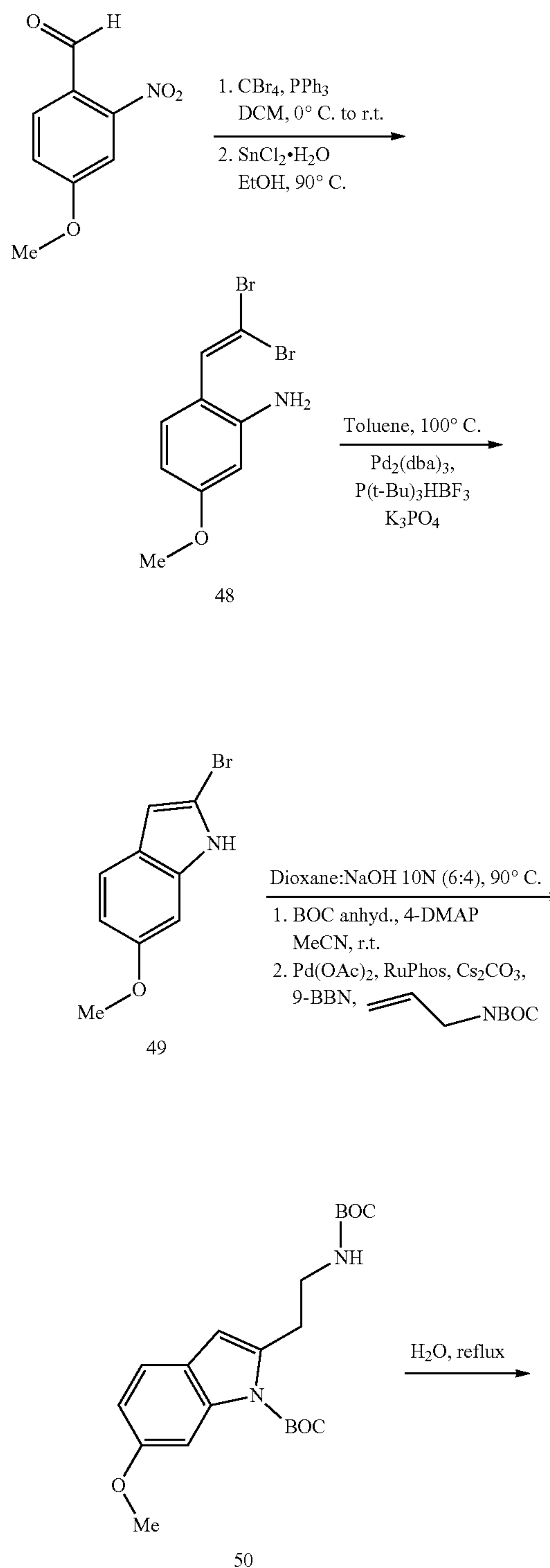
Scheme 9. Synthesis of derivatives 48-55.
