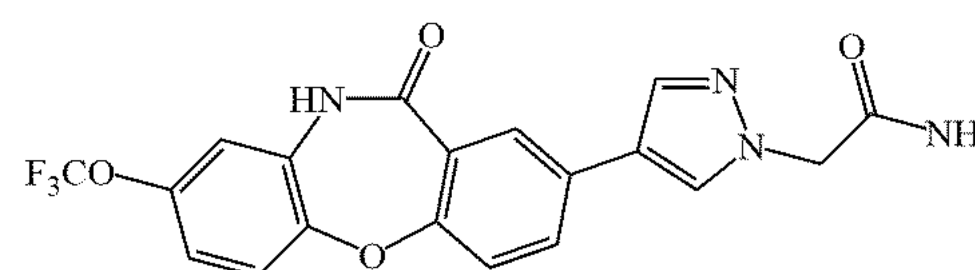
Chemical Formula: \text{C}_{19}\text{H}_{13}\text{F}_3\text{N}_4\text{O}_4 Exact Mass: 418.09 Molecular Weight: 418.33
