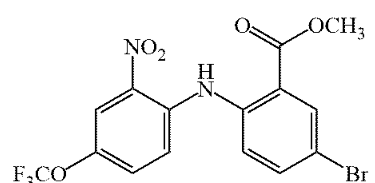
Chemical Formula: \text{C}_{15}\text{H}_{10}\text{BrF}_3\text{N}_2\text{O}_5 Exact Mass: 433.97 Molecular Weight: 435.15
