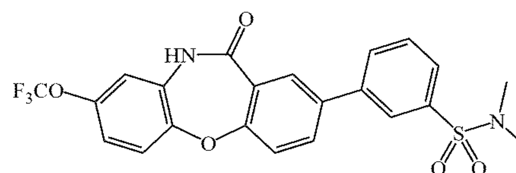
Chemical Formula: C 22 H 17 F 3 N 2 O 5 S Exact Mass: 478.08 Molecular Weight: 478.44
