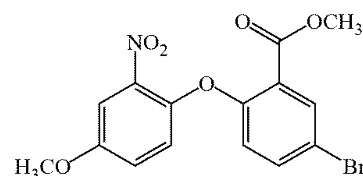
Chemical Formula: C 15 H 12 BrNO 3 Exact Mass: 380.98 Molecular Weight: 382.17
