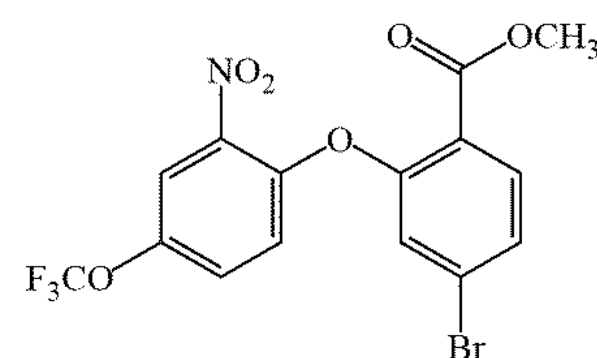
Chemical Formula: \text{C}_{15}\text{H}_9\text{BrF}_3\text{NO}_6 Exact Mass: 434.96 Molecular Weight: 436.14
