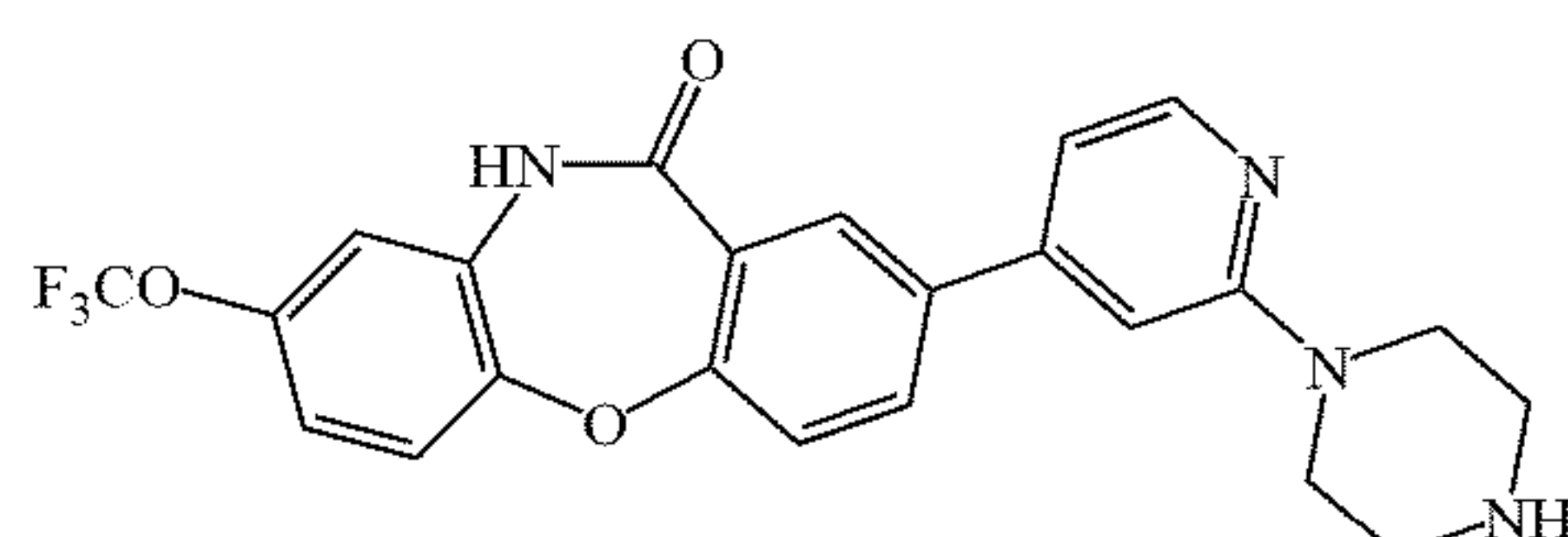
Chemical Formula: C 23 H 19 F 3 N 4 O 3 Exact Mass: 456.14 Molecular Weight: 456.43
