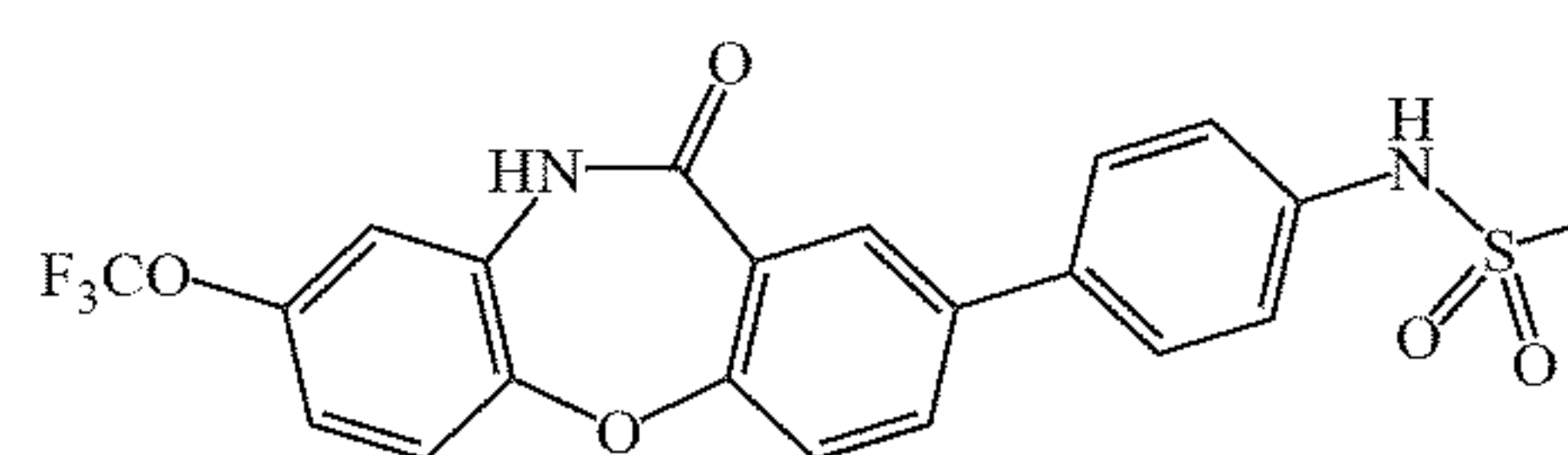
Chemical Formula: C_{21}H_{15}F_3N_2O_5S Exact Mass: 464.07 Molecular Weight: 464.42
