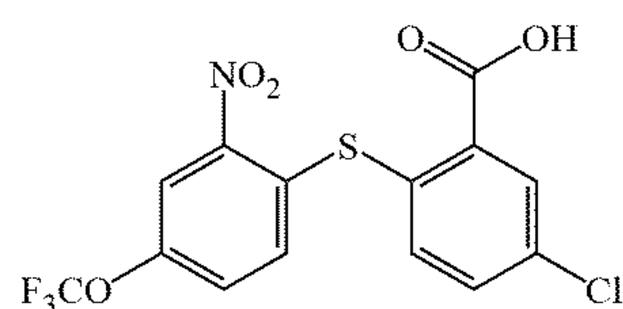
Chemical Formula: C_{14}H_7ClF_3NO_5S Exact Mass: 392.97 Molecular Weight: 393.72
