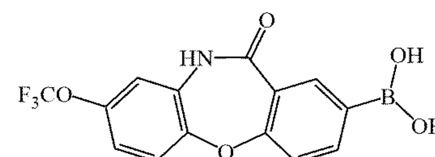
Chemical Formula: C 14 H 9 BF 3 NO 5 Exact Mass: 339.05 Molecular Weight: 339.03
