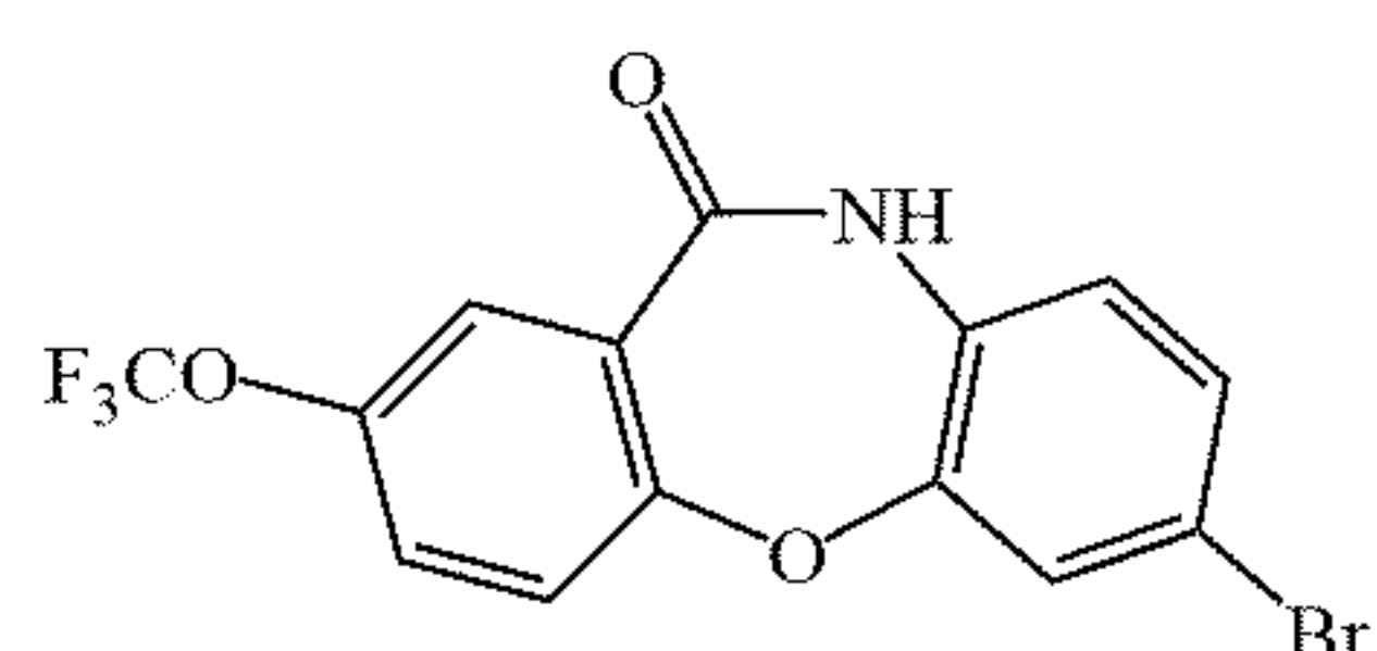
Chemical Formula: C 14 H 7 BrF 3 NO 3 Exact Mass: 372.96 Molecular Weight: 374.11
