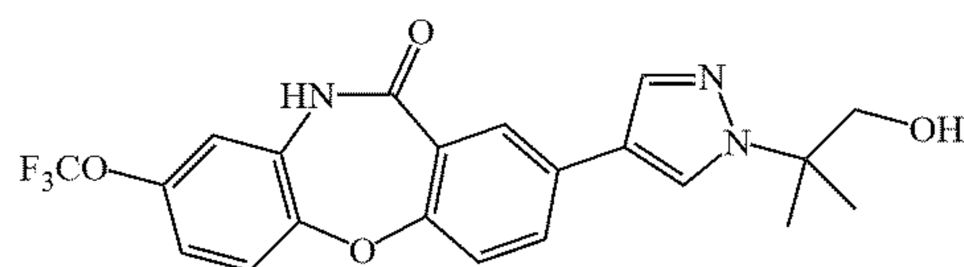
Chemical Formula: C 21 H 18 F 3 N 3 O 4 Exact Mass: 433.12 Molecular Weight: 433.39
