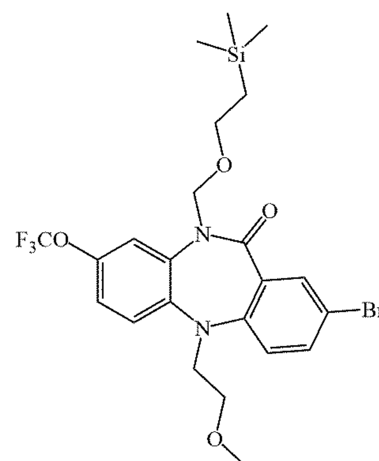
Chemical Formula: C_{23}H_{28}BrF_3N_2O_4Si Exact Mass: 544.10 Molecular Weight: 545.47
