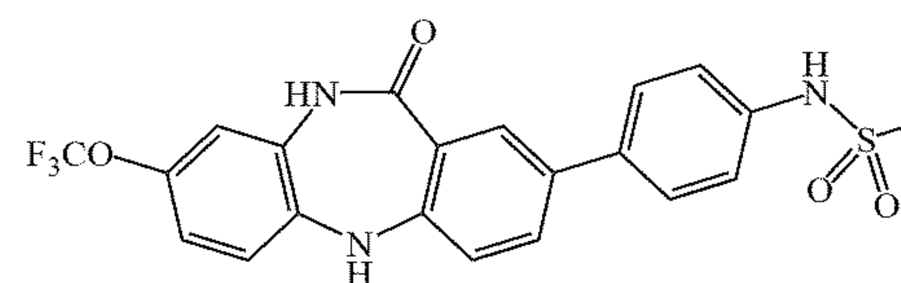
Chemical Formula: C_{21}H_{16}F_3N_3O_4S Exact Mass: 463.08 Molecular Weight: 463.43
