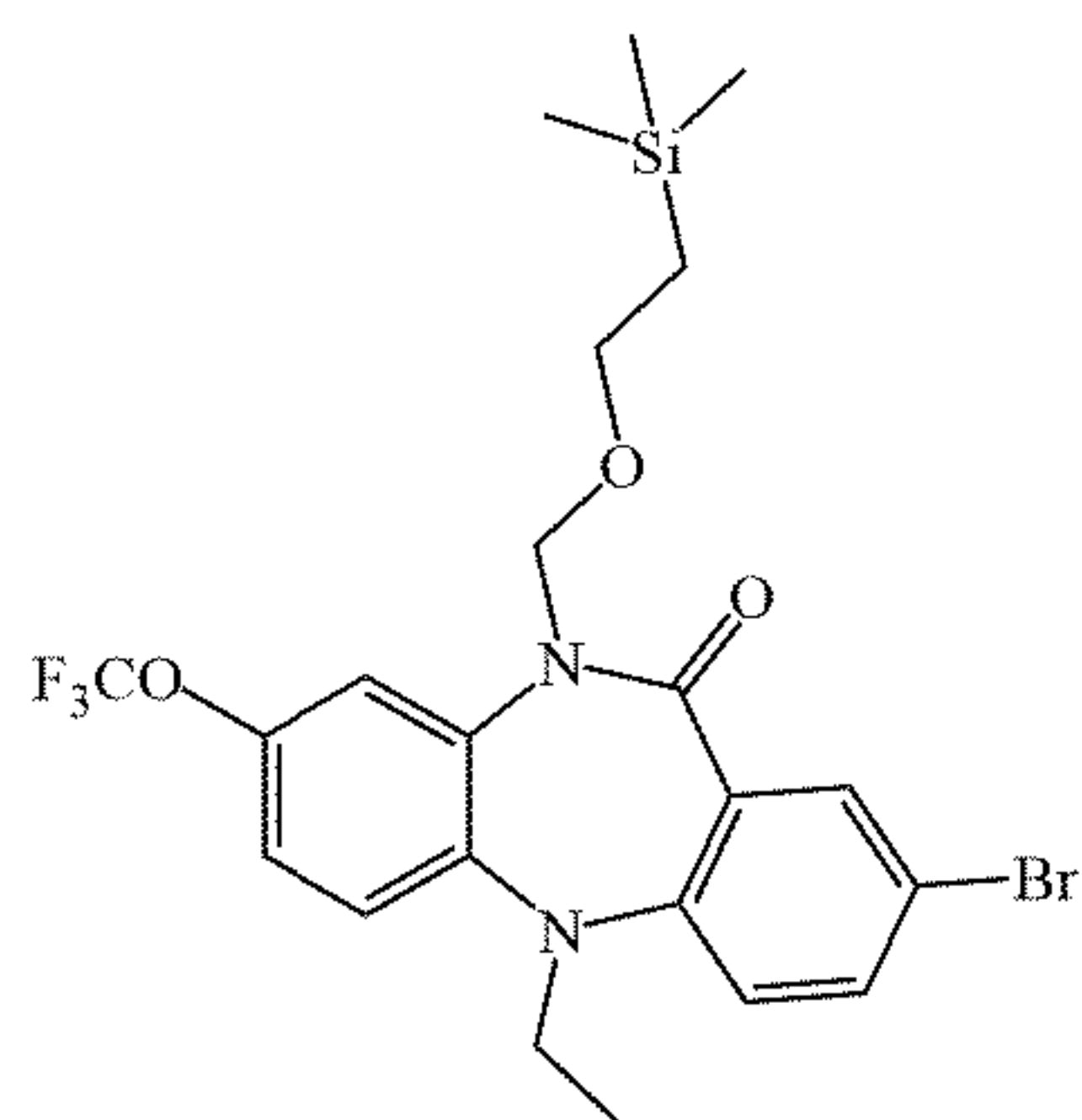
Chemical Formula: C_{22}H_{26}BrF_3N_2O_3Si Exact Mass: 530.08 Molecular Weight: 531.45
