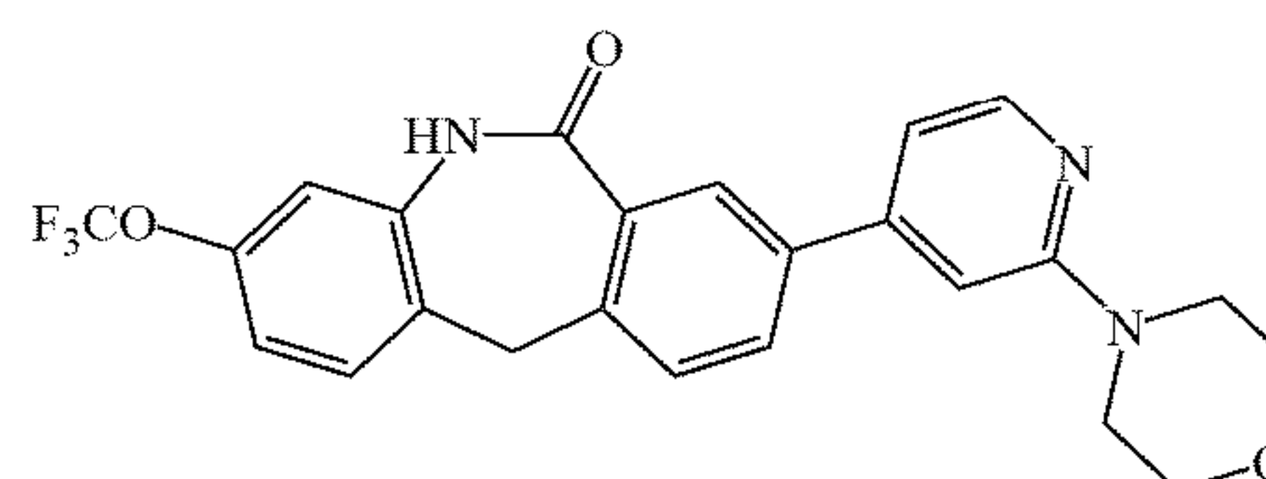
Chemical Formula: C 24 H 20 F 3 N 3 O 2 Exact Mass: 455.15 Molecular Weight: 455.14
