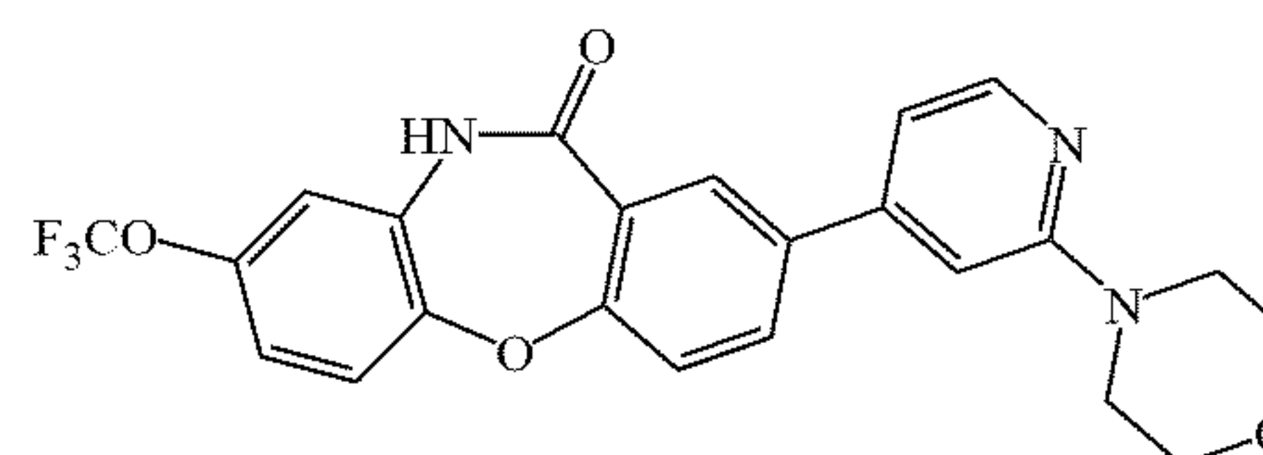
Chemical Formula: C 23 H 18 F 3 N 3 O 4 Exact Mass: 457.12 Molecular Weight: 457.41
