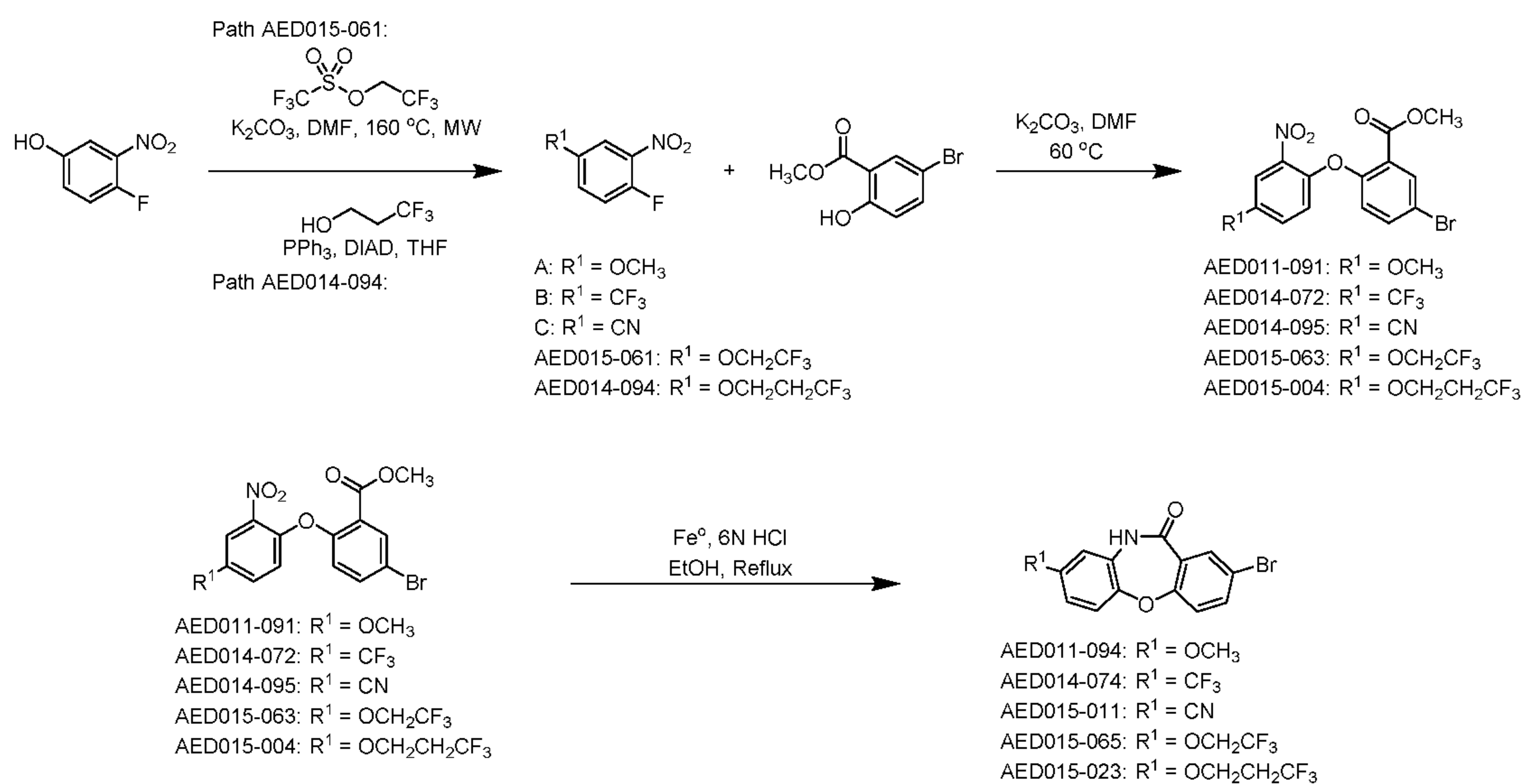
Scheme 6
