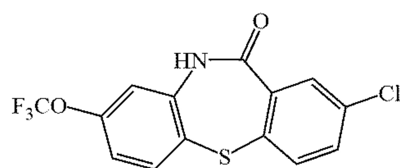
Chemical Formula: C_{14}H_7ClF_3NO_2S Exact Mass: 344.98 Molecular Weight: 345.72
