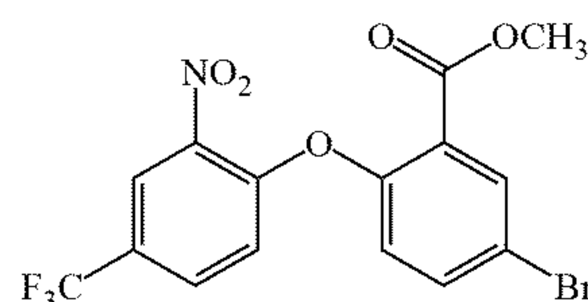
Chemical Formula: C 15 H 9 BrF 3 NO 5 Exact Mass: 418.96 Molecular Weight: 420.14
