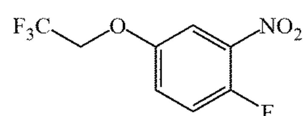
Chemical Formula: C 8 H 5 F 4 NO 3 Exact Mass: 239.02 Molecular Weight: 239.13
