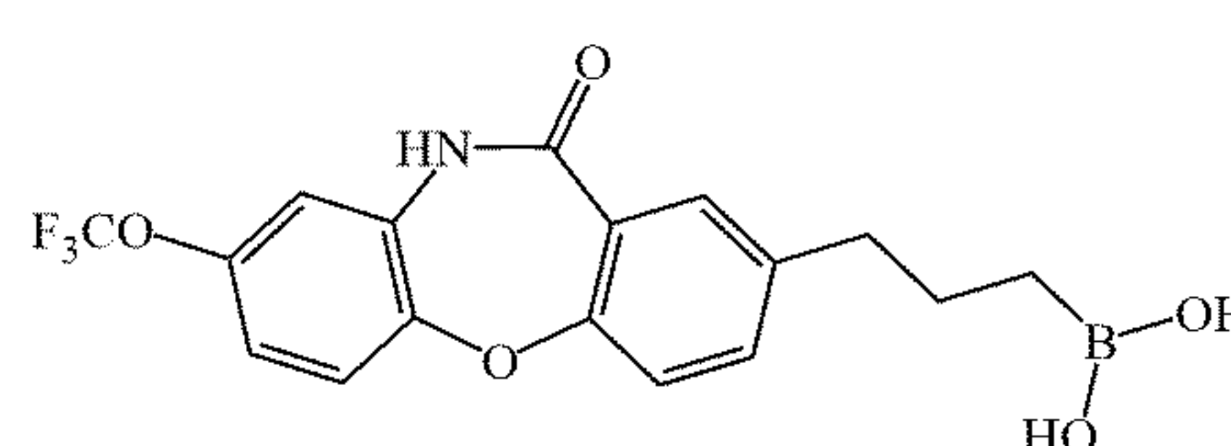
Chemical Formula: C_{17}H_{15}BF_3NO_5 Exact Mass: 381.10 Molecular Weight: 381.11
