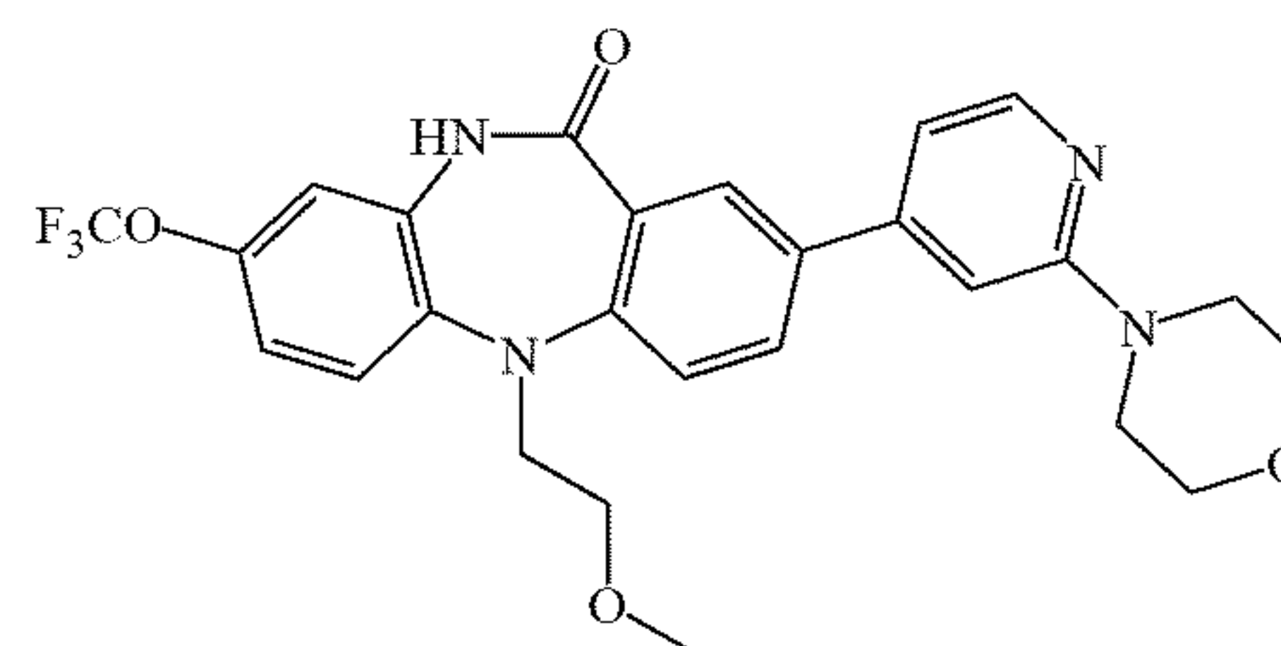
Chemical Formula: \text{C}_{26}\text{H}_{25}\text{F}_3\text{N}_4\text{O}_4 Exact Mass: 514.18 Molecular Weight: 514.51
