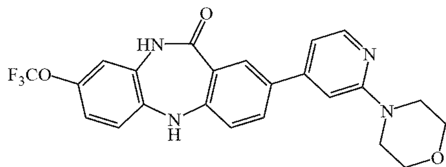
Chemical Formula: C_{23}H_{19}F_3N_4O_3 Exact Mass: 456.14 Molecular Weight: 456.43
