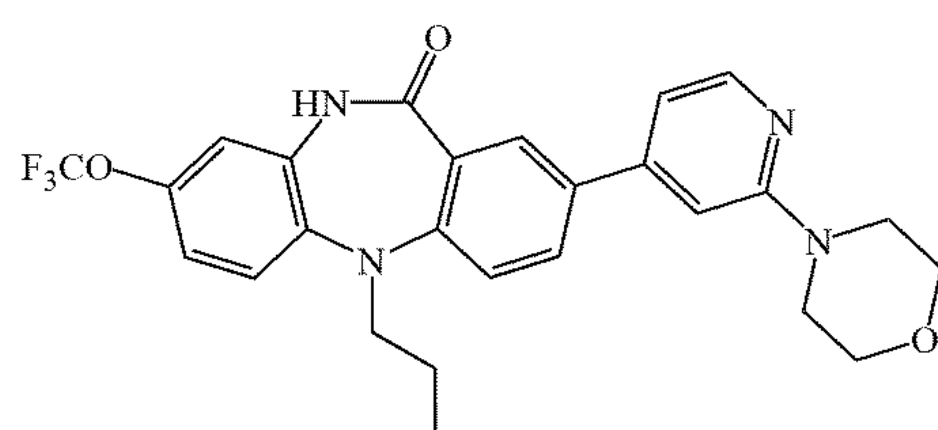
Chemical Formula: \text{C}_{26}\text{H}_{25}\text{F}_3\text{N}_4\text{O}_3 Exact Mass: 498.19 Molecular Weight: 498.51
