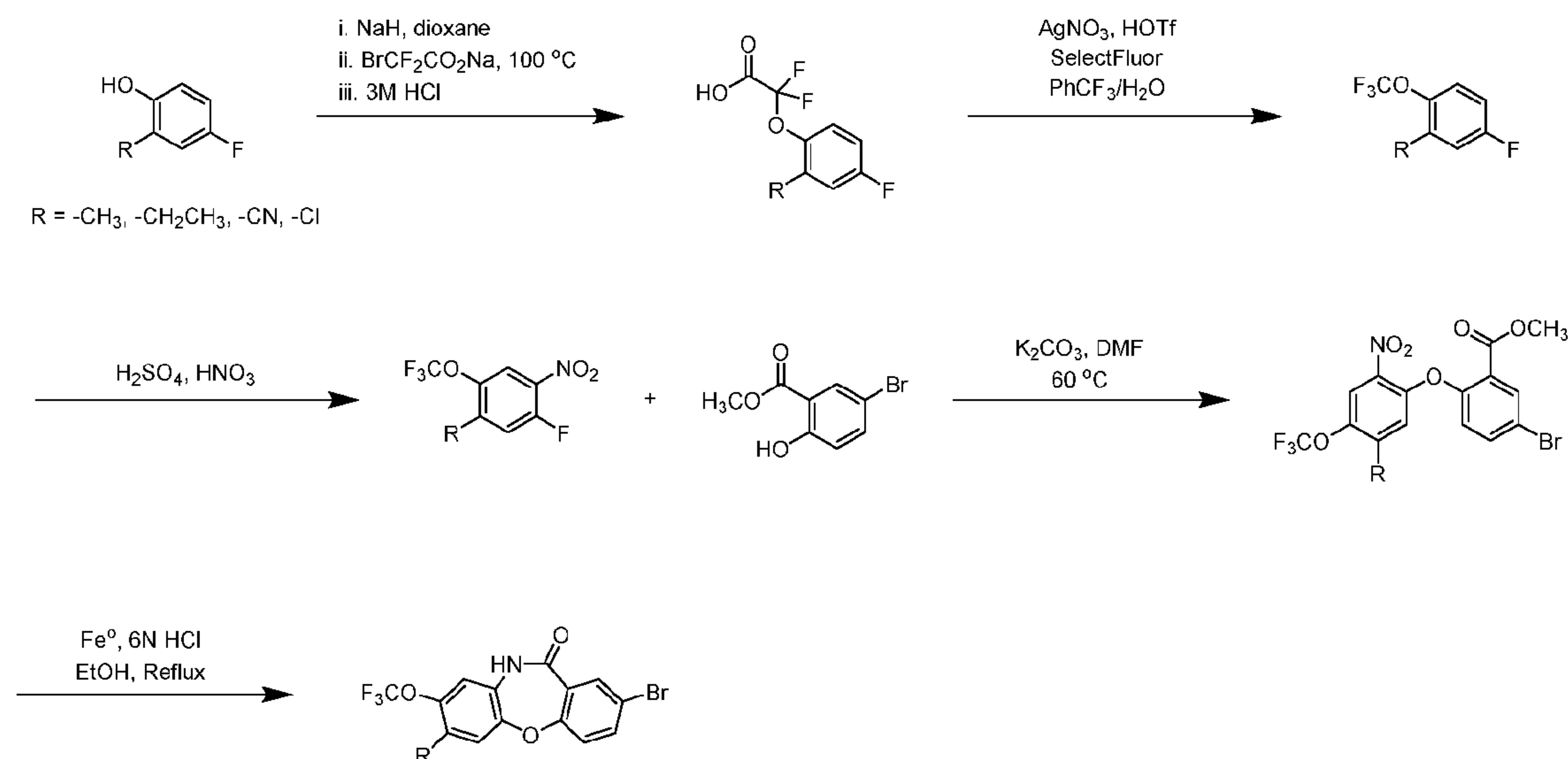
Scheme 11
