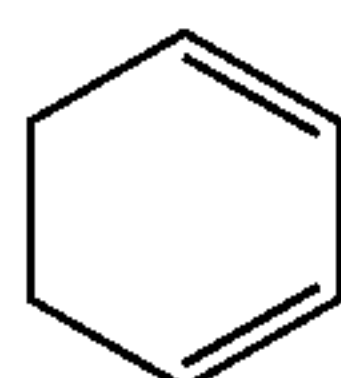
1,3-Cyclohexadiene C_6H_8 BP = 80^\circ C. , Vapor Pressure: 56 mmHg at 25^\circ C.
