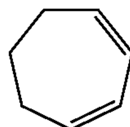
1,3-Cycloheptadiene C_7H_{12} BP = 120^\circ C. , Vapor Pressure: N/A
