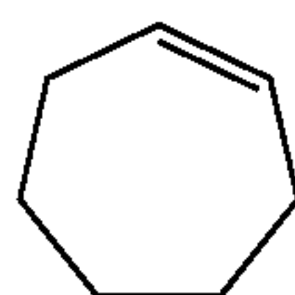
Cycloheptene C_7H_{12} BP = 113^\circ C. , Vapor Pressure: 22 mmHg at 20^\circ C.
