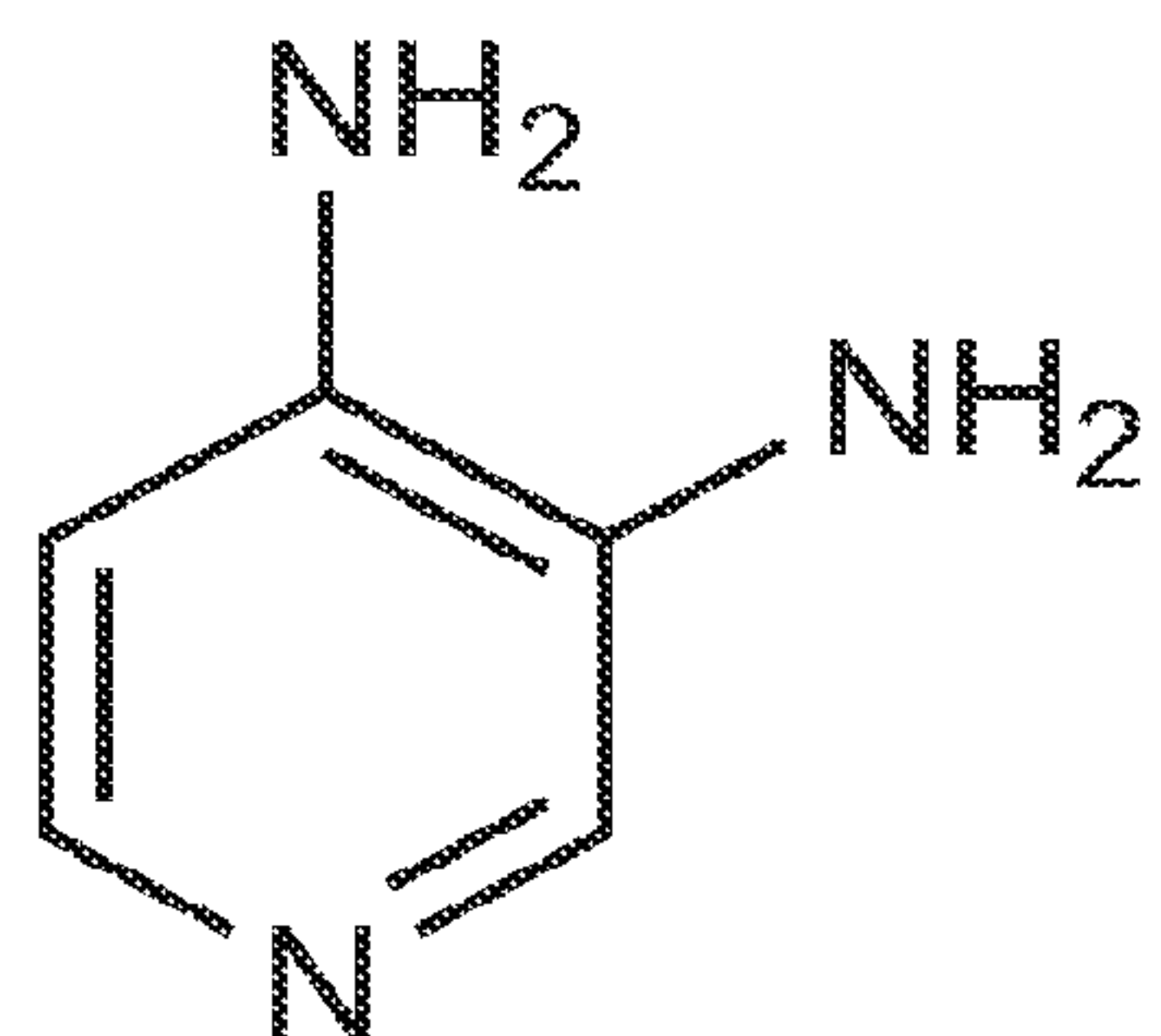
3,4-diaminopyridine
