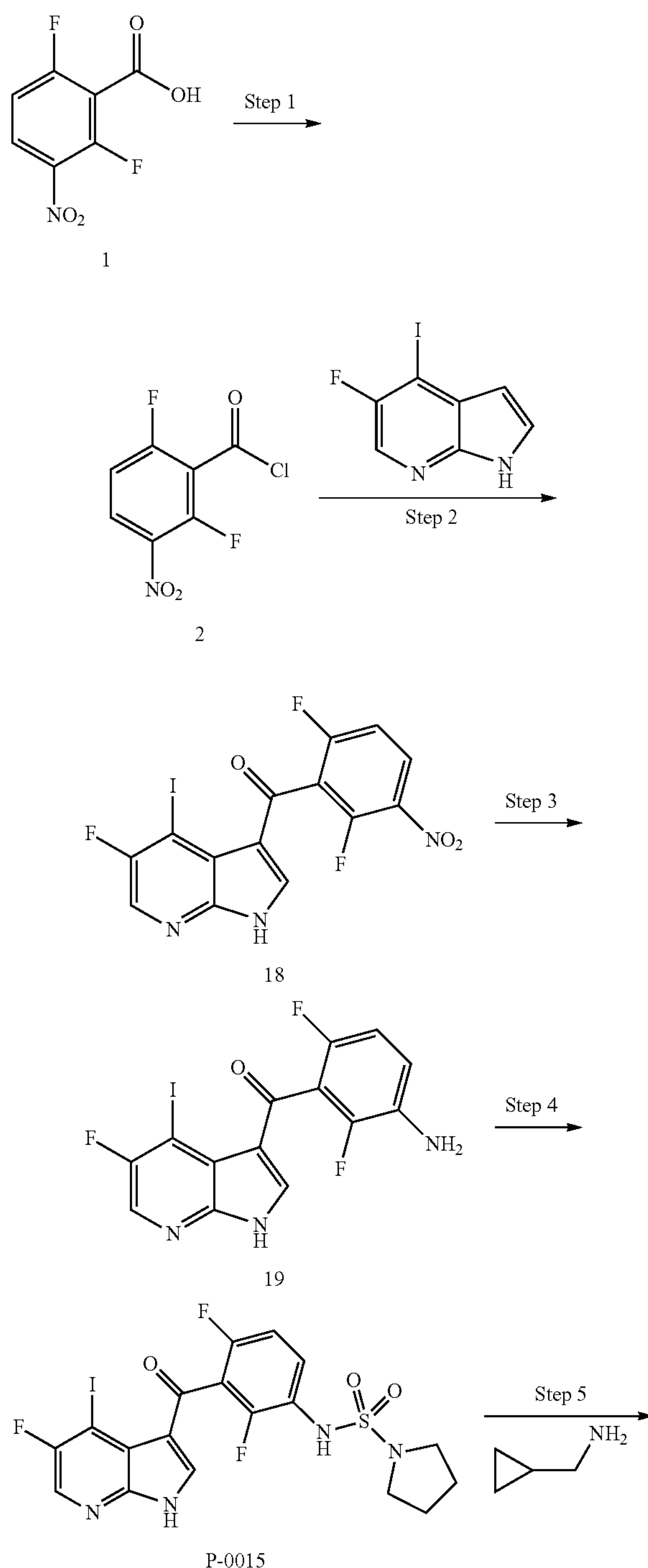
Scheme 4.
