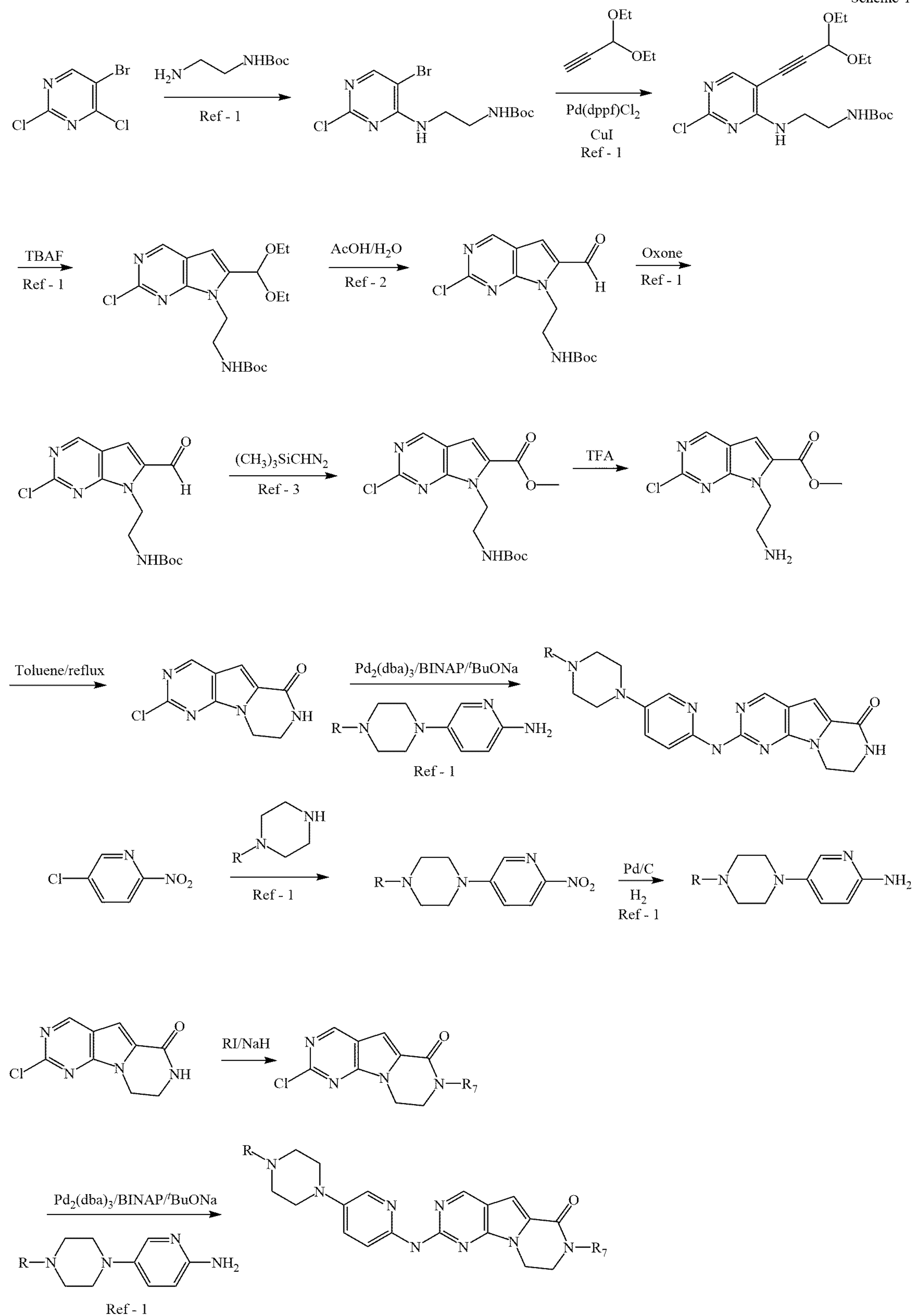
Scheme 1
