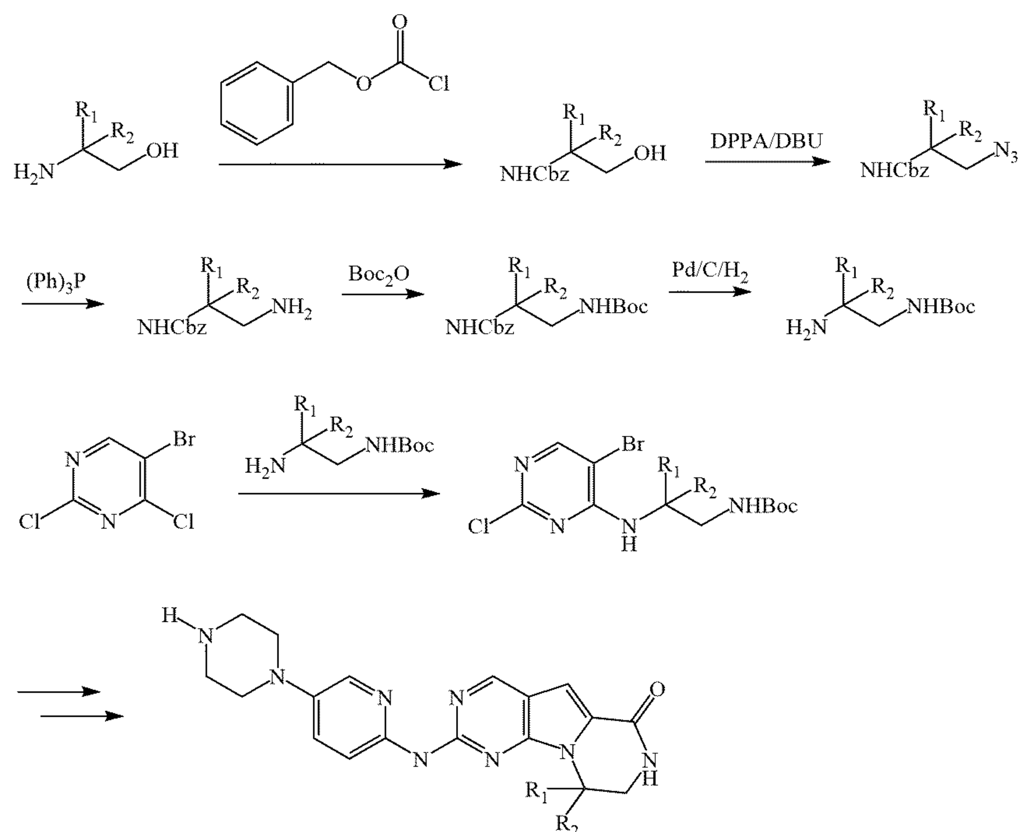
Scheme 4
