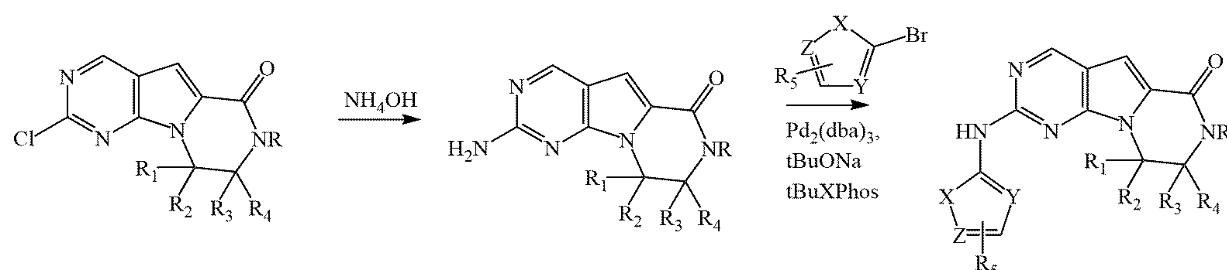
Scheme 5
