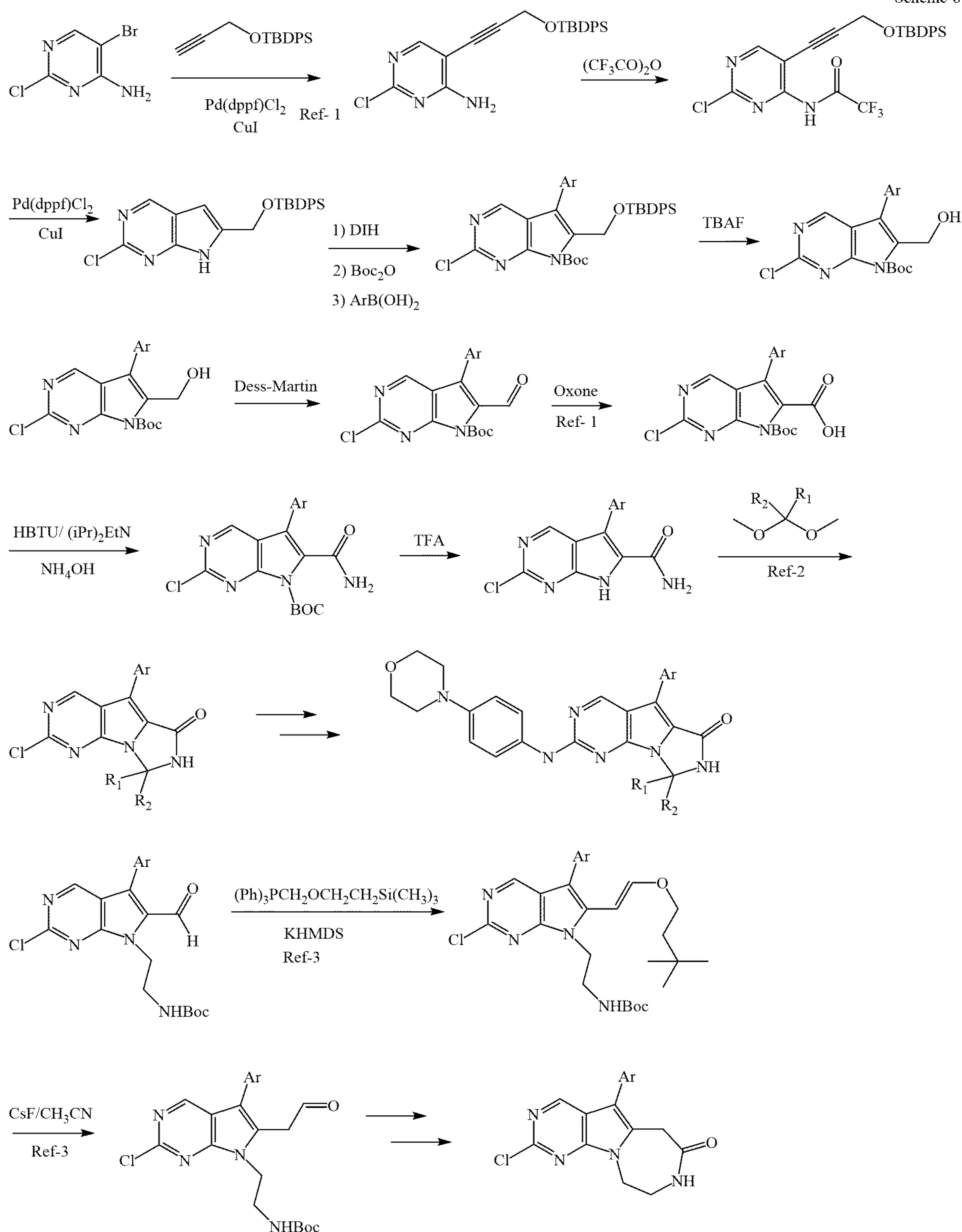
Scheme 8
