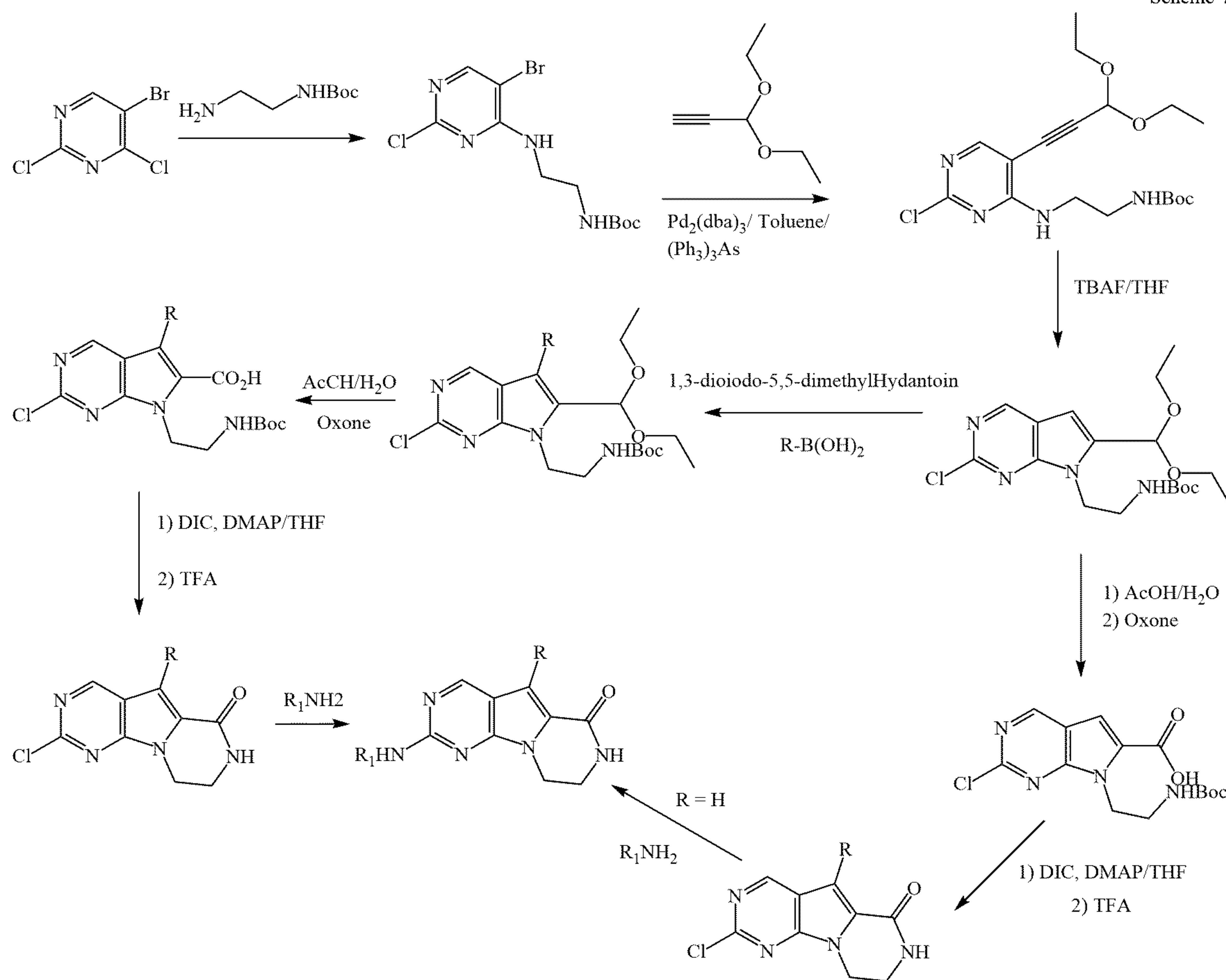
Scheme 7
