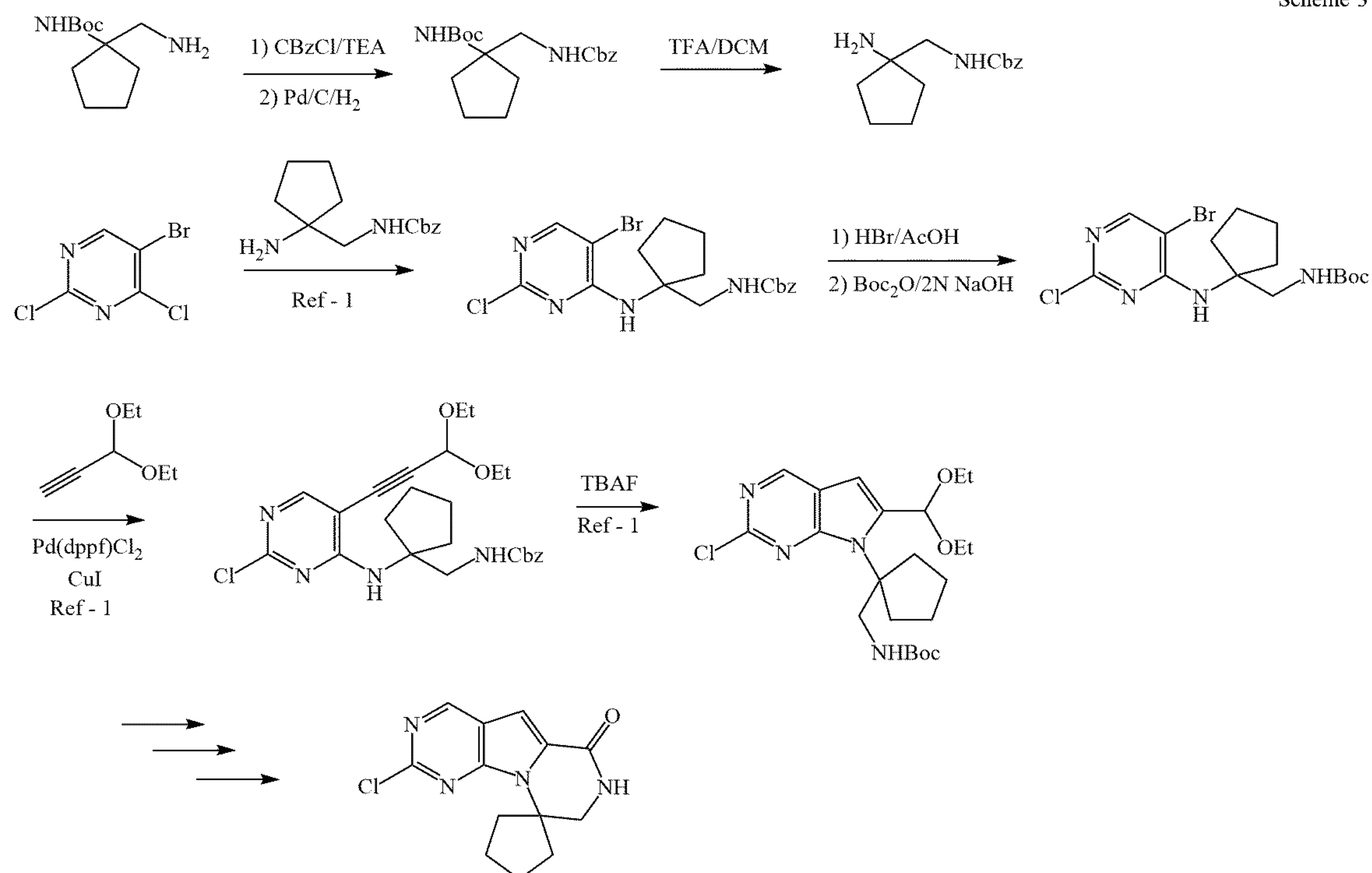
Scheme 3
