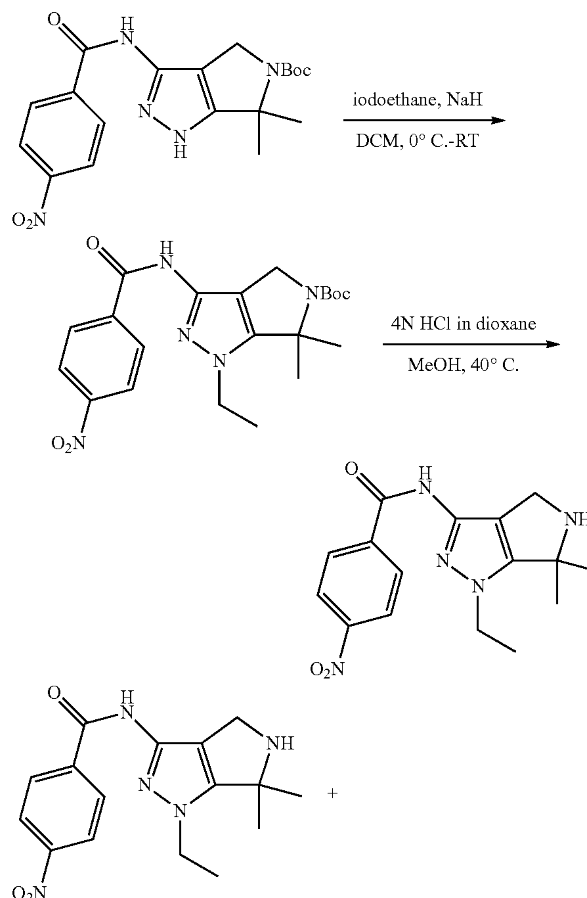
Scheme 2. synthesis of Compound I-4.
