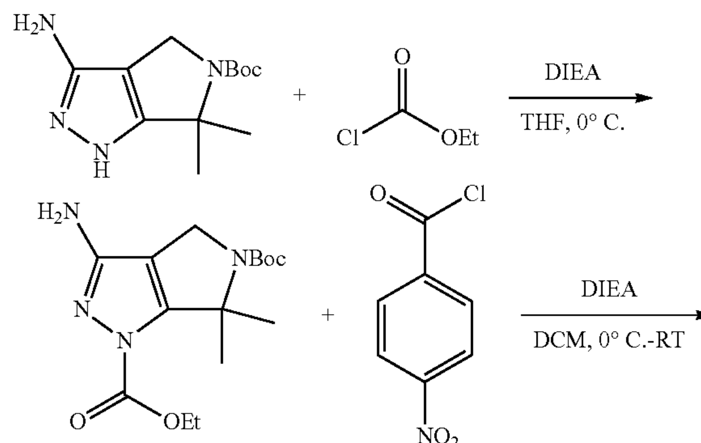
Scheme 1. Exemplary synthesis of Compound I-1.
