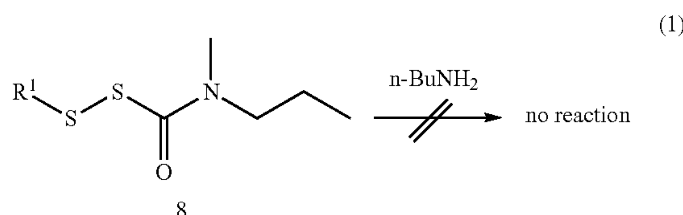
Scheme 4. Reaction of 8 with n-BuNH 2 and N-acetyl cysteine
