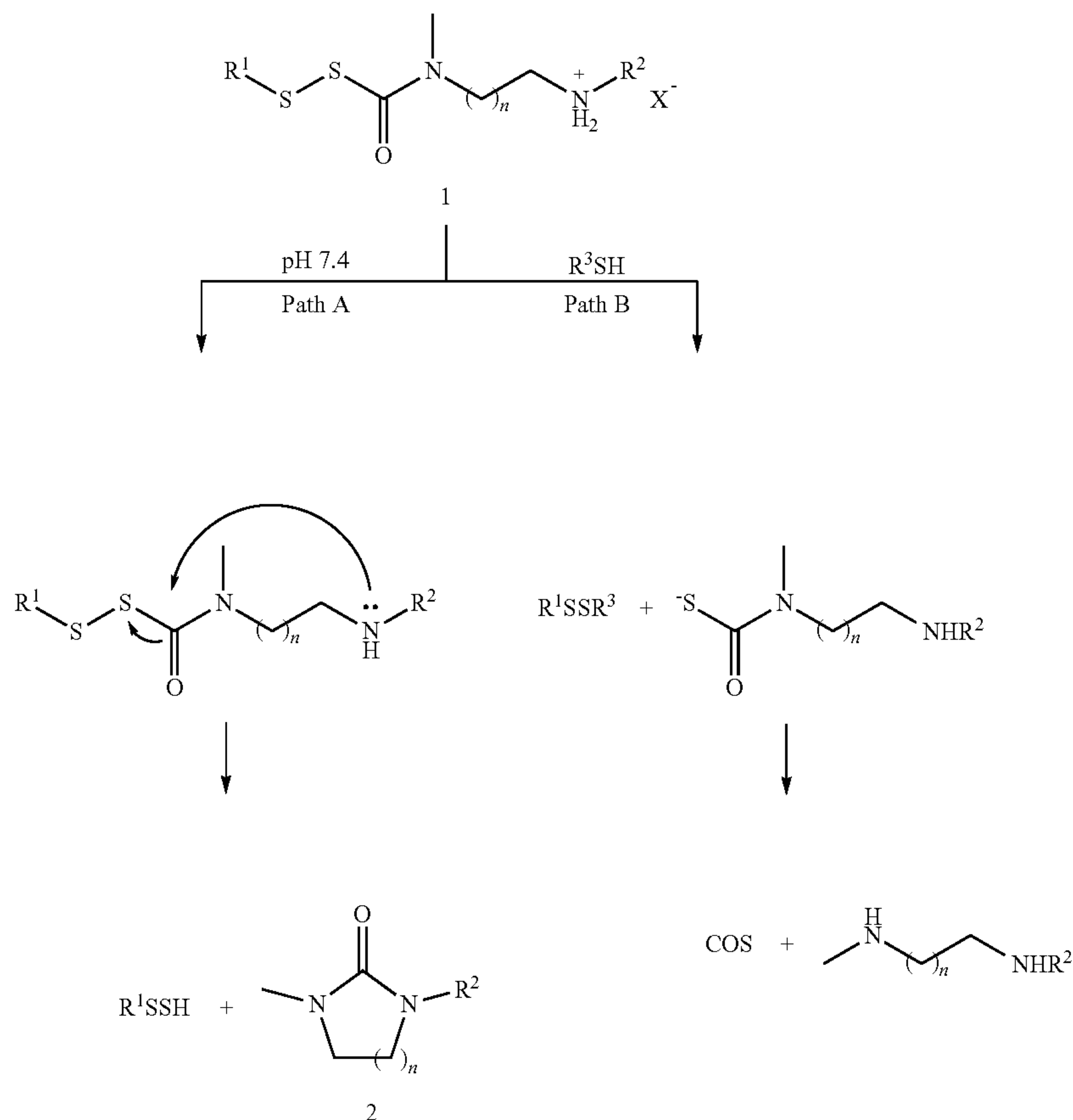
Scheme 1. Design of hydropersulfide/carbonyl sulfide precursors.
