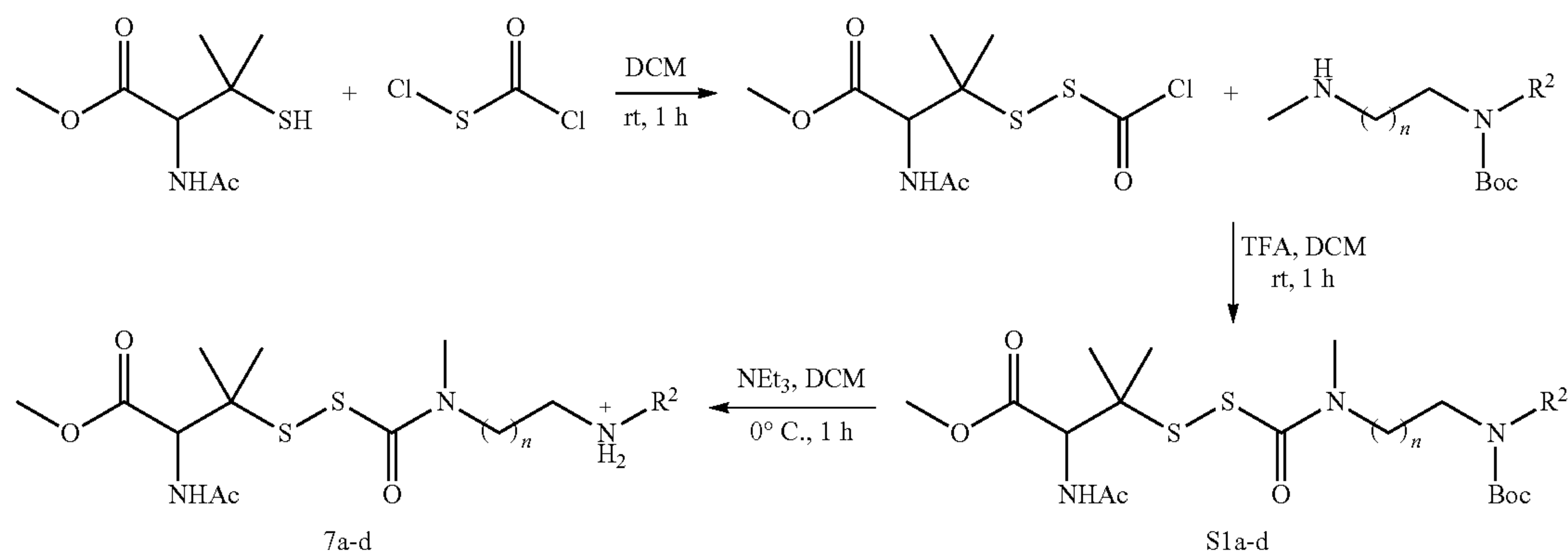
Scheme 7. Synthesis of alkylamine-substituted perthiocarbamates 7a-d
