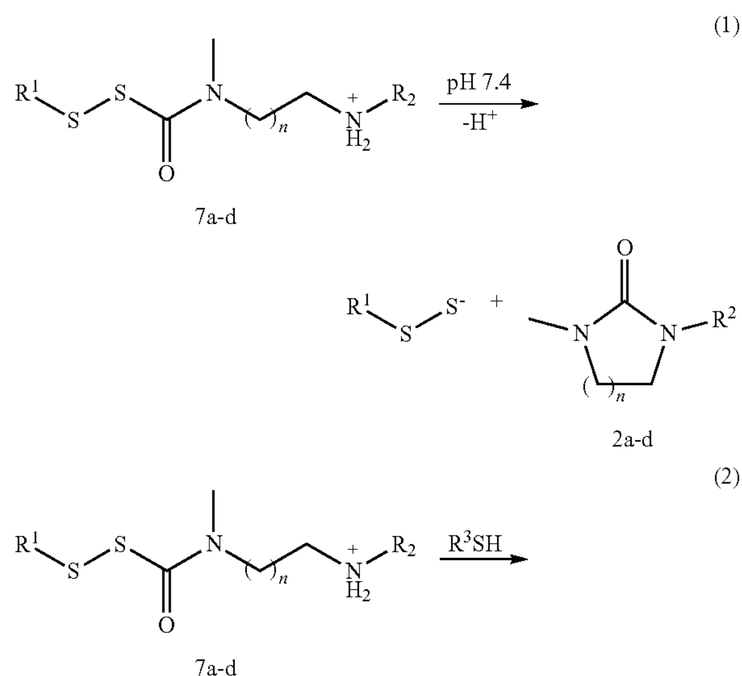
Scheme 6. RSSH and COS Generation from 7a-d in the Presence of Thiol.
