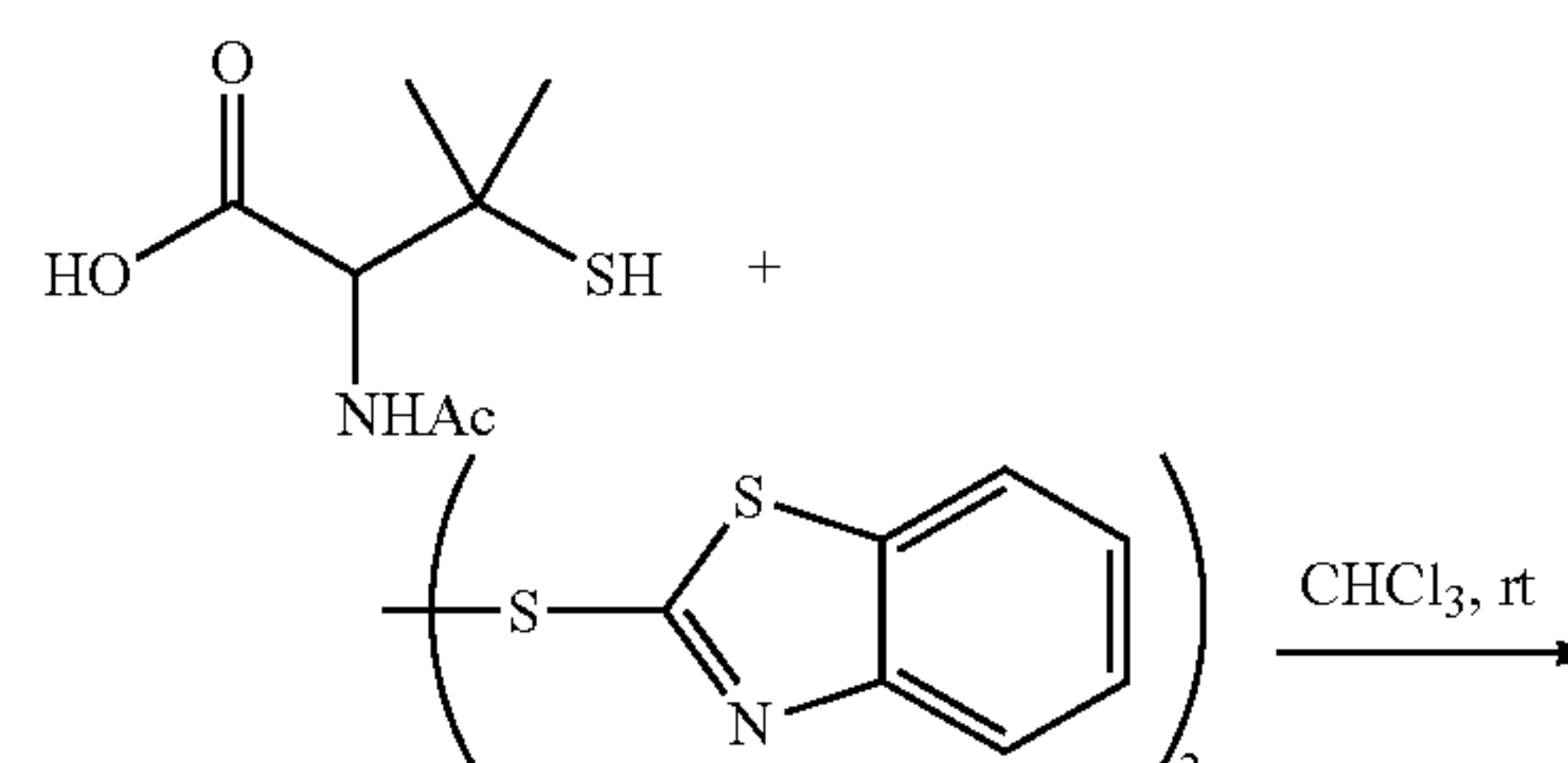
Scheme 5. Synthesis of RSS-HPE-AM 9.
