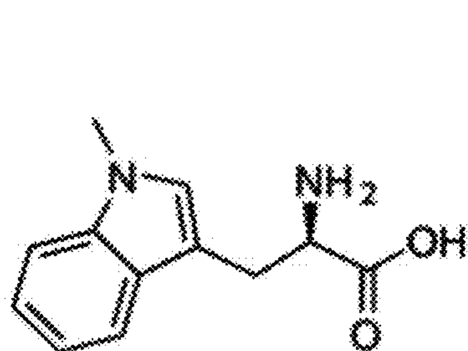
Indoximod
