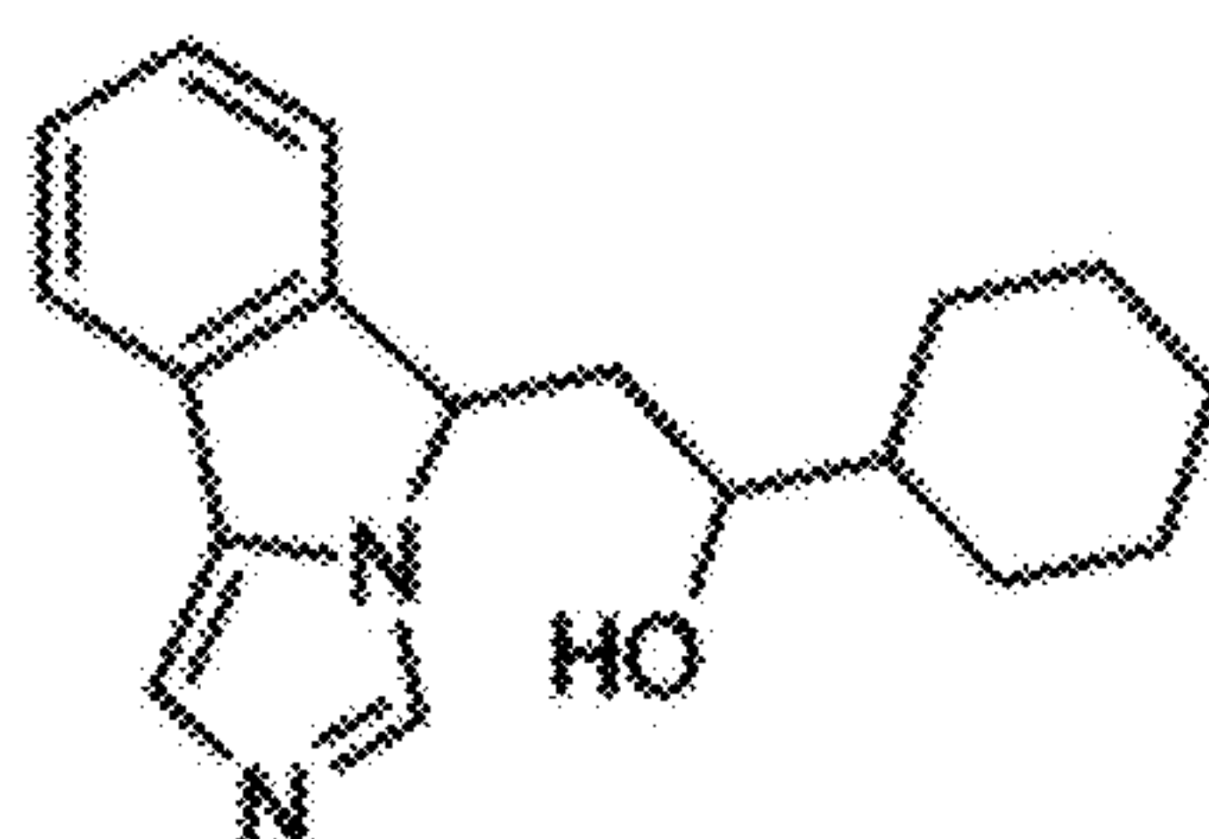
NLG919
