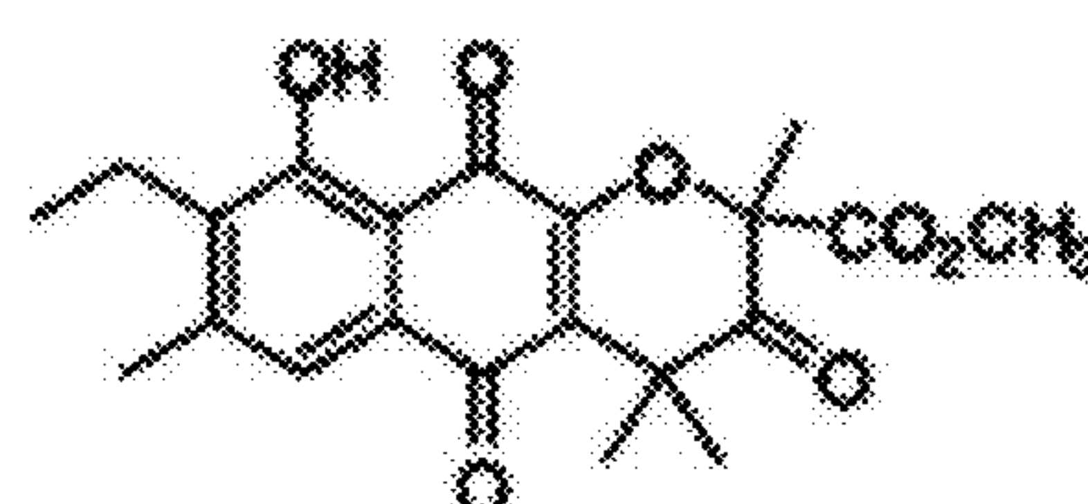
Annulin-B
