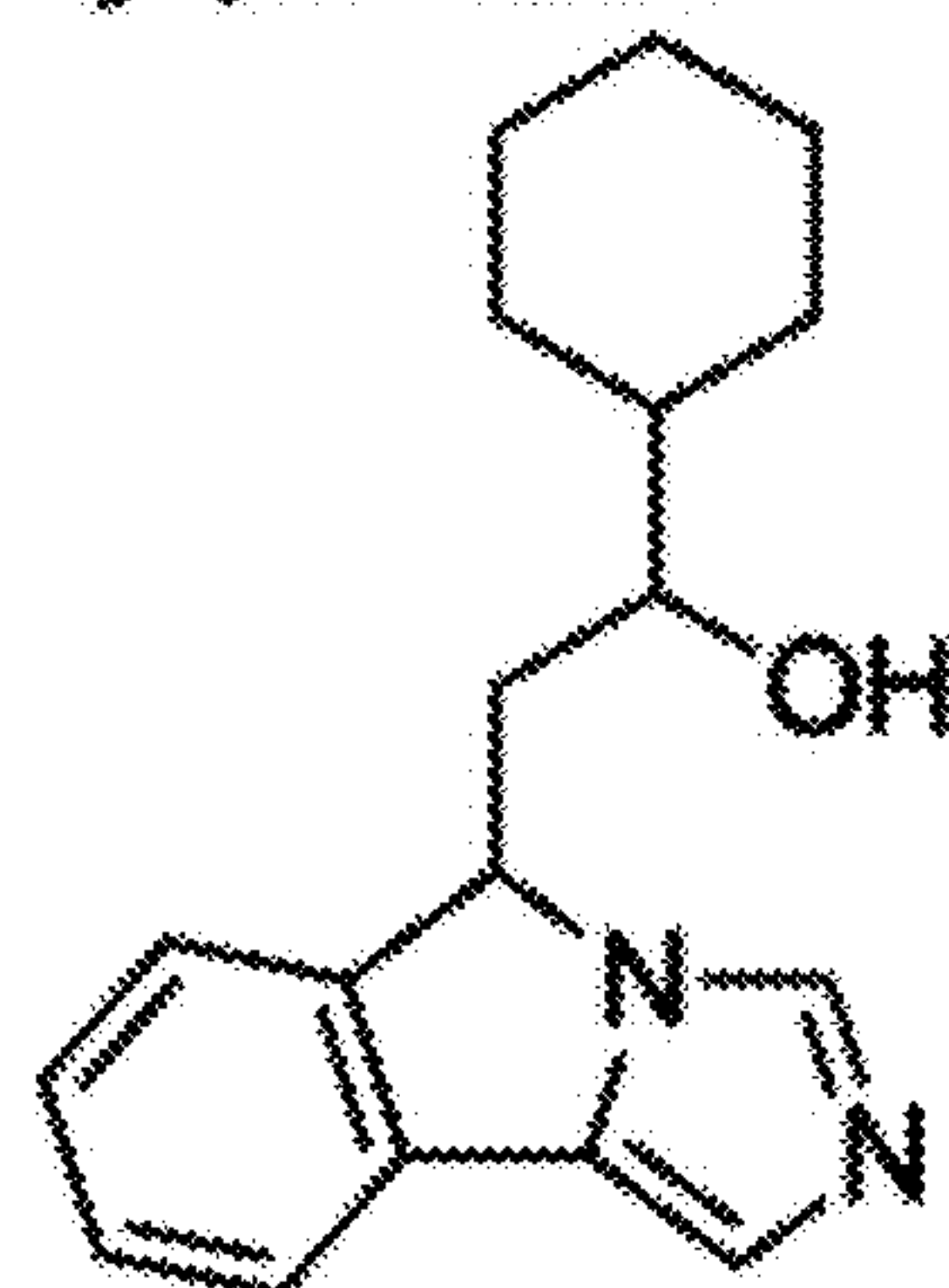
3-butyl-β-carboline
