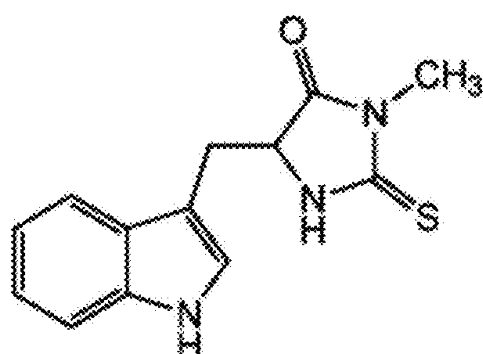
methylthiohydantoin-dl-tryptophan (Necrostatin)
