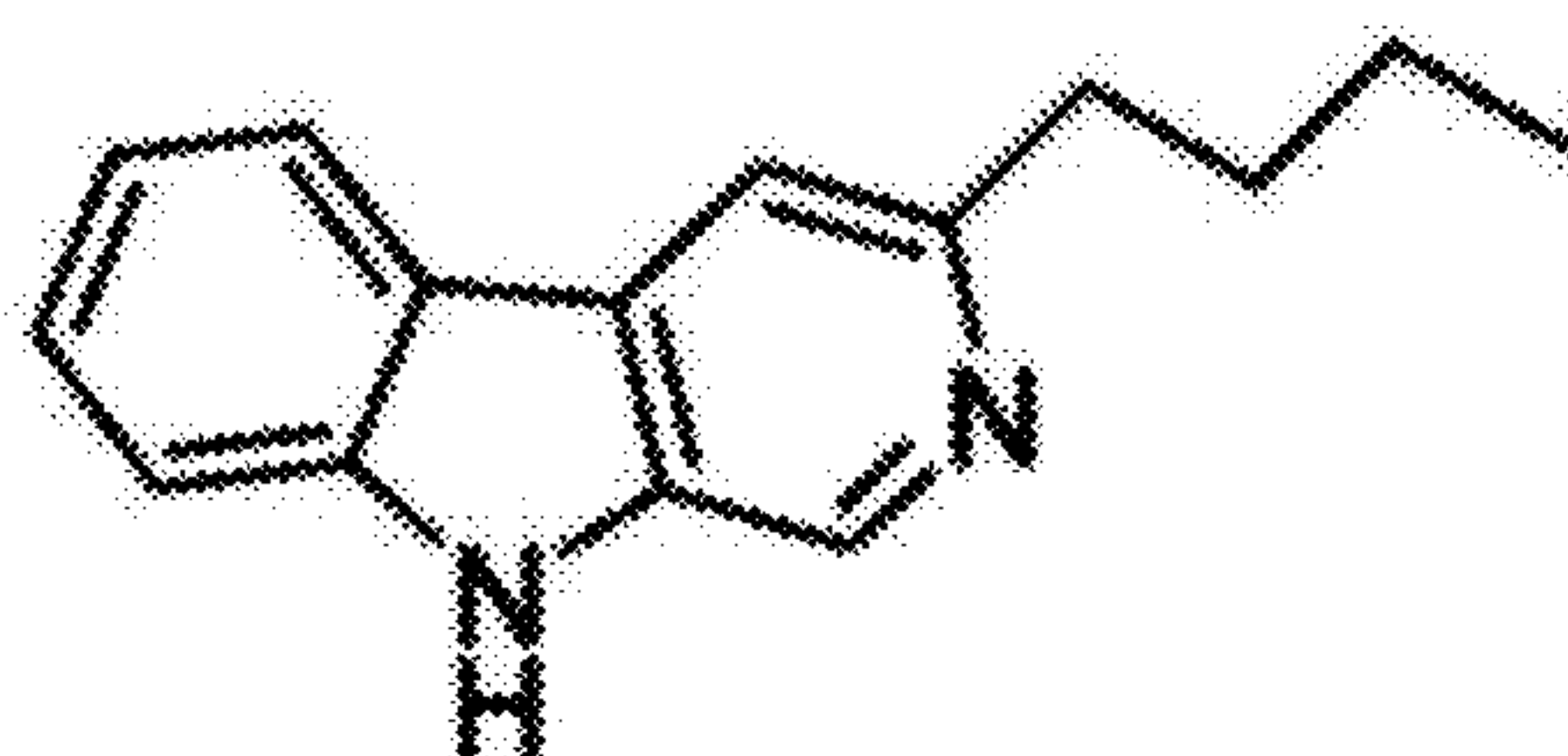
3-butyl-β-carboline
