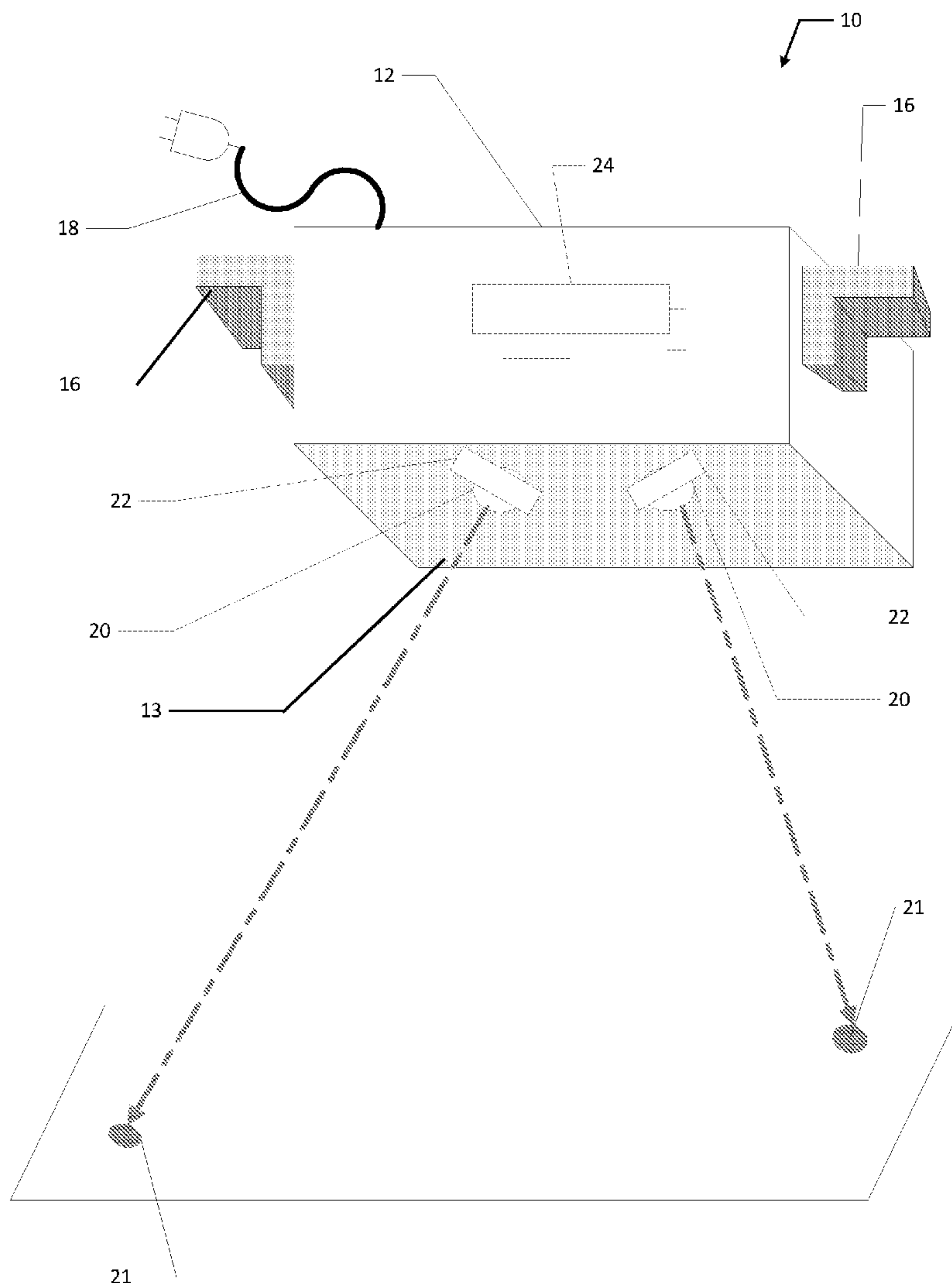
(TWO LASER APPARATUS)
