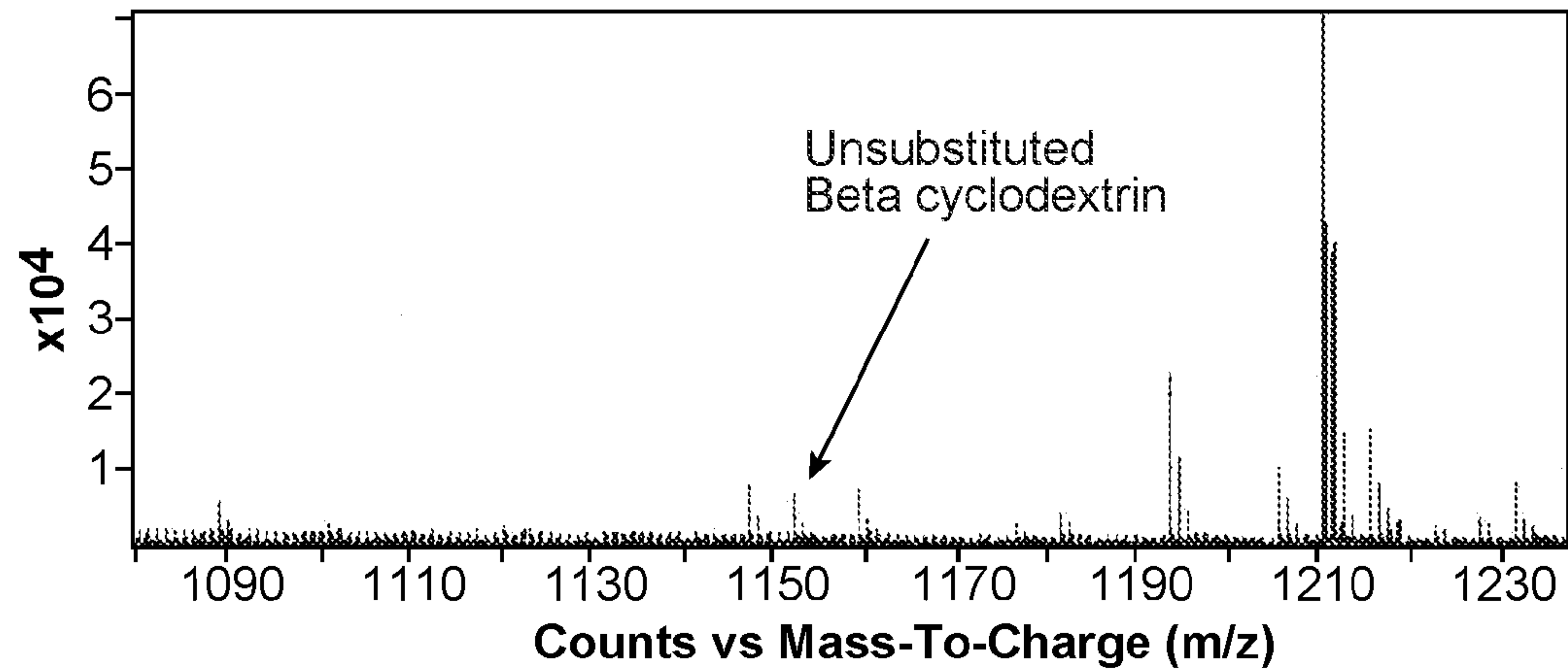
Mass Spectrum (40.03-51.95 ms)(1.553 min) - 2OH-Pr-bCD_Kleptose_Single frame_POS_001_conden..
