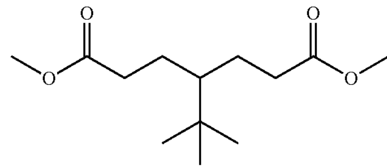
dimethyl 4-( tert -butyl)heptanedioate
