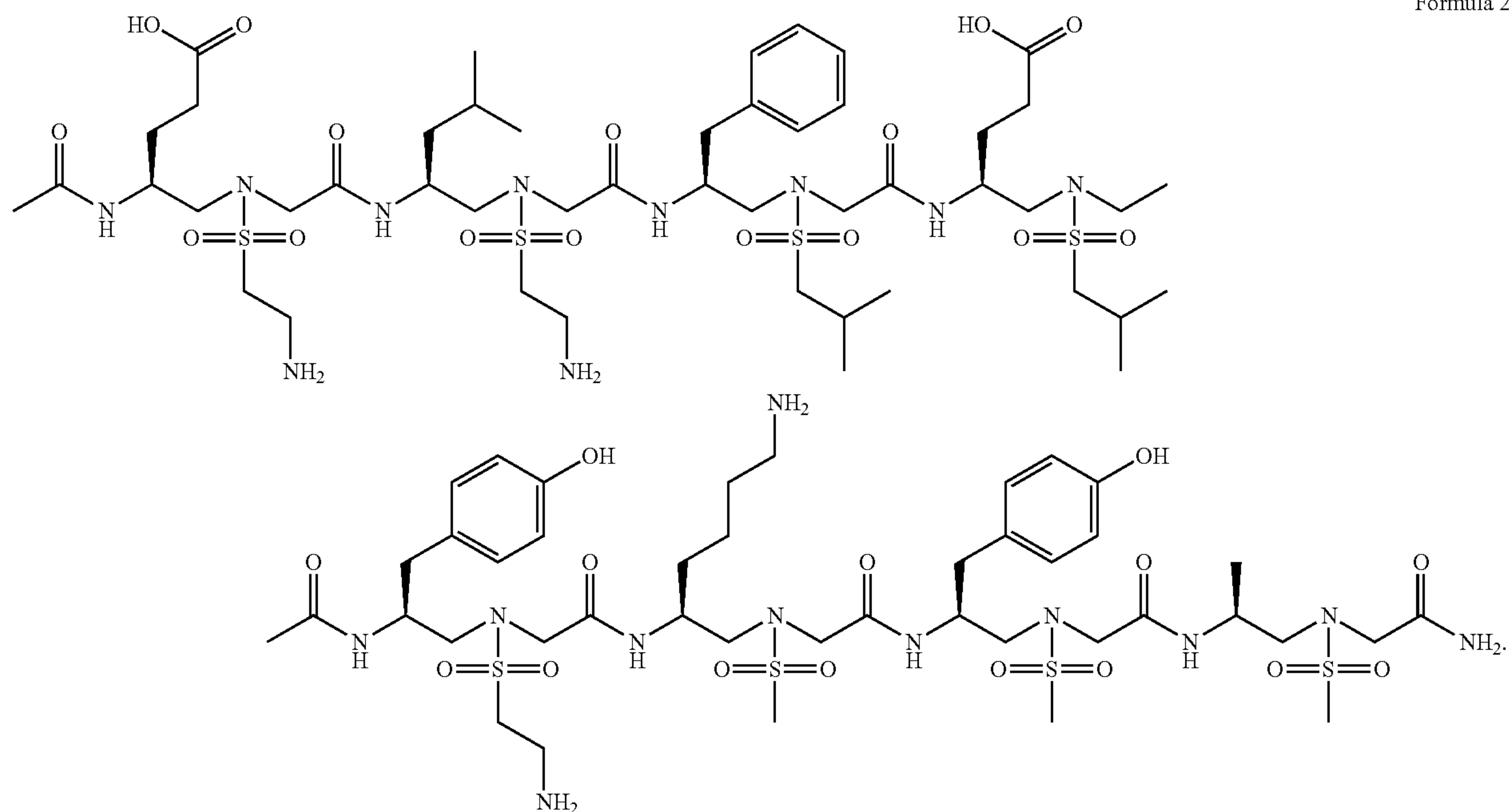
Formula 2
