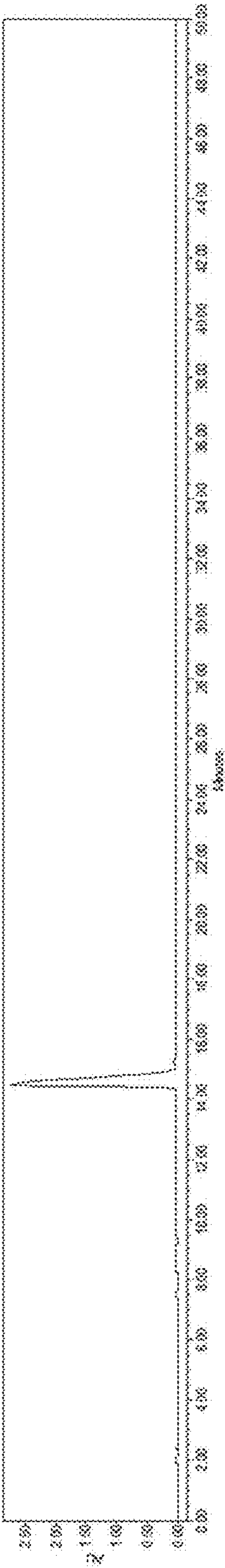
MS Spectrum Peak List
