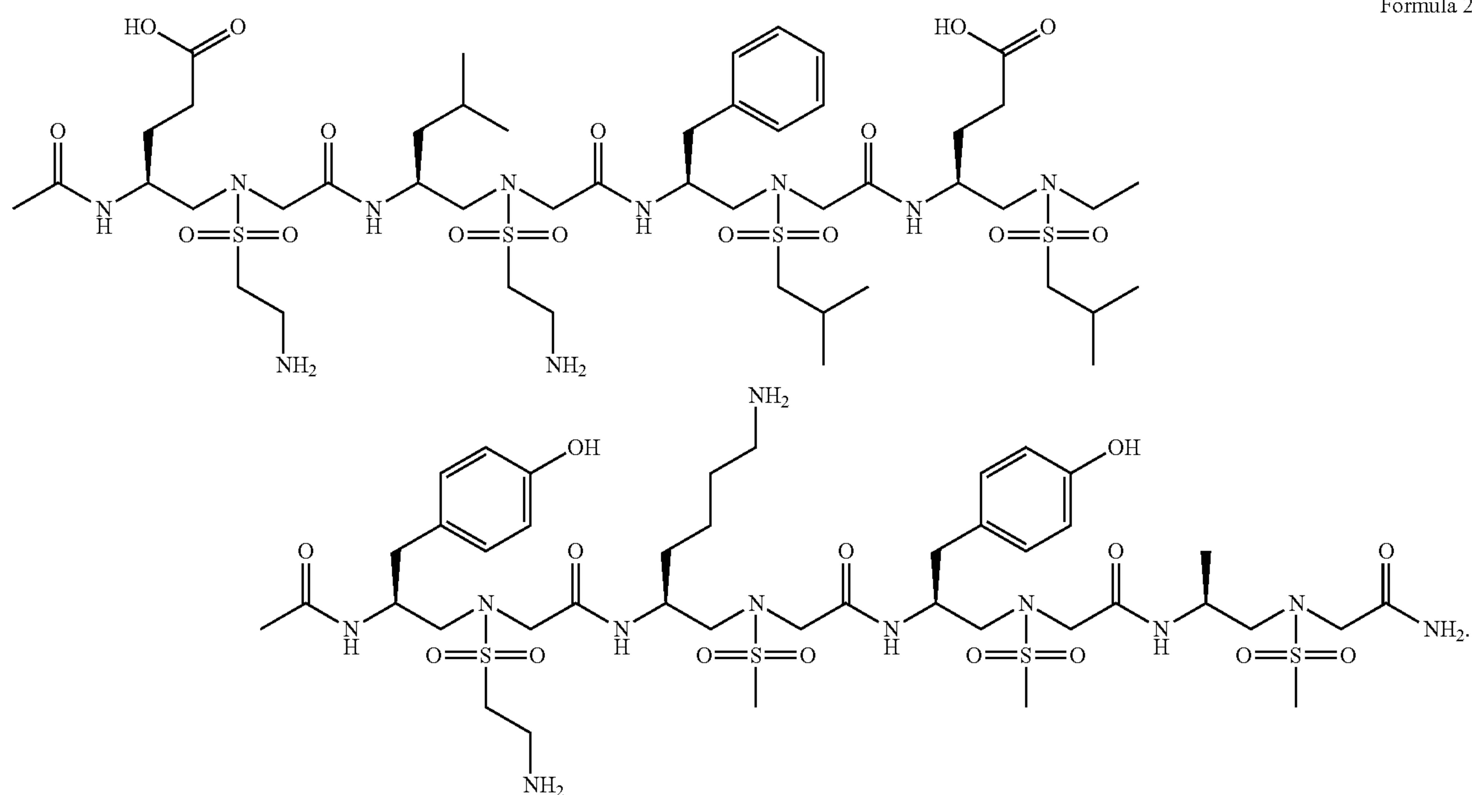
Formula 2
