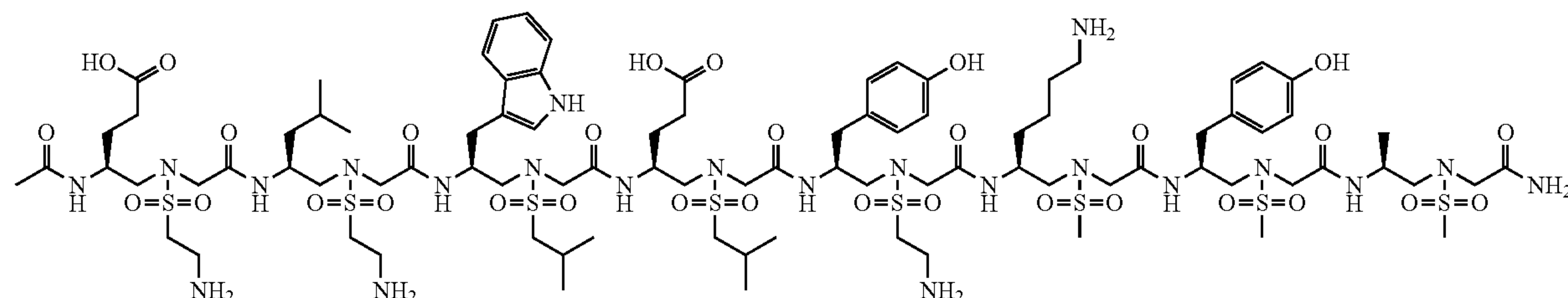
Formula 3
