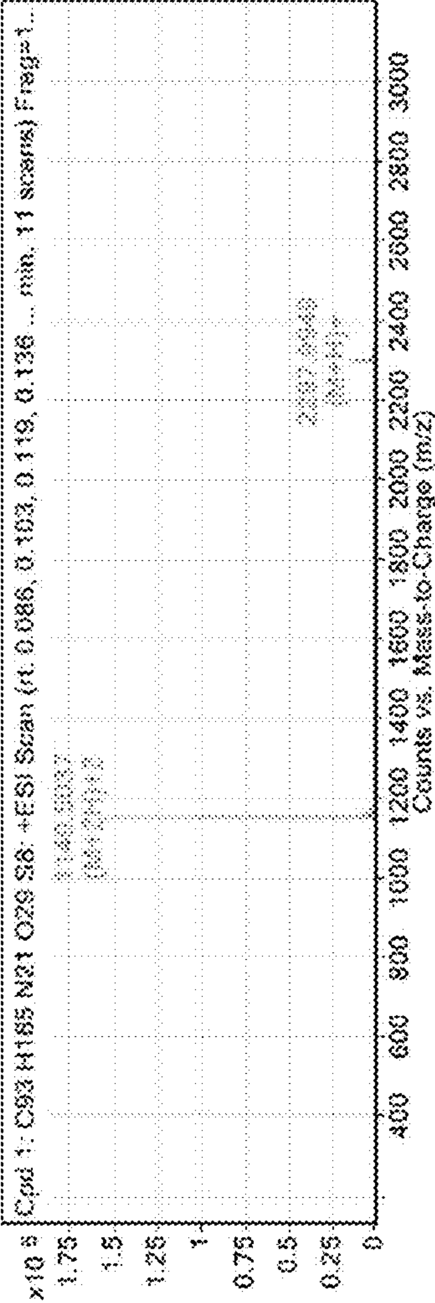
MS Spectrum
