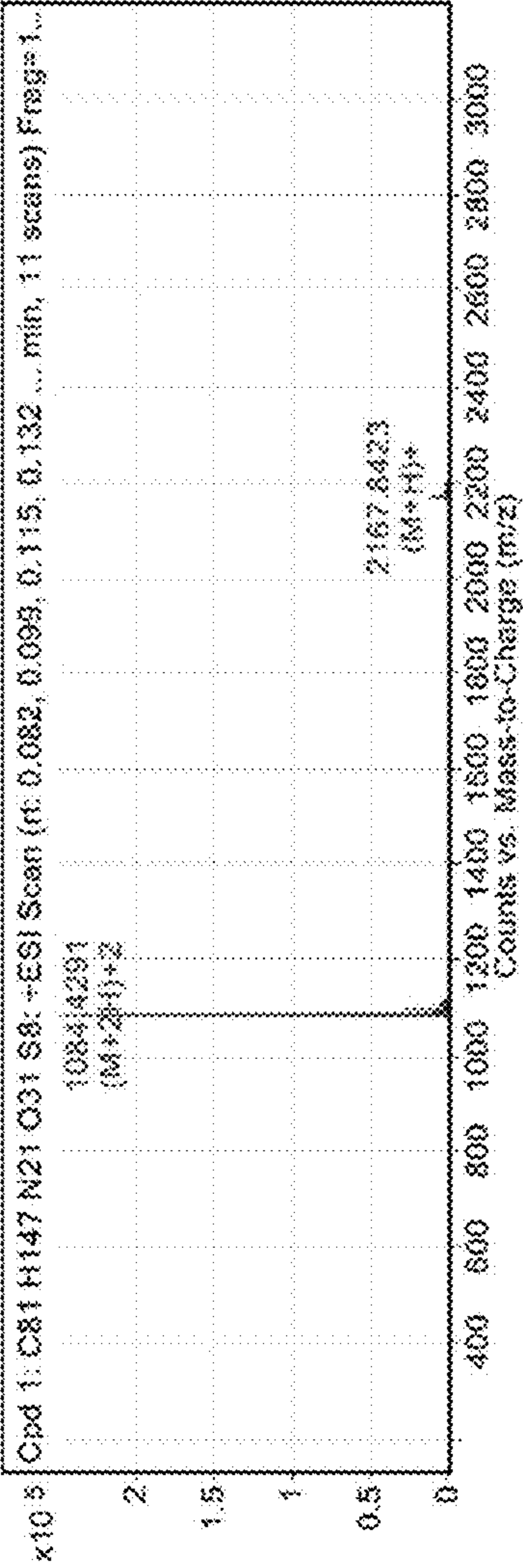
MS Spectrum
