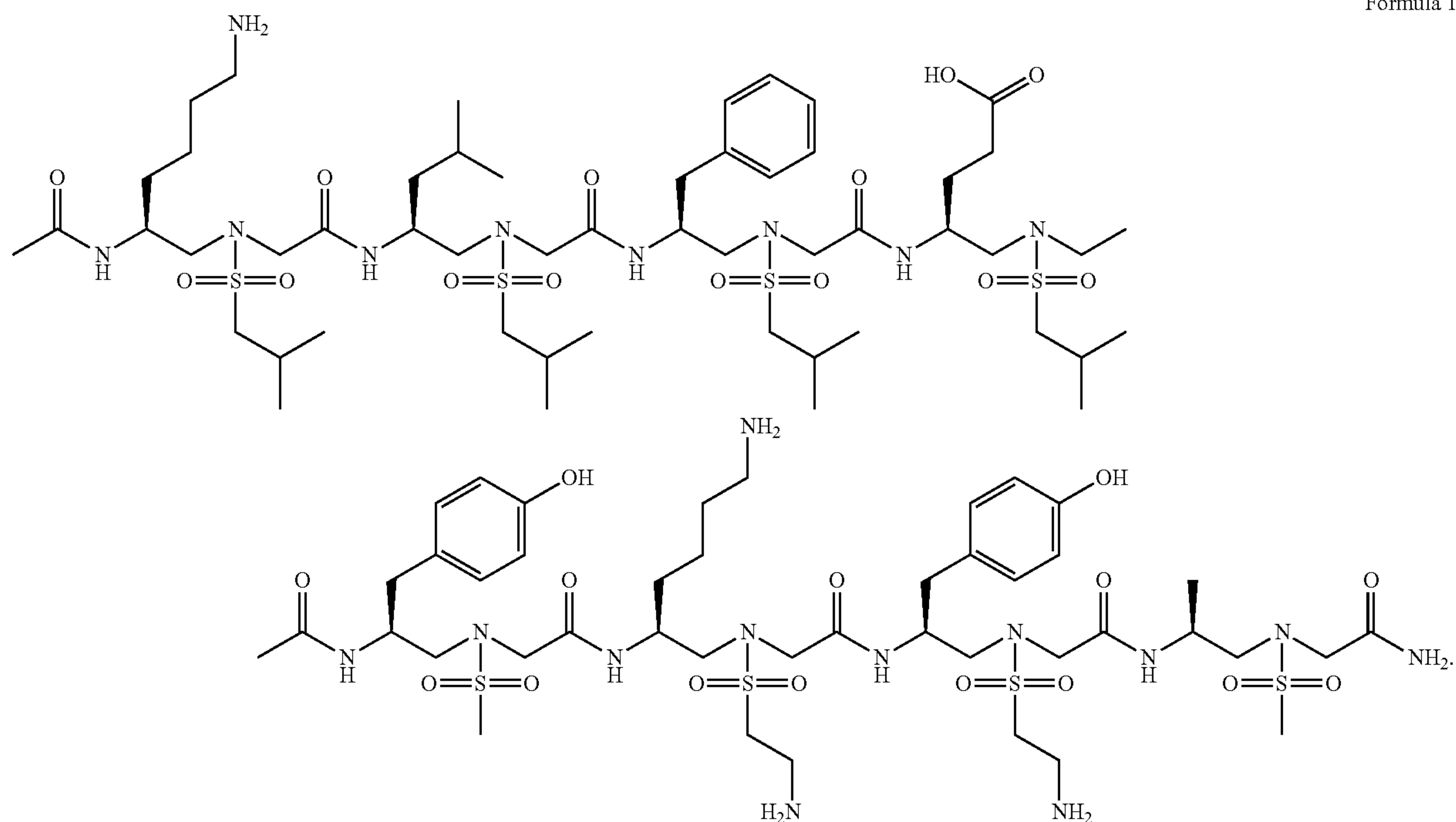
Formula 1
