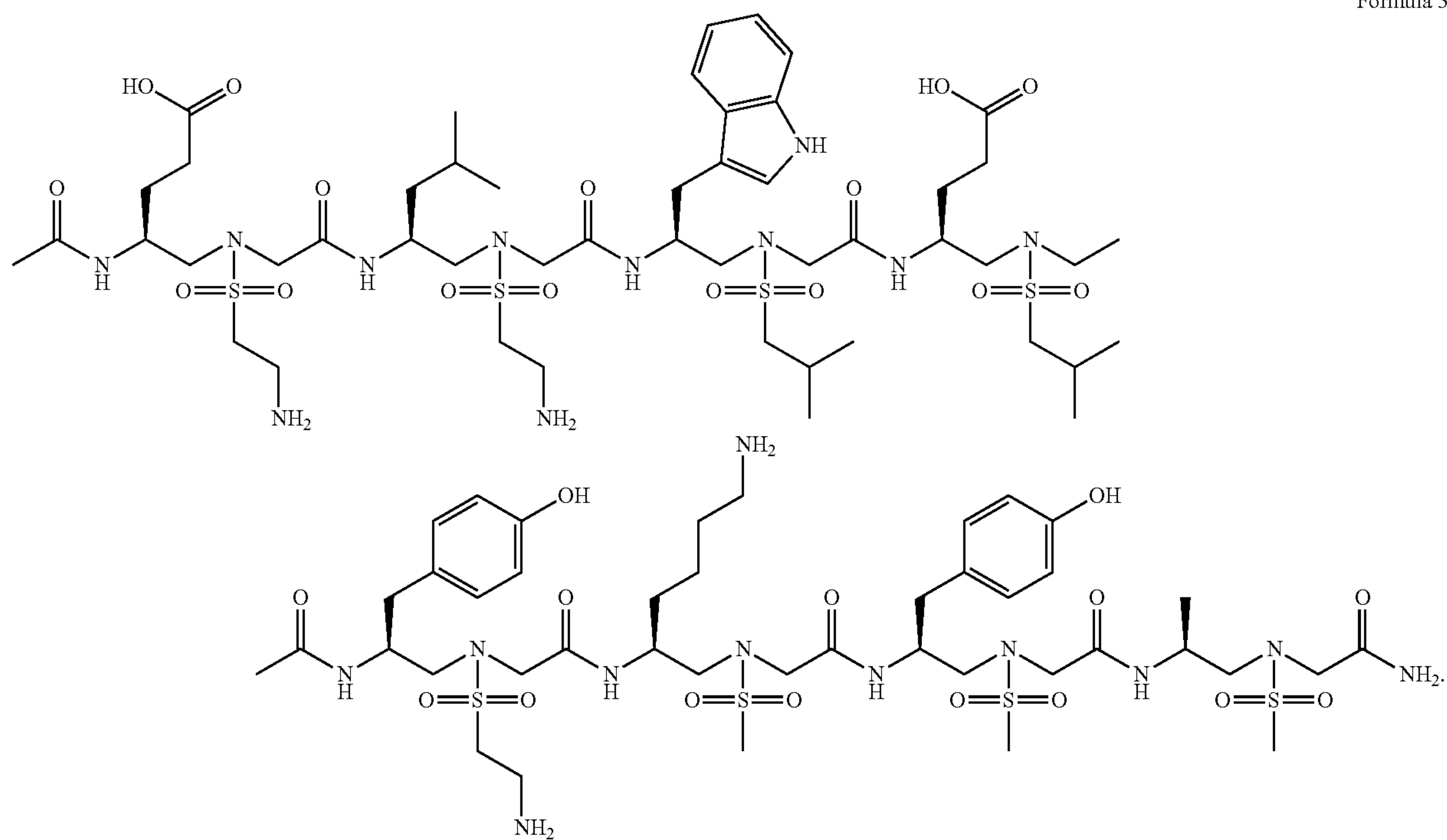
Formula 3
