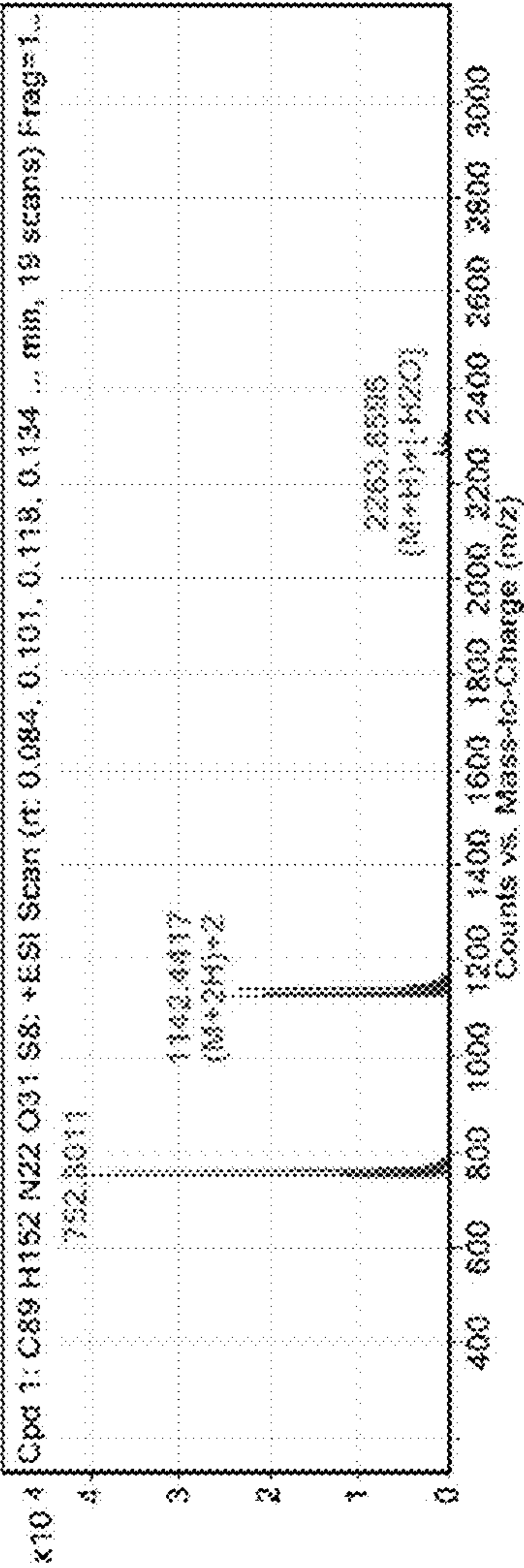
MS Spectrum
