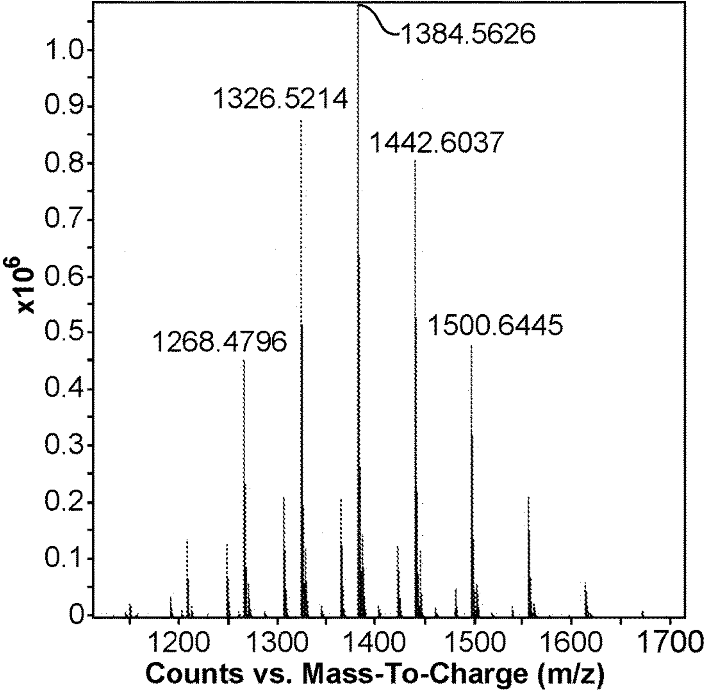
Mass Spectrum (38.72-51.30 ms)(1.557 min) - 2OH-Pr-bCD_Kleptose_Single frame_POS_001_condensed[1].d
