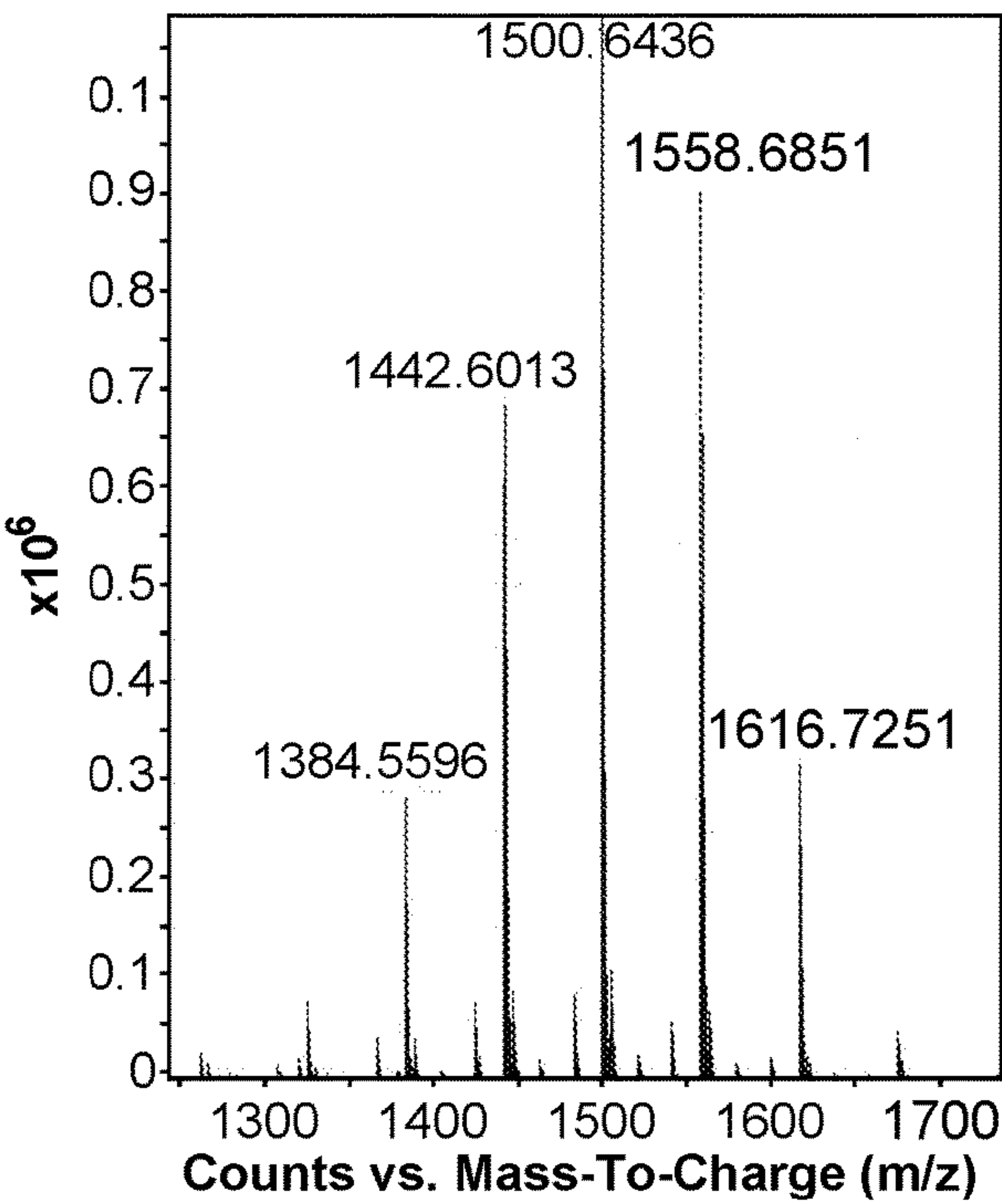
Mass Spectrum (39.21-50.97 ms)(1.557 min) - 2OH-Pr-bCD_Trappsol_Single frame_POS_001_condensed[1].d
