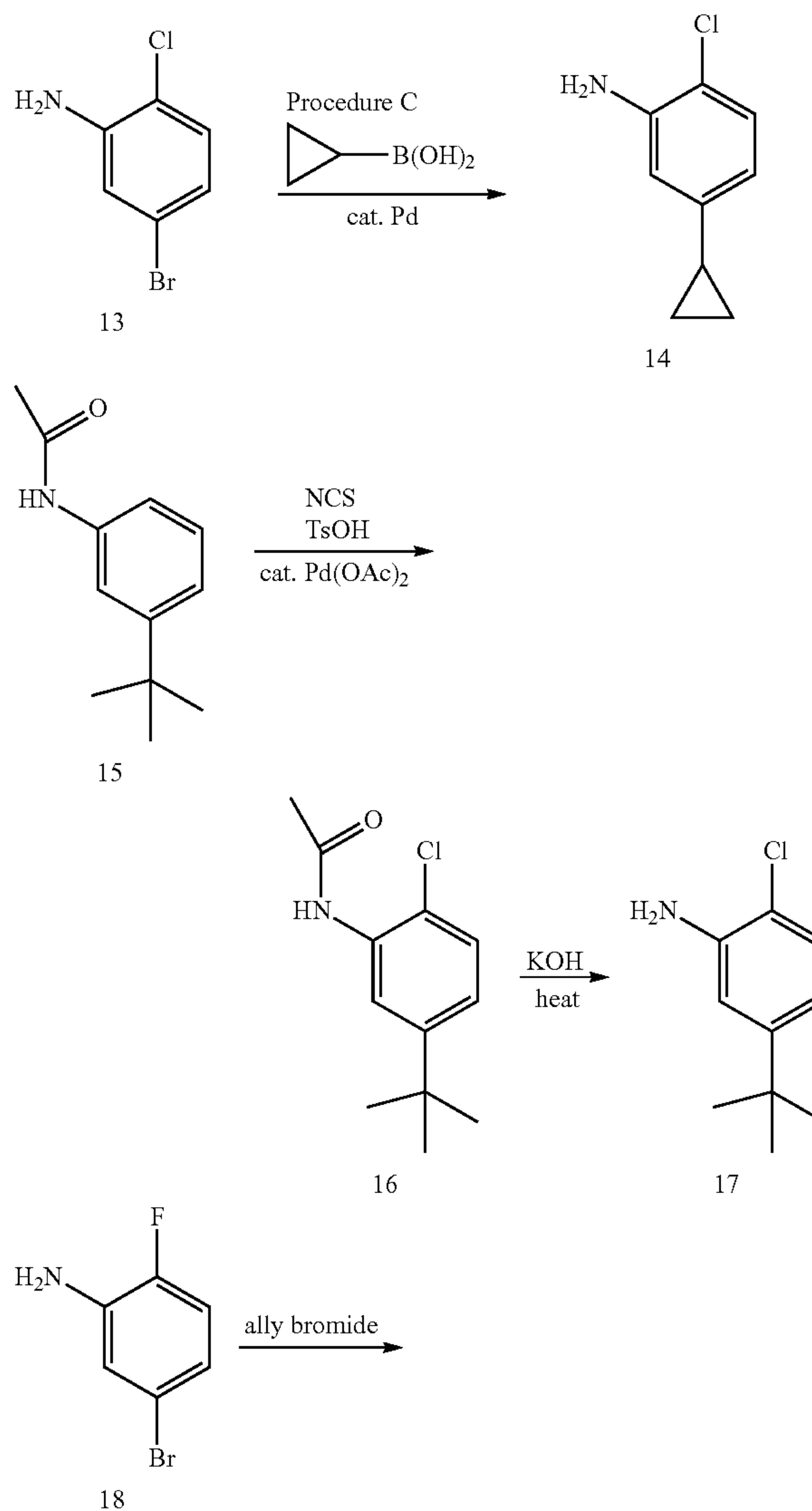
Scheme 2
