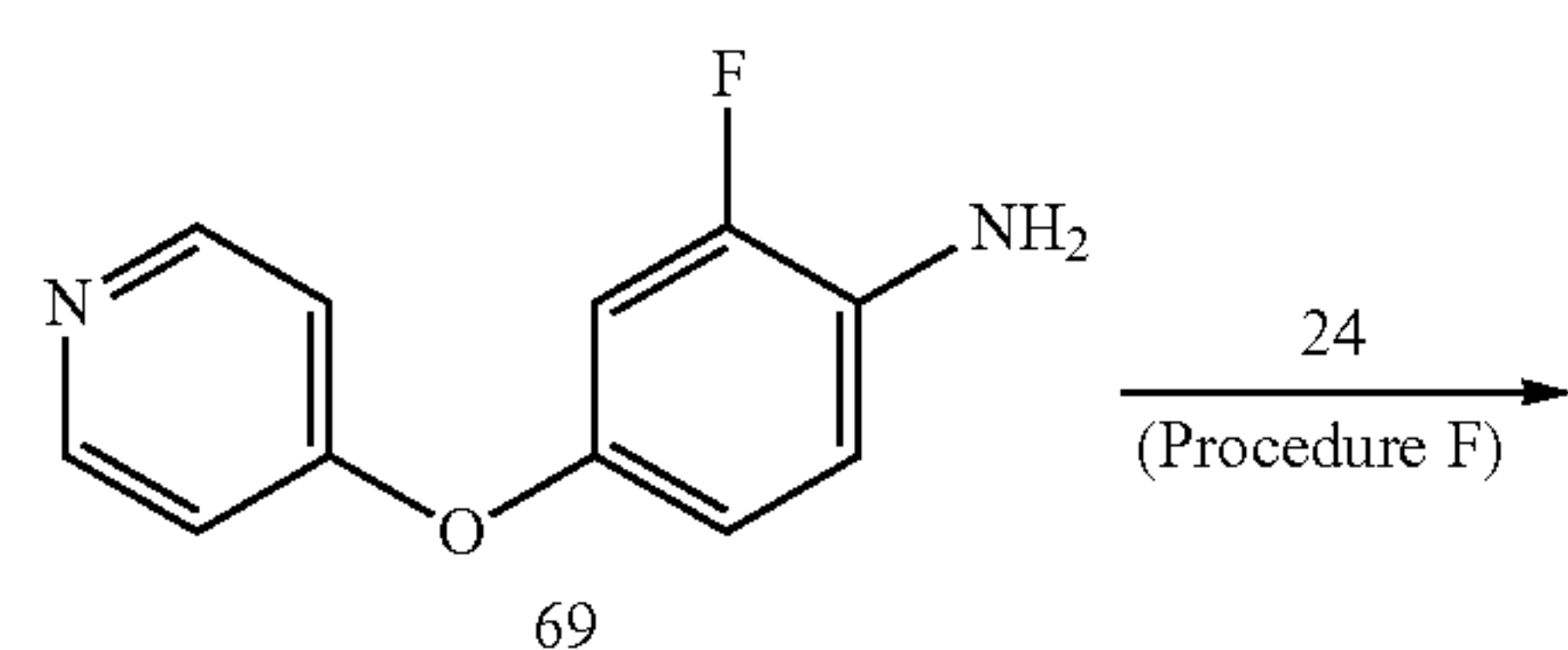
Scheme 11. Synthesis of Formula III Compounds
