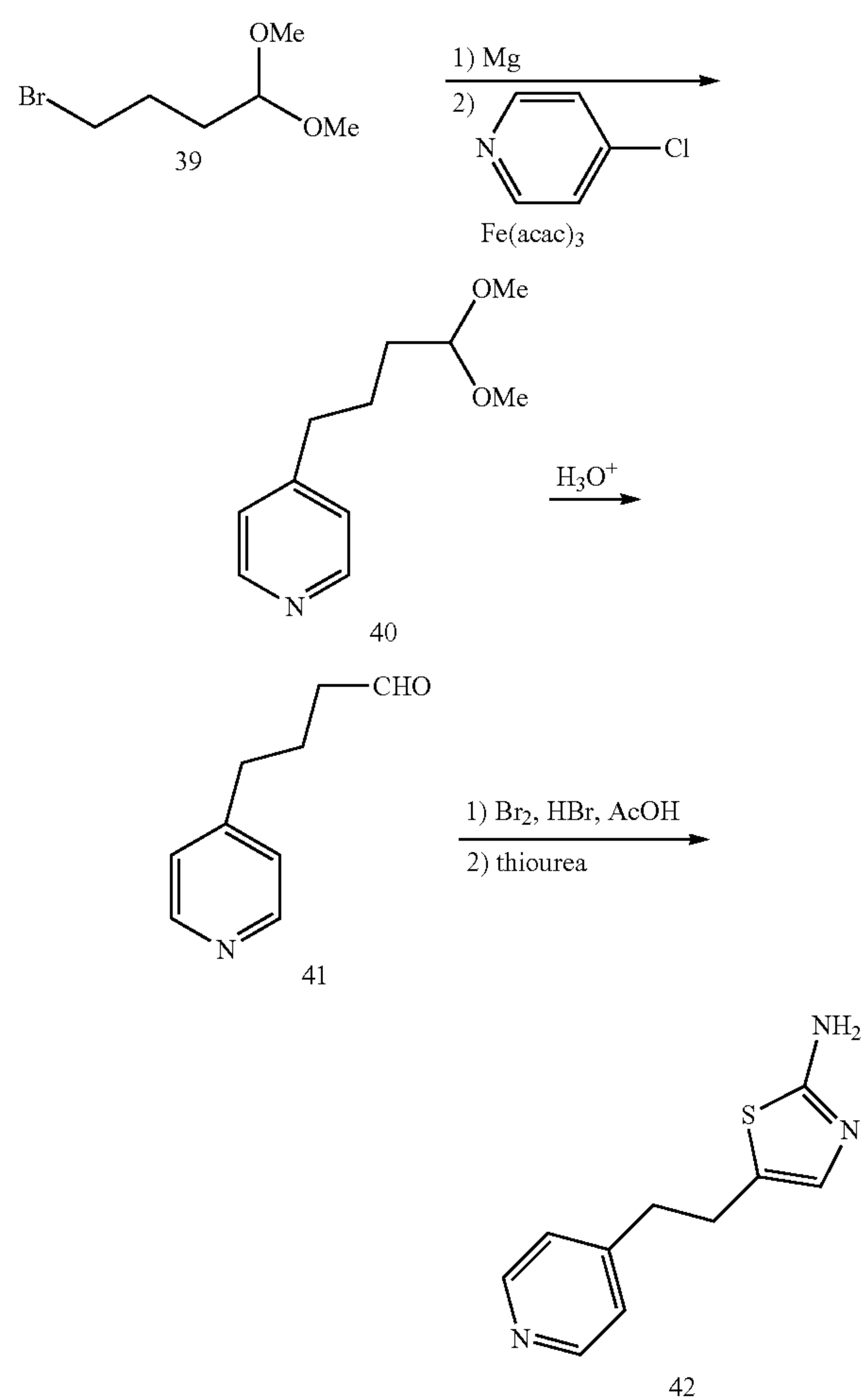
Scheme 4
