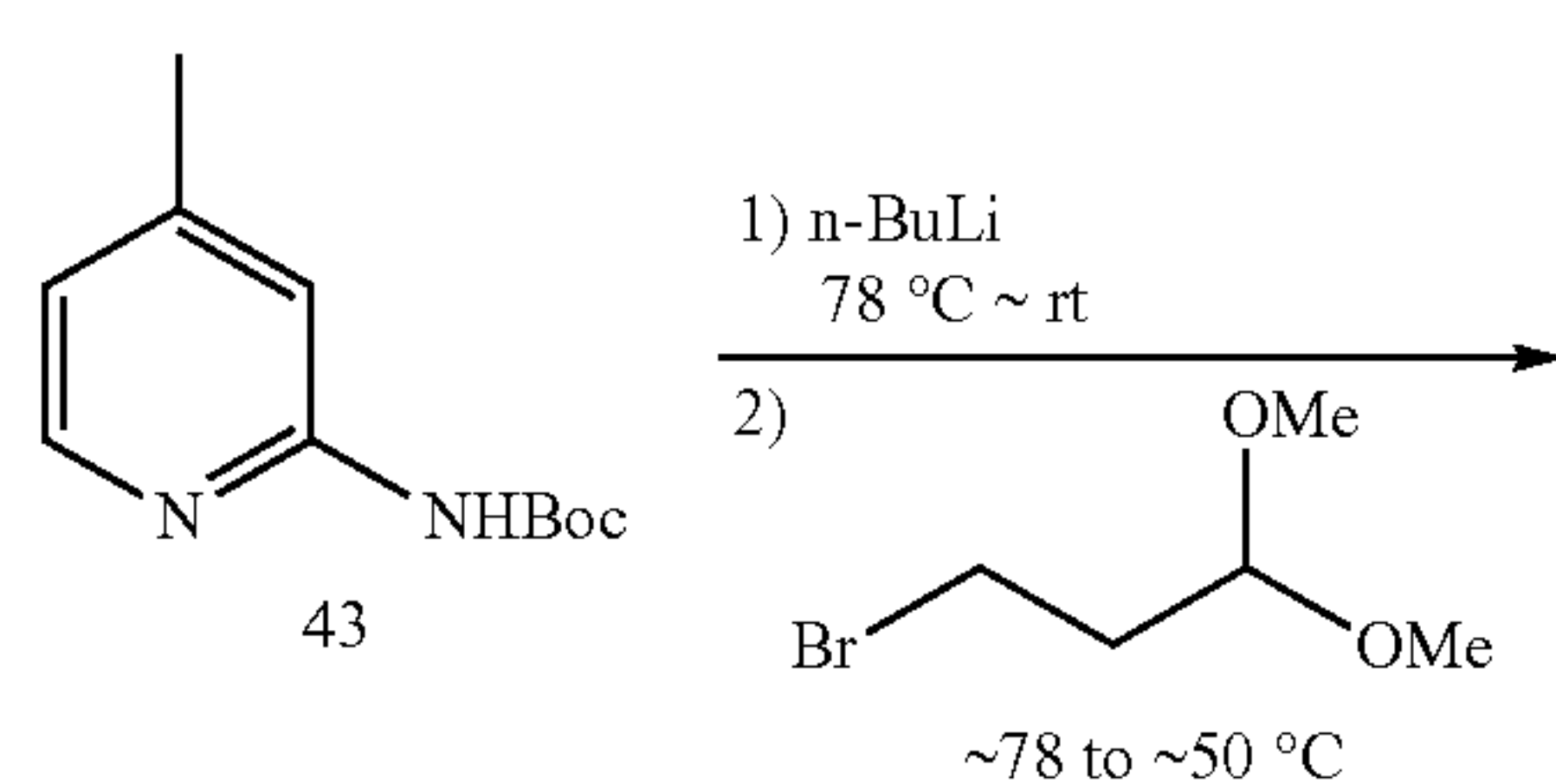
Scheme 5
