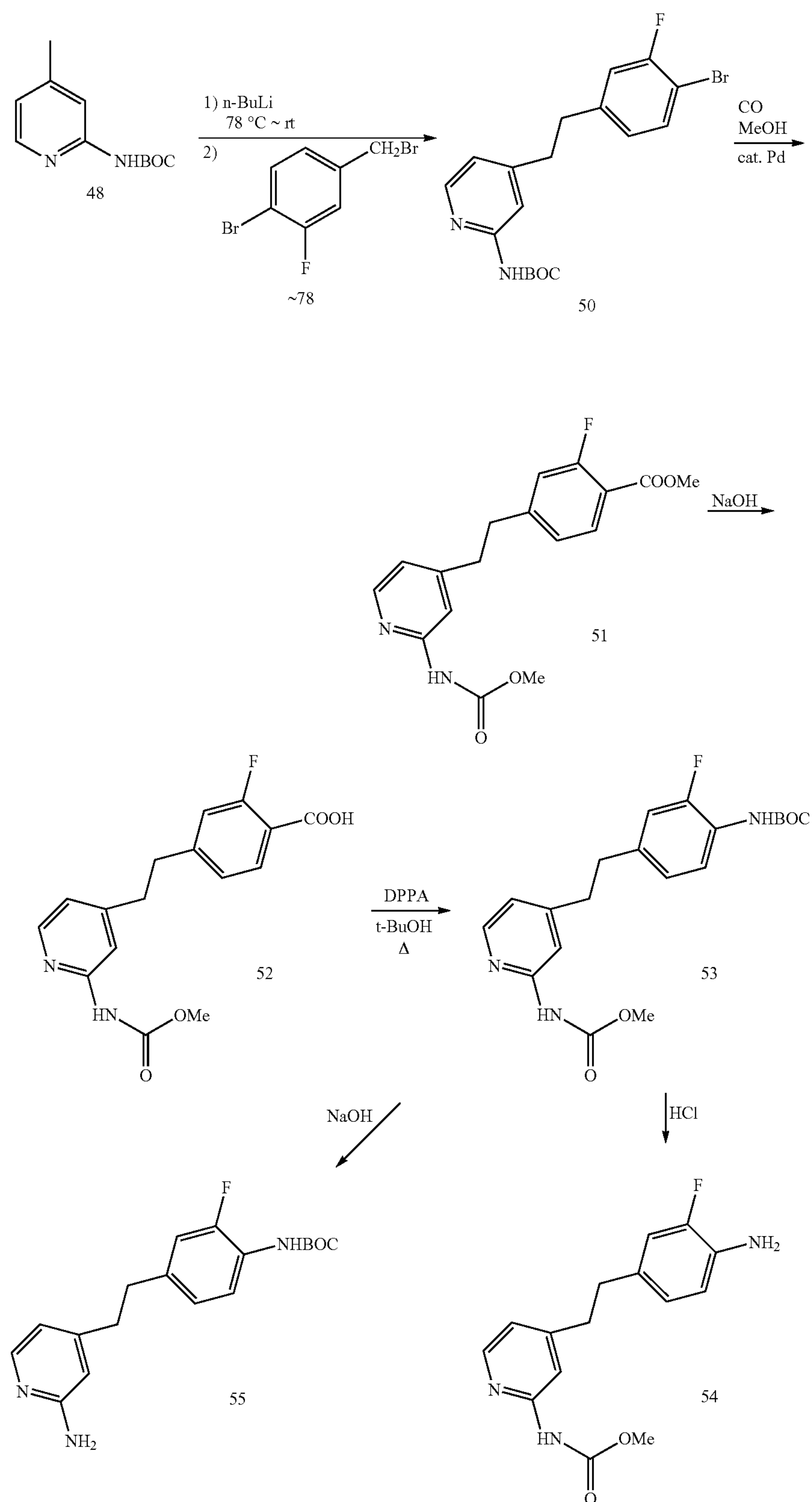
Scheme 6
