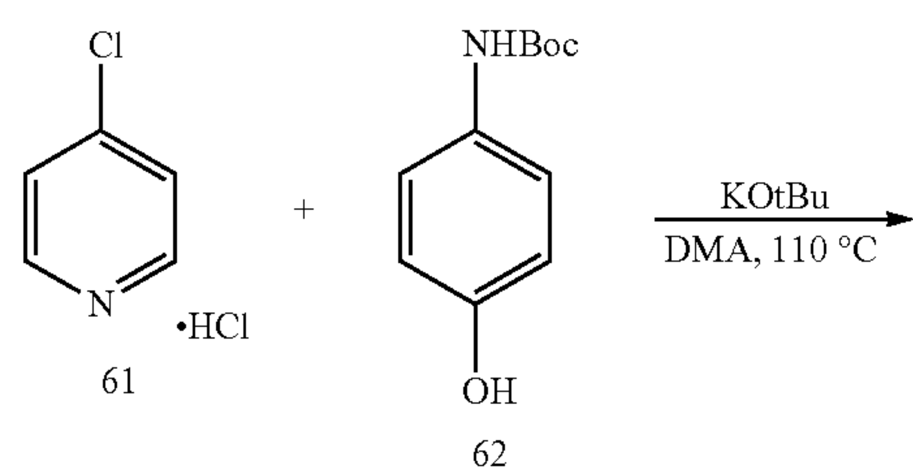
Scheme 8
