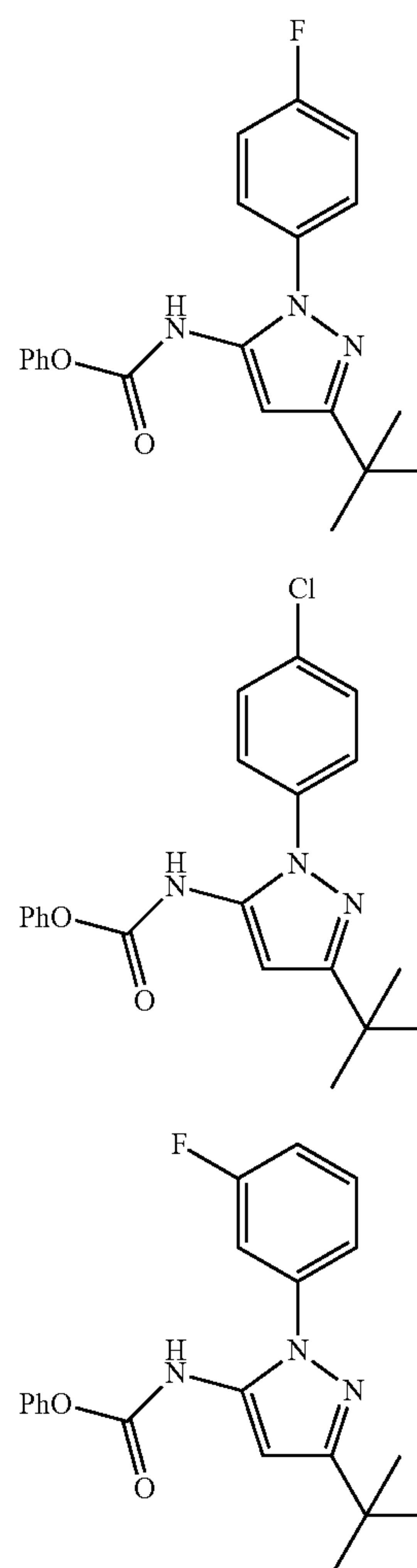
Scheme 3
