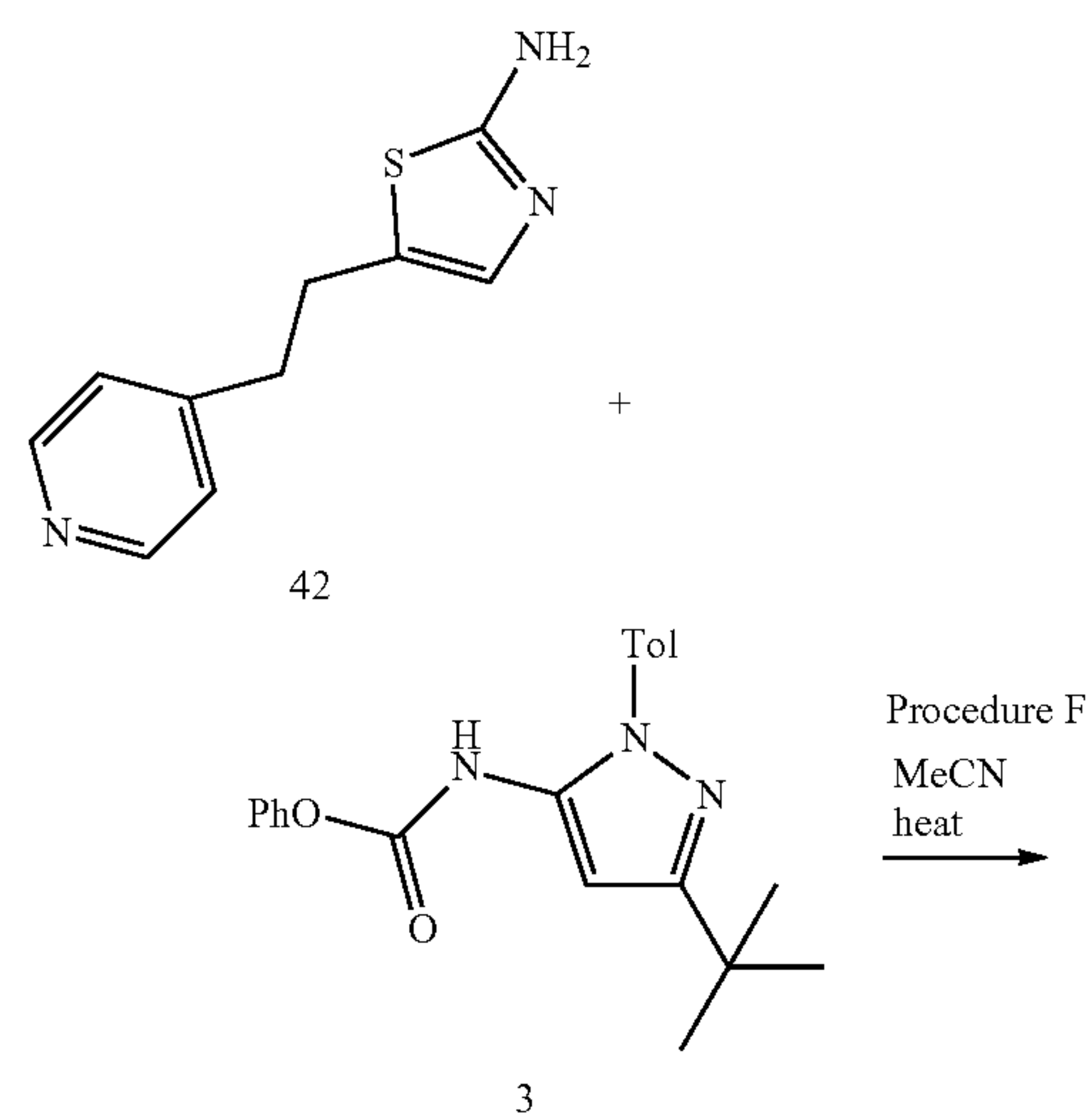
Scheme 9: Synthesis of Formula I Compounds
