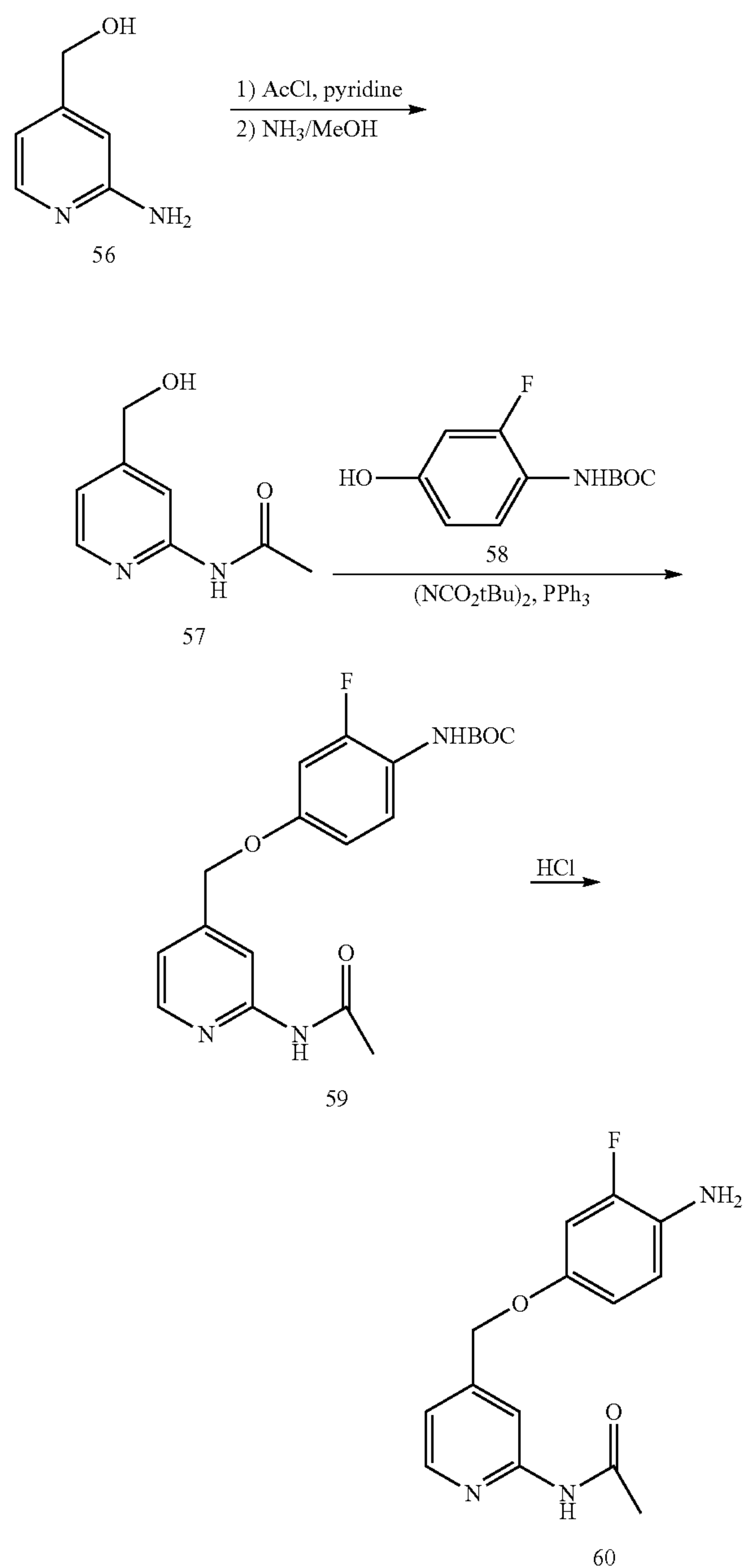
Scheme 7
