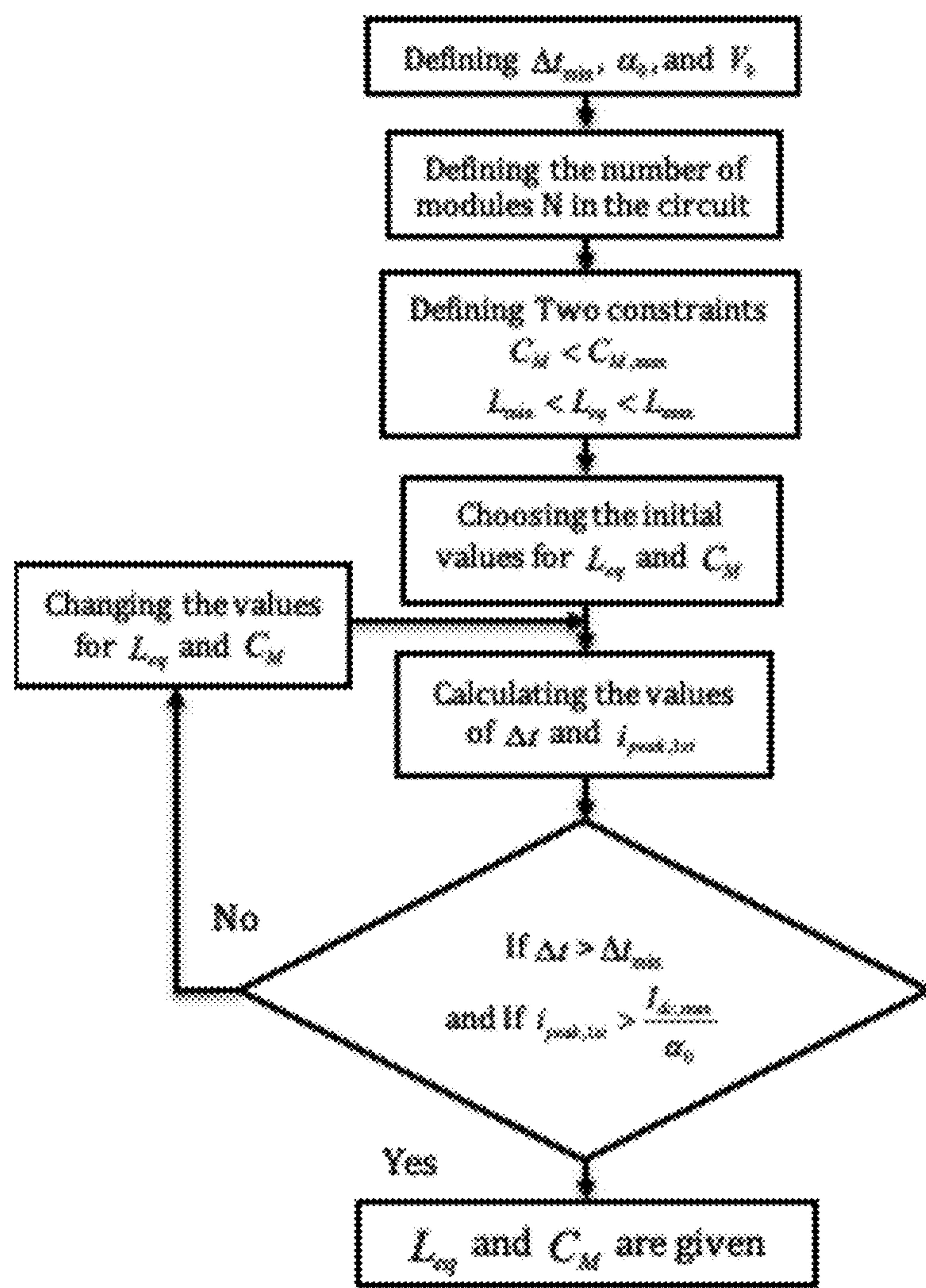
Figure 10. Proposed flowchart for determining L_{cq} and C_{st}
