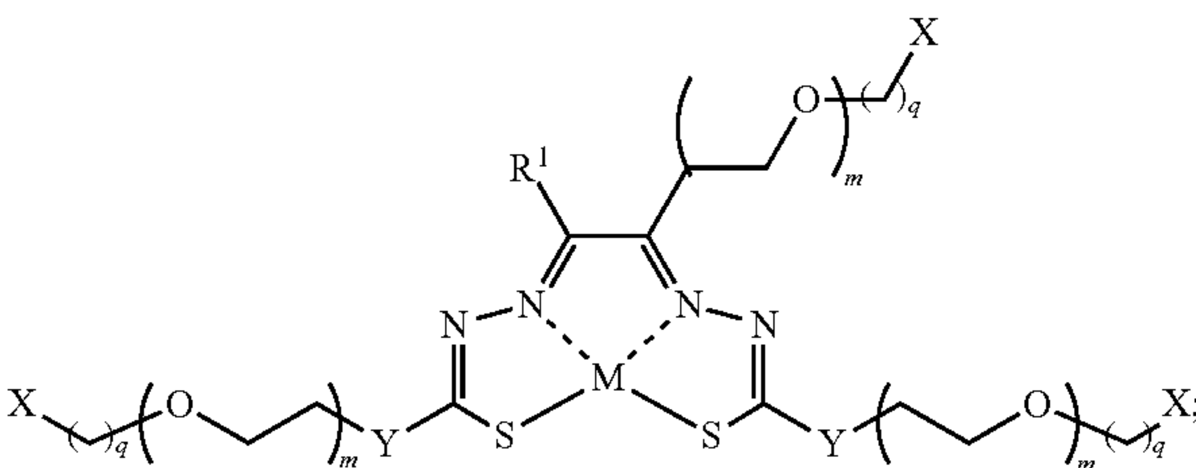
Formula IIIU
