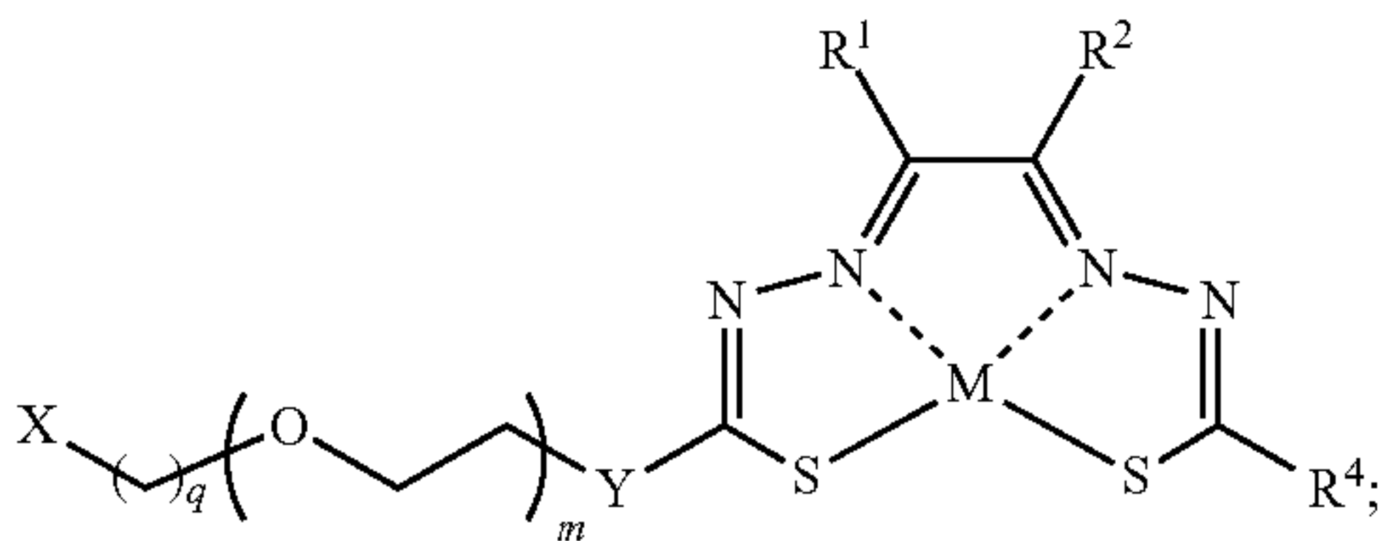
Formula IIIP
