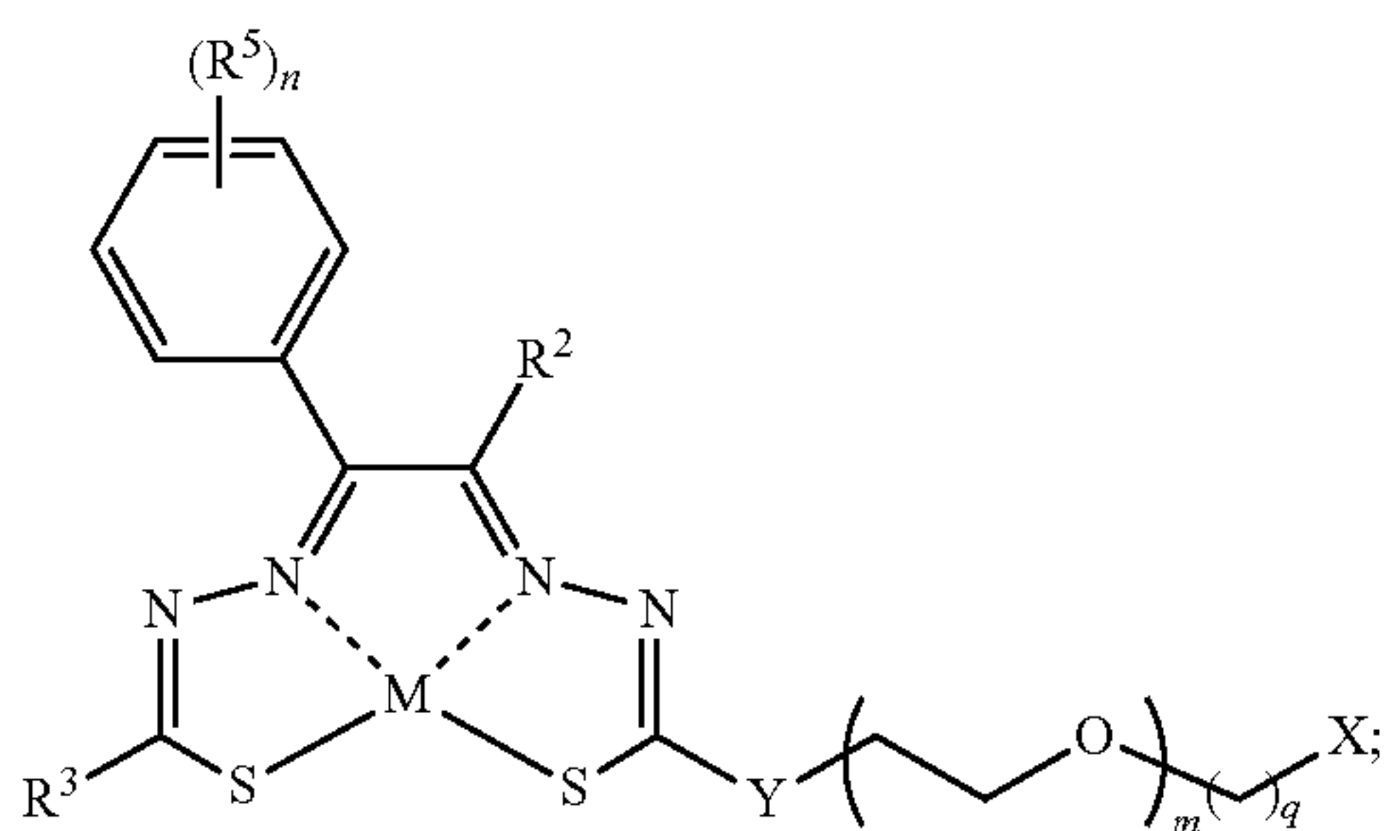
Formula IIIV'
