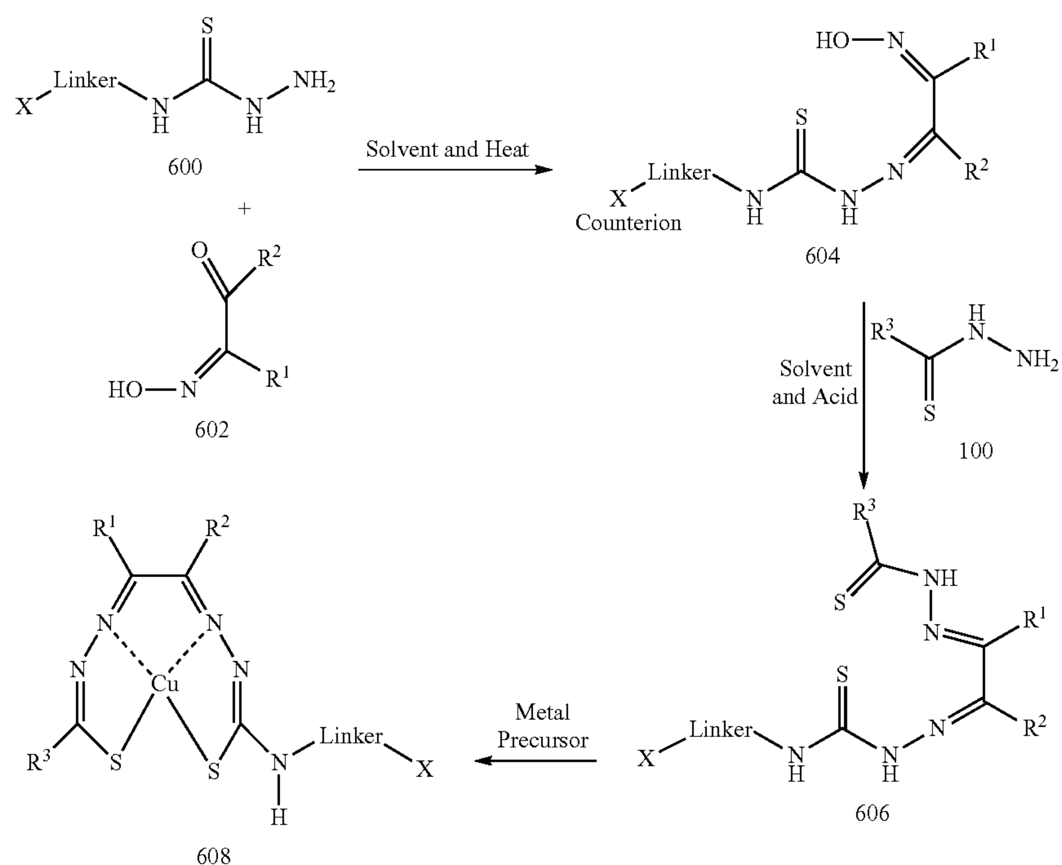
Scheme 6
