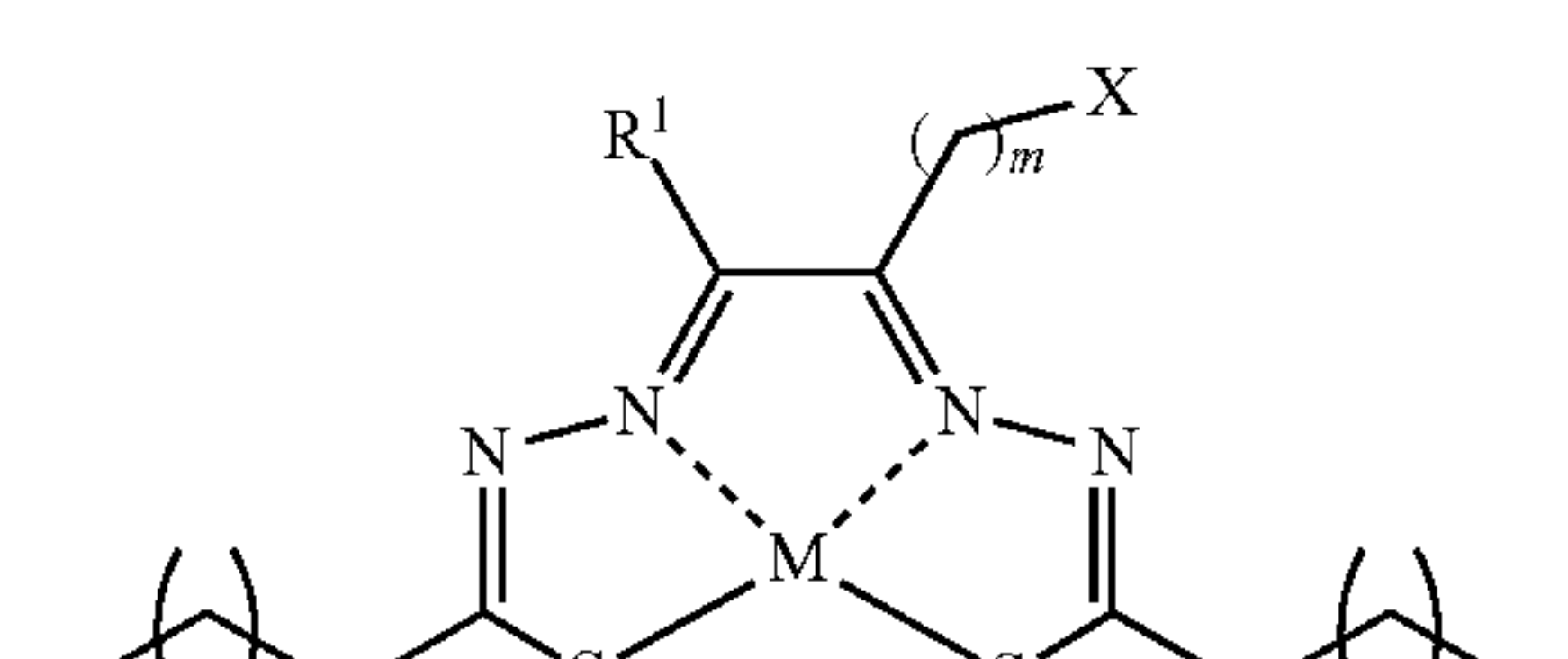
Formula IIIN
