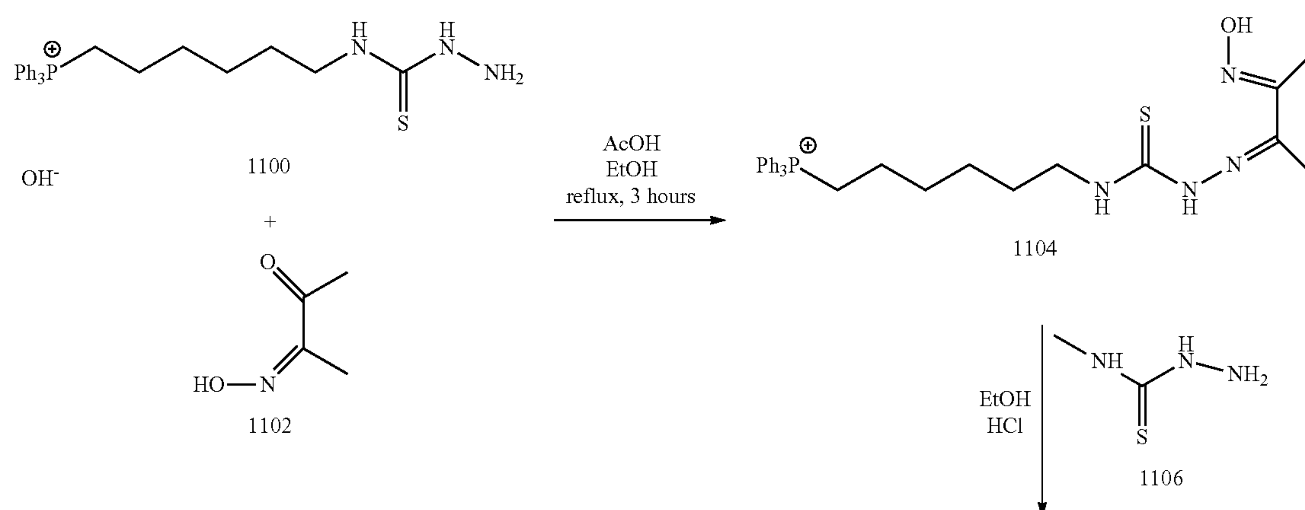
Scheme 11
