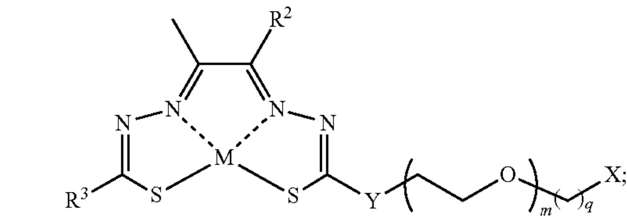
Formula IIIO'
