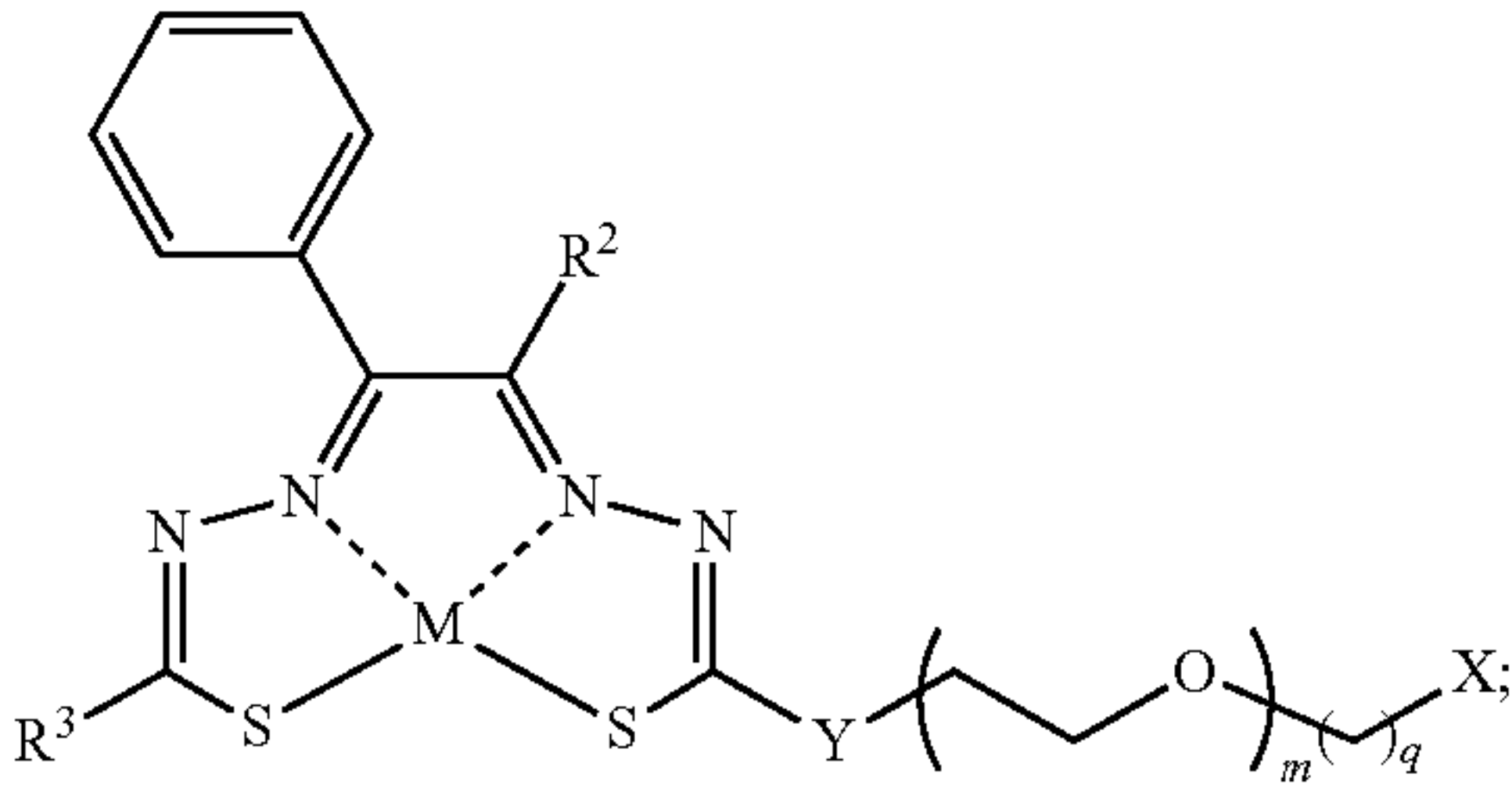
Formula IIIL'
