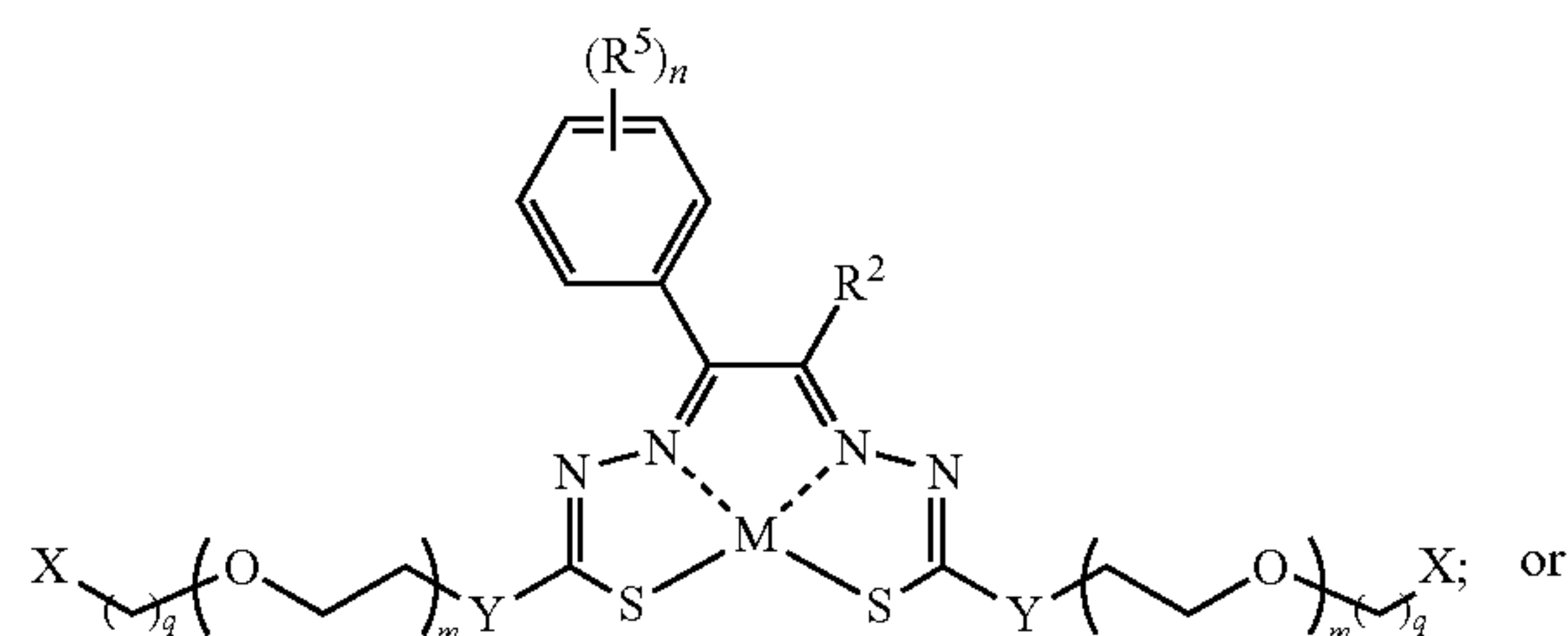
Formula IIIX'
