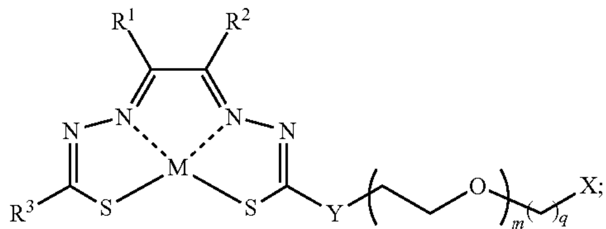
Formula IIIS
