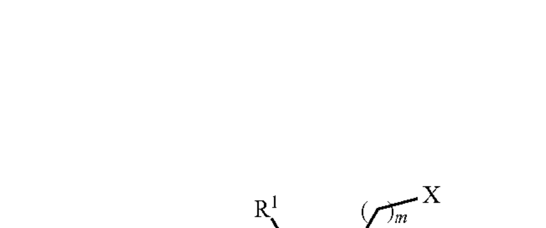
Formula IIIO
