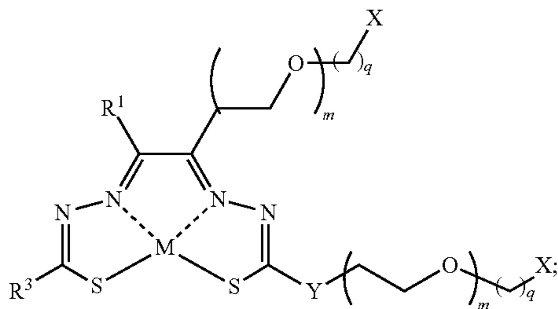
Formula IIIU
