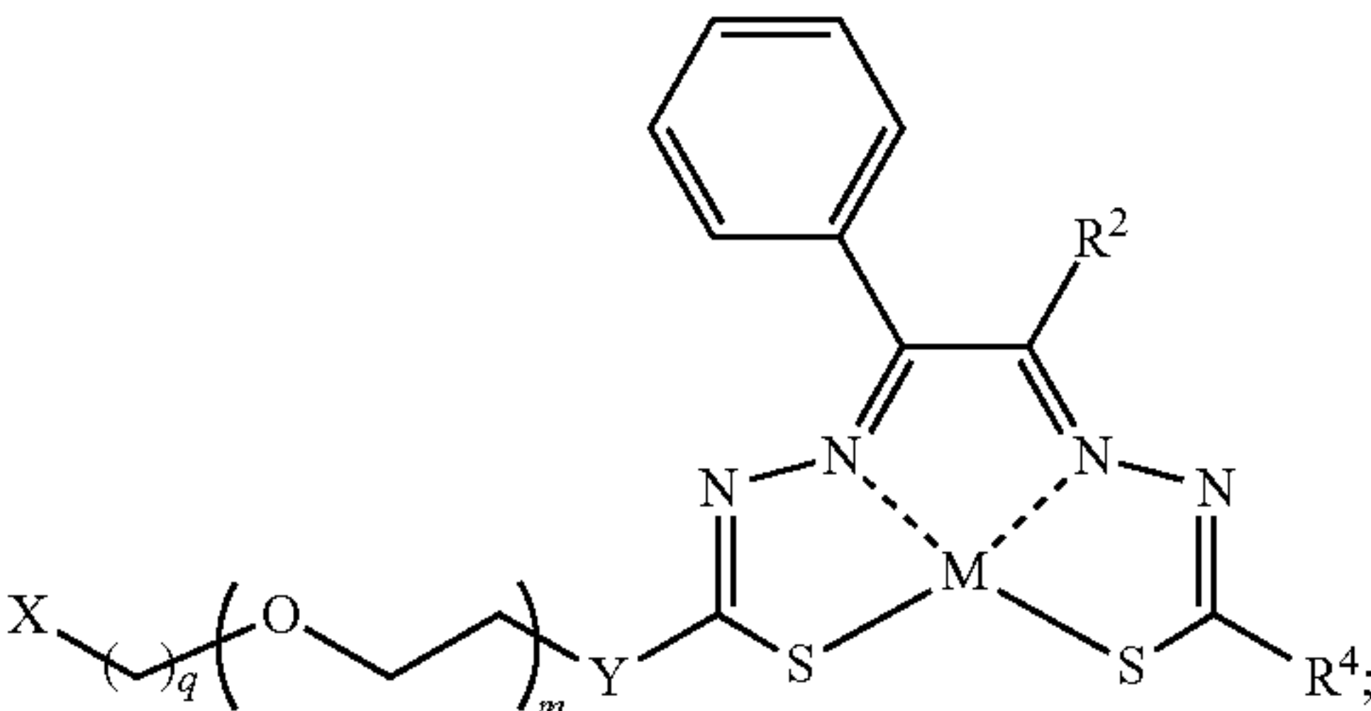
Formula IIIO'
