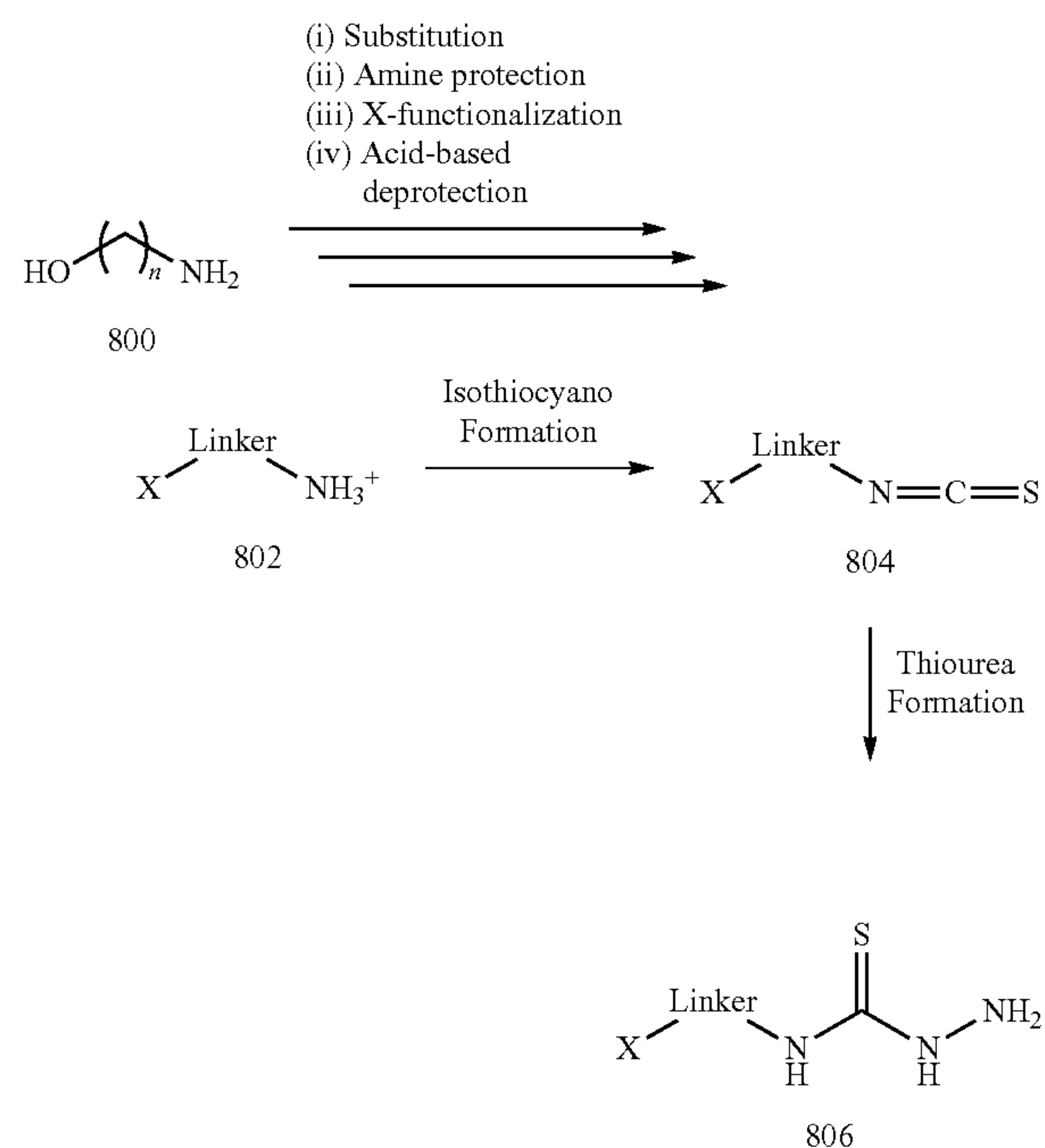
Scheme 8
