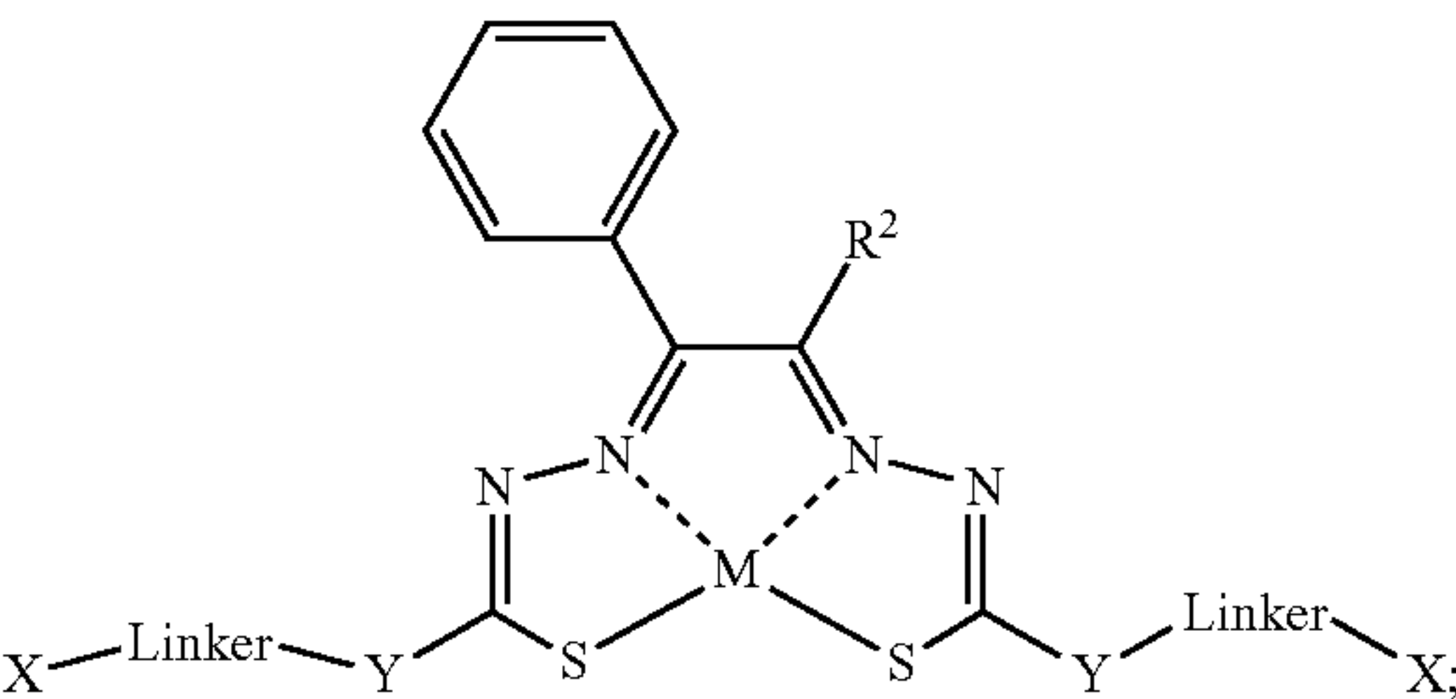
Formula IIIA'
