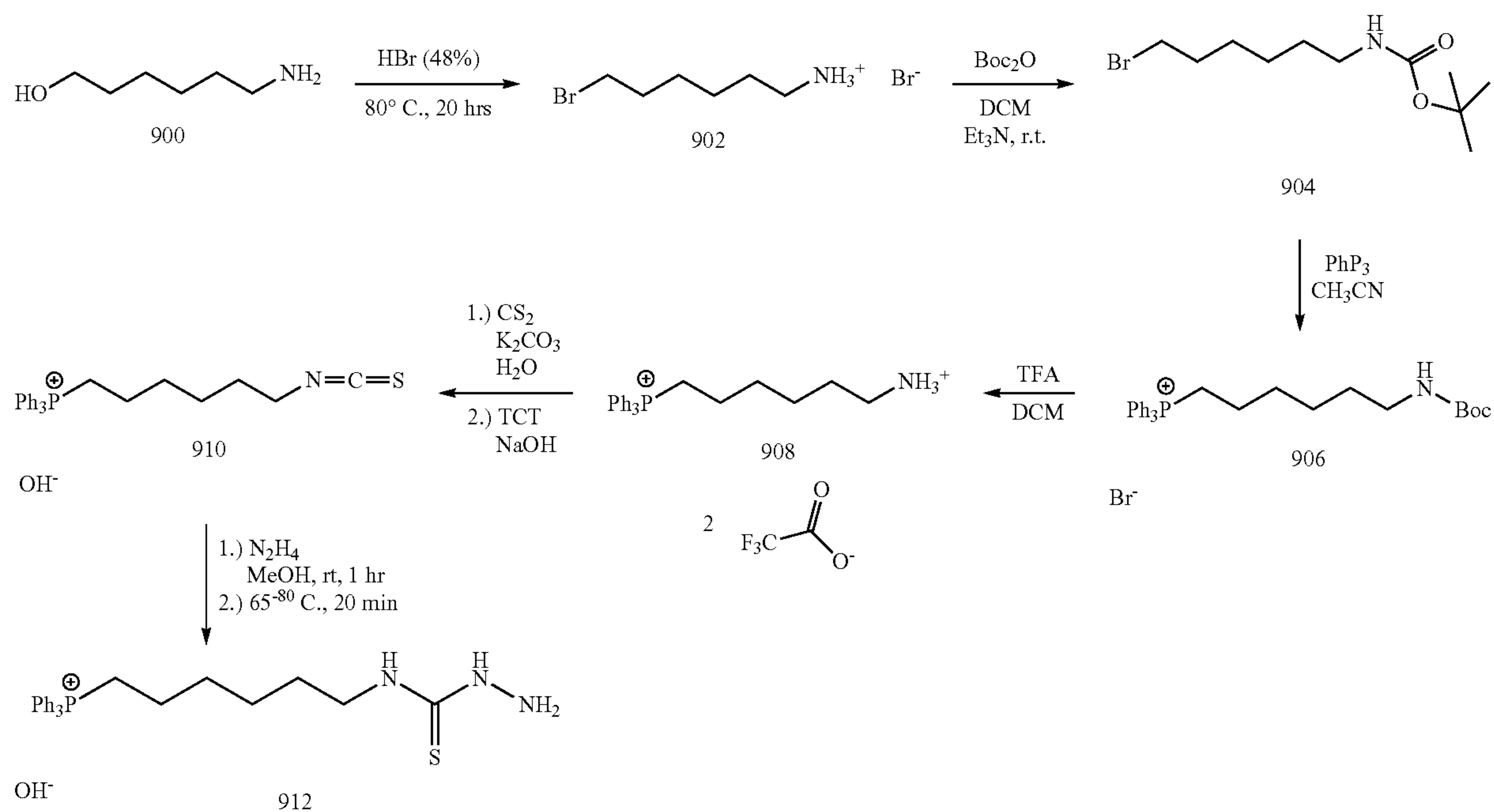
Scheme 9
