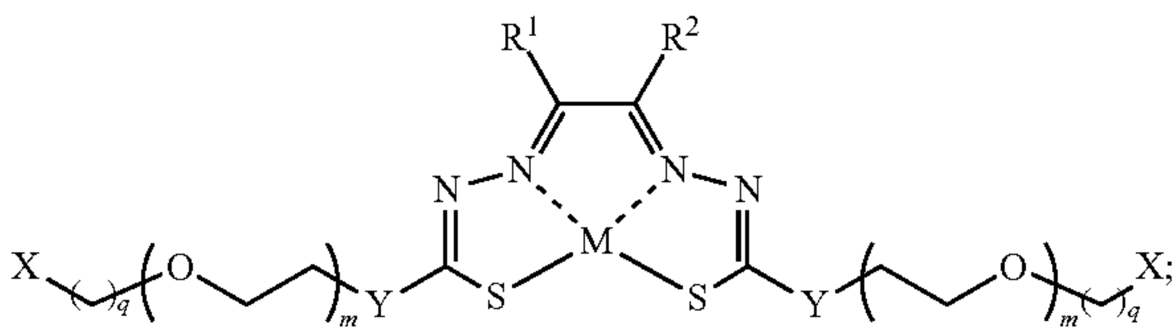
Formula IIIR
