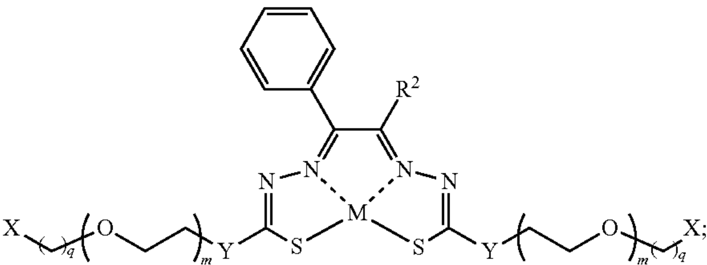
Formula IIIM'
