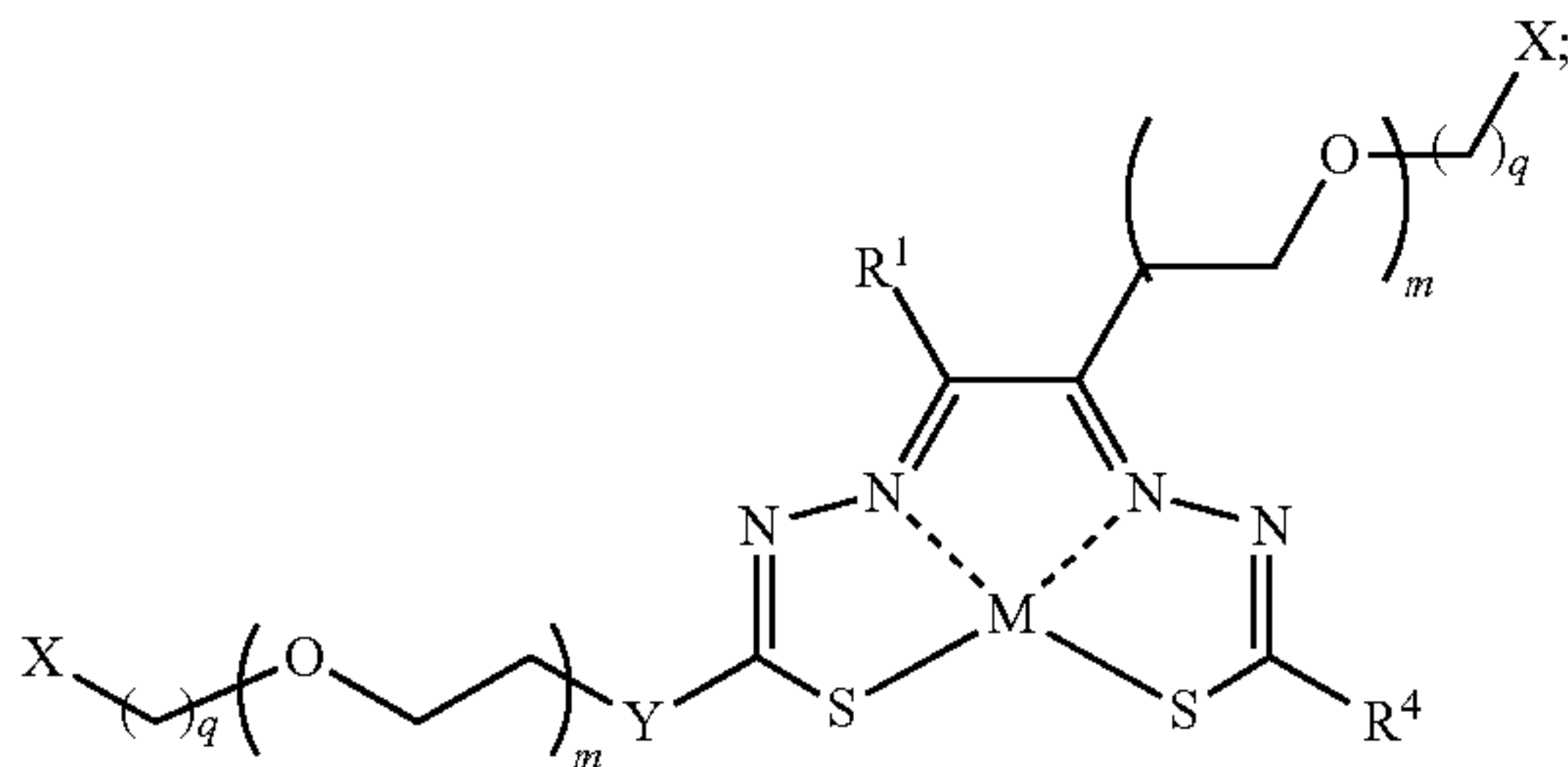
Formula IIIT
