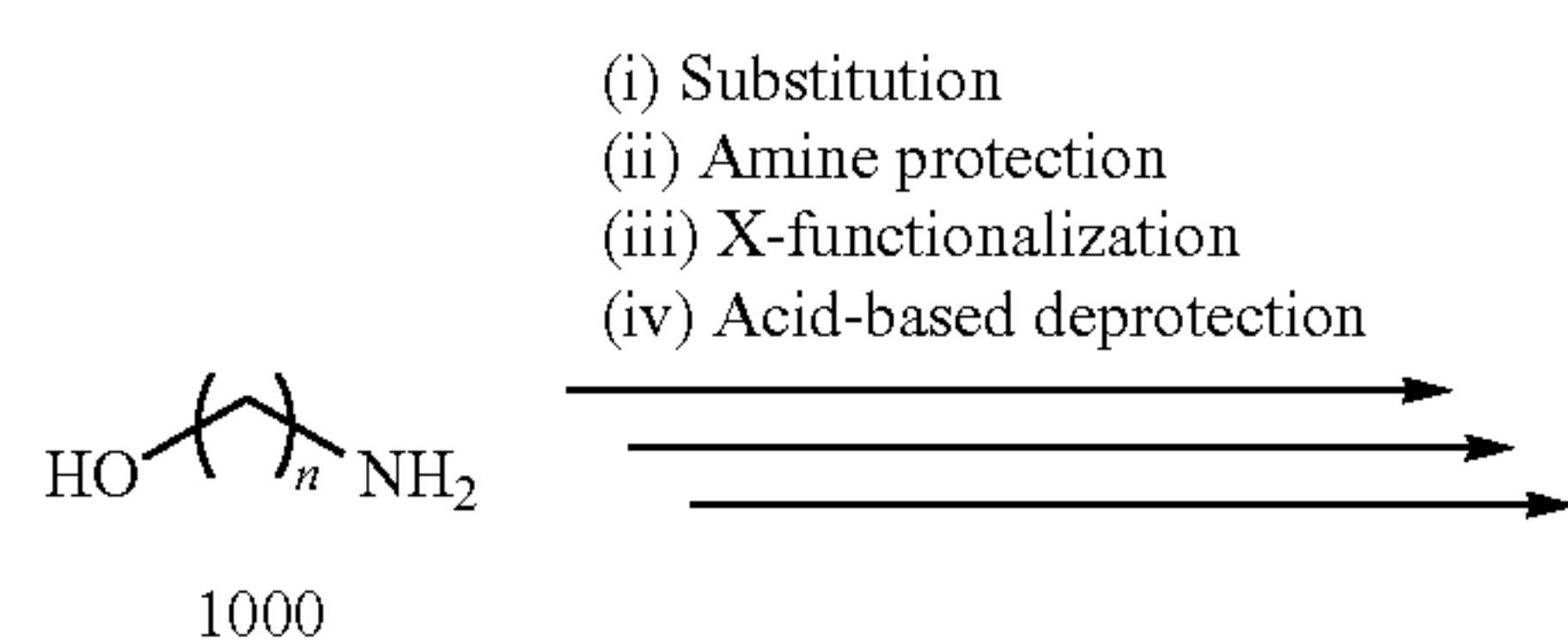
Scheme 10
