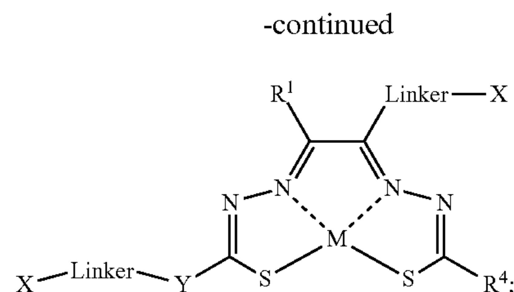
Formula IIIF
