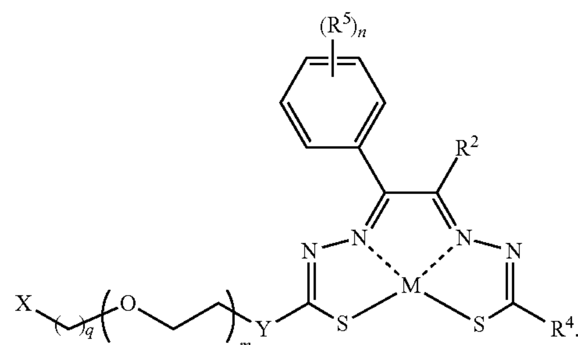
Formula IIYY'
