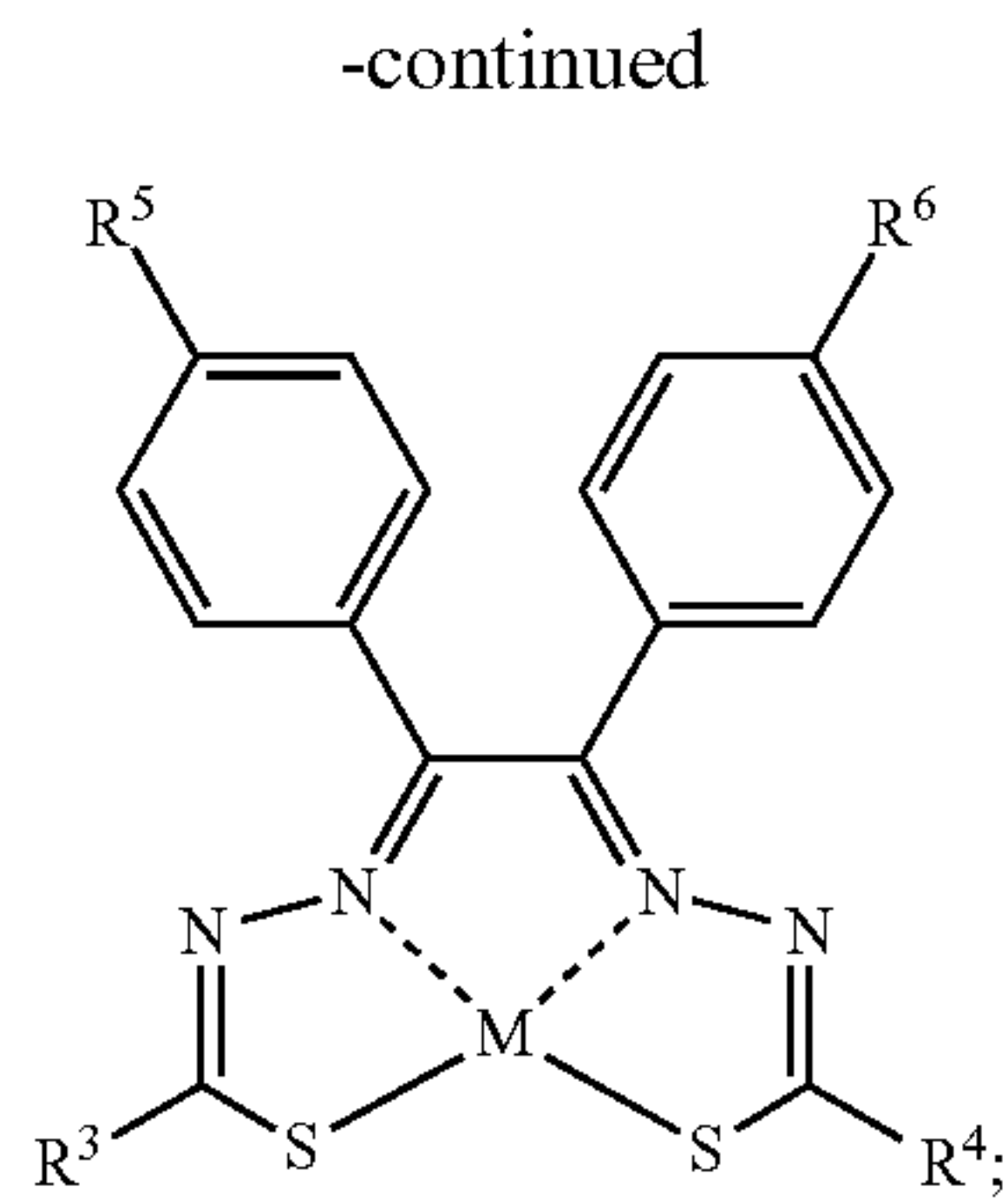
Formula IIE
