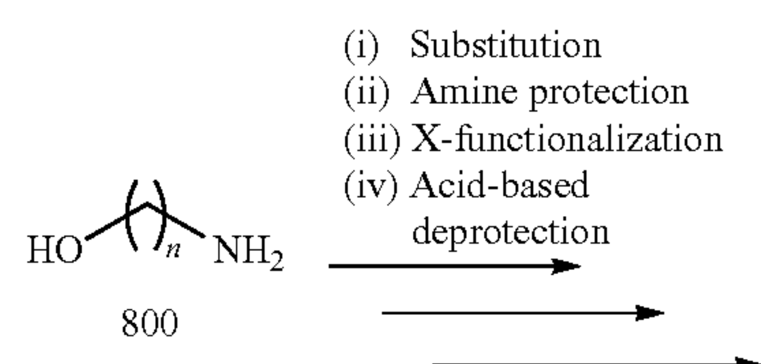
Scheme 8
