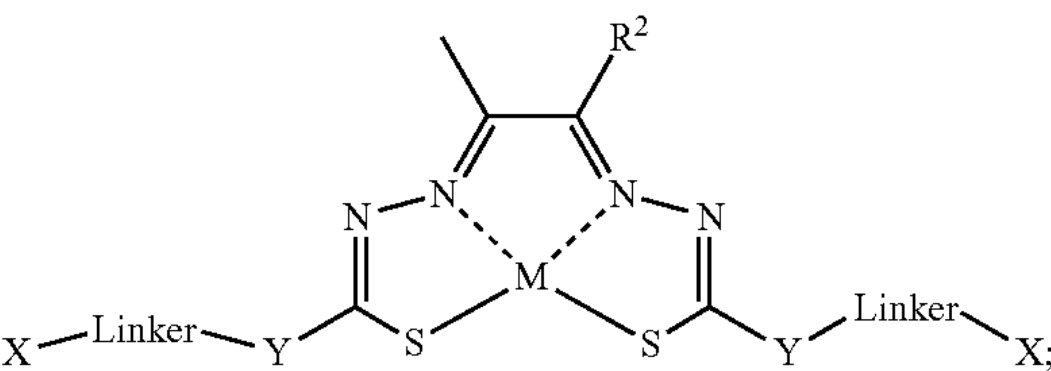
Formula IIIC'
