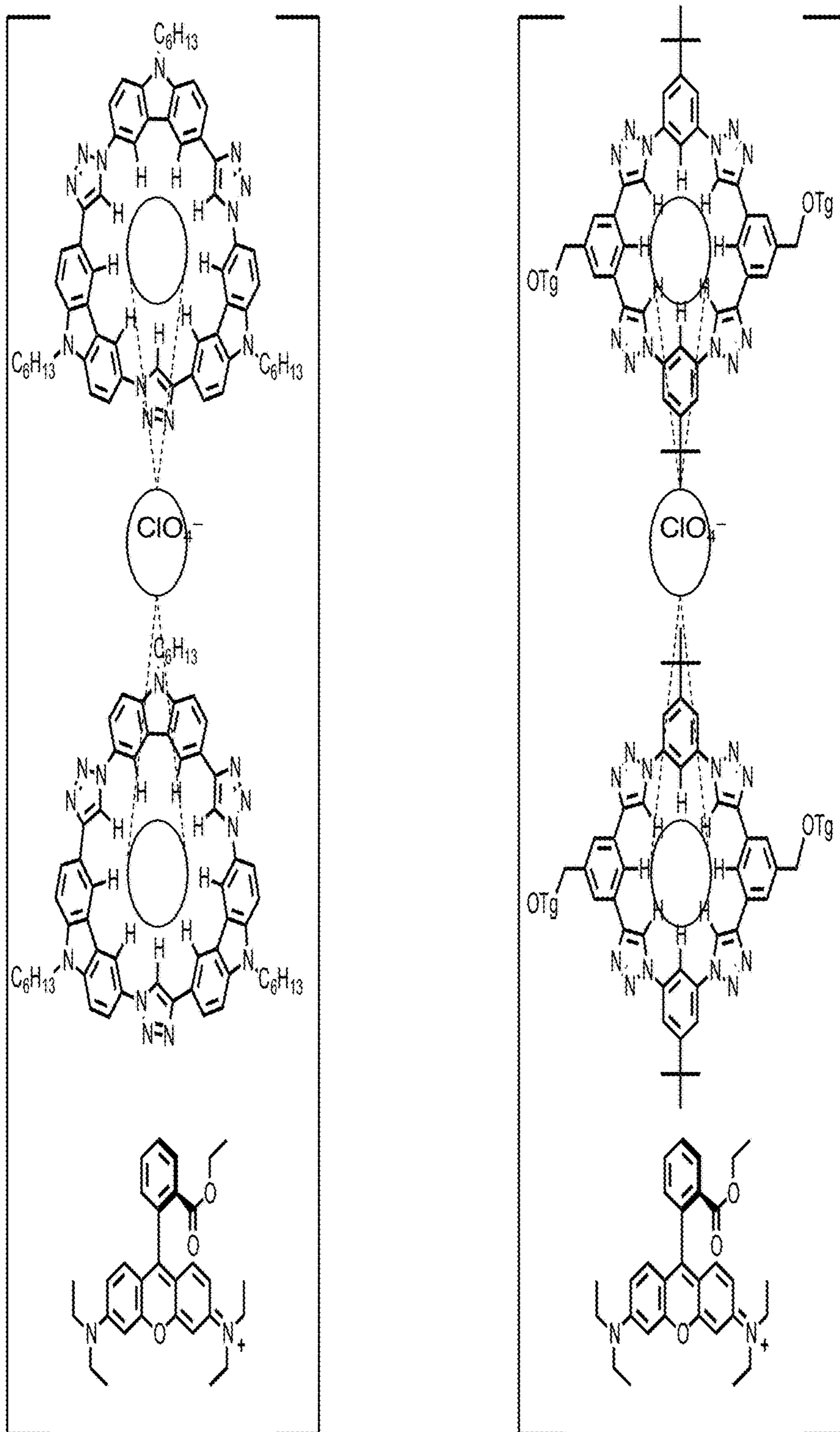
AB-SMILES (tricarbo-C6) 2 (ClO 4 ) (rhodamine 3B)
