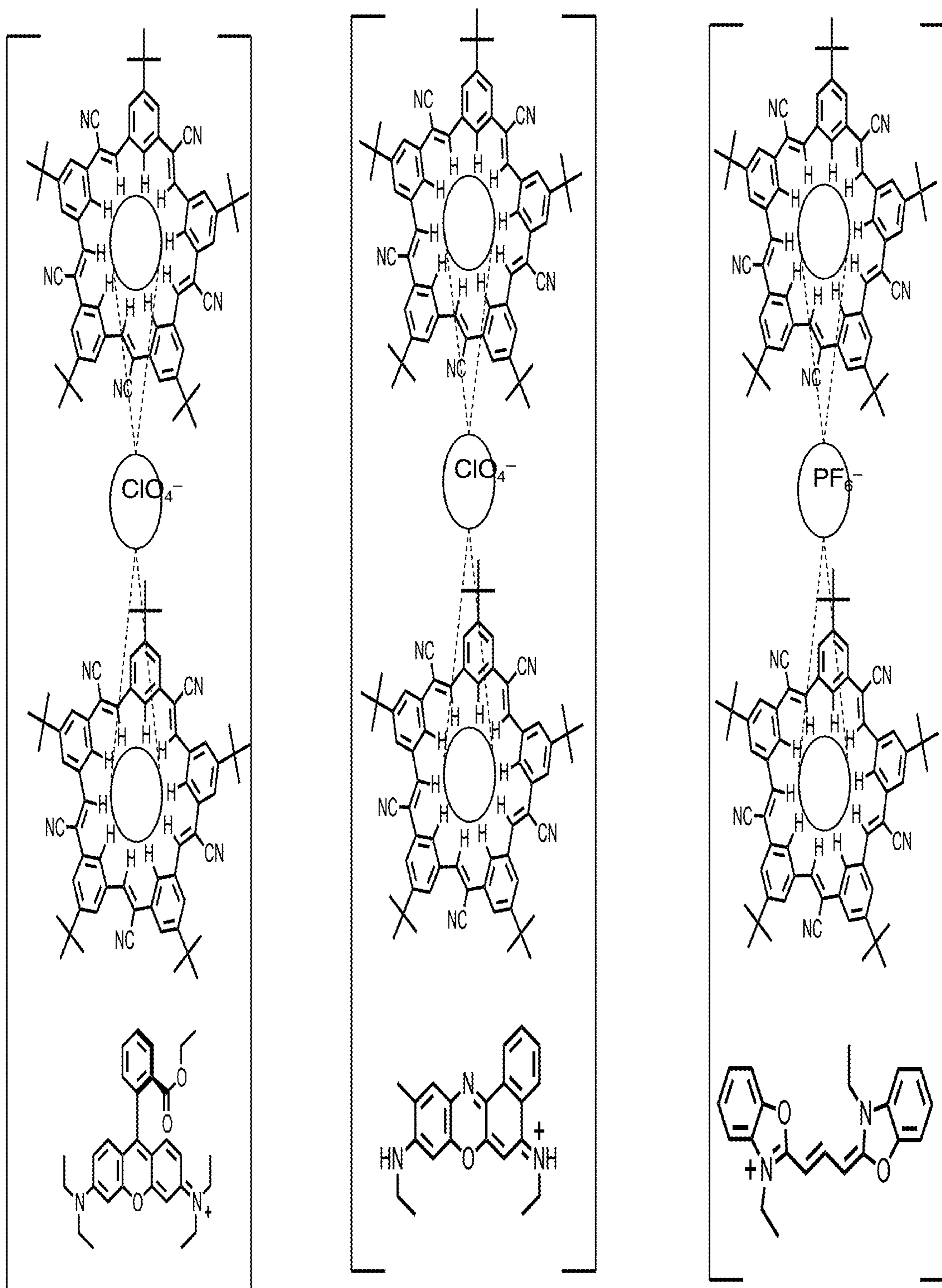
FL-SMILES (cyanostar) 2 (PF 6 ) (DIOC 2 )
