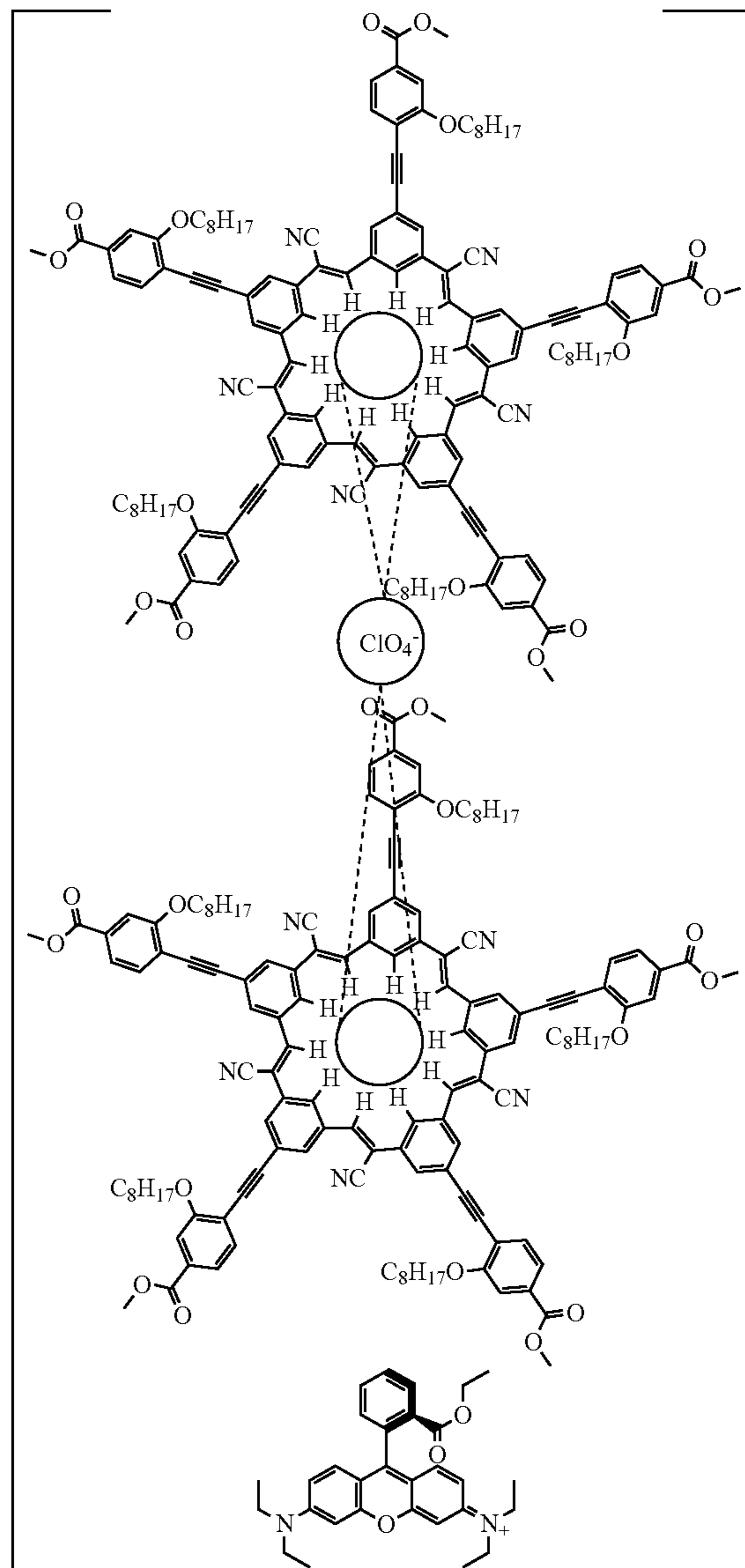
(I-12)
