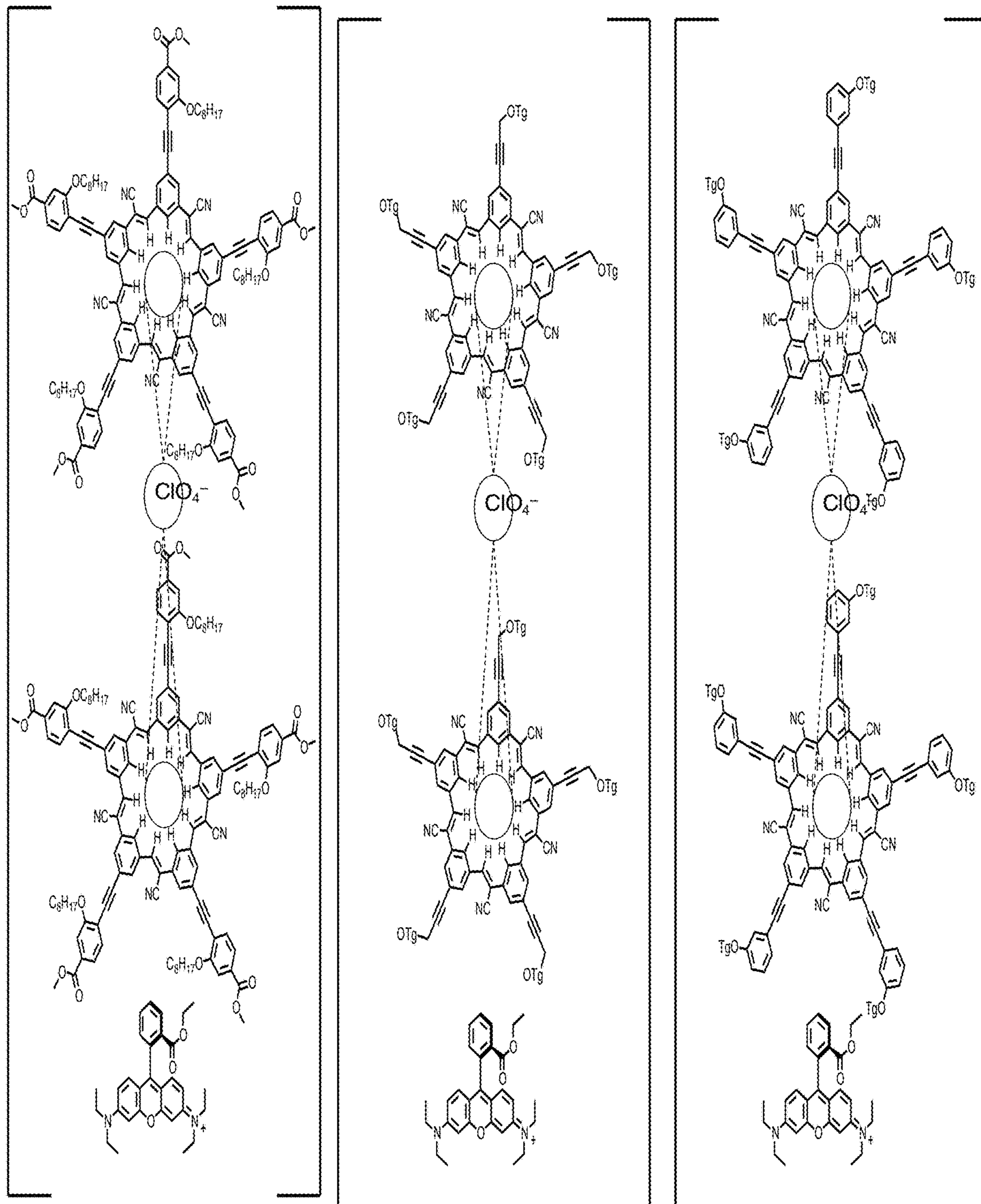
FL-SMILES (cyanostar 2) 2 (ClO 4 ) (rhodamine 3B)
