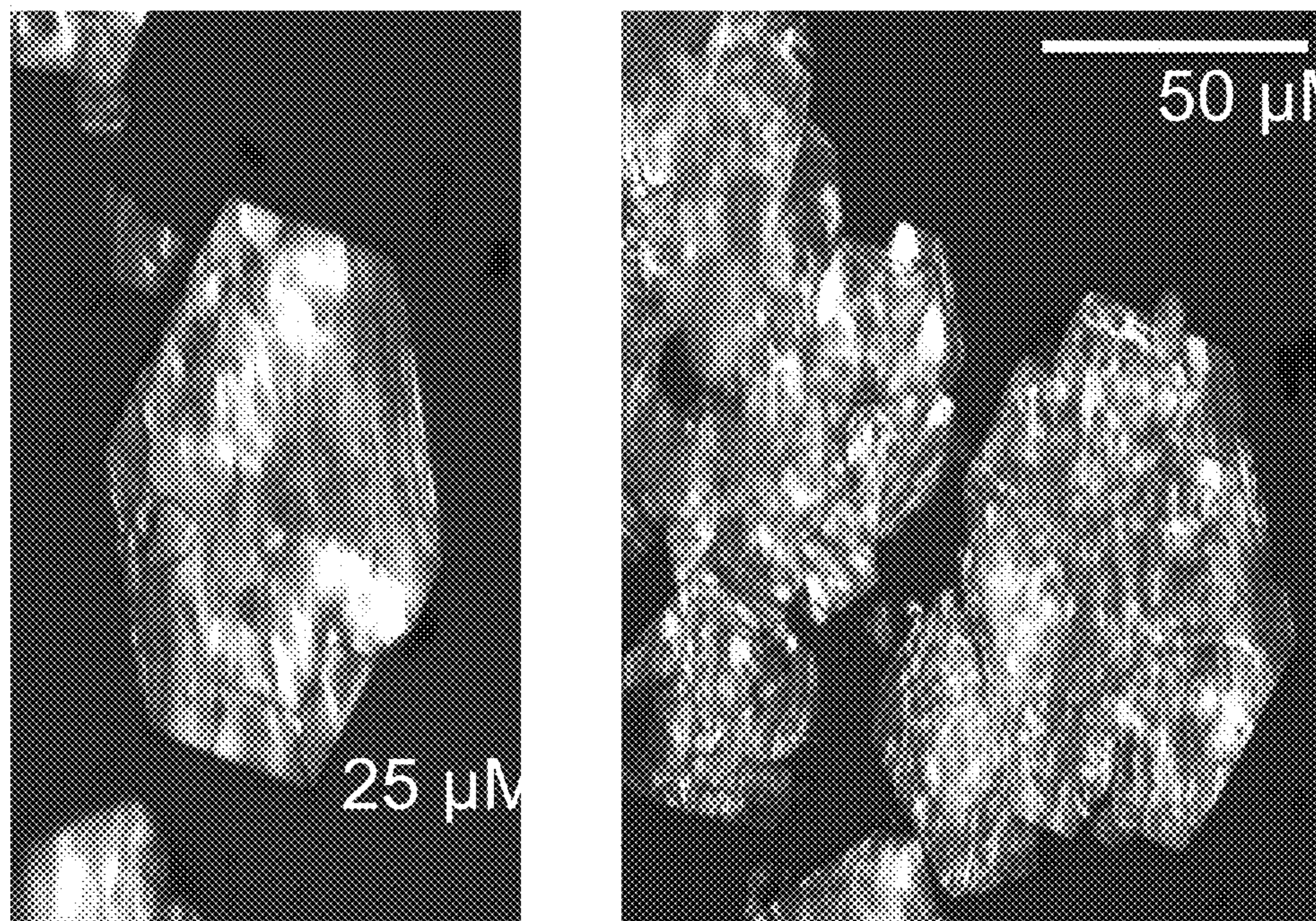
FL-SMILES (cyanostar) 2 (BF 4 ) (DAOTA)
