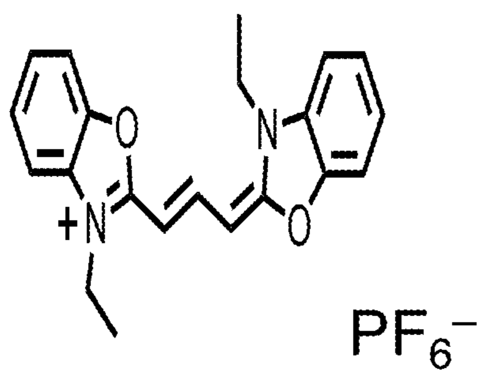
DIOC 2 ·PF 6 (Cyanine)
