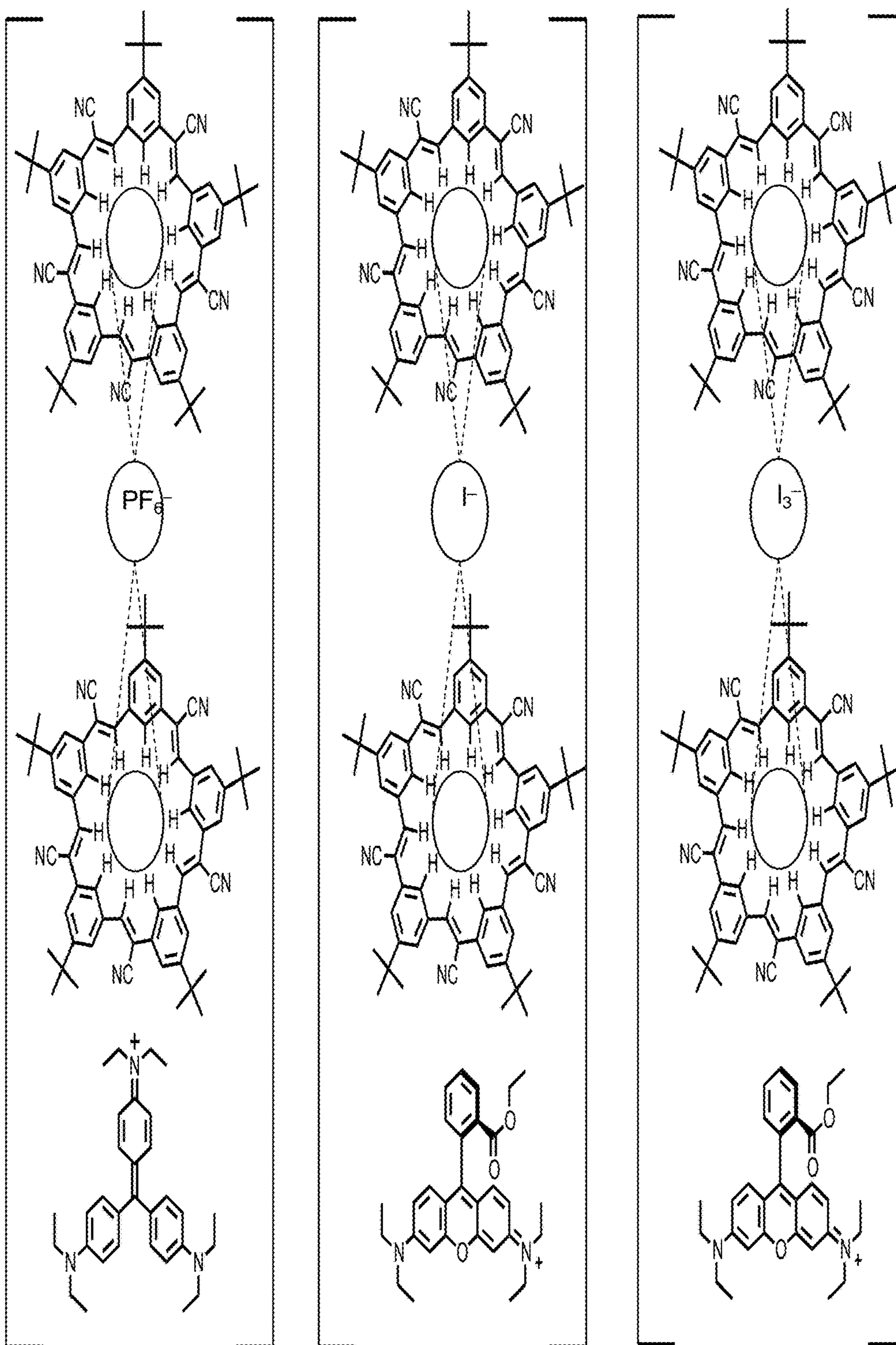
AB-SMILES (cyanostar) 2 (PF 6 ) (Ethyl violet)
