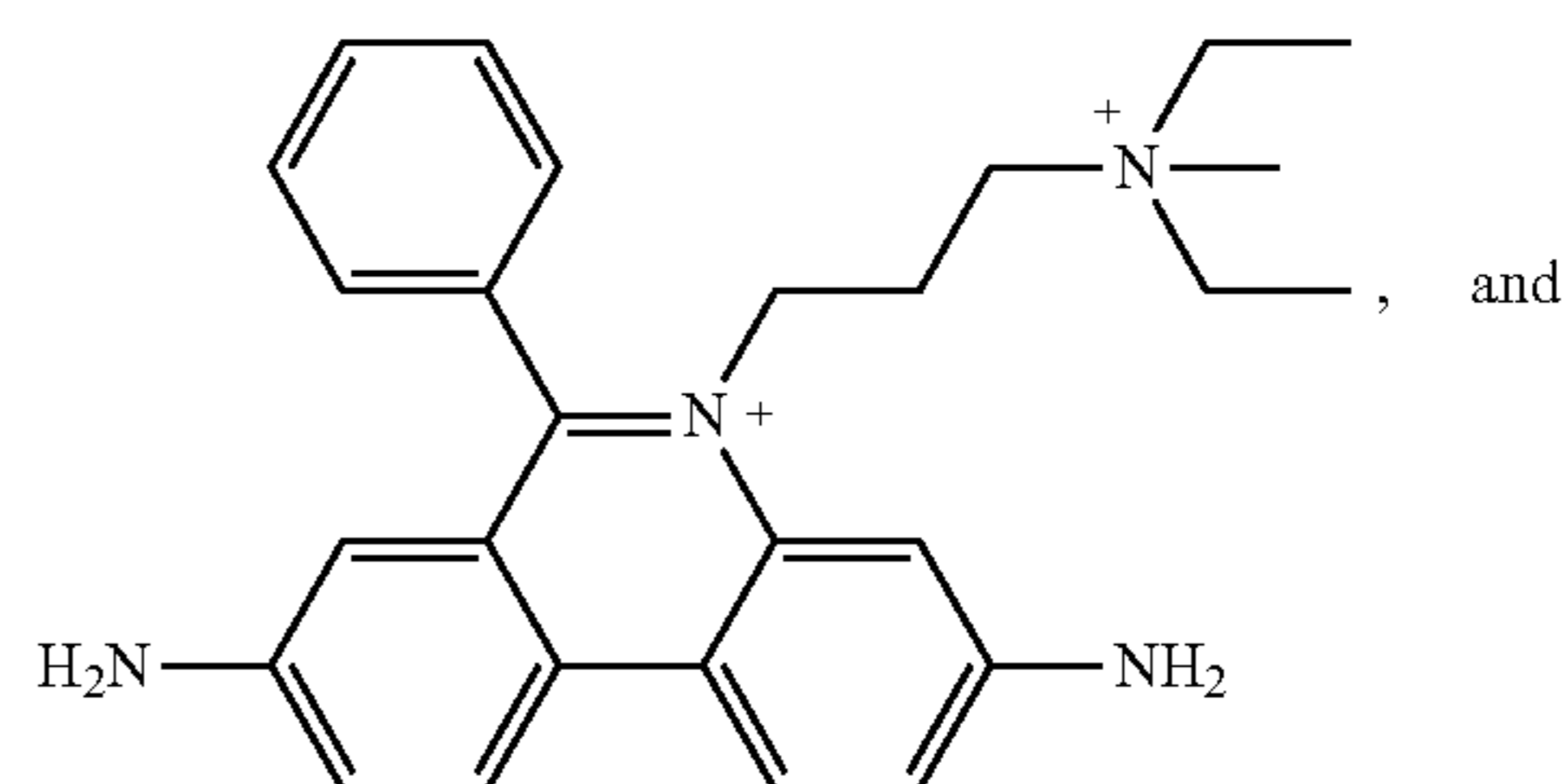
(Propidium)
