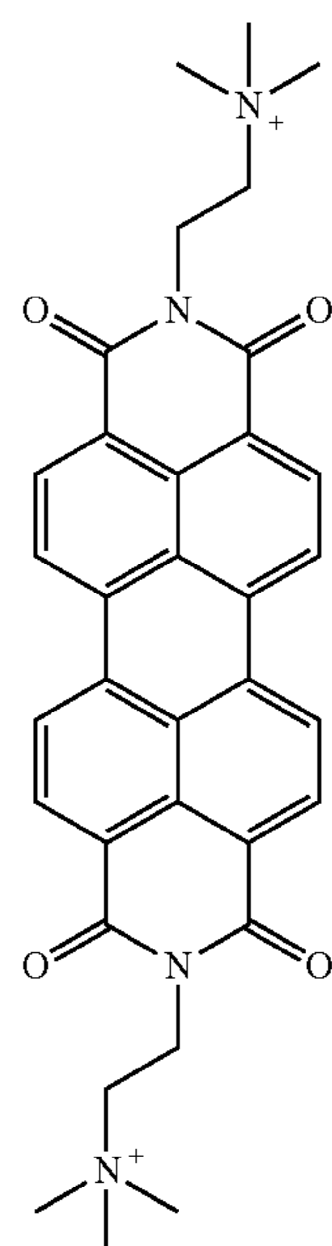
(Perylene diimide)
