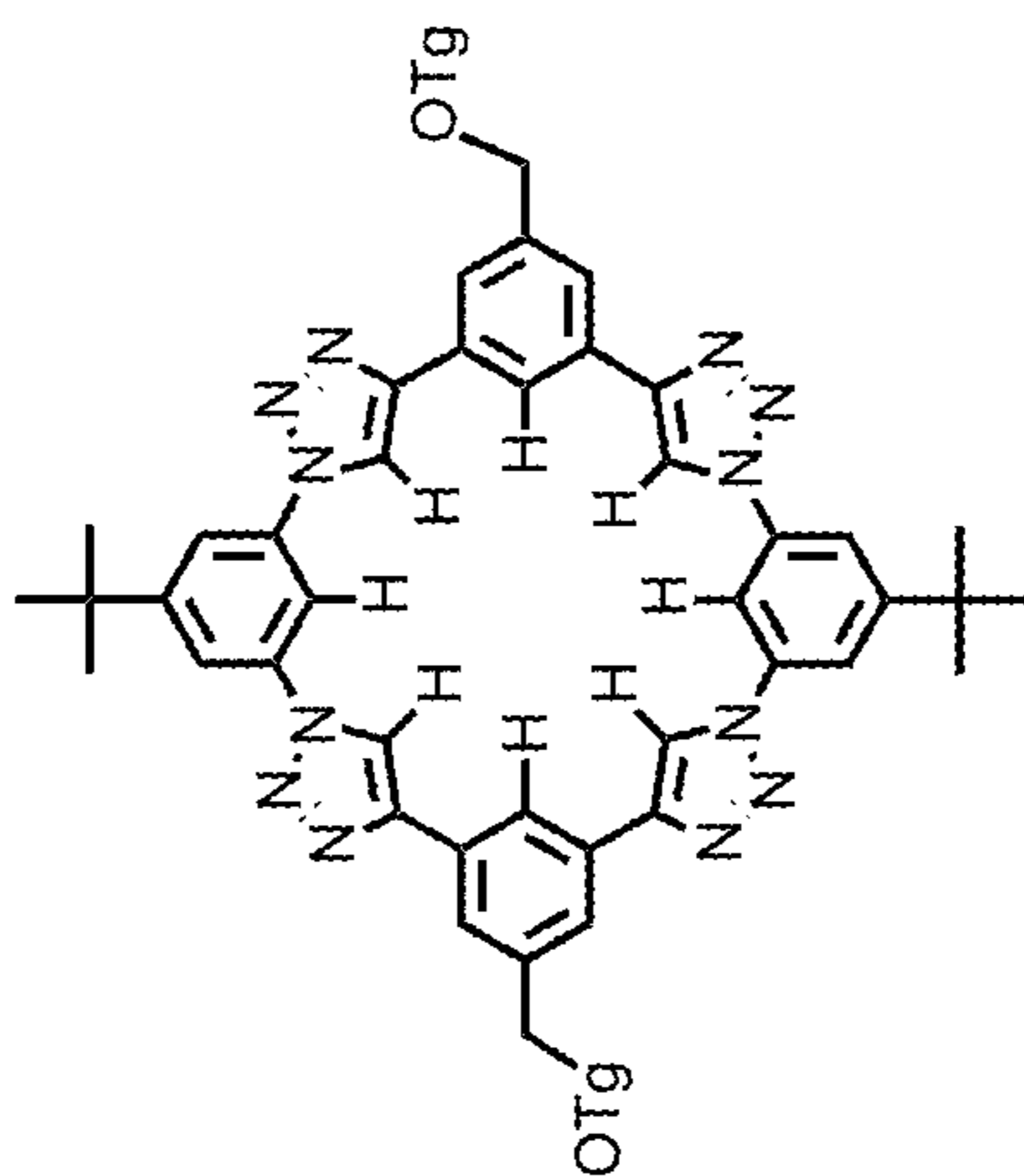
Triazolophane
