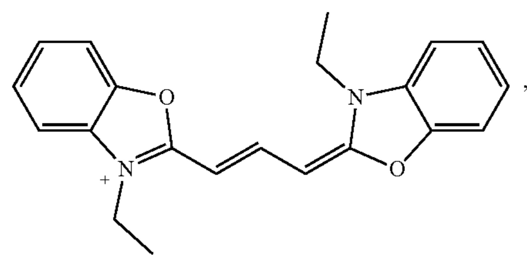
(Cyanine DIOC 2 )
