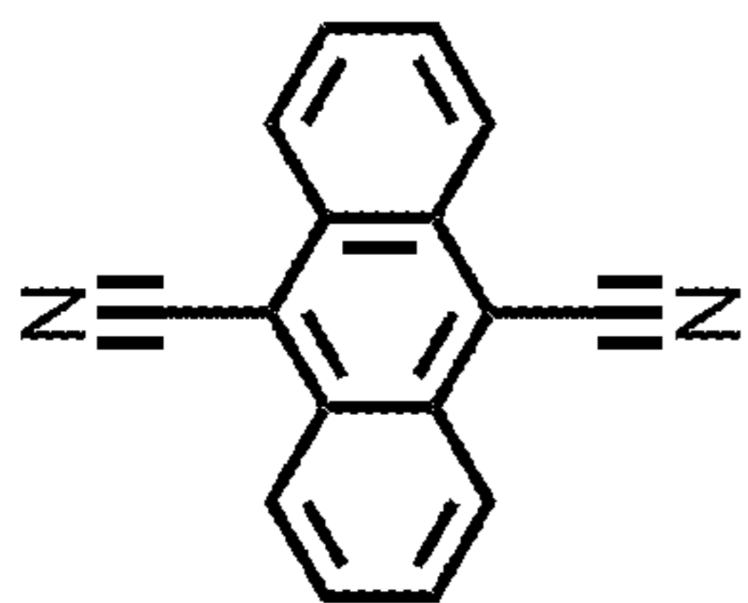
Neutral dye dicyanoanthracene
