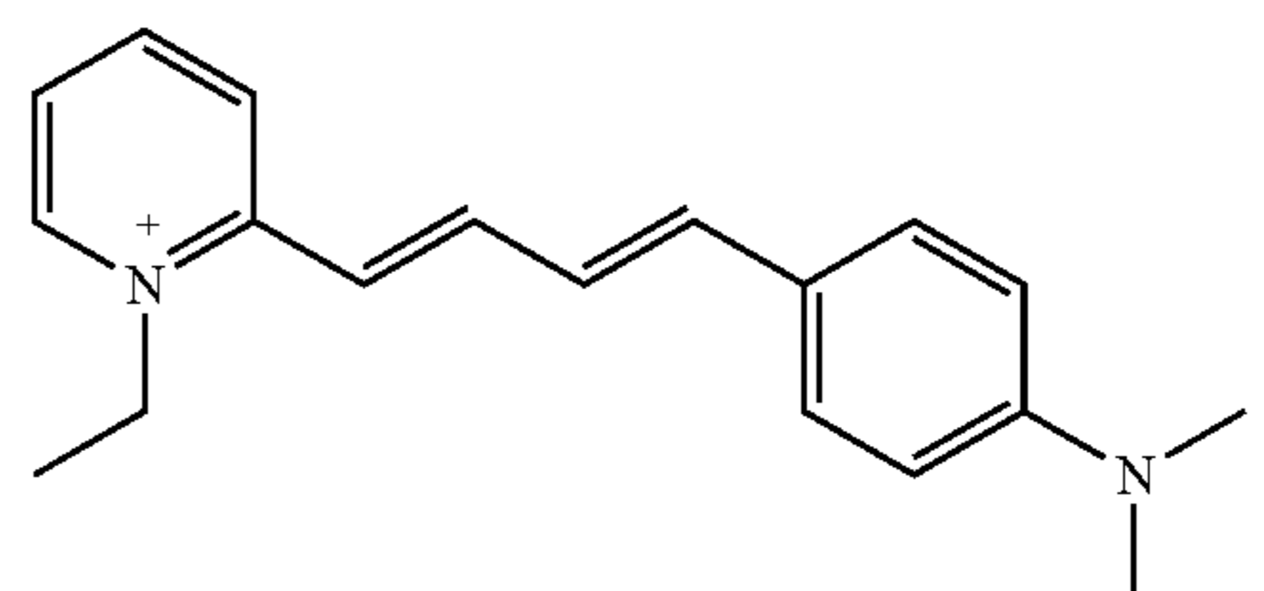
(Pyridin 1)
