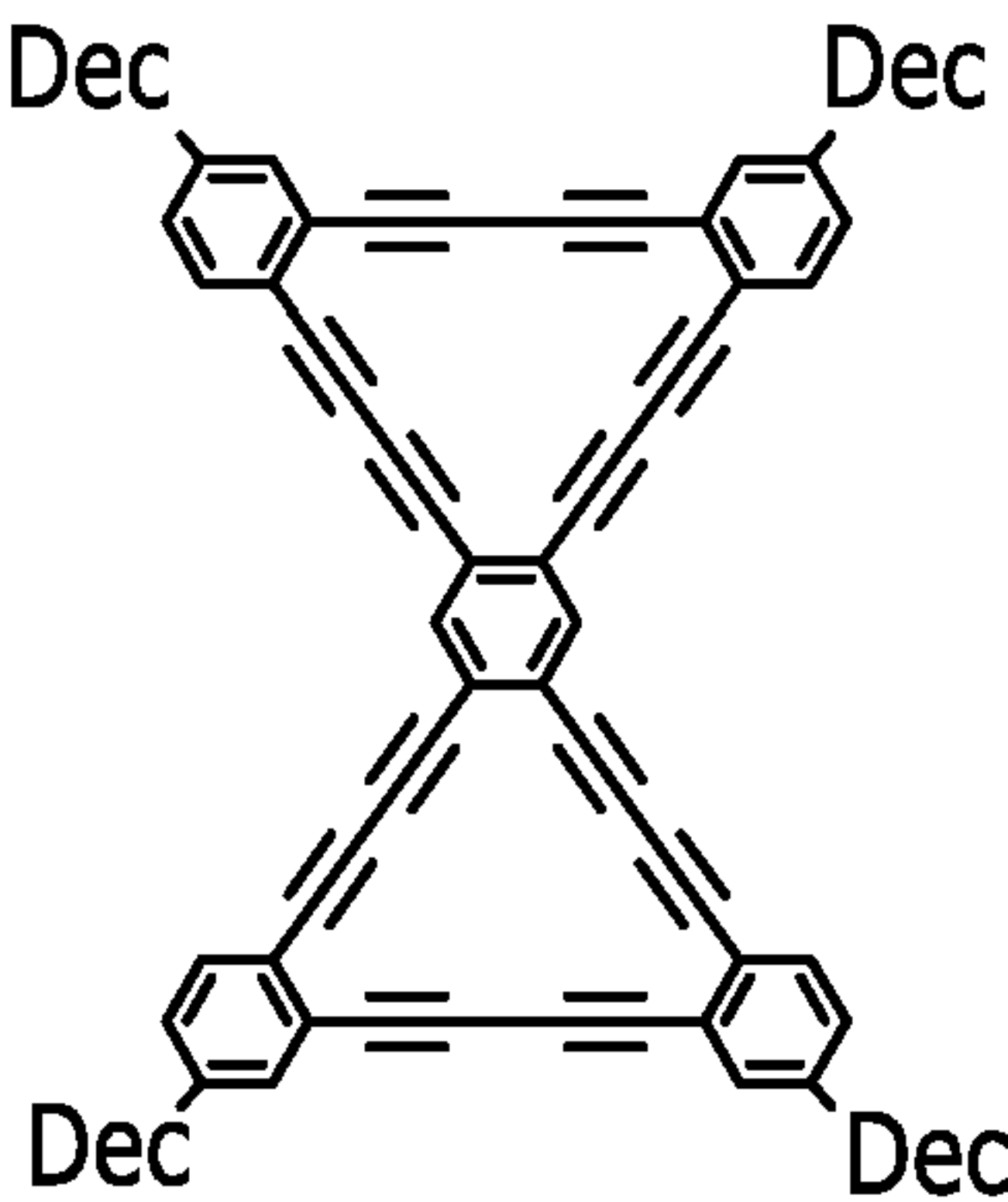
Bis[18]Annulene BT
