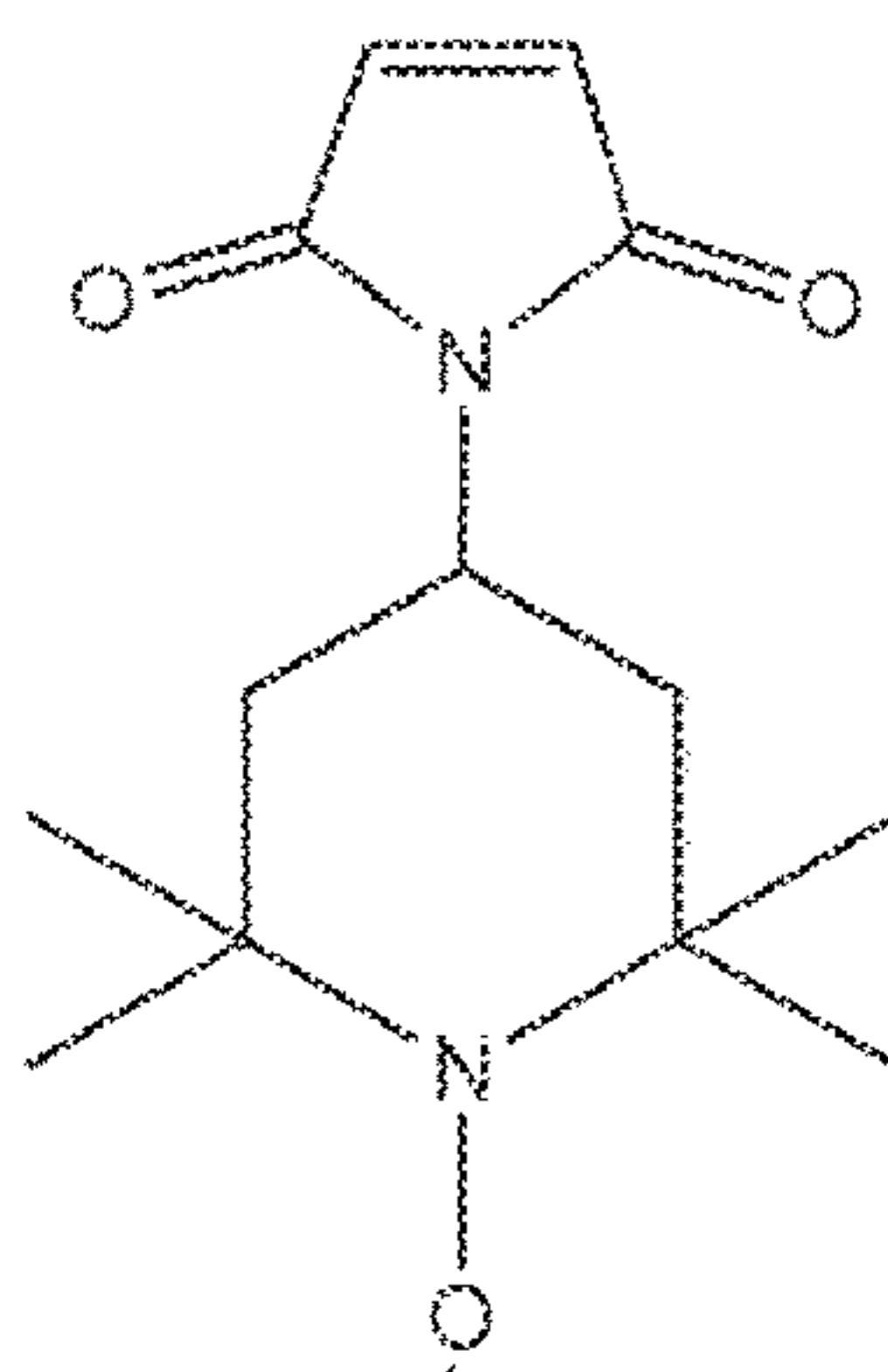
4-Maleimido-TEMPO, LogP=2.9
