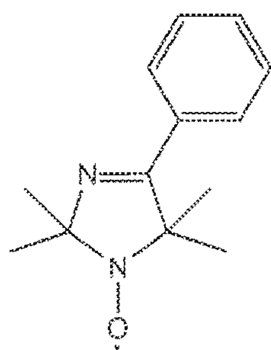
Nitronyl nitroxide, LogP=1.7
