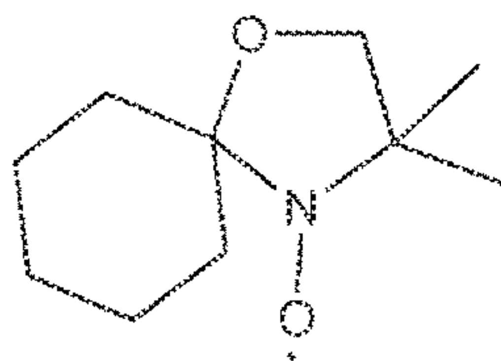
Doxyl radical, LogP=2.6
