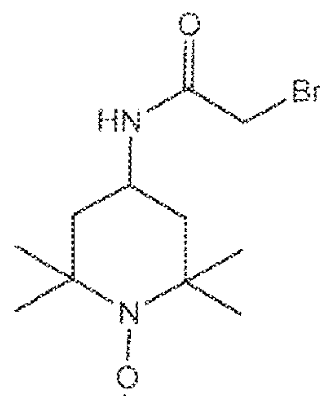
4-(2-Bromoacetamido)- TEMPO, LogP=1.9
