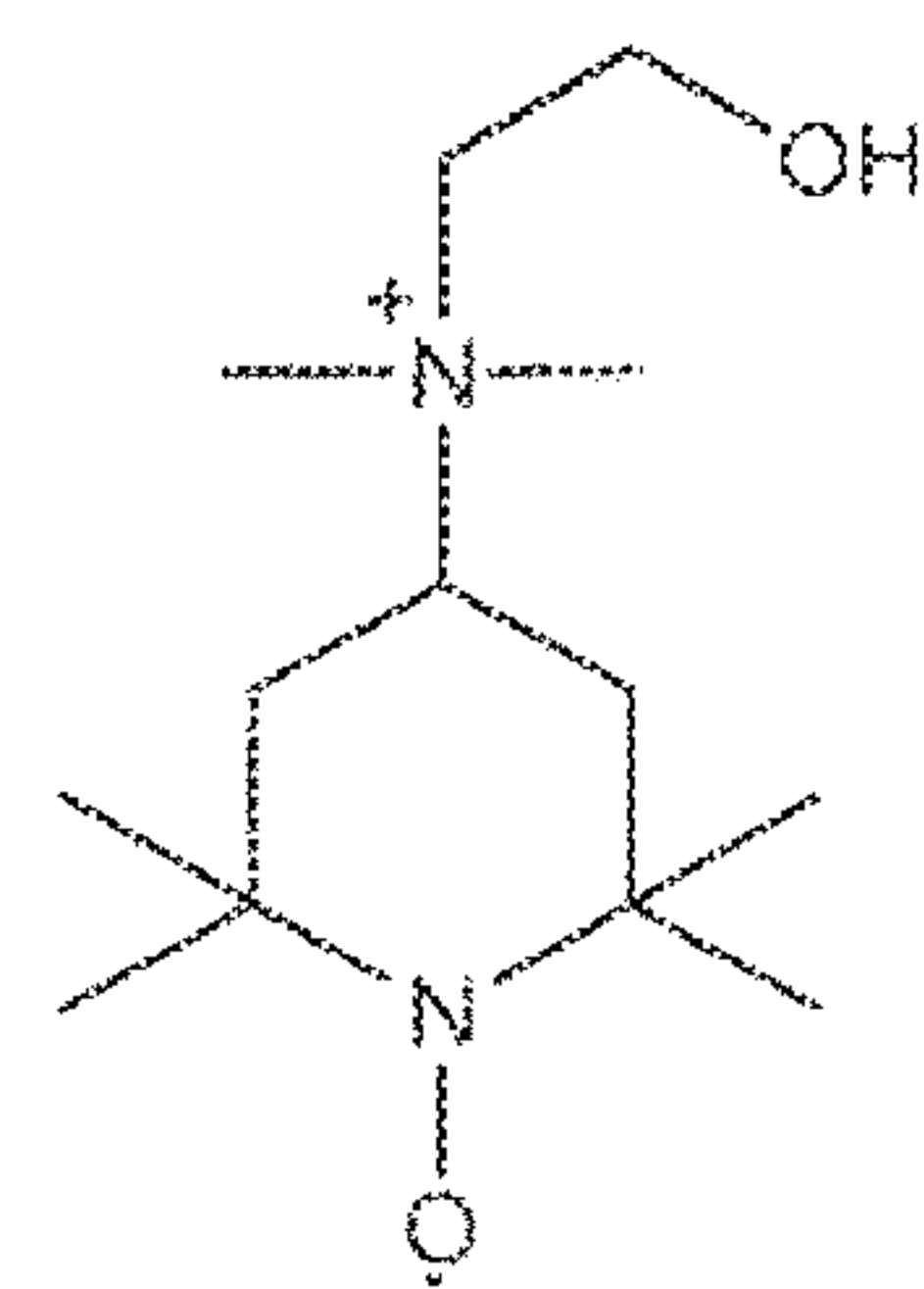
TEMPO choline, LogP=2.5
