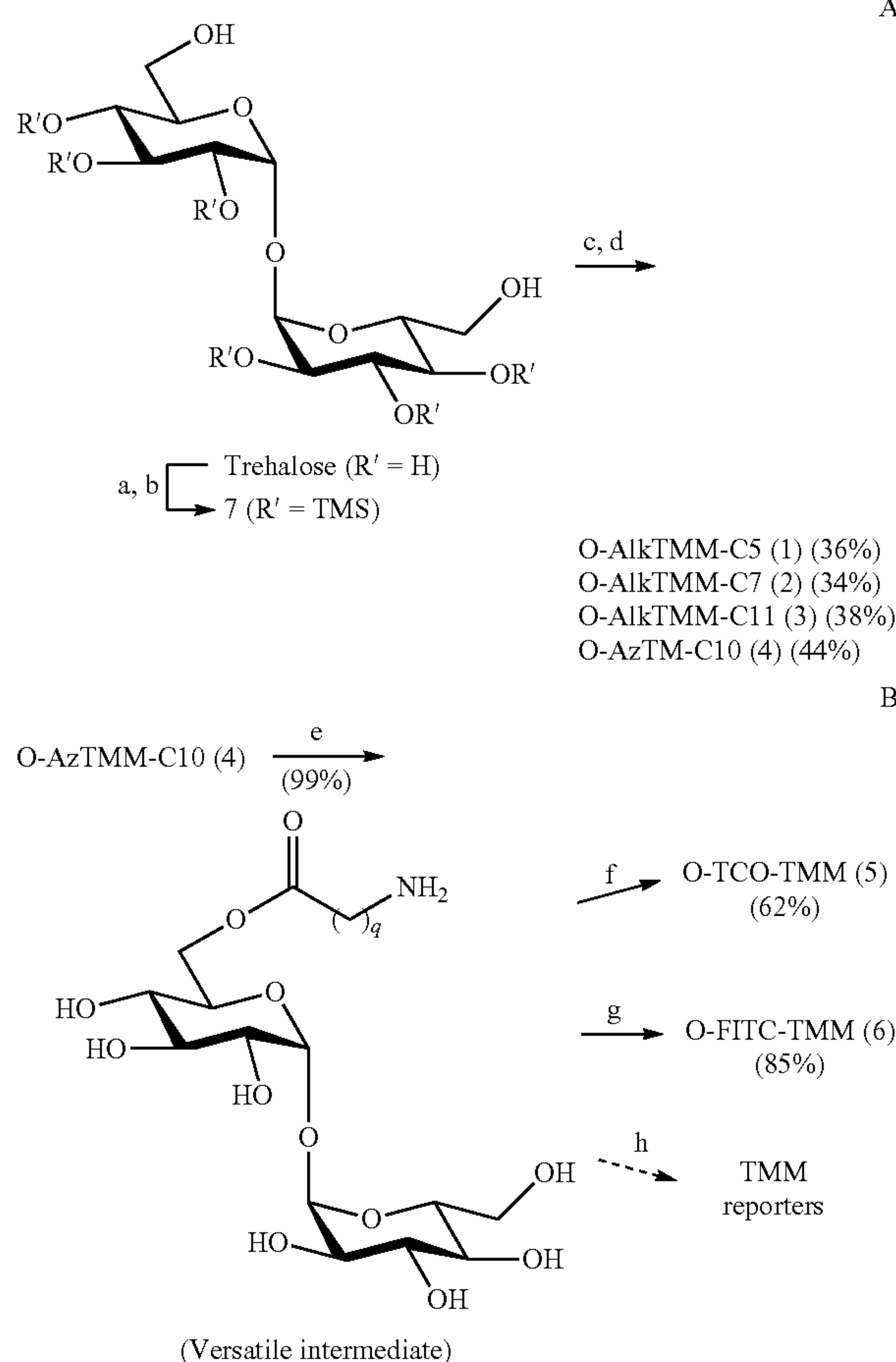
Scheme 3
