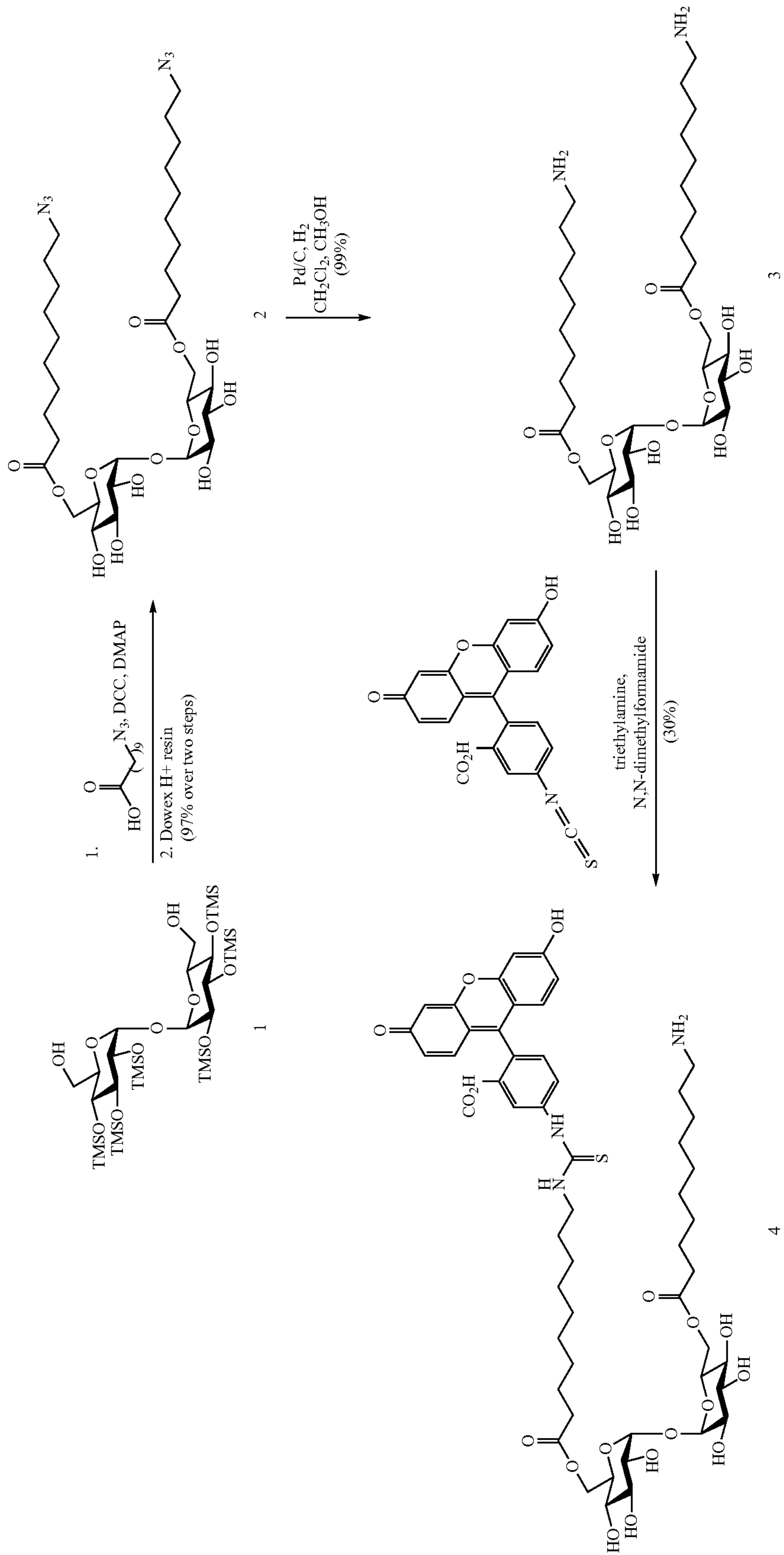
Scheme 4
