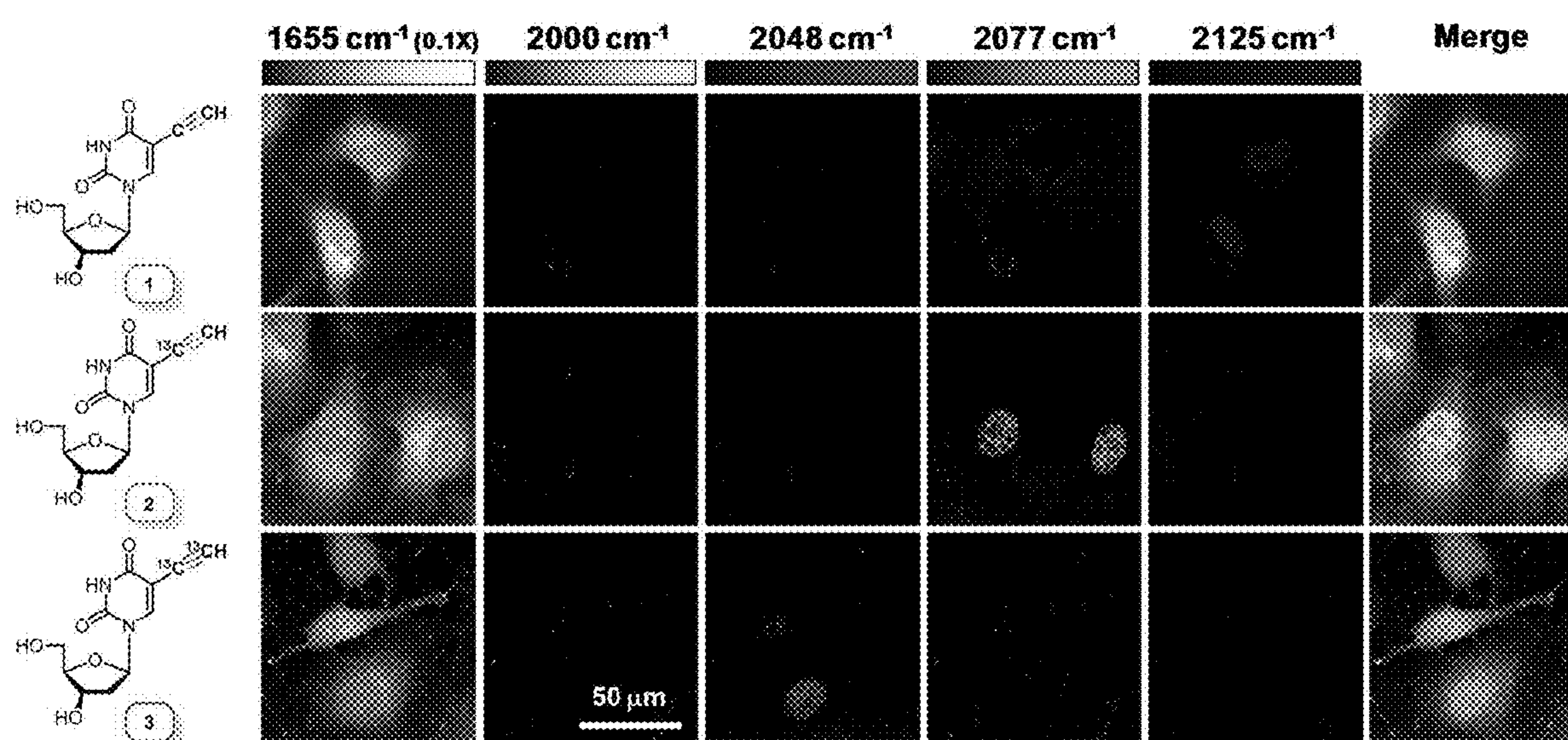
Multicolor imaging of DNA synthesis (EdU (1); EdU- 13 C (2) and EdU- 13 C 2 (3)).
