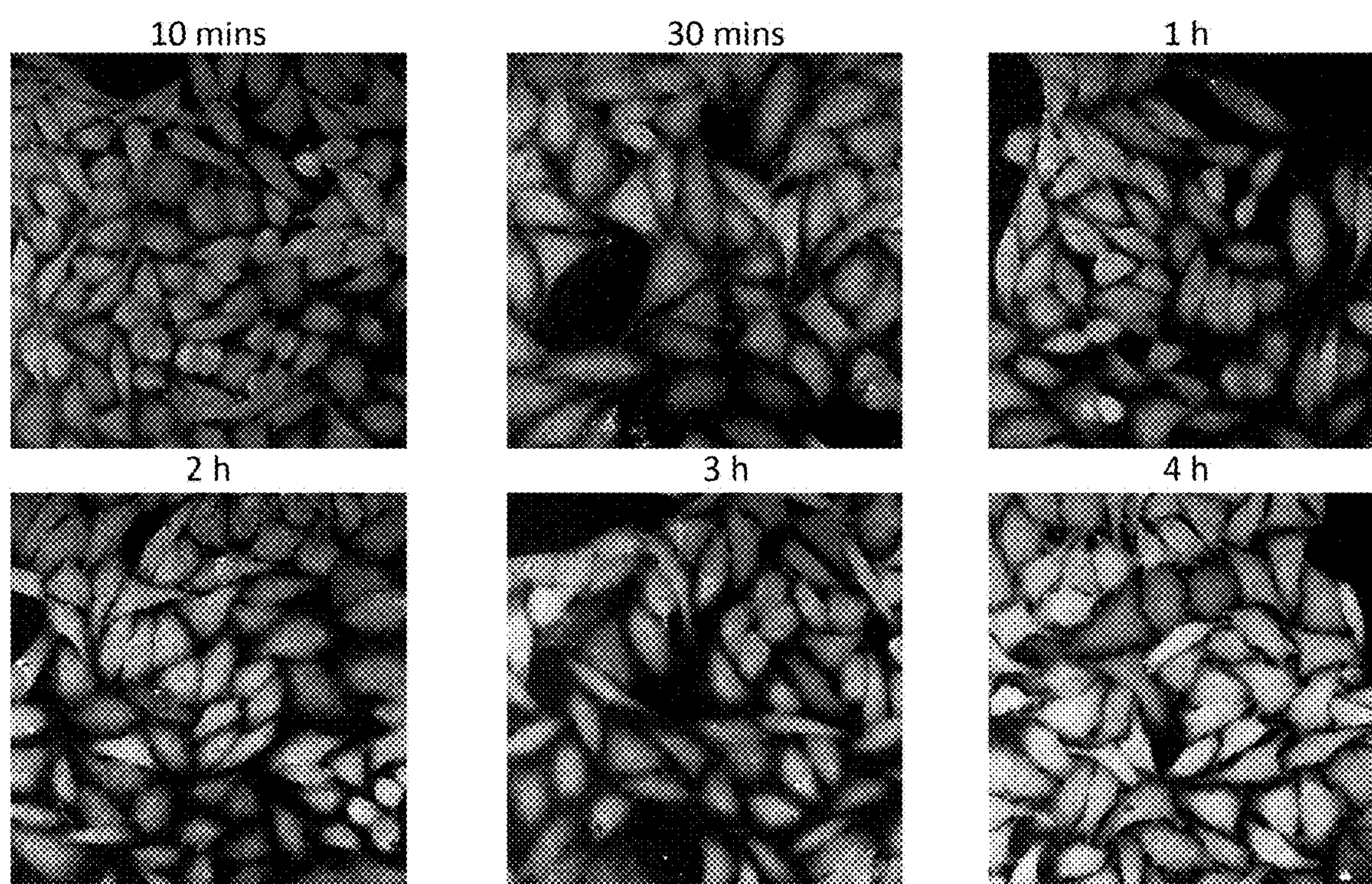
Time-dependent alkyne-glucose (32 mM) uptake in live HeLa cells for 10min, 30 min, 1h, 2h, 3h and 4h time point. The glucose signal inside mammalian cells is increasing over time
