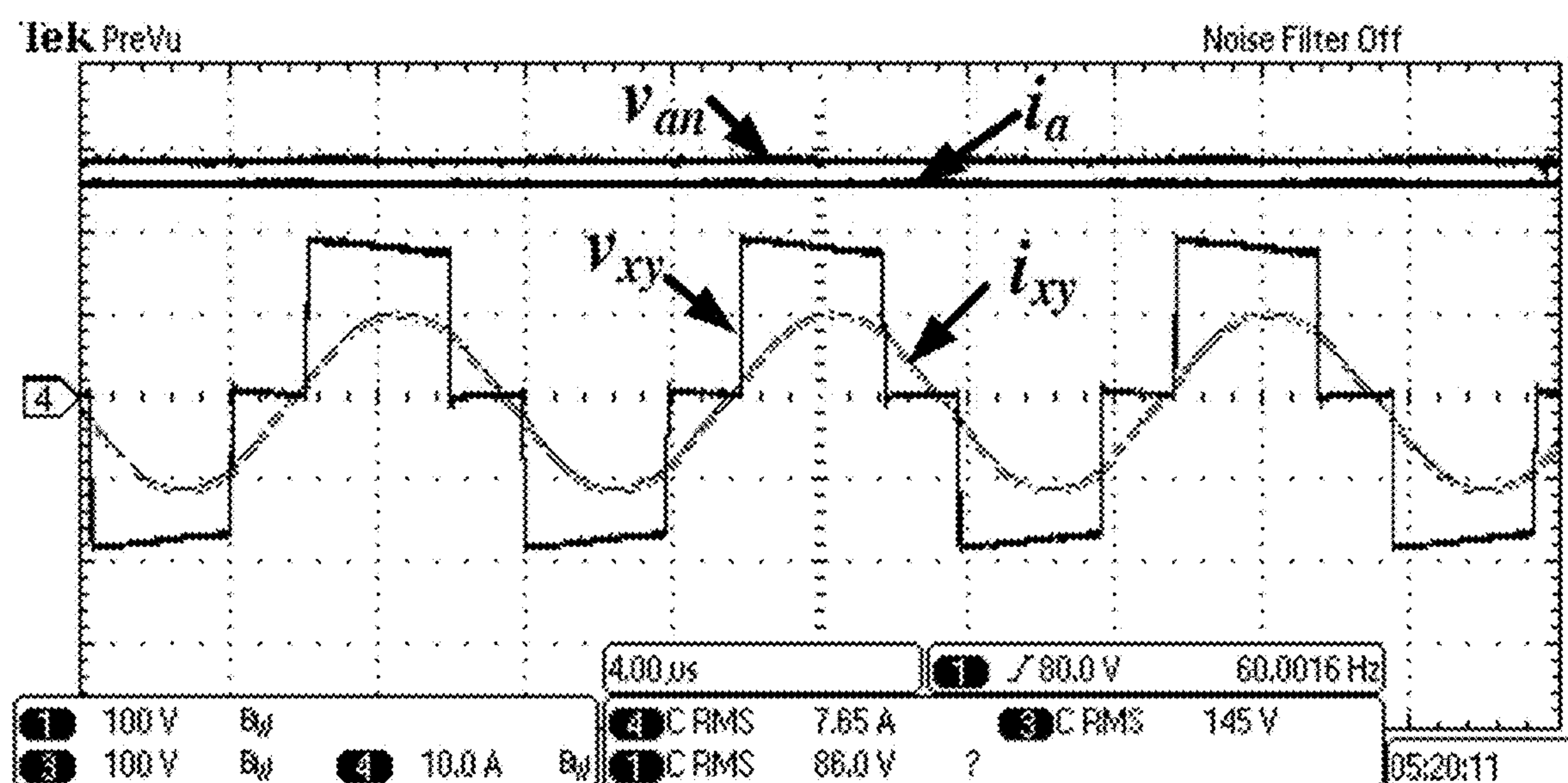
Plot of 3-level tank voltage ( v_{xy} ) at equal d_{pu} and d_{on}
