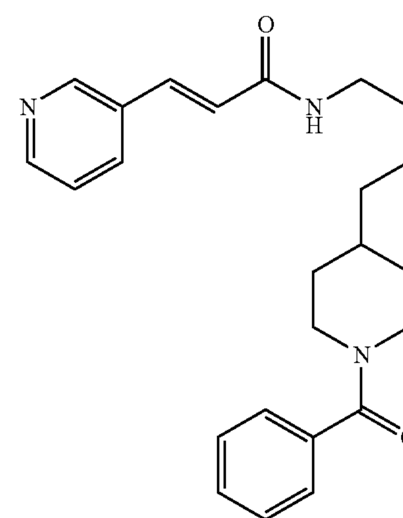
FK866 (APO866)
