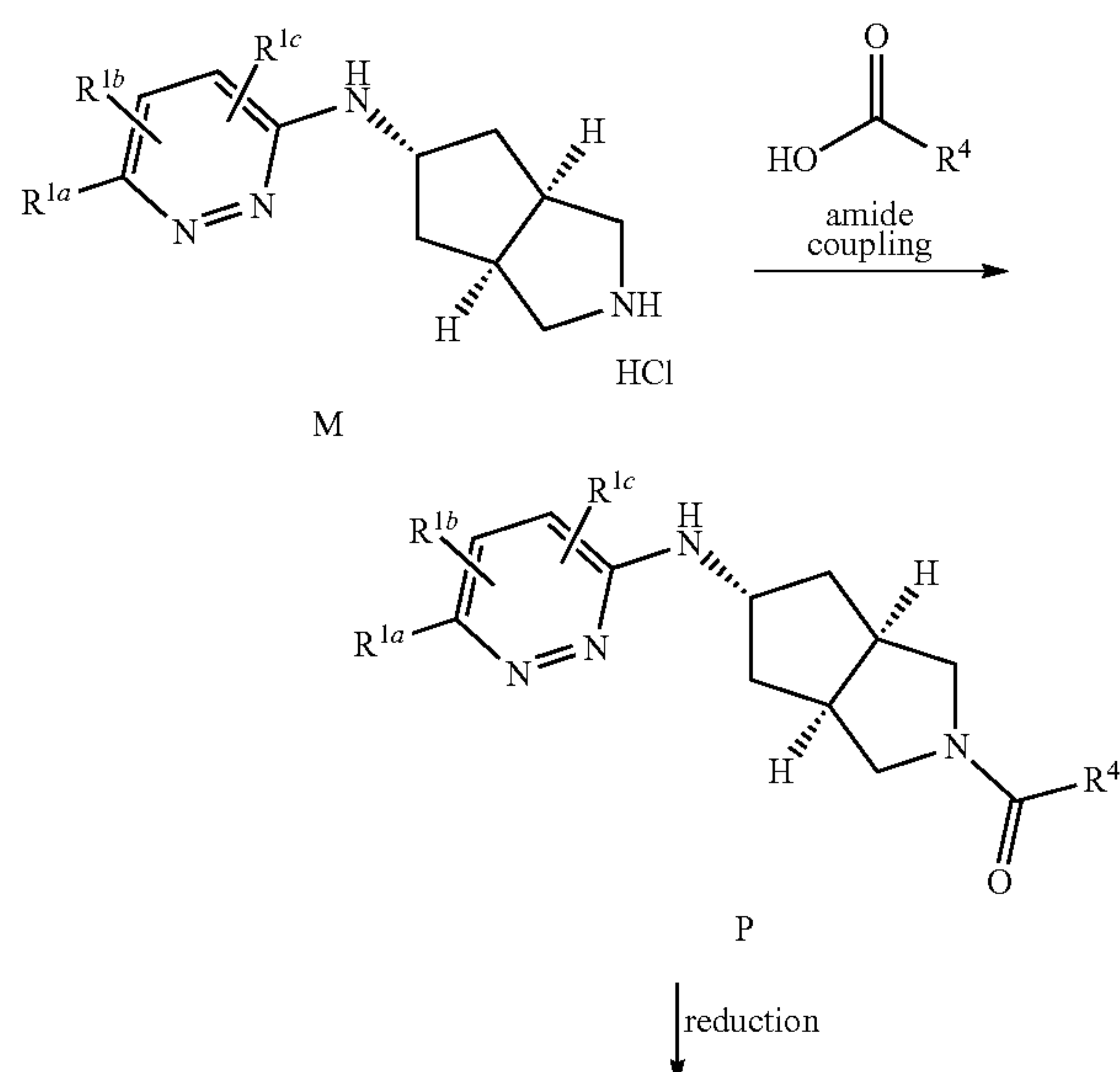
Scheme 6
