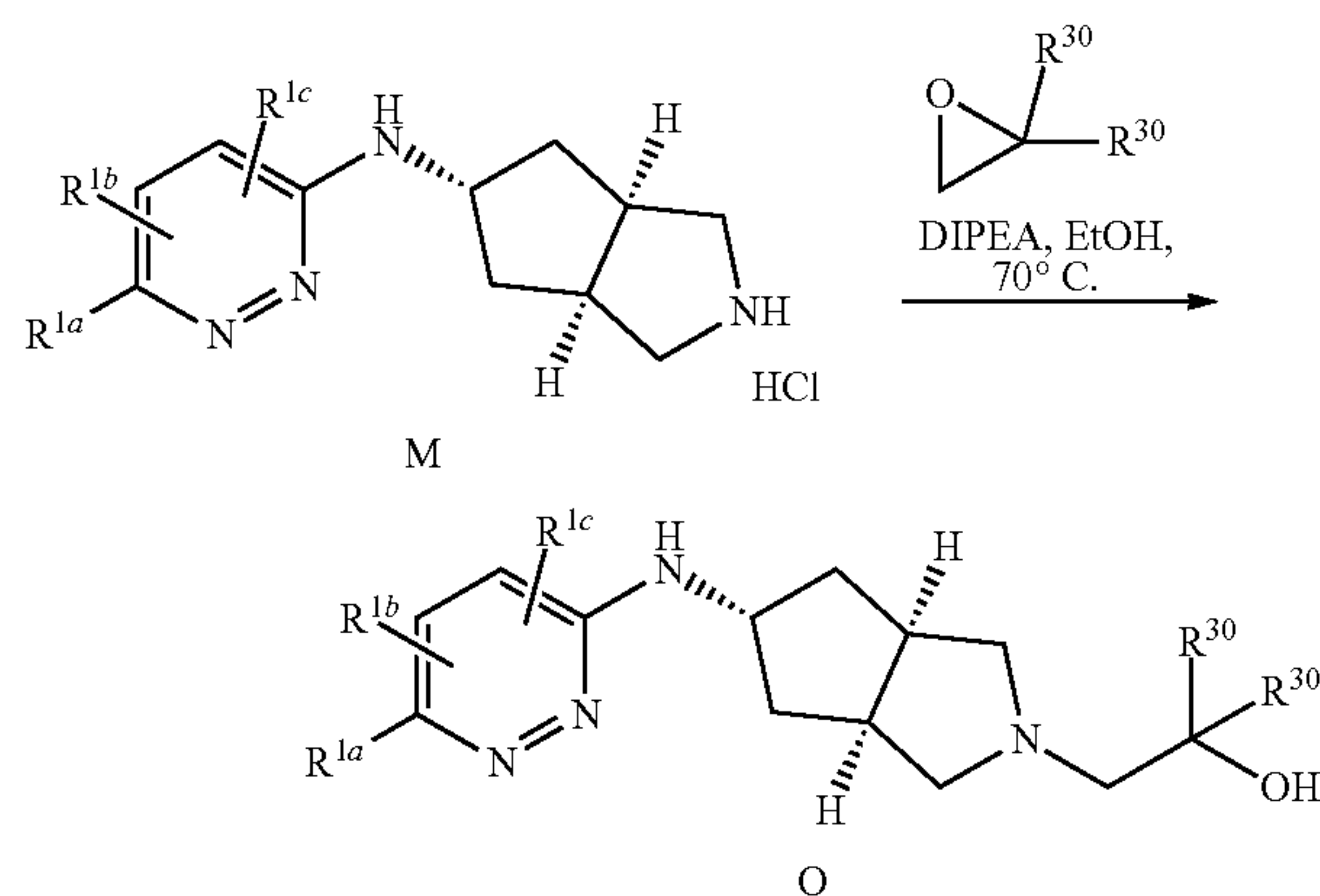
Scheme 5
