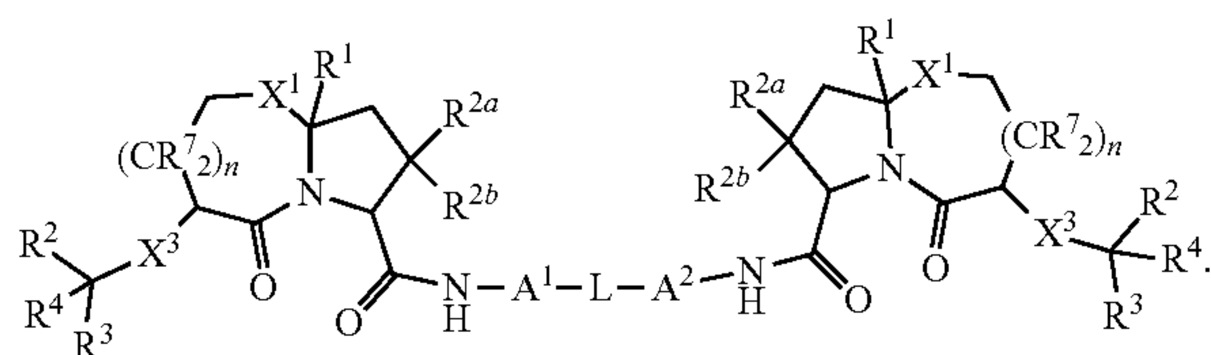
Formula III
