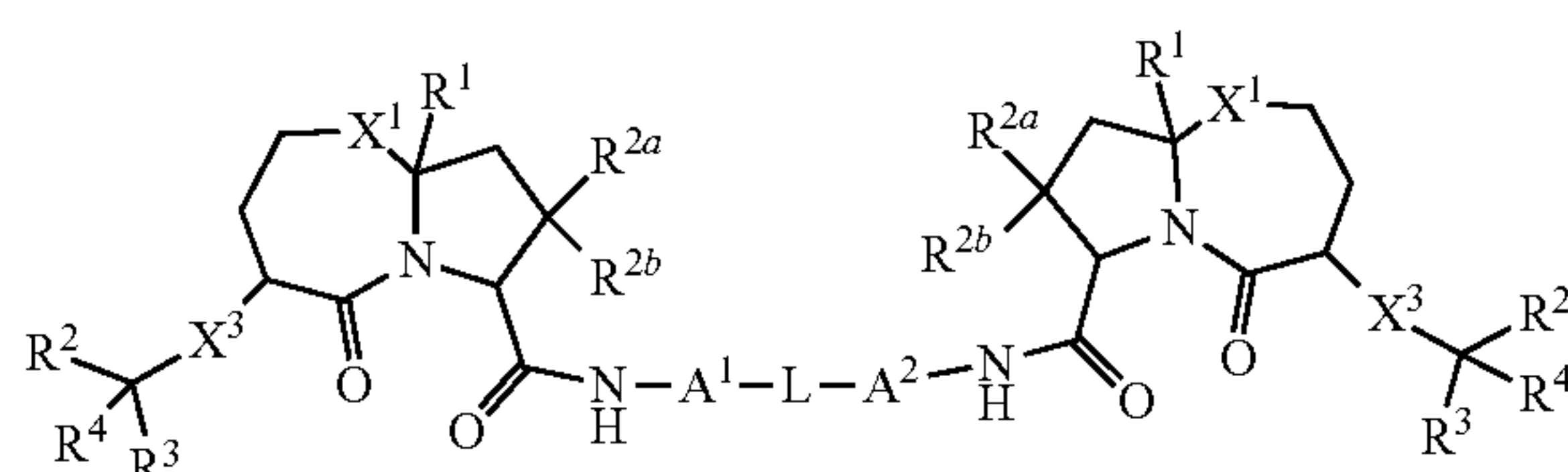
Formula II
