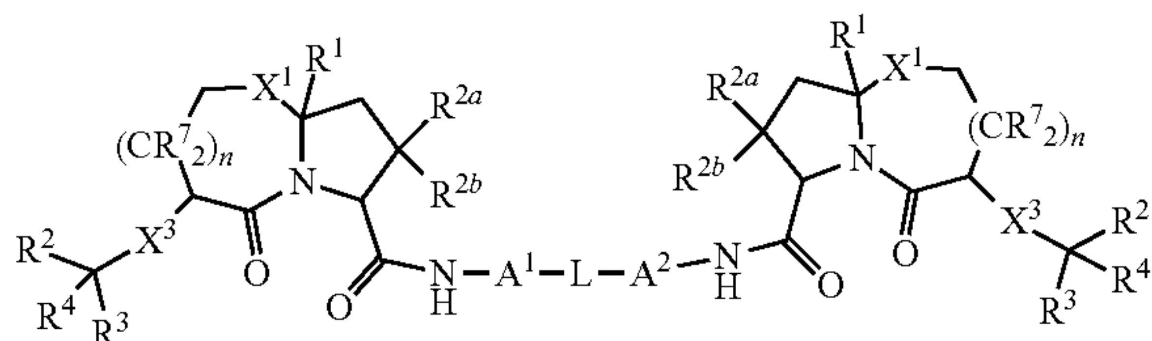
Formula (I)
