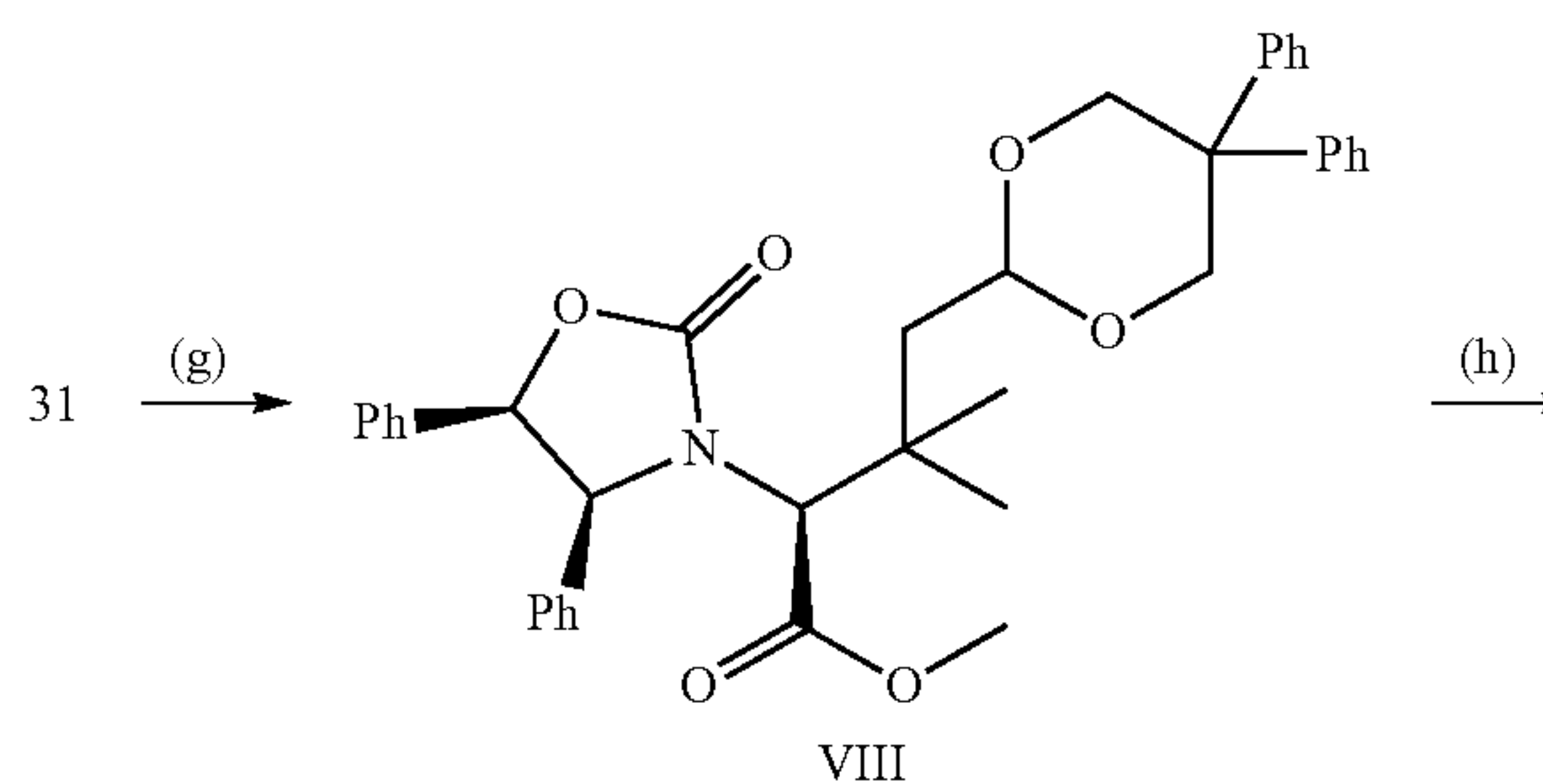
Scheme 2
