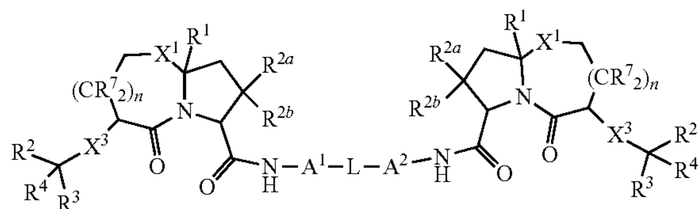
Formula (I)
