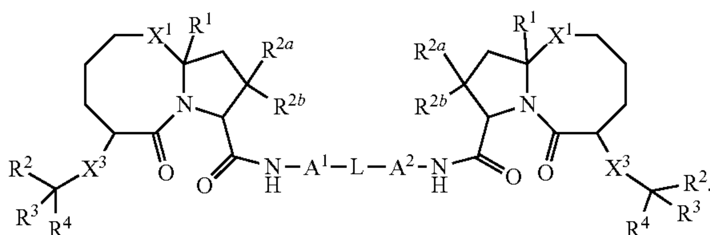
Formula III
