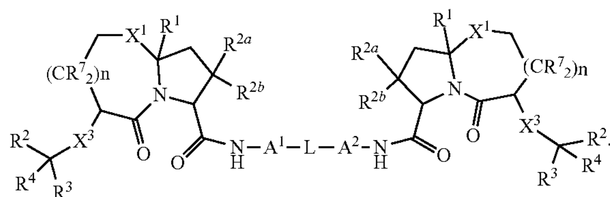
Formula (I)
