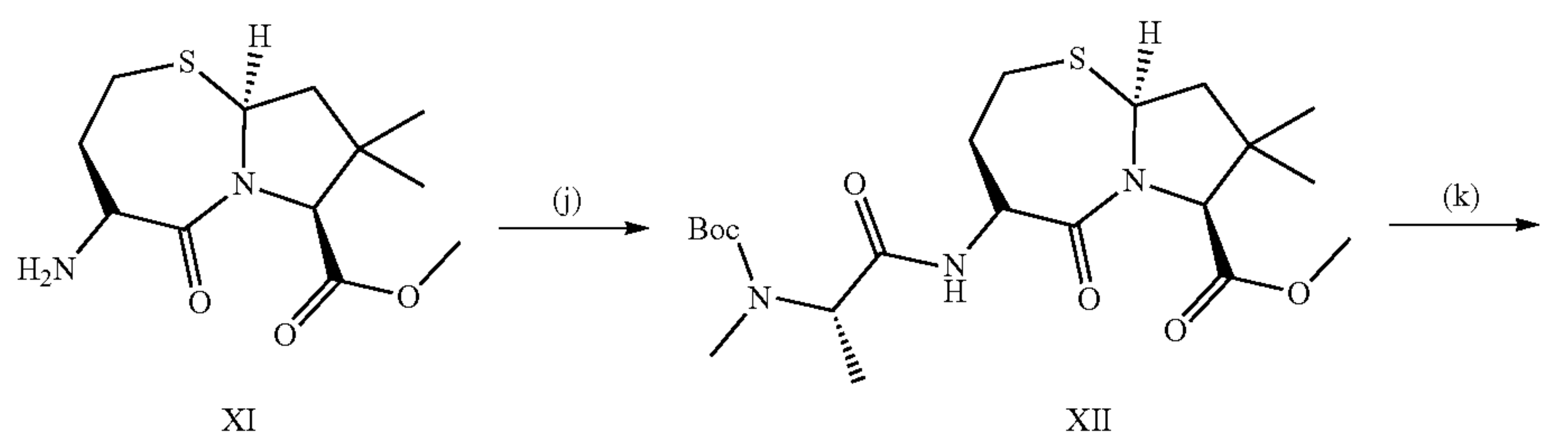
Scheme 3
