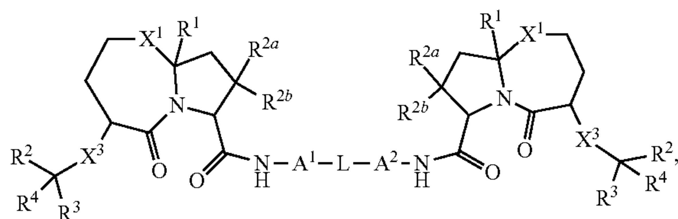
Formula II
