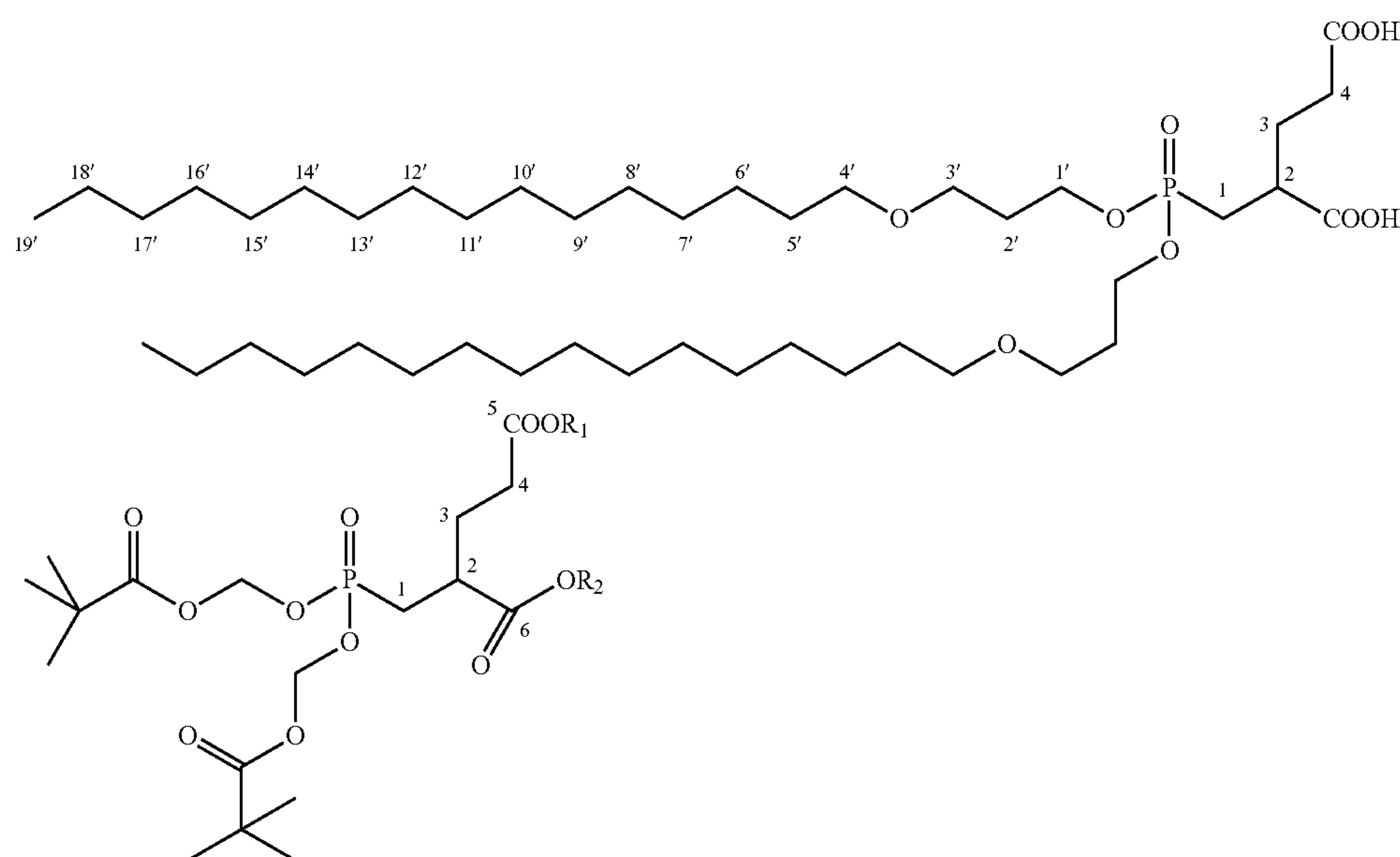
General formula for compounds: MK-798, MK-803, MK-804, TT-201212A, TT-150313 ( R_1, R_2 = H, \text{alkyl} )
