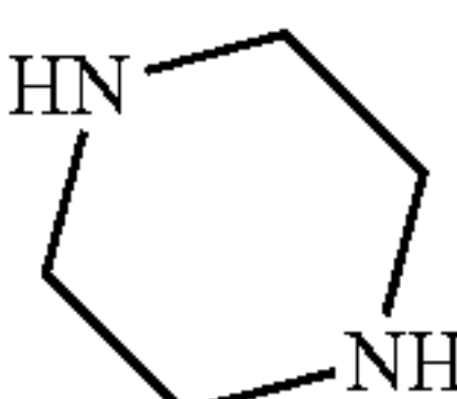
piperazine
