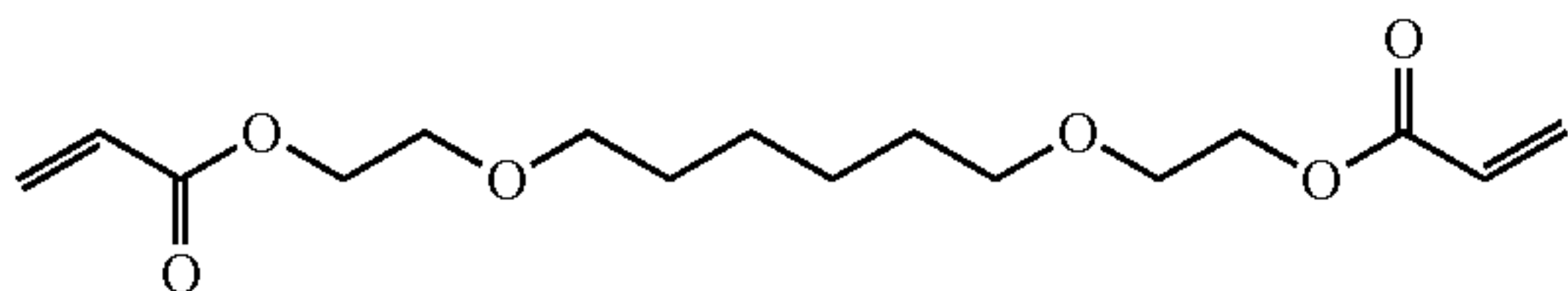
2,2'-(hexane-1,6-diylbis(oxy))bis(ethane-2,1-diyl) diacrylate
