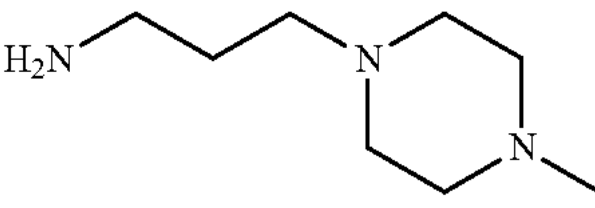
1-(3-aminopropyl)-4-methylpiperazine
