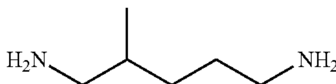
2-methylpentane-1,5-diamine
