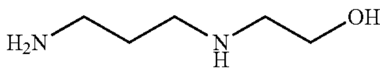
2-(3-aminopropylamino)ethanol
