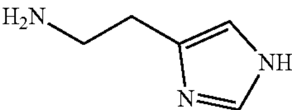
histamine
