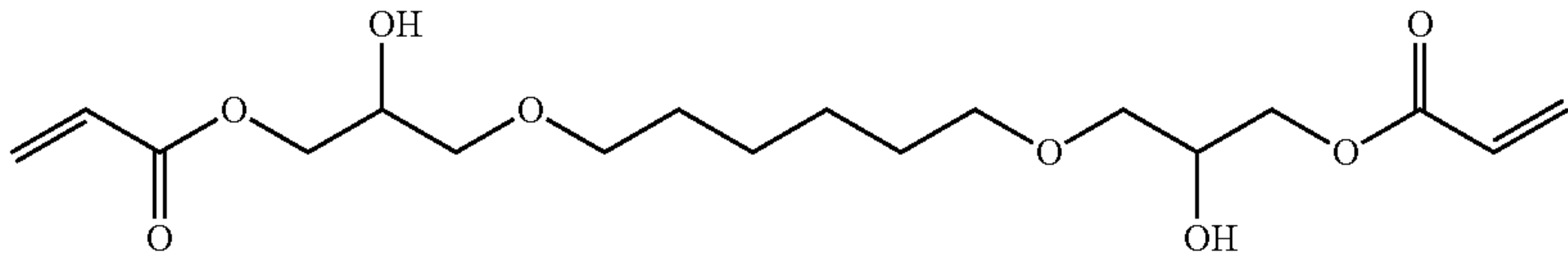
1,6-(hexanediylbis[oxy(2-hydroxy-3,1-propanediyl)]) bisacrylate
