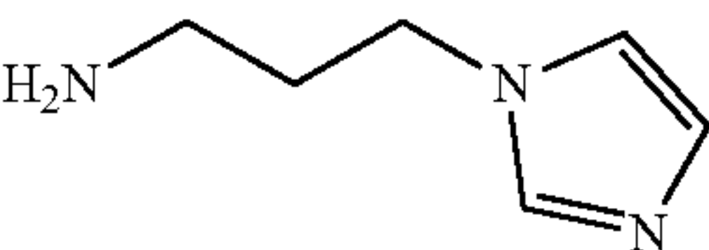
N-(3-aminopropyl)-imidazole
