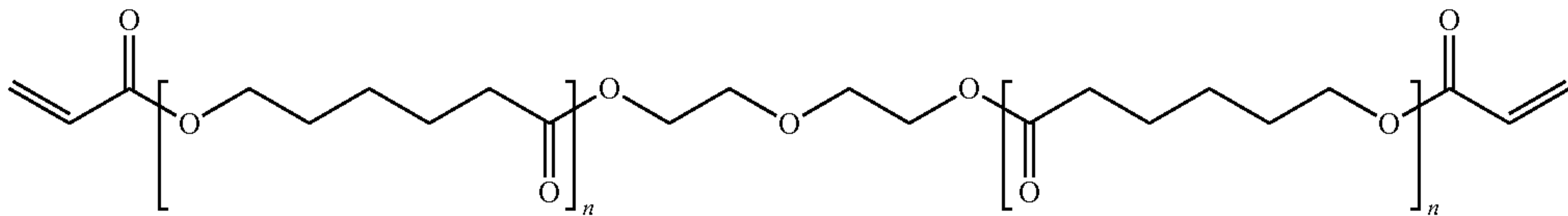
polycaprolactone diacrylate
