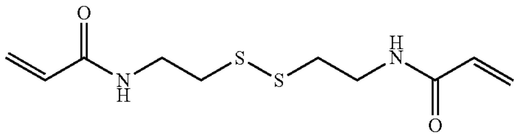
N,N'-bis(acrylyl)cystamine
