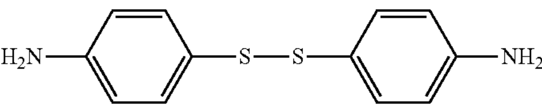
4-aminophenyl disulfide
