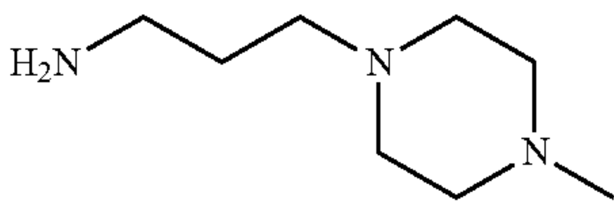
1-(3-aminopropyl)-4-methylpiperazine
