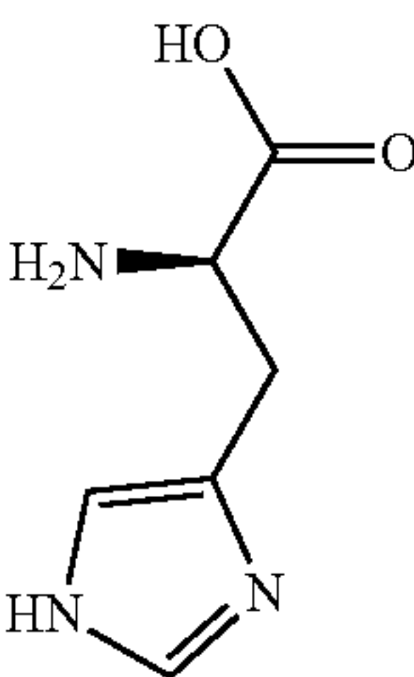
D-histidine
