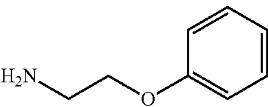
2-phenoxyethanamine
