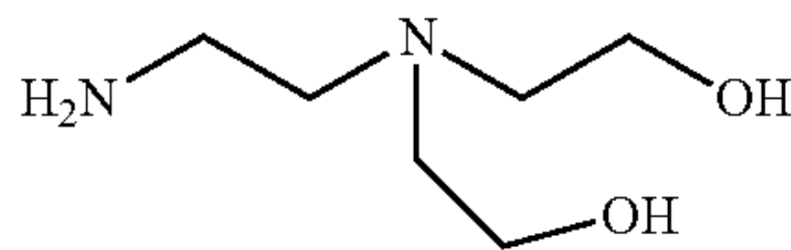
2-2'-(2-aminoethylazanediyl)diethanol
