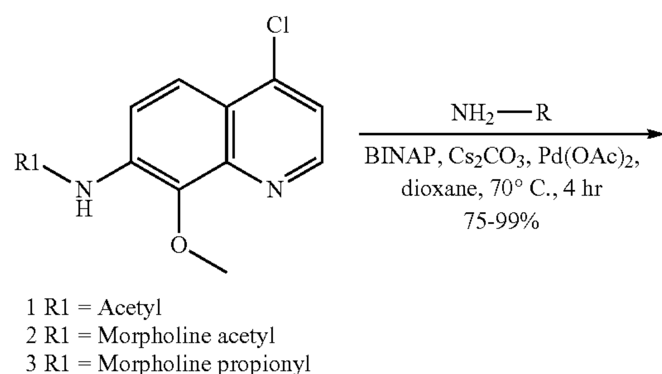
Scheme XIV. Synthesis of series 4 alkyl amine analogs.
